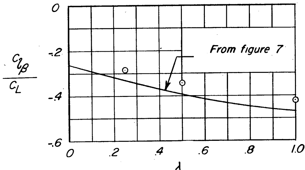
Figure 12.- Comparison of experimental and calculated effect
