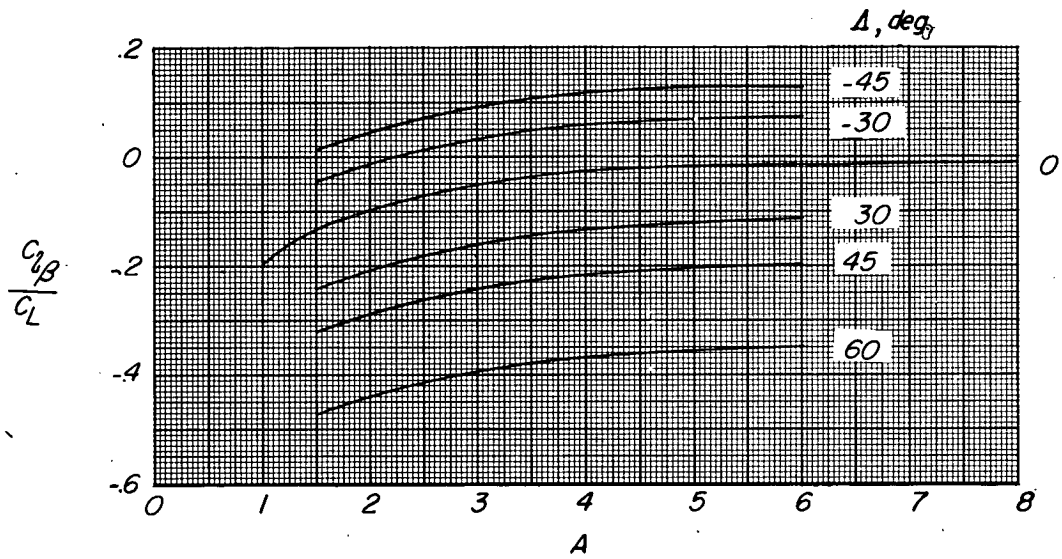
(a) \lambda = 0.
