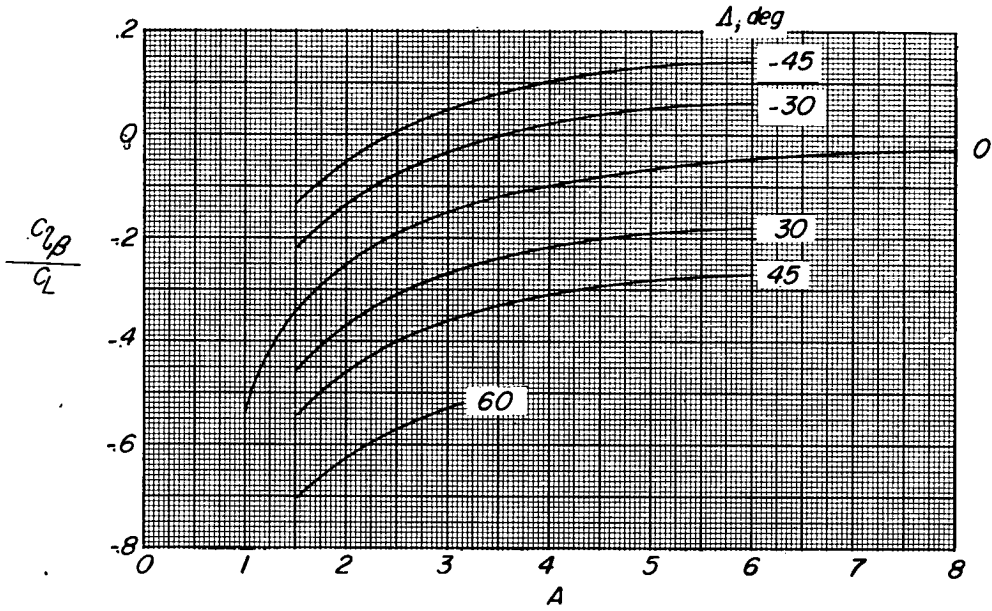
(c) \lambda = 0.50.
