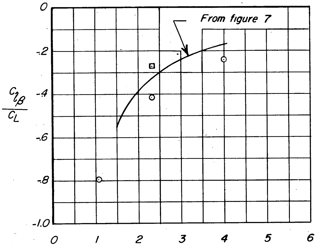
(b) Triangular wings. Figure 11.- Concluded.
