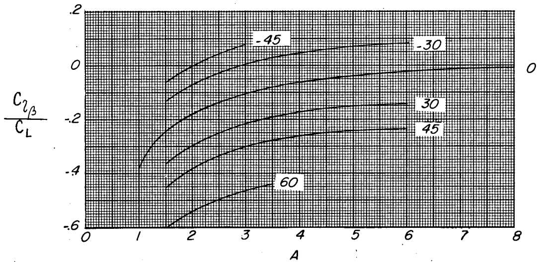
(b) \lambda = 0.25.
