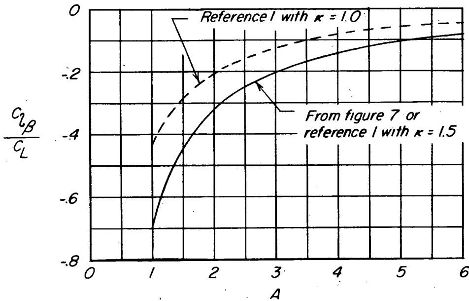
(b) \lambda = 1.00 .
