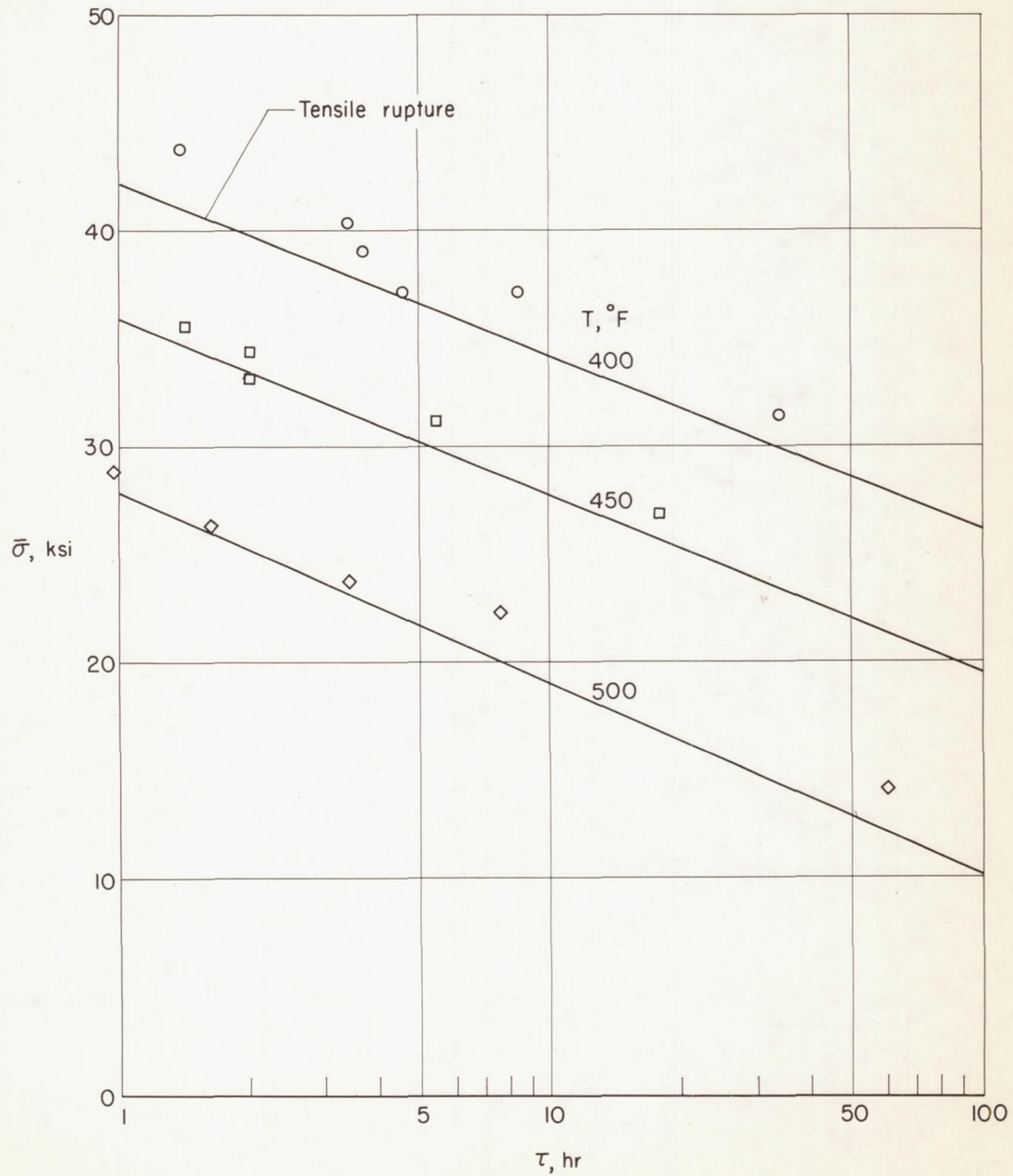
Figure 12.- Comparison of tensile and plate compressive-creep lifetime. b/t = 20 ; 2024-T3 aluminum alloy.
