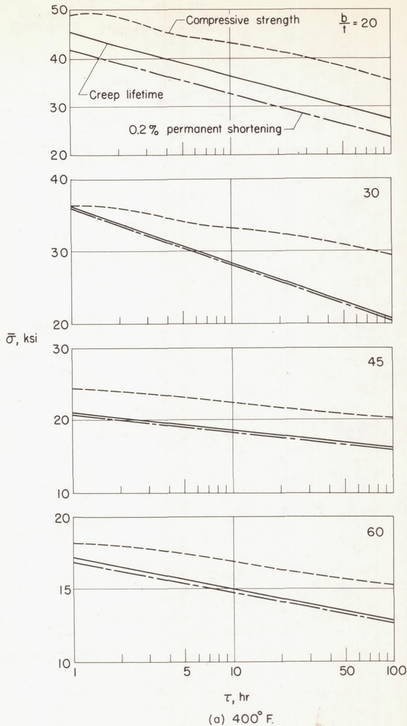
Figure 14.- Comparison of the predicted maximum compressive stresses for exposure times ranging from 1 to 100 hours, experimental stresses that produce creep failure, and experimental stresses that produce 0.2-percent permanent shortening in plates.
