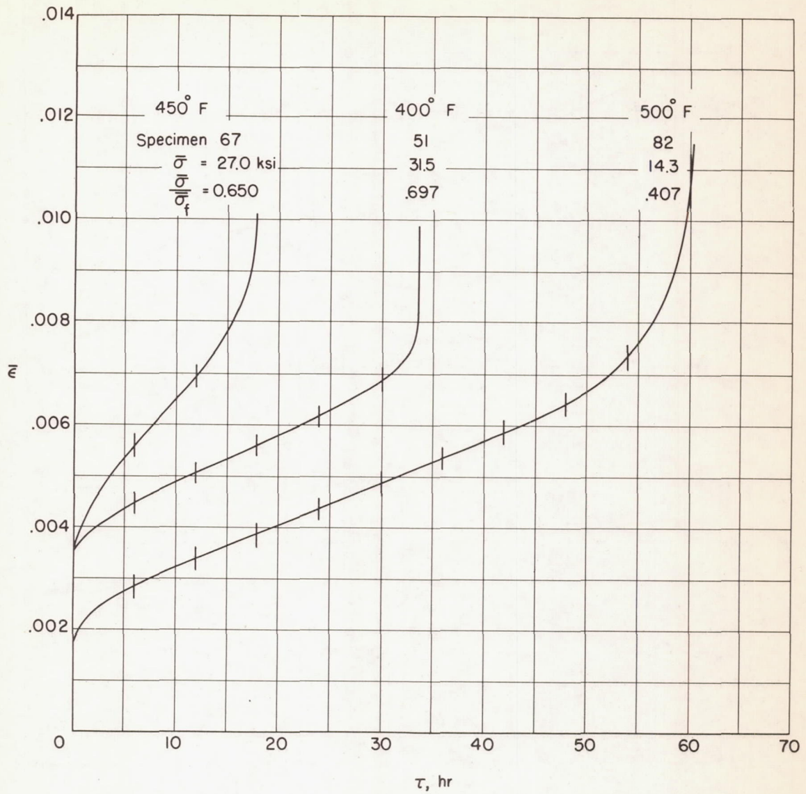
Figure 10.- Plate creep curves from tests interrupted at 6-hour intervals. b/t = 20 .
