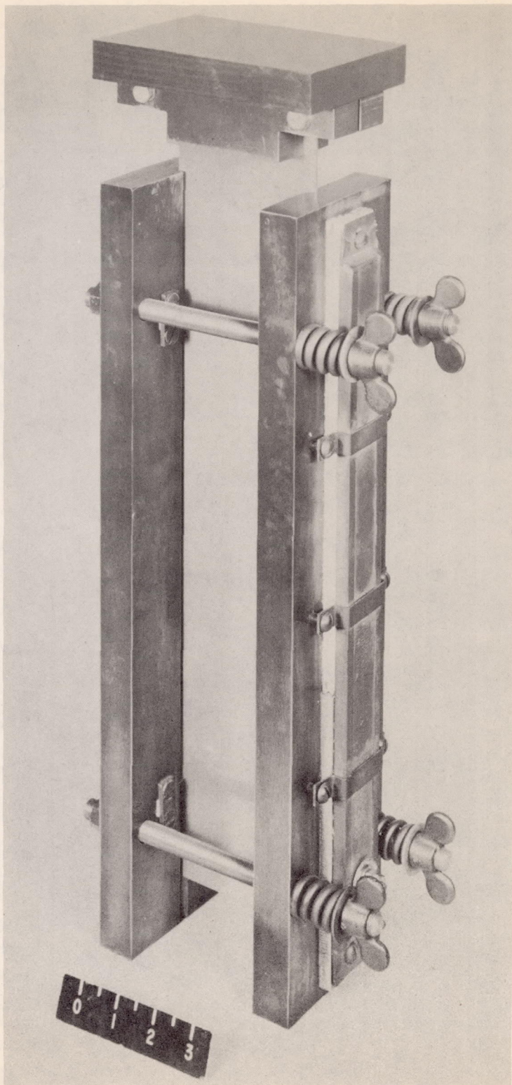
Figure 1.- V-groove fixture. L-90006
