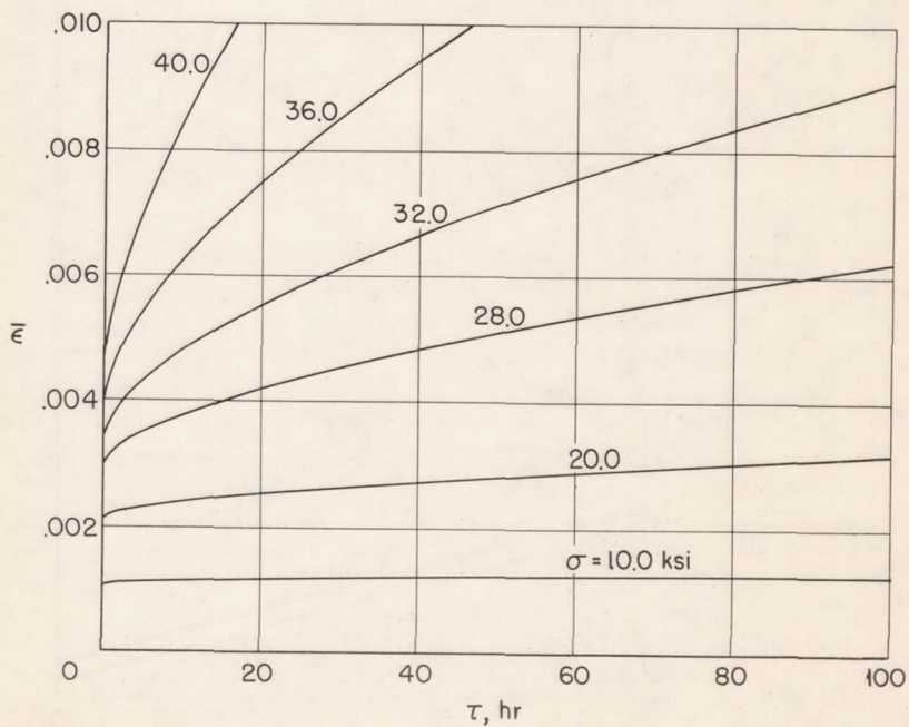
Figure 16.- Curves defined by \epsilon = \frac{\sigma}{E} + Ae^{B\sigma} \tau^K which describe the first and second creep stages for plates with width-thickness ratio of 20 at 400° F.
