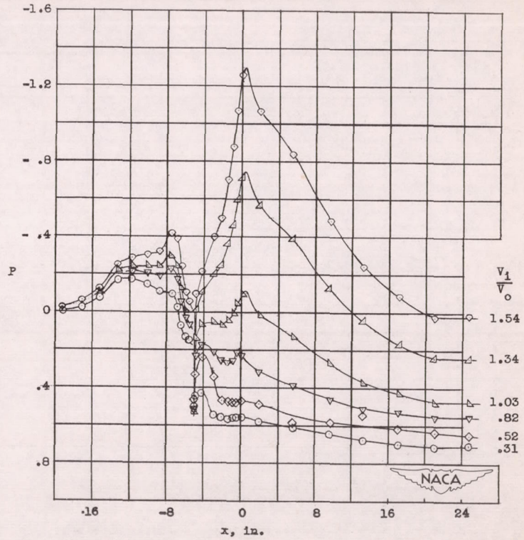
(b) Configuration III, C_{Q1} = 1.6 .
