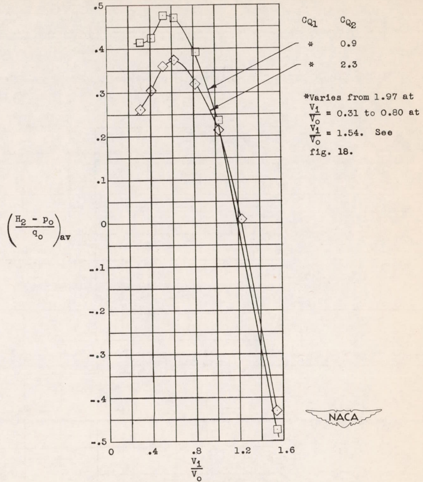
(f) Configuration VI - Second slot.
