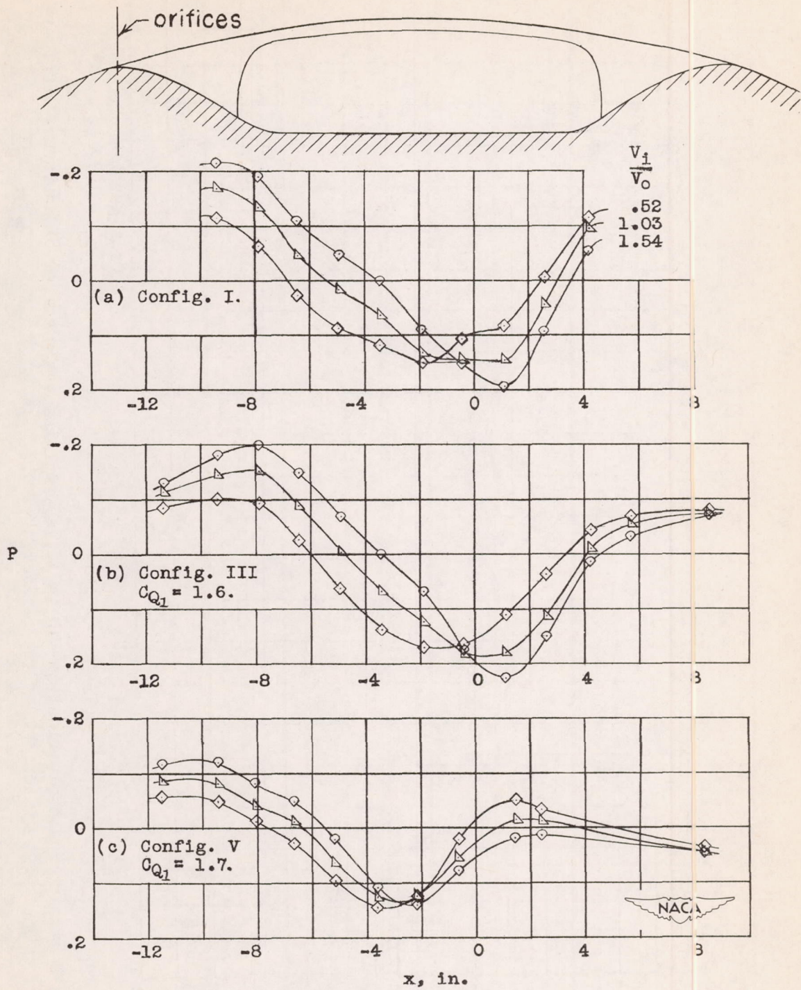
Figure 11.- Static-pressure distributions along edge of dimple. Boundary layer B.
