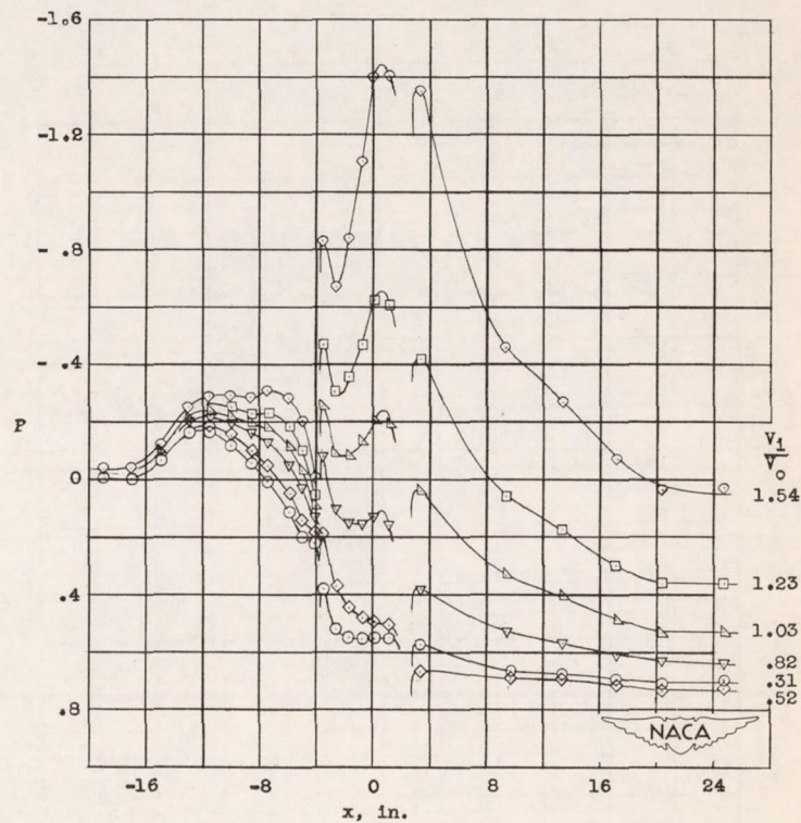
(a) Configuration V, C_{Q1} = 1.7, C_{Q2} = 0.9 .
