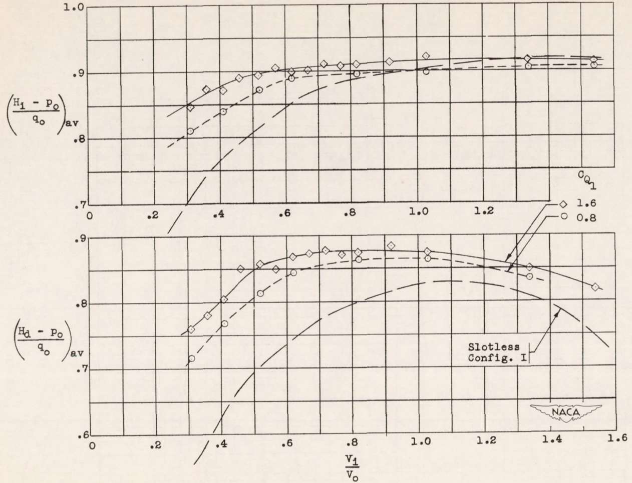
(a) Configuration III.
