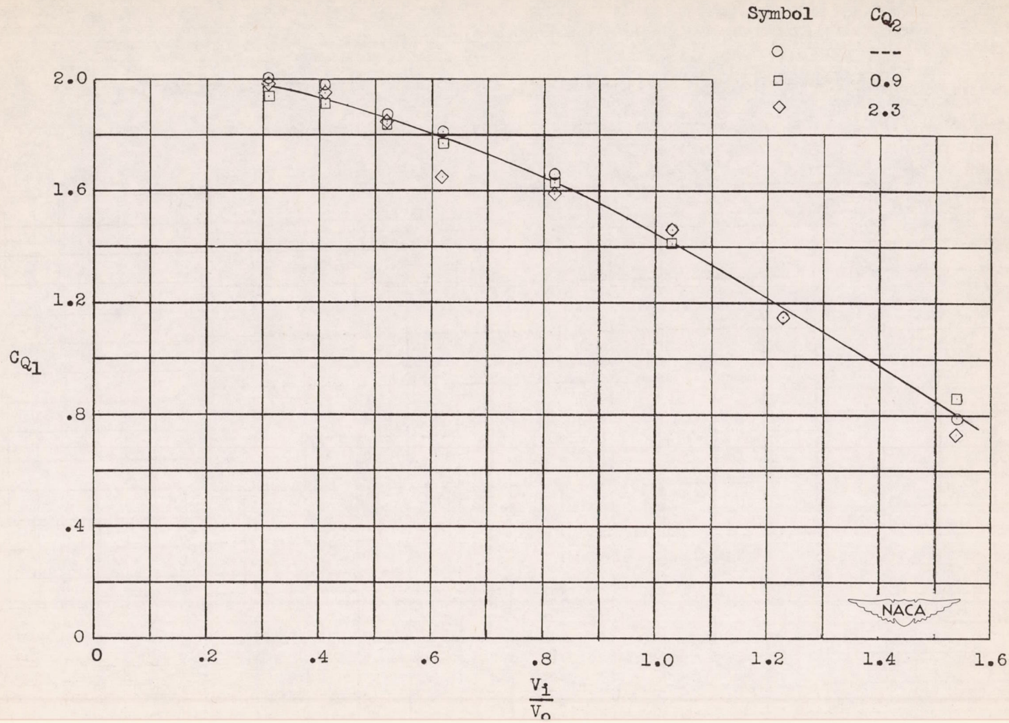
Figure 18.- Suction-flow quantity provided by bypass of configuration VI. Boundary layer B.
