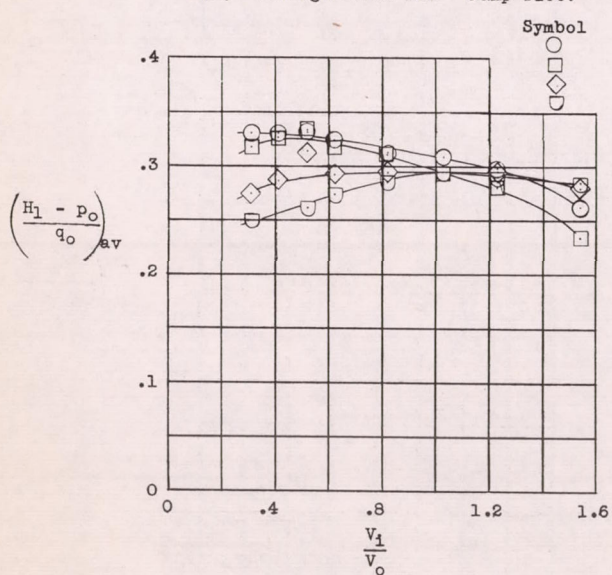
(b) Configuration V - Ramp slot.
