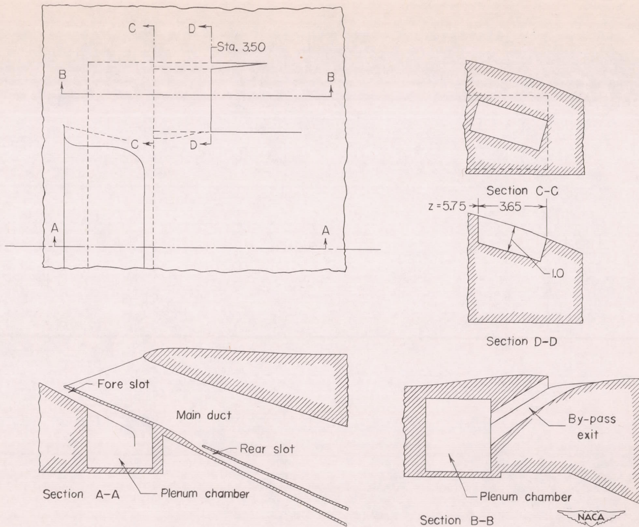
Figure 5.- Bypass ducting of configuration VI.
