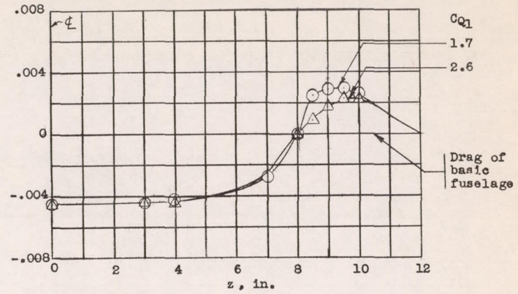
(b) Configuration V. Effect of suction quantity, \frac{V_1}{V_0} = 0.52 .
