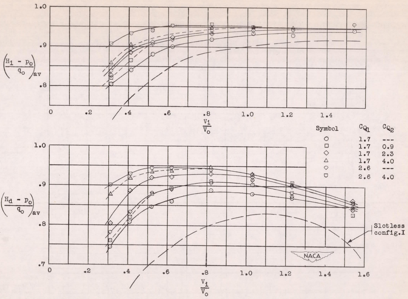
(b) Configuration V.
