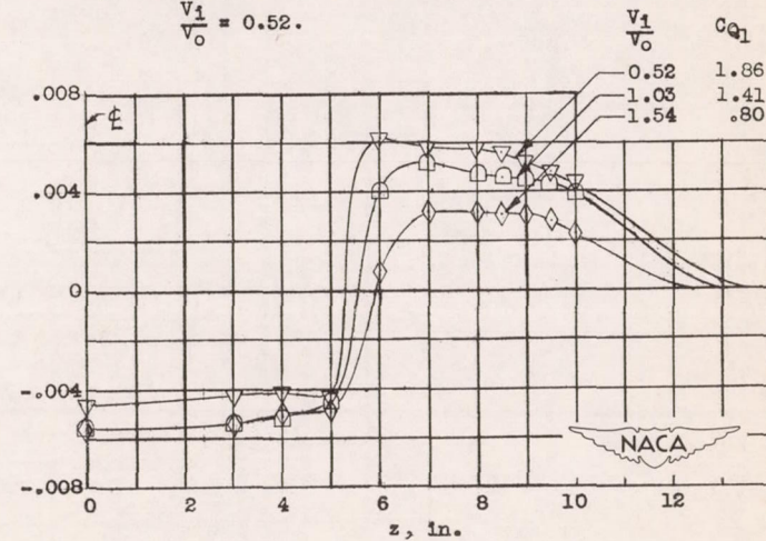
(d) Configuration VI. Effects of inlet-velocity ratio and suction quantity.
