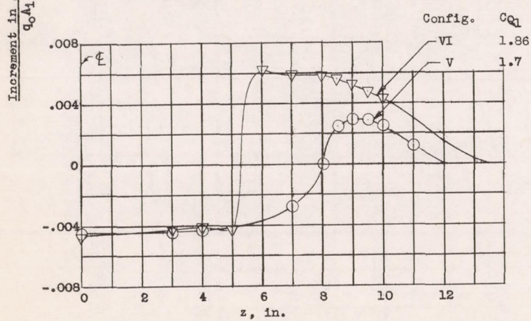
(c) Configurations V and VI. Effect of bypass installation, \frac{V_1}{V_0} = 0.52 .
