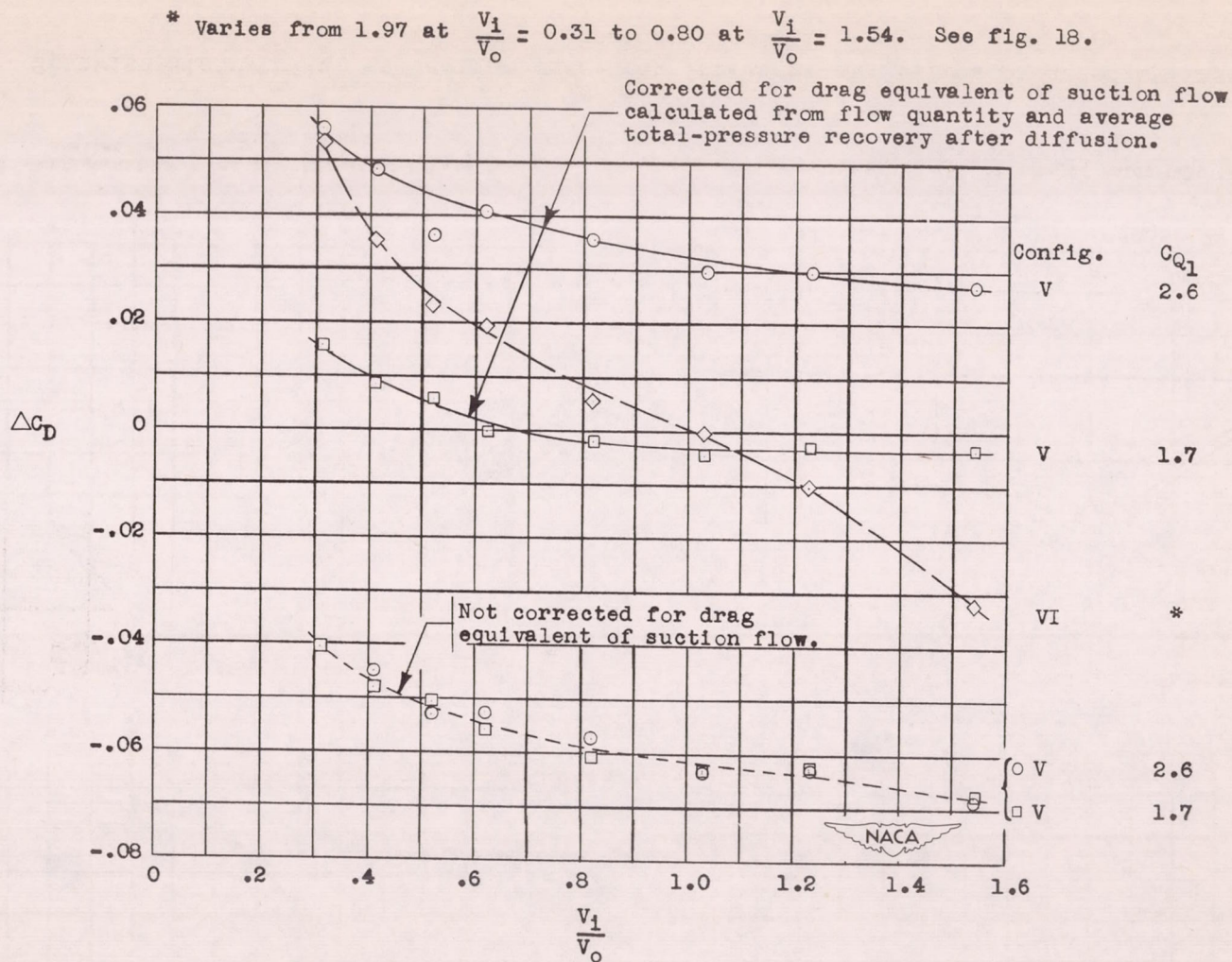
Figure 22.- Increase in external drag caused by installation of scoop. Boundary layer B.
