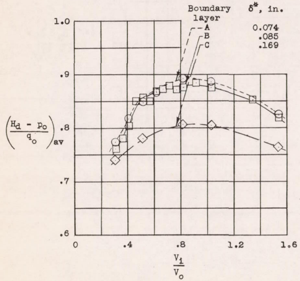
(a) Configuration III, C_{Q1} = 1.6 .
