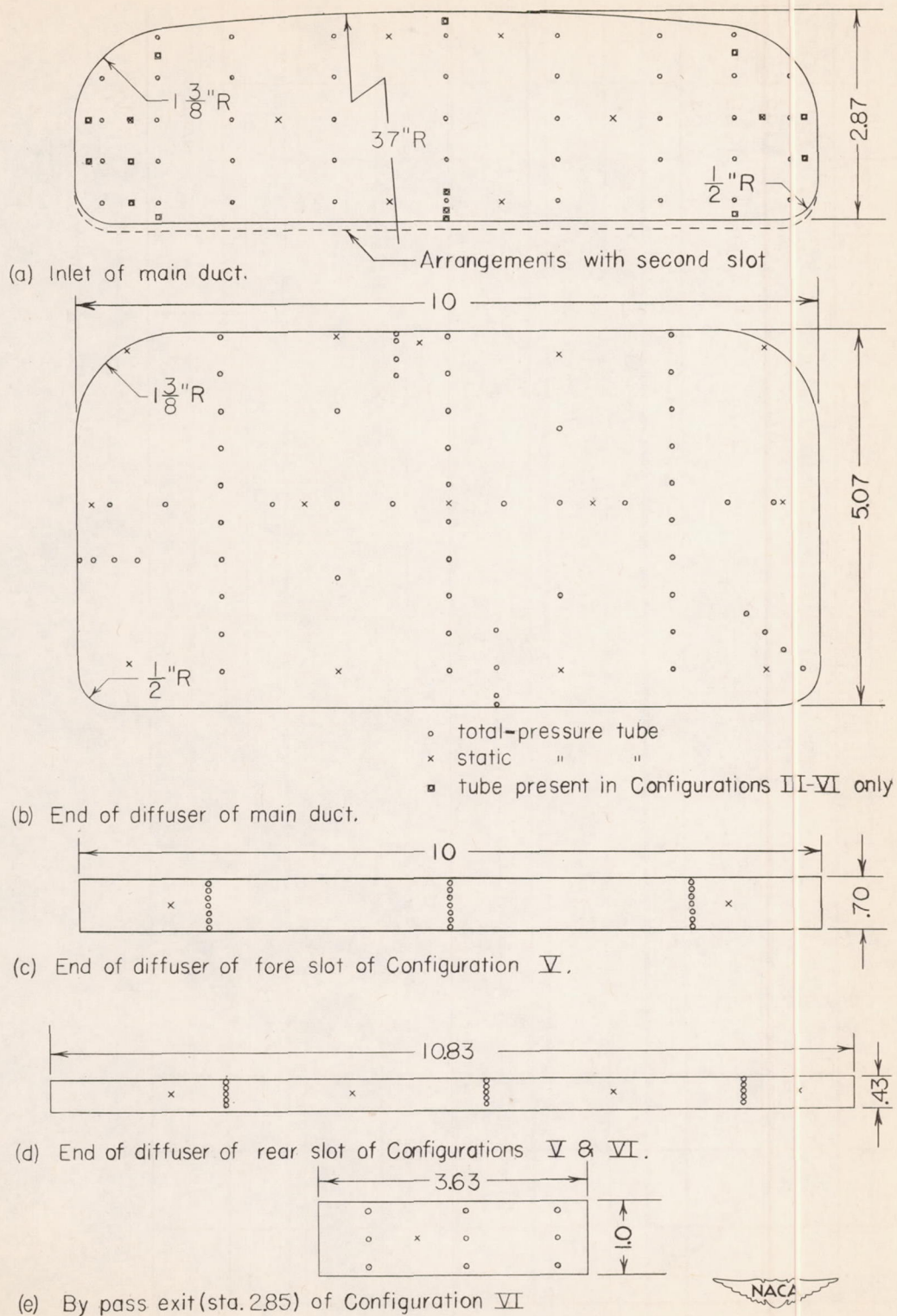
Figure 6.- Dimensions and instrumentation of measuring stations in ducting.
