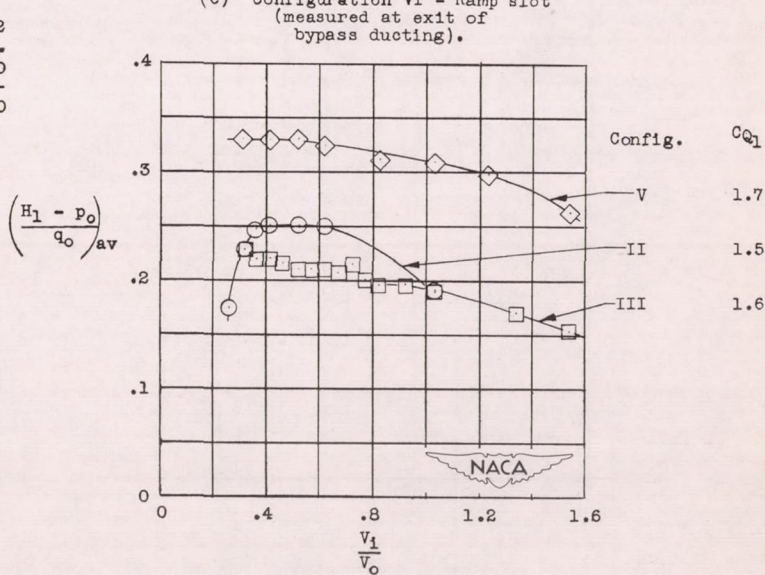
(d) Comparison of ramp slots of configurations II, III, and V.
