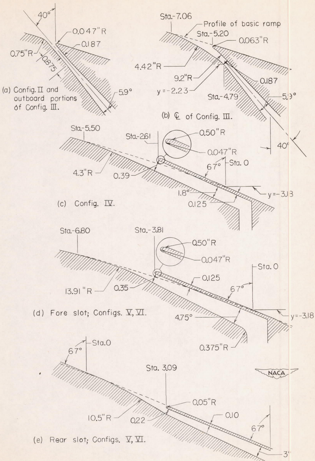
Figure 4.- Dimensions of boundary-layer slots.
