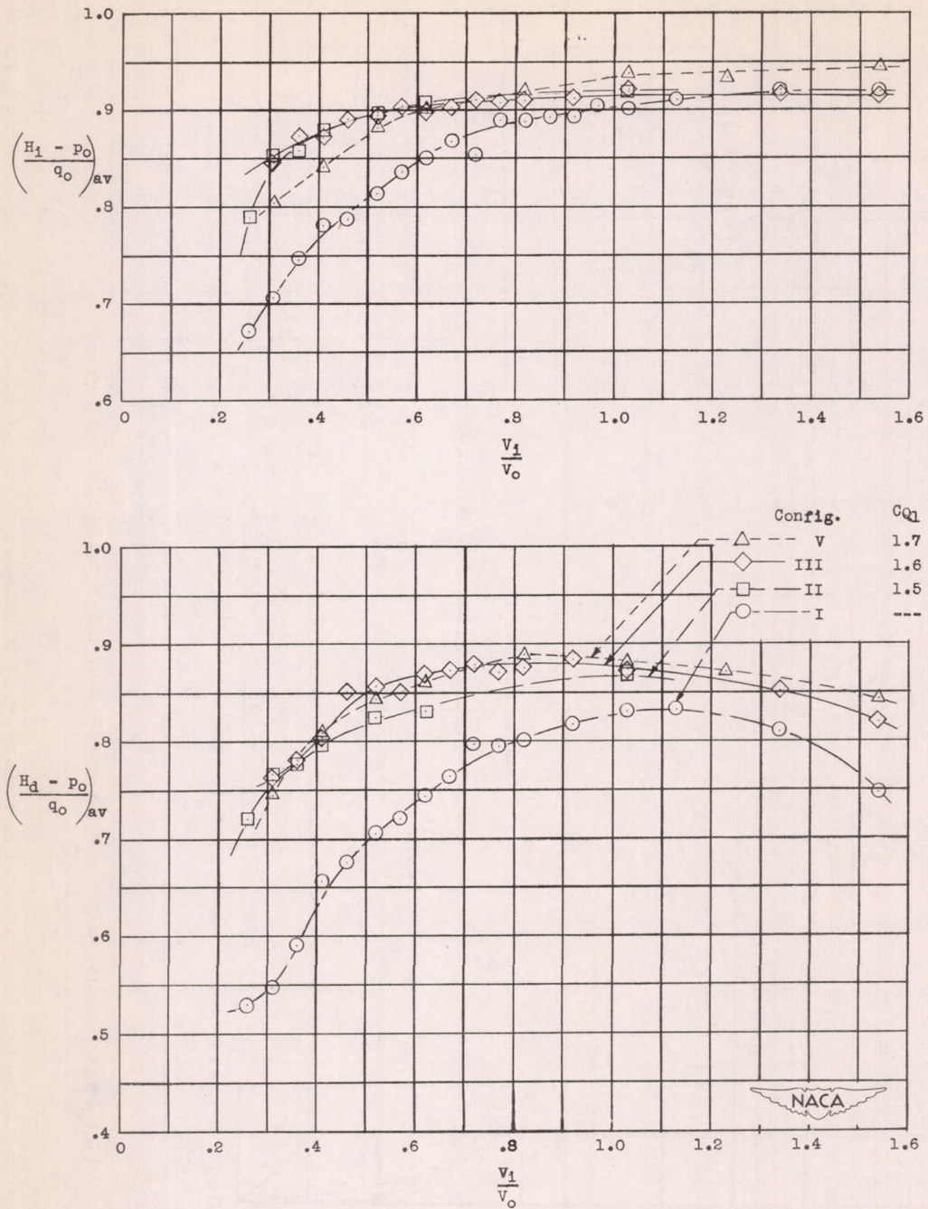
(a) Configurations I, II, III, and V. Effect of ramp slot configuration. Standard ramp without sidewalls, no second slot, boundary layer B.
