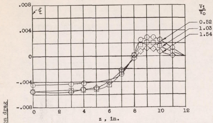
(a) Configuration V. Effect of inlet-velocity ratio, C_{Q1} = 1.7 .
