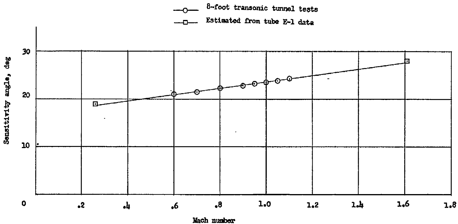
Figure 11.- Variation of sensitivity angle with Mach number of ogival tube E-2.
