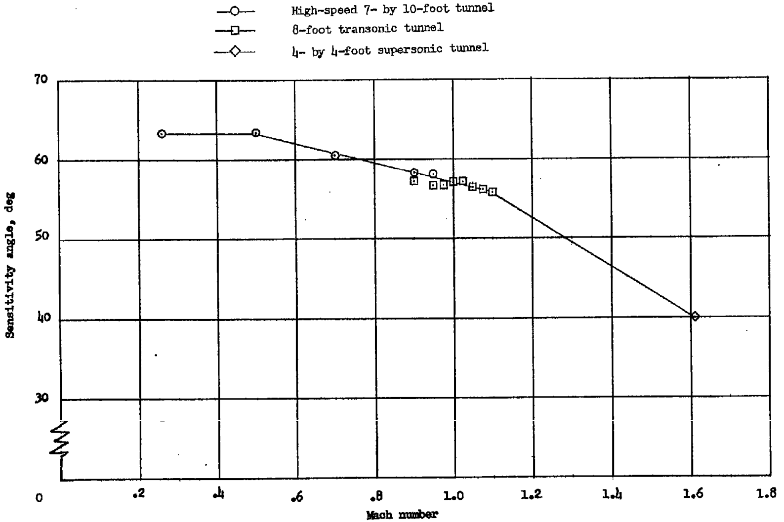
Figure 13.- Variation of sensitivity angle with Mach number of shielded tube A g -16.
