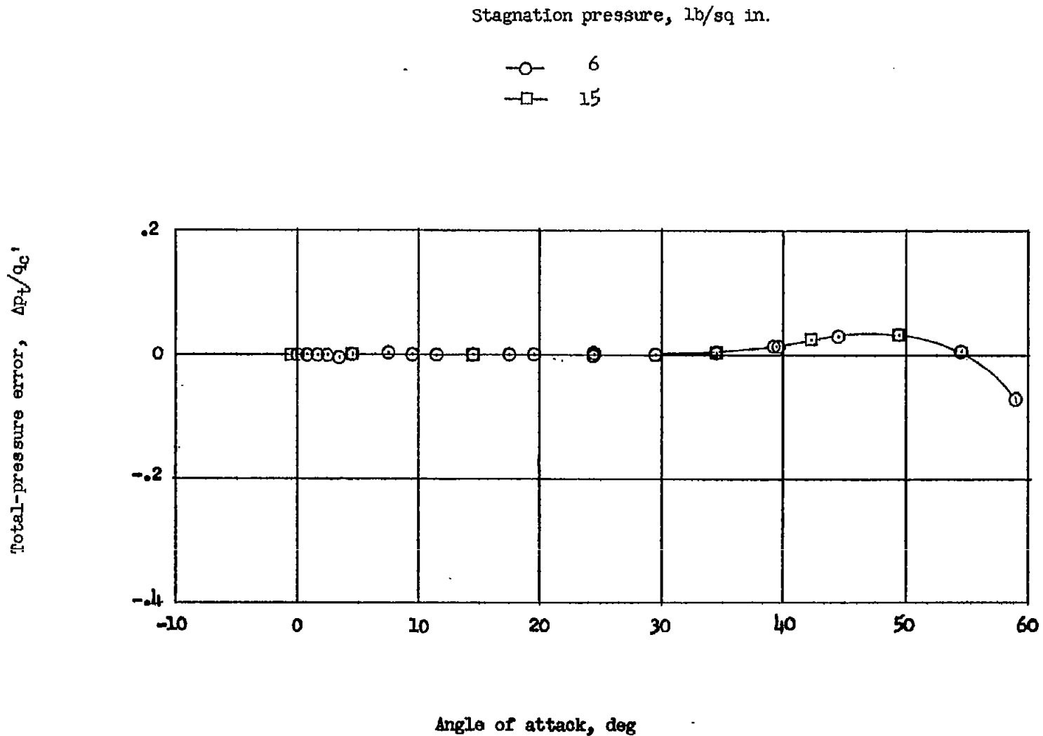
Figure 4.- Variation of total-pressure error with angle of attack of shielded tube A_3-12 at M = 1.61 .
