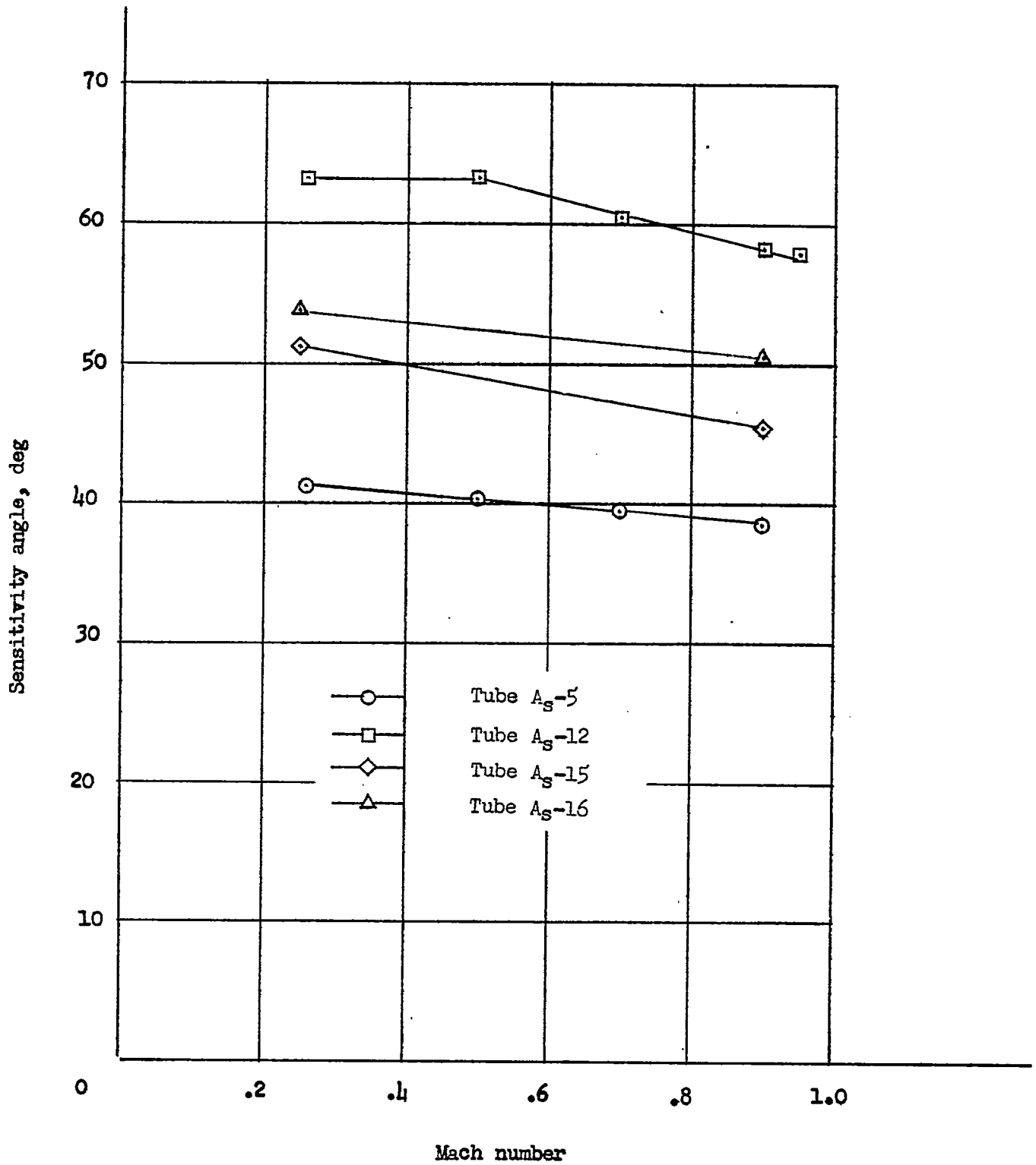
Figure 12.- Variation of sensitivity angle with Mach number of four tubes with shields having conical and curved entries.
