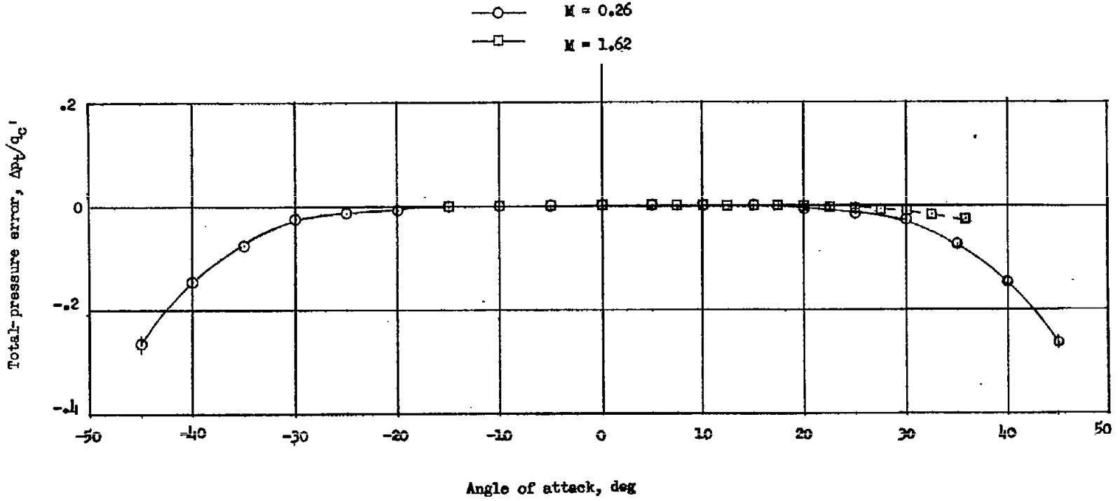
Figure 3.- Variation of total-pressure error with angle of attack of tube A-2 at subsonic and supersonic speeds.
