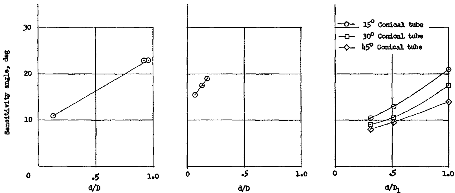
Figure 5.- Variation of sensitivity angle with size of impact opening of cylindrical and conical tubes. M = 0.26 .
