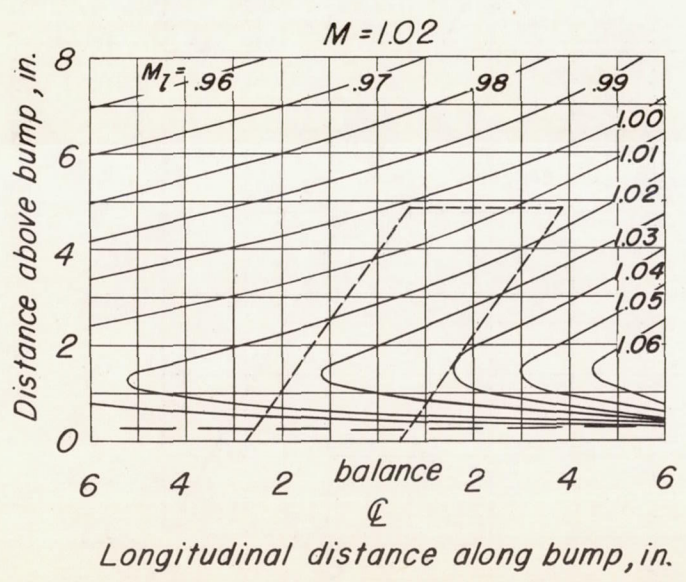
Figure 5.- Typical Mach number contour over transonic bump in region of model location.
