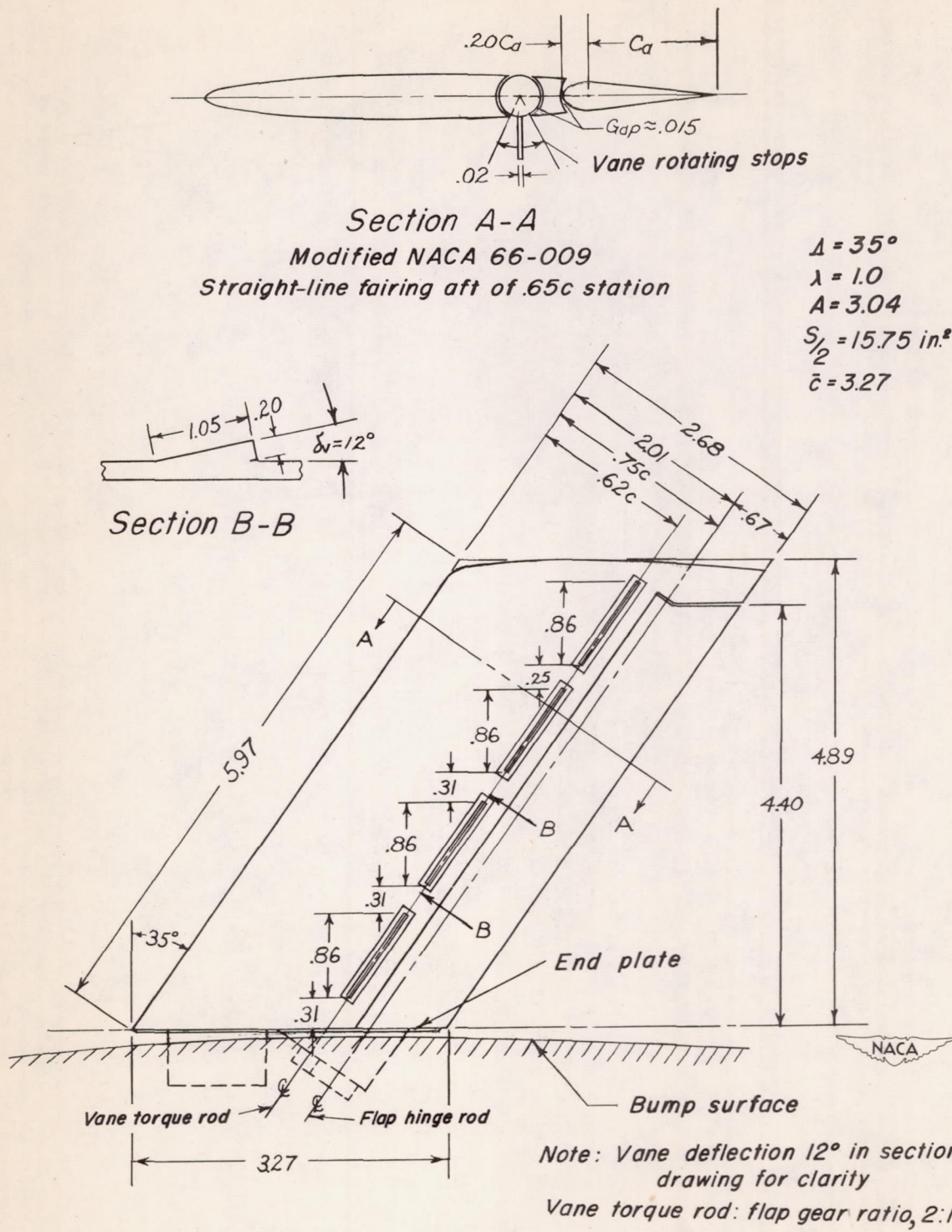
Figure 2.- Plan form and cross section of the left semispan model. (All dimensions are in inches.)
