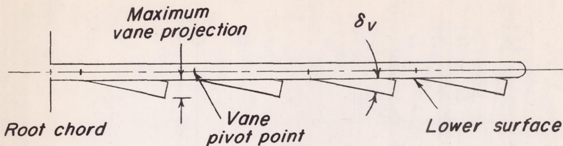
Section through wing parallel to leading edge and forward of vanes ( \delta_v = 12^\circ )
