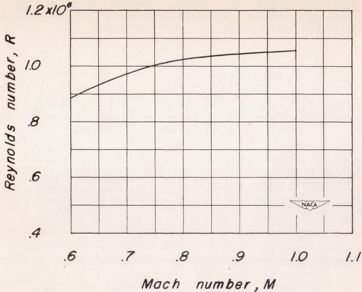
Figure 6.- Variation of average Reynolds number with Mach number.
