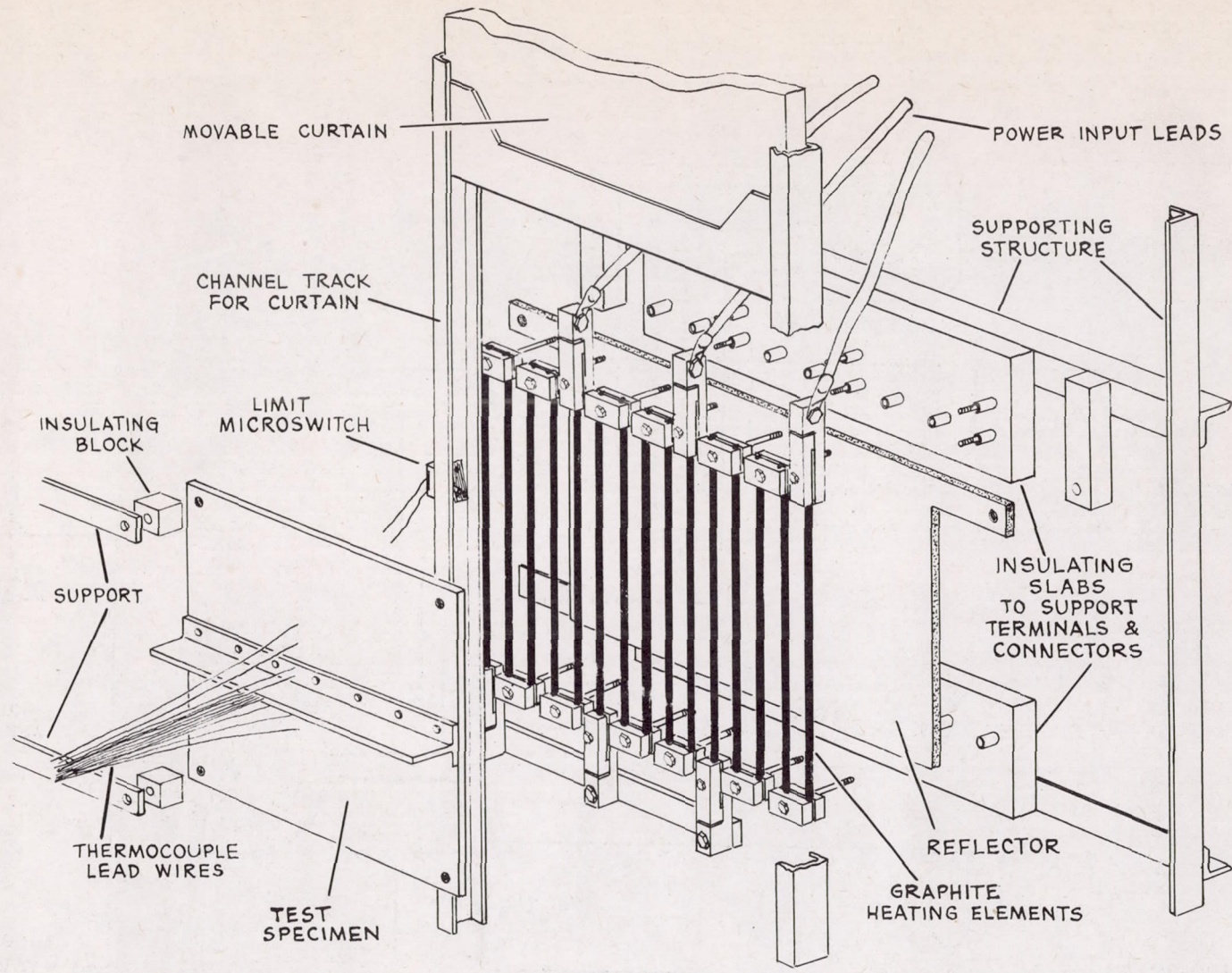
Figure 2.- Detailed exploded view of apparatus.
