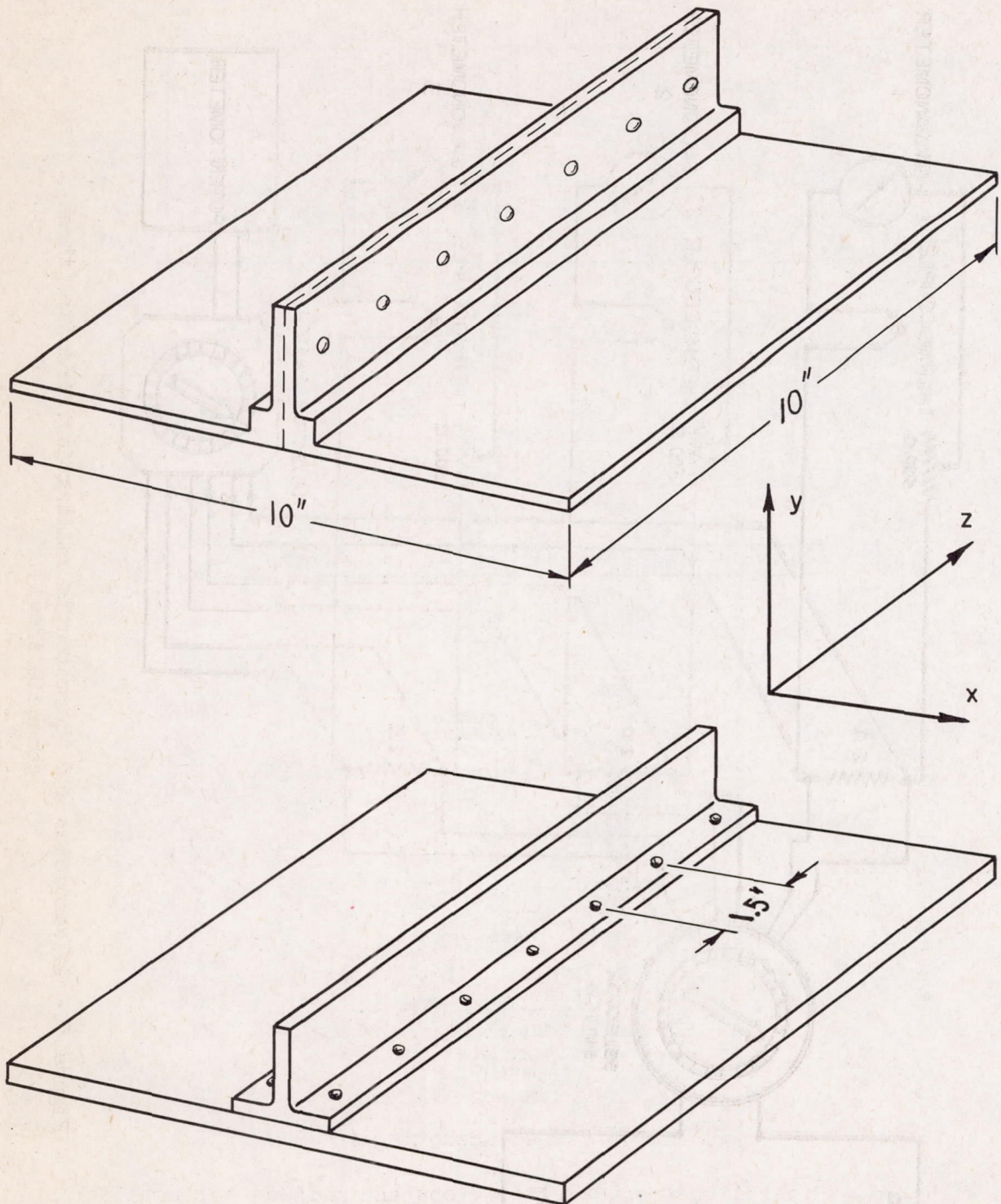
Figure 4.- Typical integral and riveted specimens.
