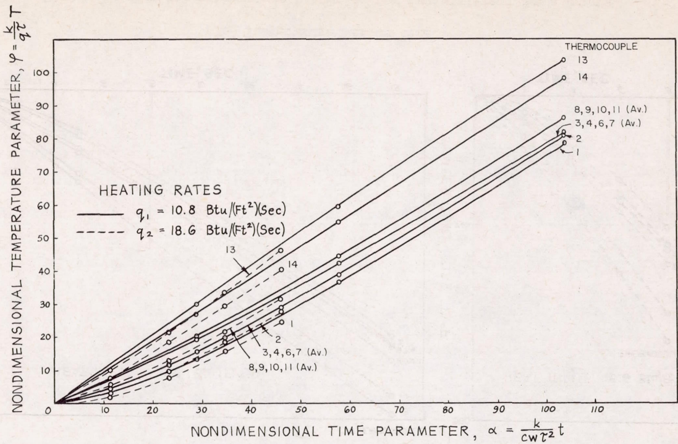
(b) Nondimensional temperature versus nondimensional time. k = 1.98 \times 10^{-3} \text{ Btu}/(\text{in.})(\text{sec})(^\circ\text{F}) ; c = 0.22 \text{ Btu}/(\text{lb})(^\circ\text{F}) ; w = 0.10 \text{ lb}/\text{cu in.} ; \tau = 0.125 \text{ in.}
