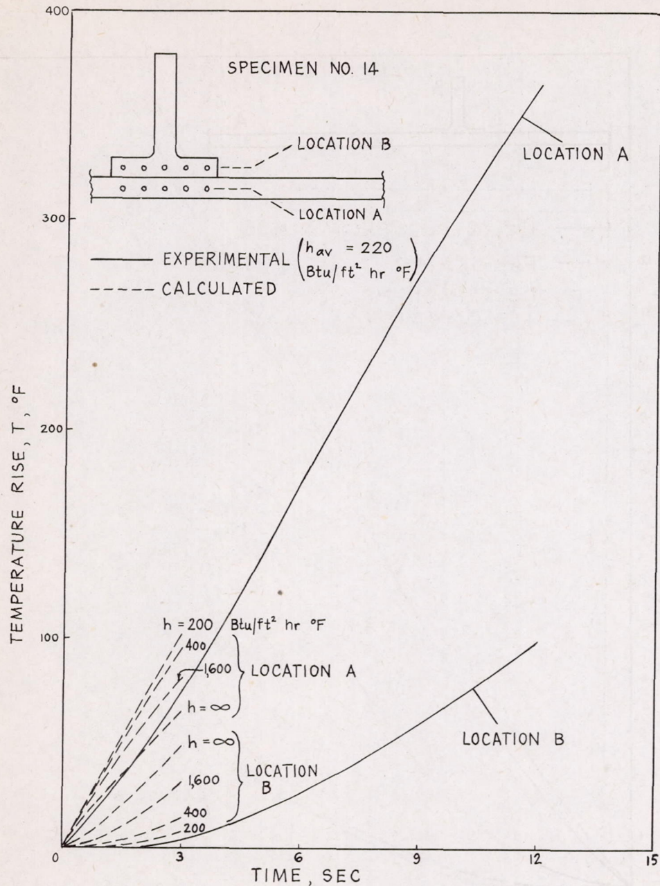
(a) Trial calculations showing effect of various interface conductance values.
