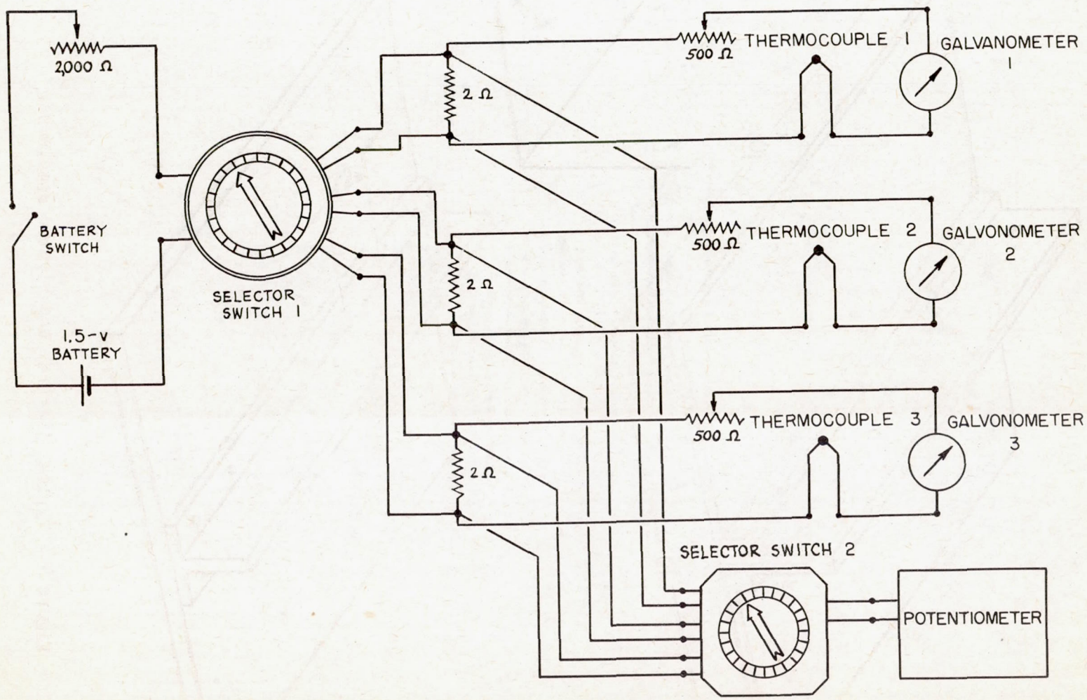
Figure 3.- Galvanometer and thermocouple calibrating circuits (three channels shown).
