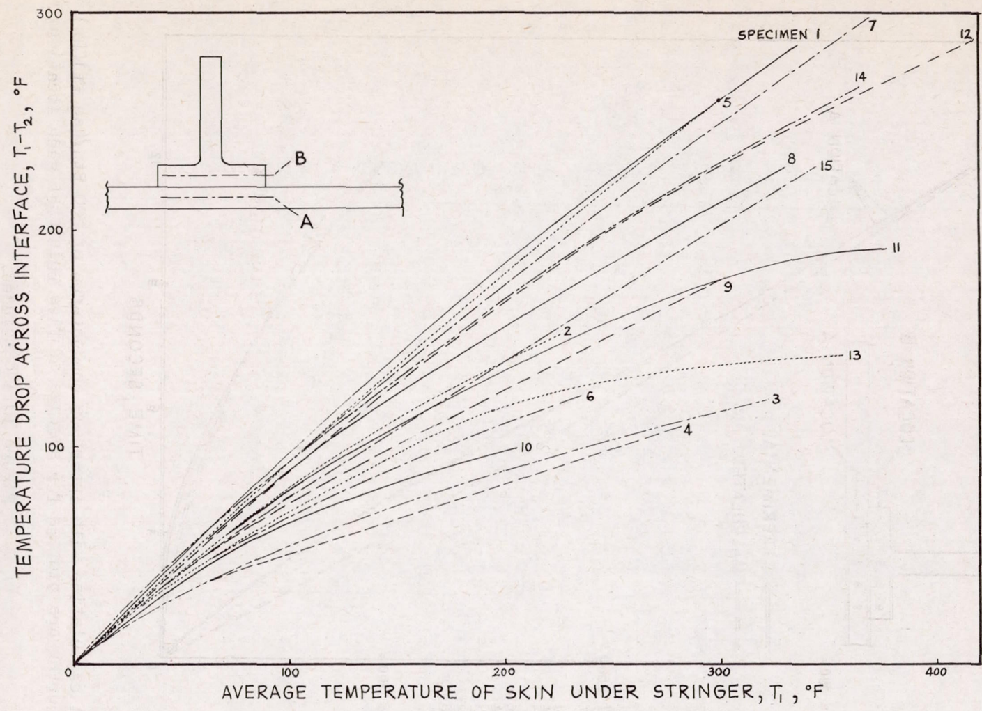
Figure 11.- Transient temperature drop across interface versus skin temperature under stringer for all geometries tested. T_1 , average temperature at station A; T_2 , average temperature at station B.
