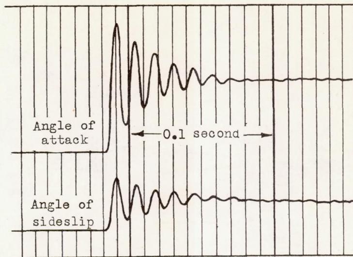
Figure 3.- Damping record obtained in Langley high-speed 7- by 10-foot tunnel. Mach number, 0.8; static pressure, 9.58 psi.
