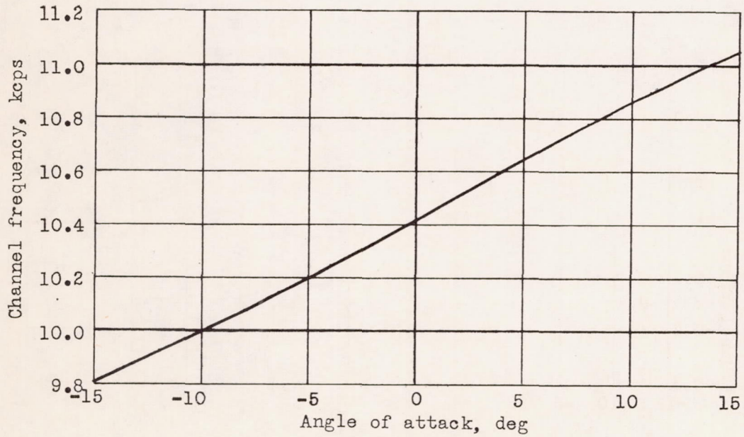
Figure 9.- Calibration on 10-kilocycle audio channel.
