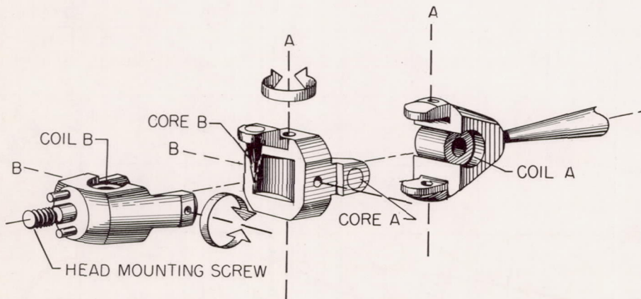
(b) Universal joint configuration, exploded view.
