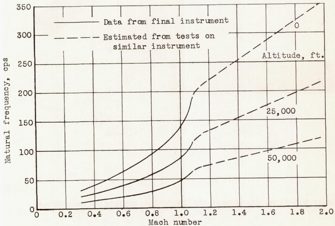
Figure 4.- Plot of natural frequency against Mach number at different altitudes.
