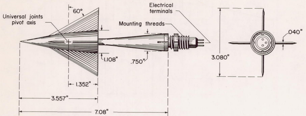
(a) External configuration.
