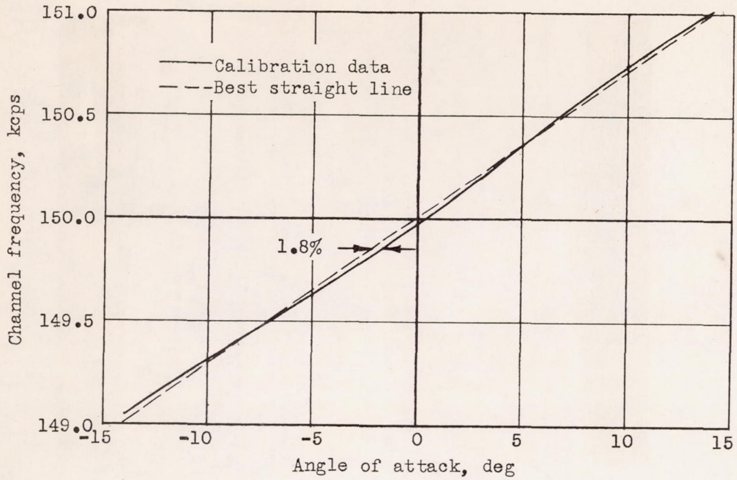
Figure 8.- Calibration on 150-kilocycle channel.
