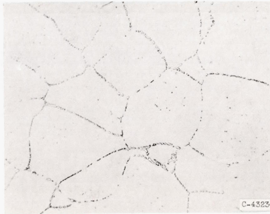
(c) 31.5-Percent-aluminum plus 2.0-percent-molybdenum, homogenized at 2300° F for 24 hours.
