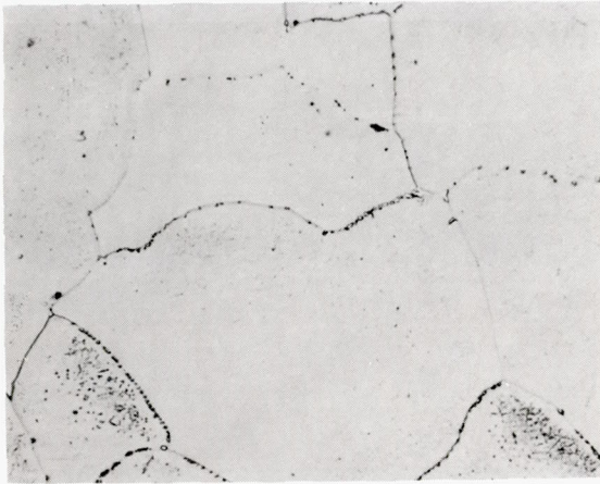
(a) 31.5-Percent-aluminum plus 0.5-percent-molybdenum, homogenized at 2300° F for 24 hours.
