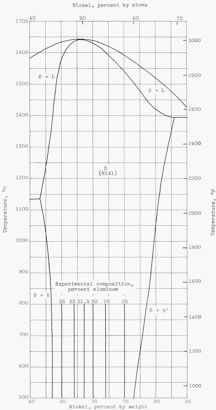
Figure 1. - Area of nickel-aluminum phase diagram under investigation (ref. 10).
