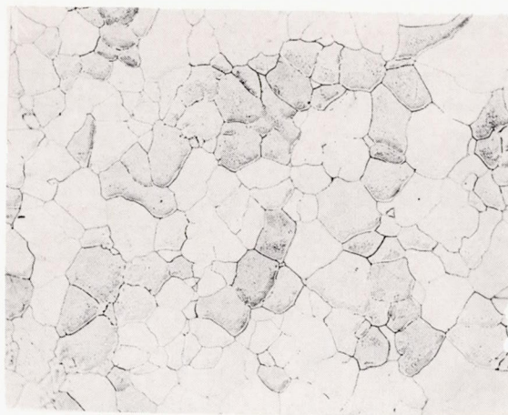
(c) 31.5-Percent-aluminum plus 1.0-percent-molybdenum NiAl, homogenized at 2300° F for 24 hours.
