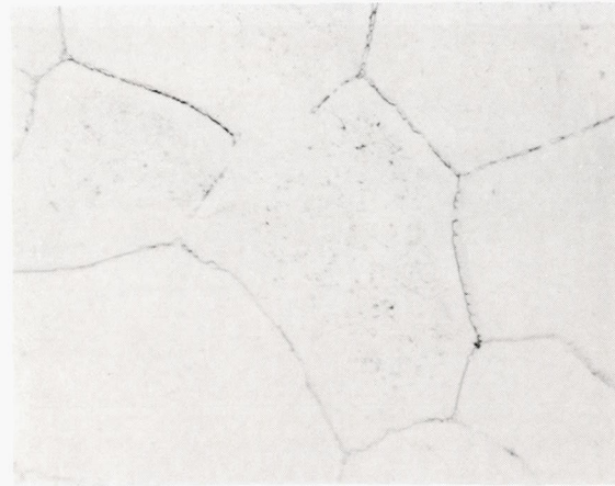
(b) 31.5-Percent-aluminum plus 1.0-percent-molybdenum, homogenized at 2300° F for 24 hours.
