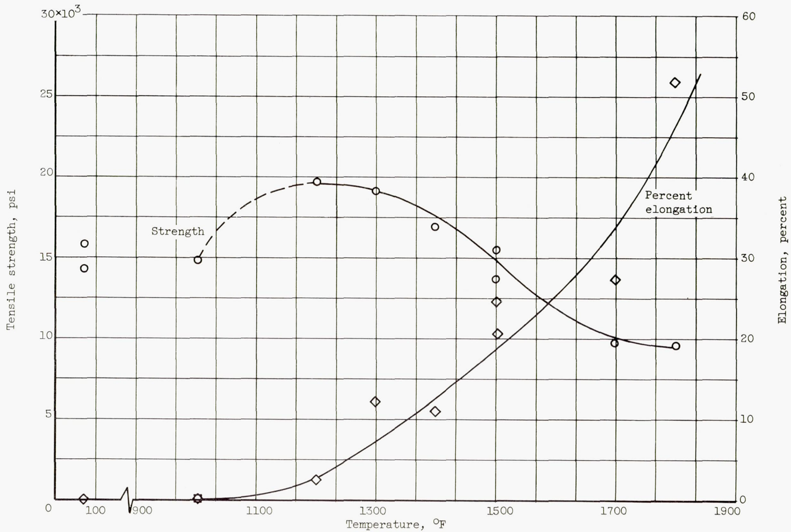
Figure 7. - Effect of temperature on tensile properties of stoichiometric (31.5-percent-aluminum) NiAl.
