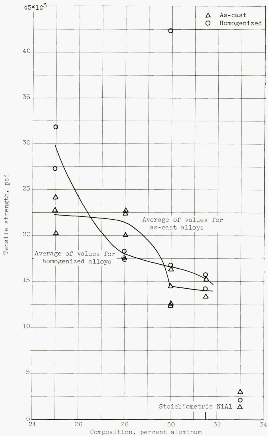
Figure 5. - Effect of composition on room-temperature strength of as-cast and homogenized alloys of NiAl phase.
