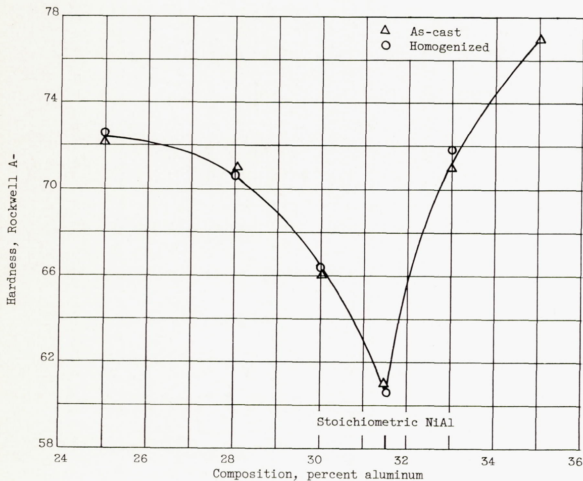
Figure 4. - Effect of composition on hardness of NiAl phase.
