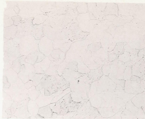
(b) 31.5-Percent-aluminum plus 0.5-percent-molybdenum NiAl, homogenized at 2300° F for 24 hours.
