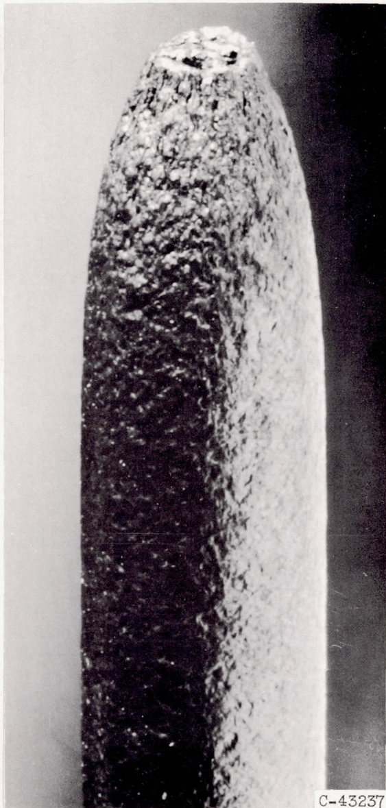
(b) 1700° F tensile test. 31.5- Percent-aluminum and 1-percent- molybdenum alloy.
