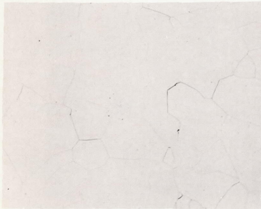
(c) 30-Percent-aluminum NiAl, homogenized at 2400° F for 6 hours.
