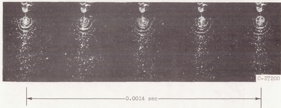
Figure 4. - Successive frames from high-speed motion pictures of formation of spray from two impinging jets of water.
