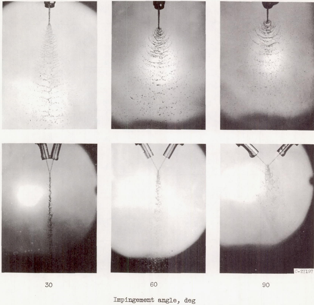
Figure 14. - Effect of impingement angle on spray pattern. Jet diameter, 0.025 inch; jet velocity, 60 feet per second; fluid, water.
