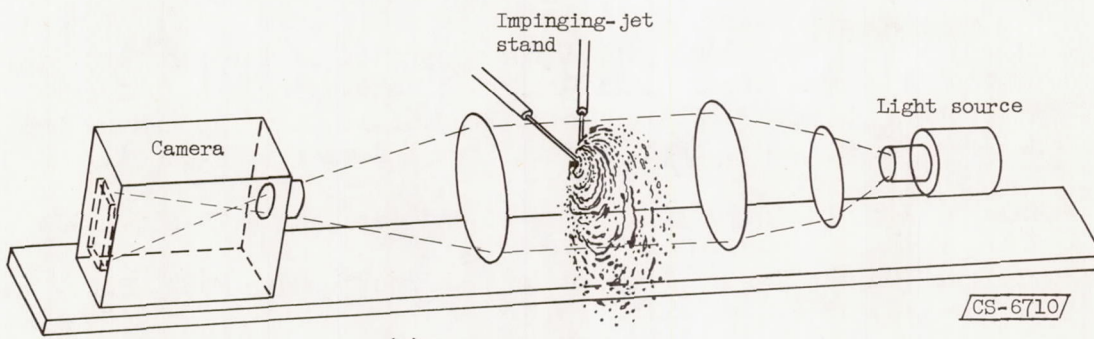
(b) Photographic apparatus.
