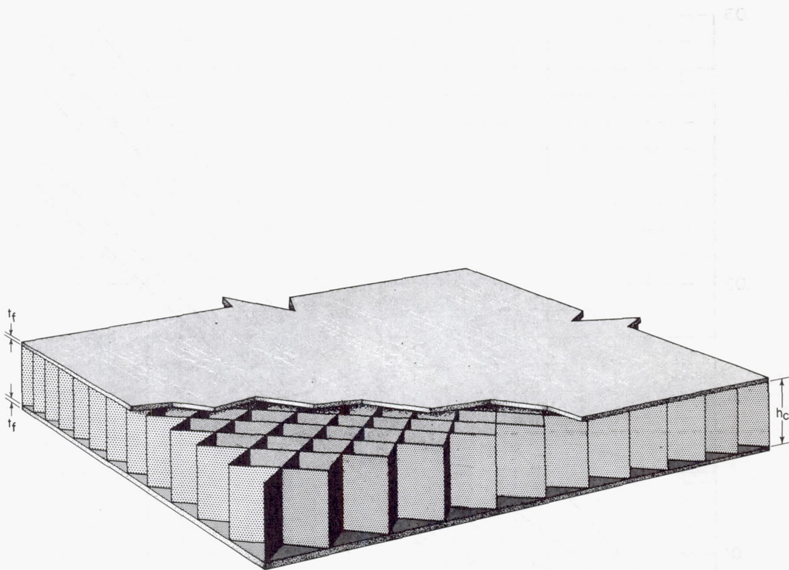
Figure 1.- Section of typical cellular-core sandwich plate.
