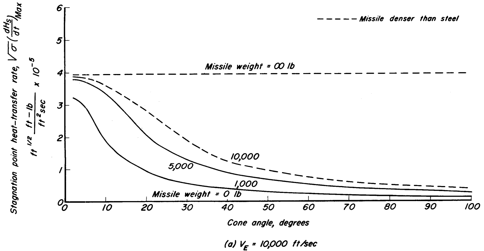
Figure 11. - Maximum rate of convective heat transfer to the stagnation point of spherically tipped cones of the same volume entering the earth's atmosphere at an angle of 30^\circ to the horizontal and velocities of 10,000, 20,000, and 30,000 ft/sec (volume = 16.34 cu ft).
