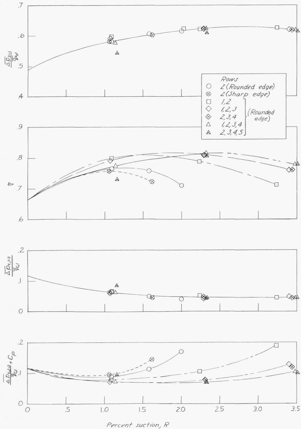
Figure 12.- Variation of static-pressure-rise coefficient, diffuser effectiveness, and loss coefficient at station 3 with percent suction. \theta_1 = 0^\circ .
