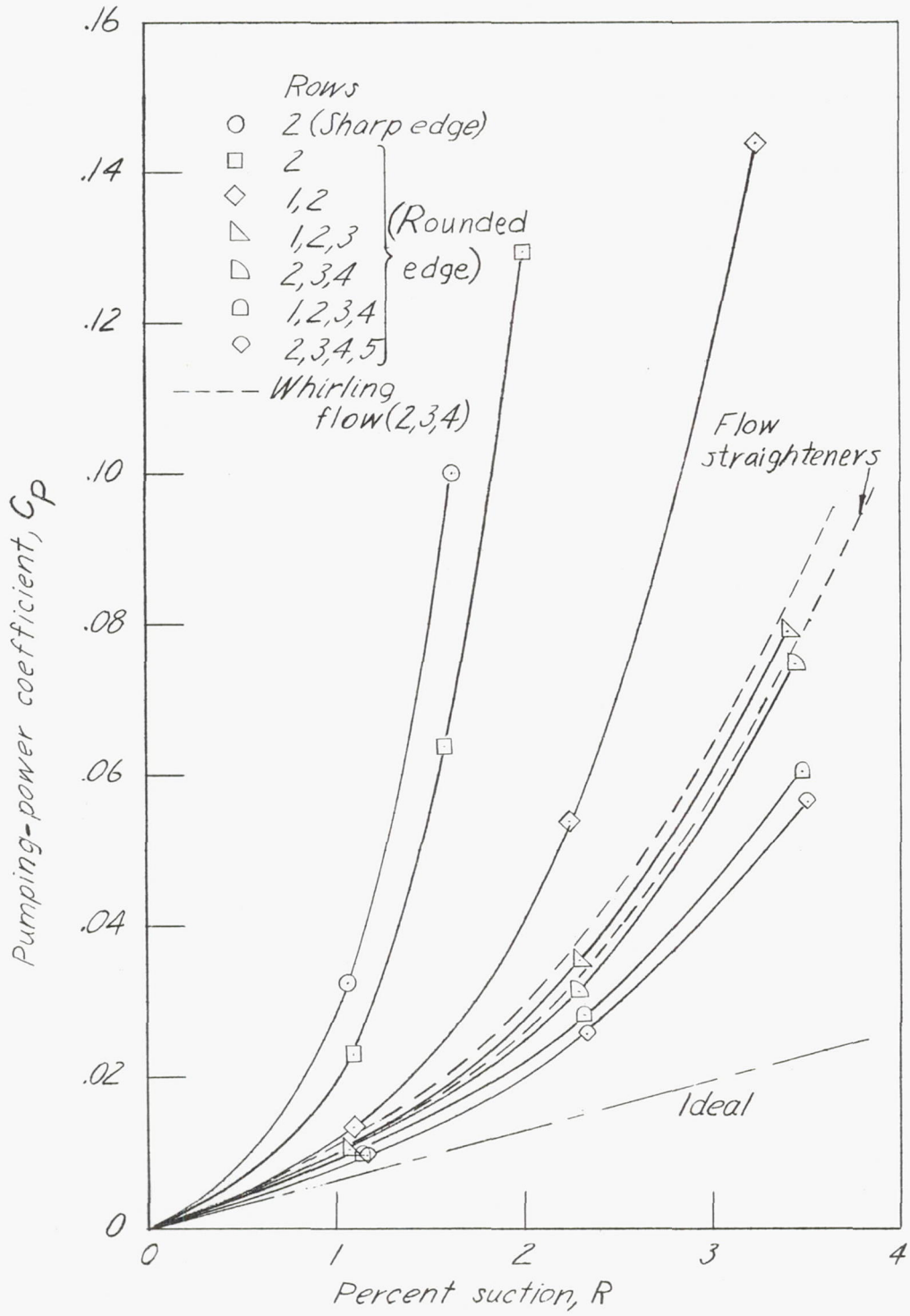
Figure 11.- Variation of pumping-power coefficient with percent suction.
