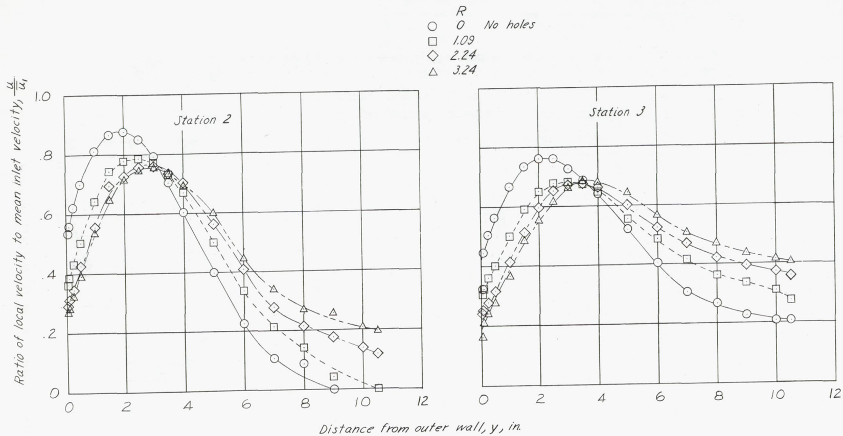
Figure 6.- Velocity distributions at stations 2 and 3 with suction through rows 1 and 2. \bar{\theta}_1 = 0^\circ .
