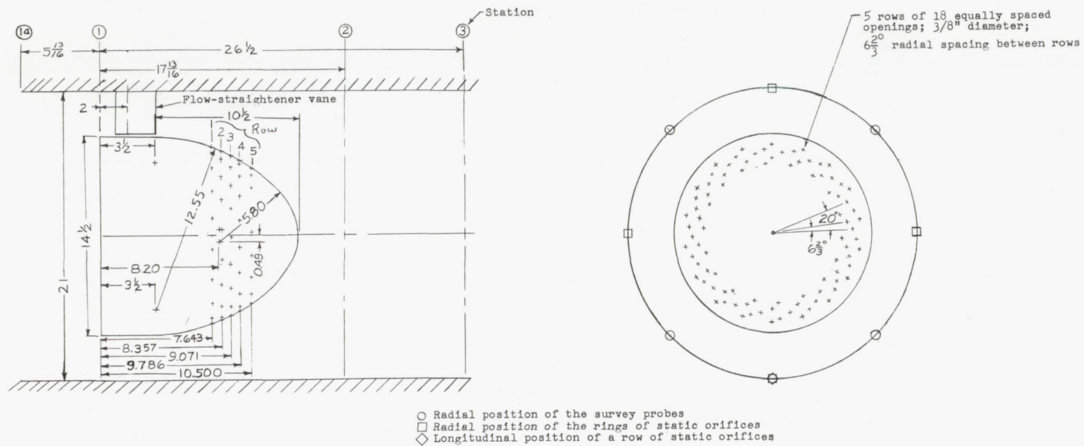
(b) Line drawing of diffuser. All dimensions are in inches unless otherwise indicated.
