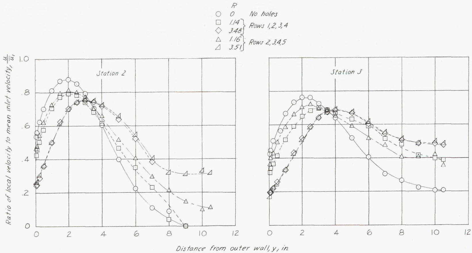
Figure 8.- Velocity distributions at stations 2 and 3 with suction through rows 1, 2, 3, and 4 and 2, 3, 4, and 5. \theta_1 = 0^\circ .
