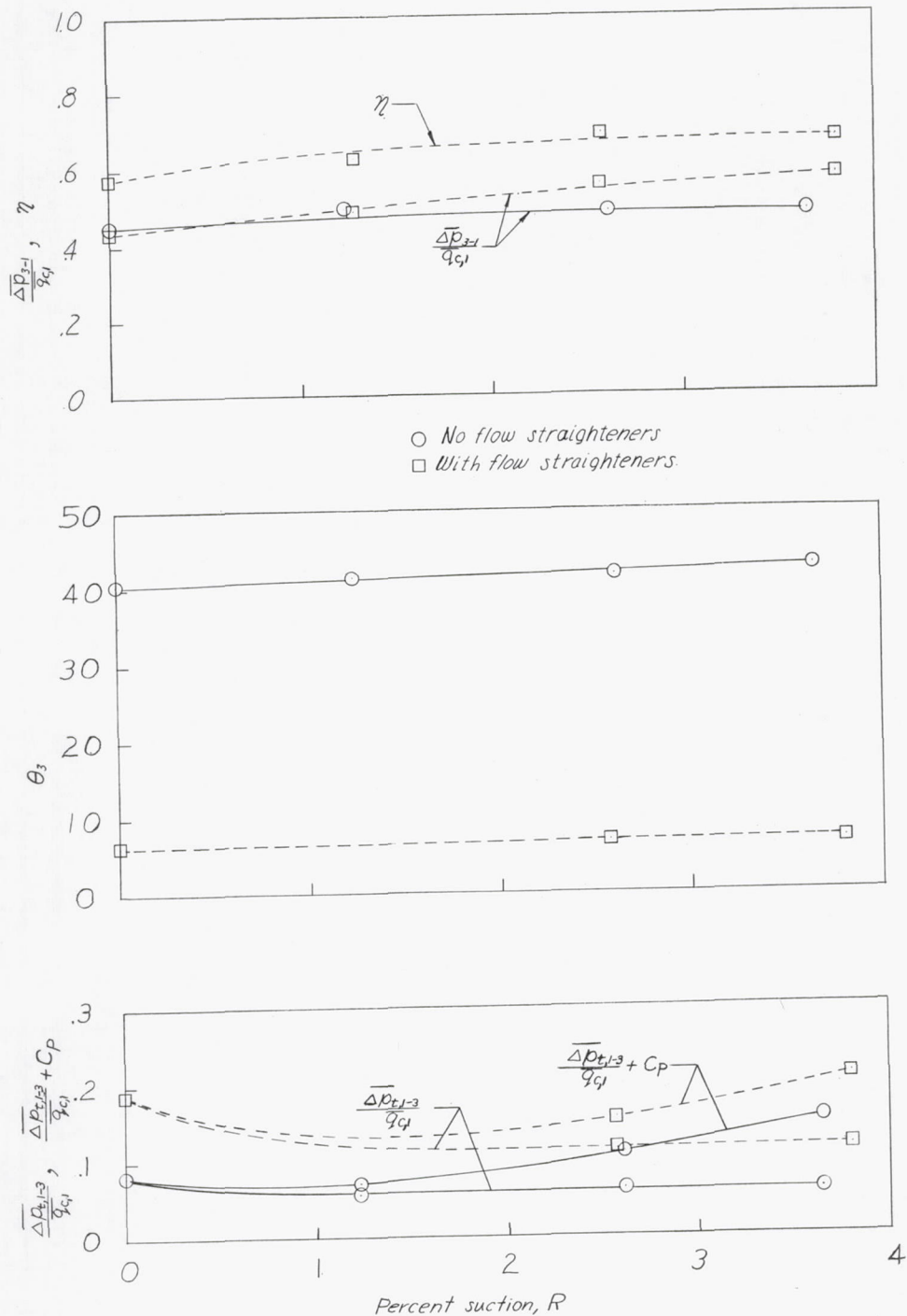
Figure 16.- Variation of static-pressure-rise coefficient, diffuser effectiveness, mean flow angle, and loss coefficient at station 3 with percent suction. \theta_1 = 19.5^\circ .
