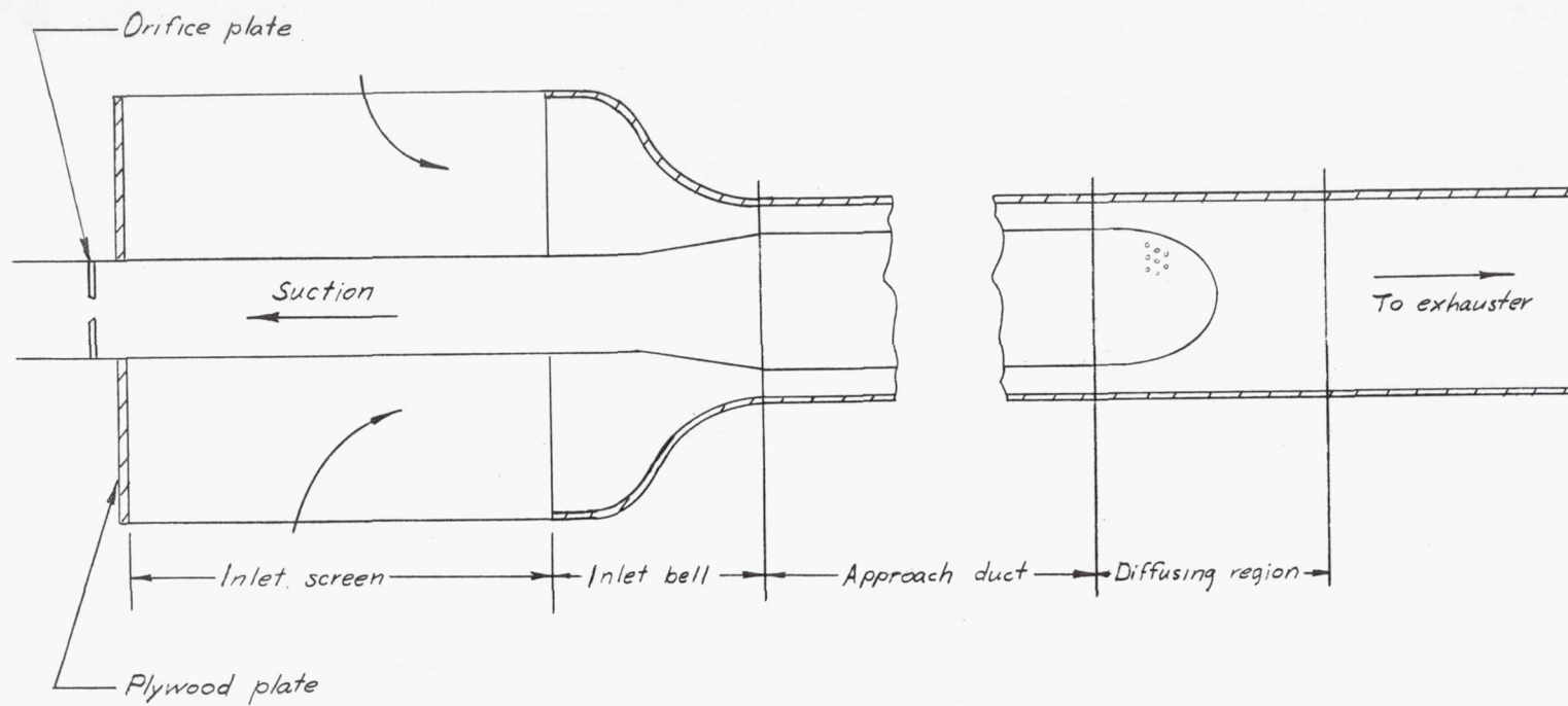
(a) General duct arrangement.
