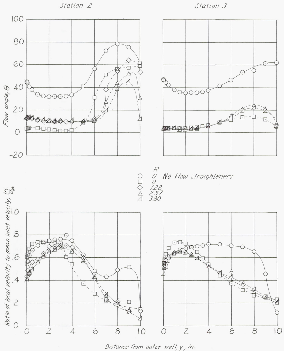
Figure 15.- Velocity and flow-angle distributions at stations 2 and 3 with \theta_1 = 19.5^\circ and suction through rows 2, 3, and 4. With flow straighteners.
