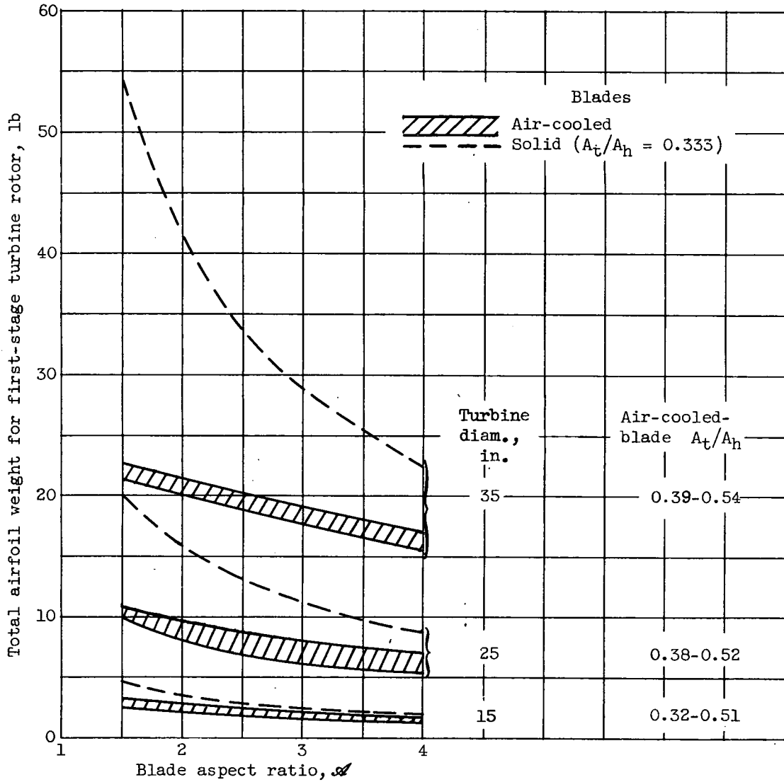
(a) First stage. Hub-tip radius ratio, 0.73.
