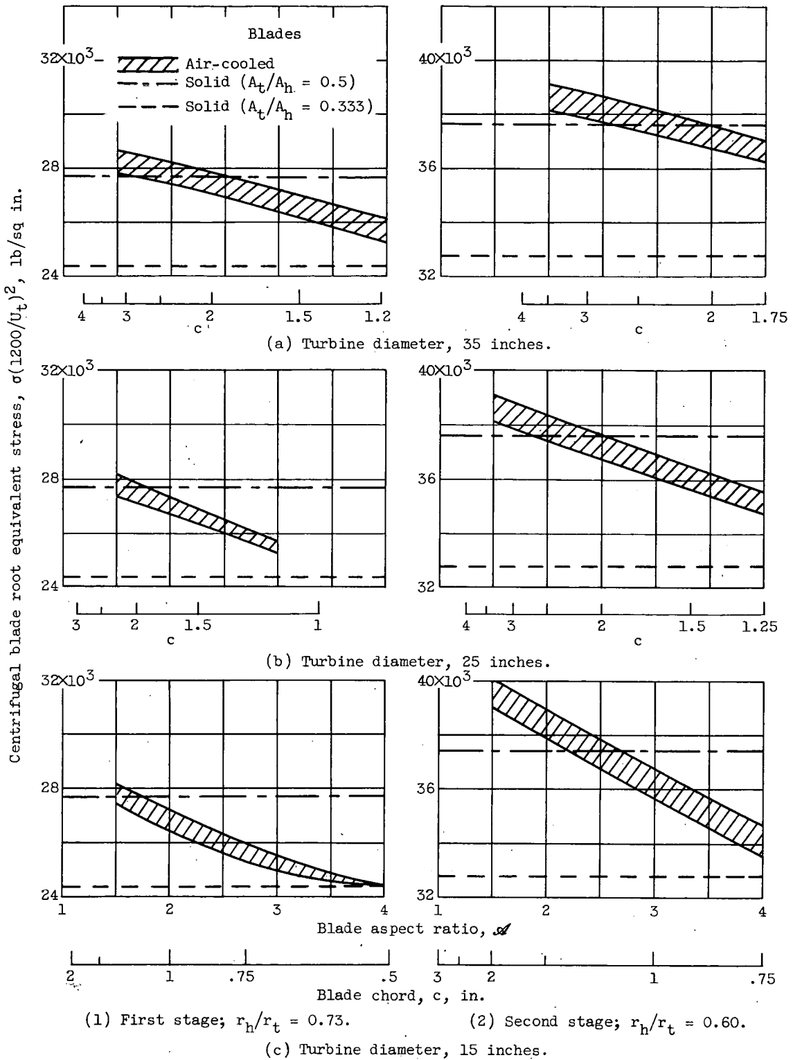
Figure 4. - Air-cooled-turbine blade root stresses.
