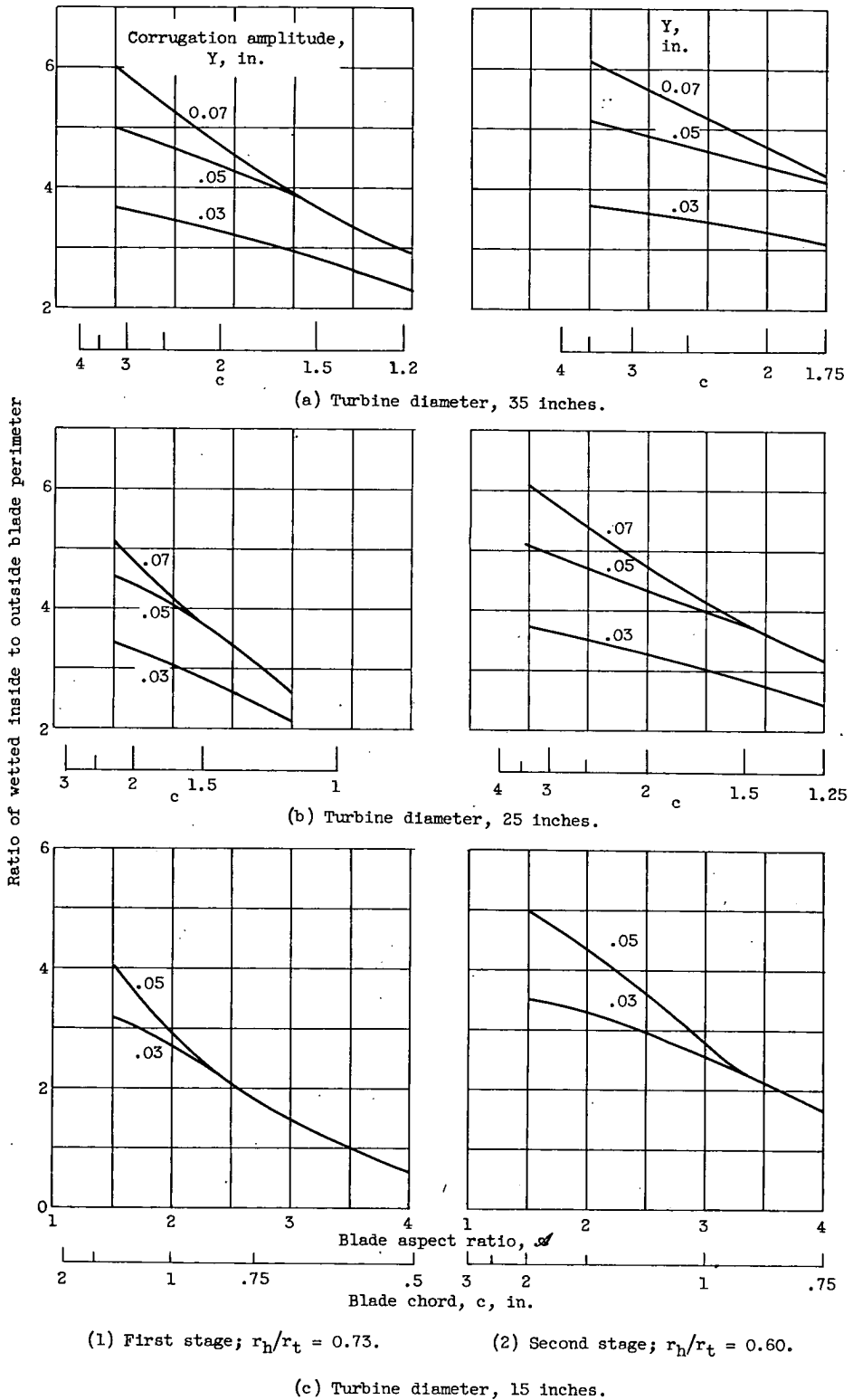
Figure 5. - Effect of turbine blade size on inside heat-transfer surface area.
