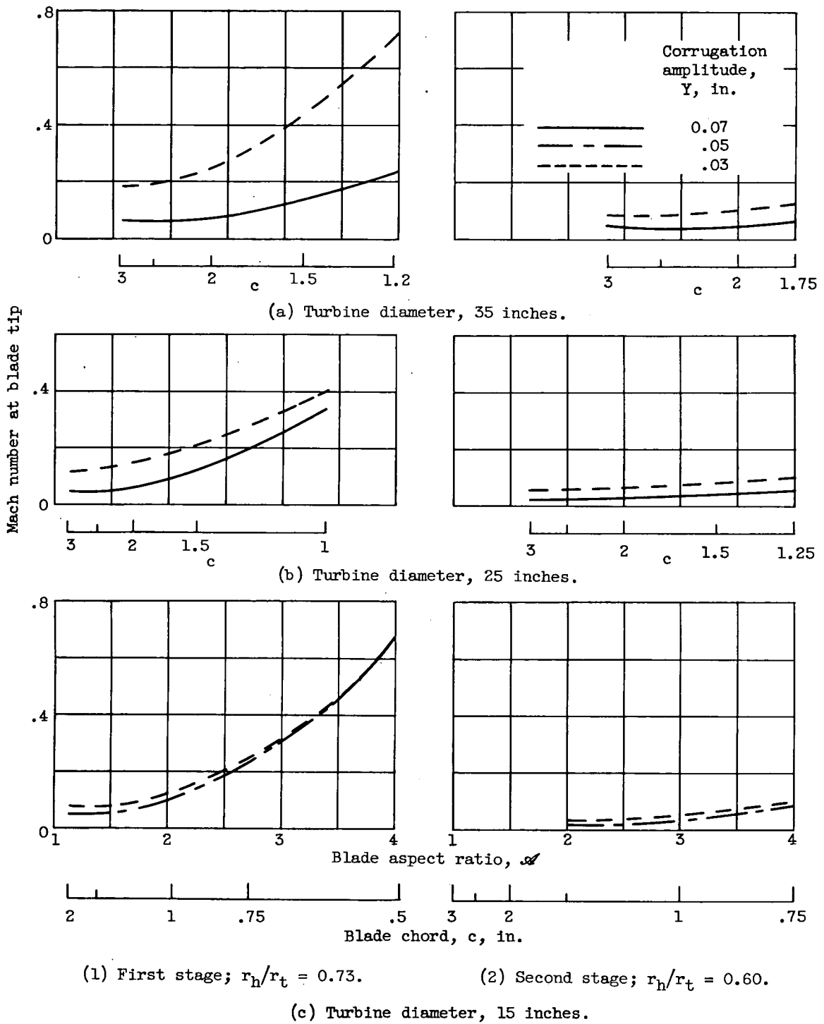
Figure 10. - Effect of turbine blade size on cooling-air Mach number at blade tip.
