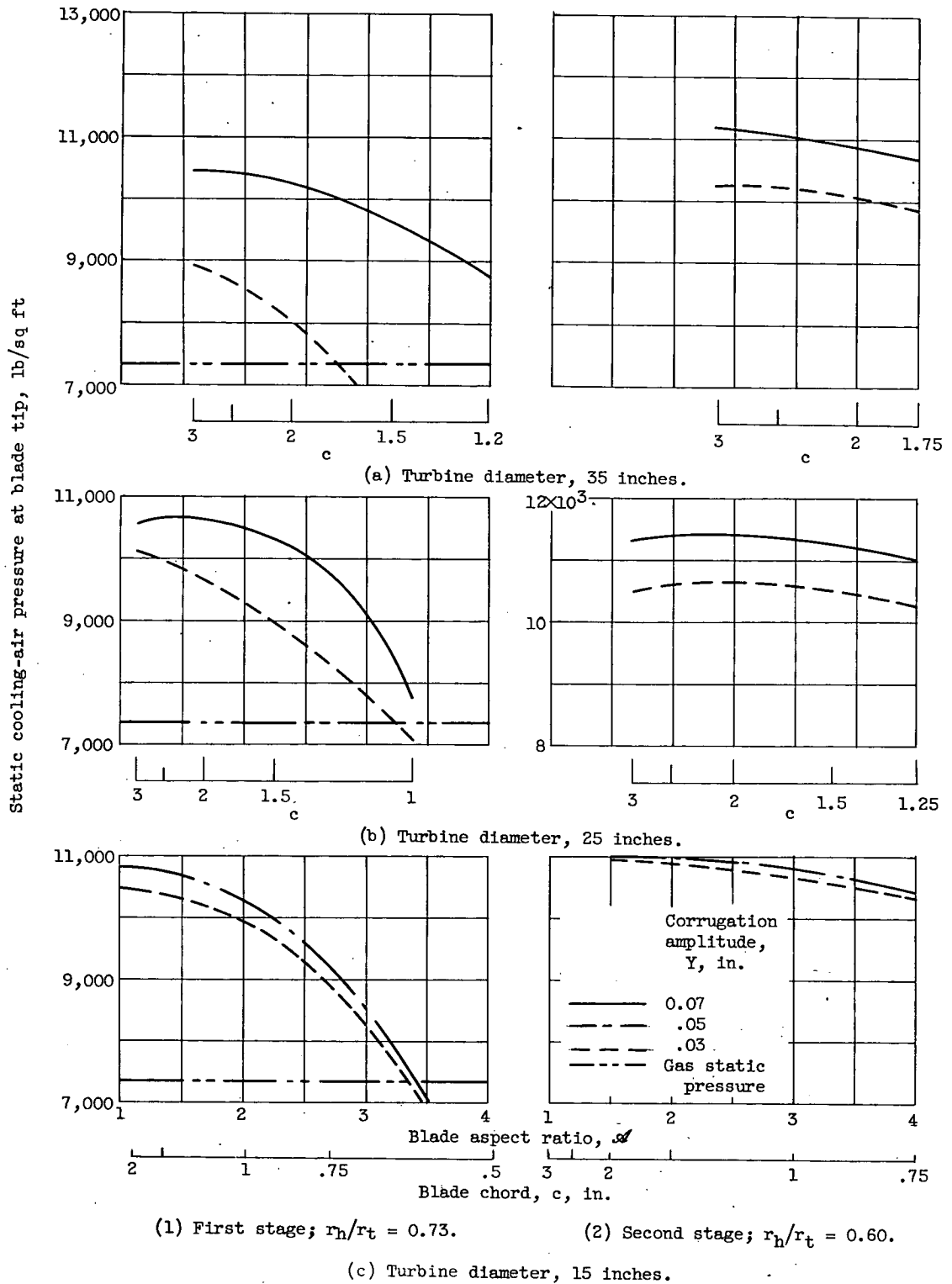
Figure 9. - Effect of turbine blade size on static cooling-air pressure at blade tip.
