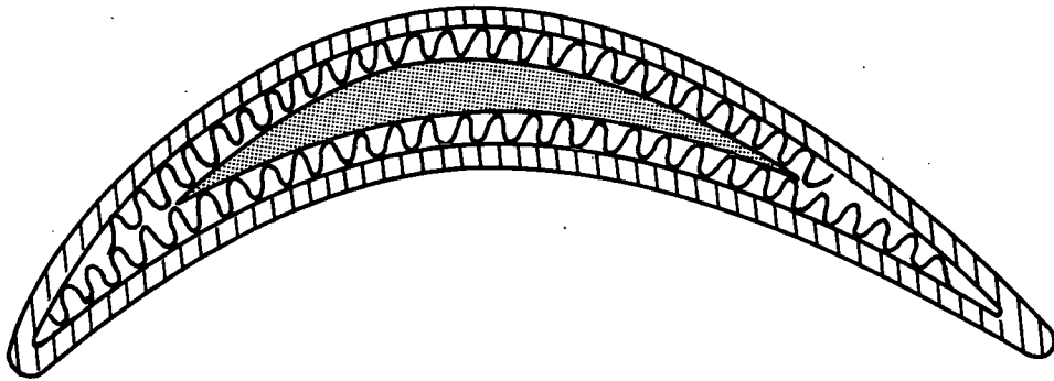
(a) Typical corrugated-insert blade.
