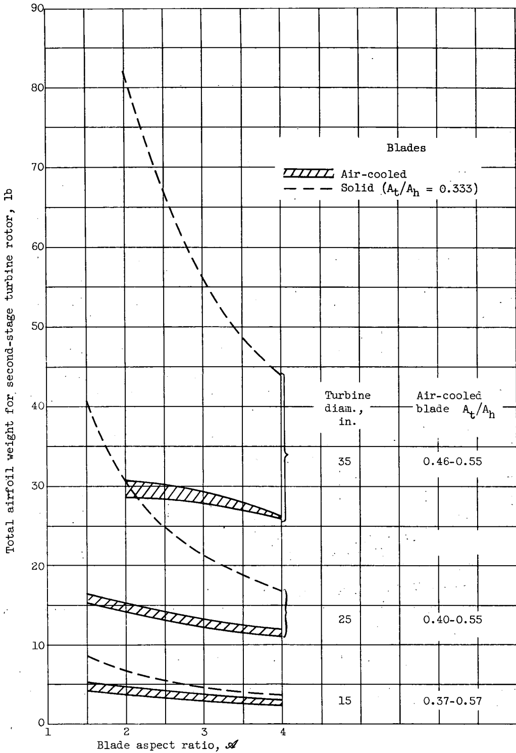
(b) Second stage. Hub-tip radius ratio, 0.60.
