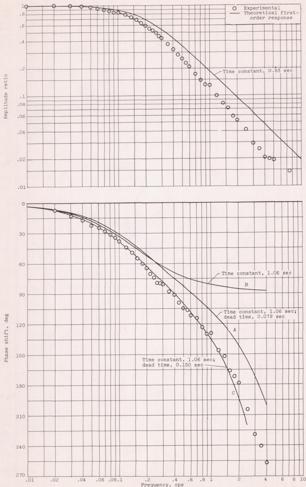
Figure 4. - Frequency response of engine rotational speed to sinusoidal input to fuel valve. Operating range, 95.5±3 percent rated speed.
