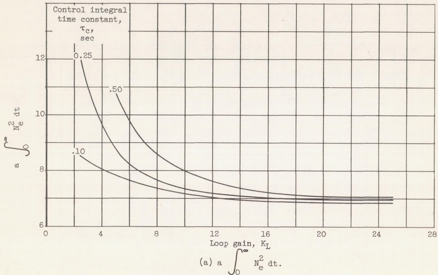
Figure 20. - Variation of integral criteria with loop gain for speed-area control type I.
