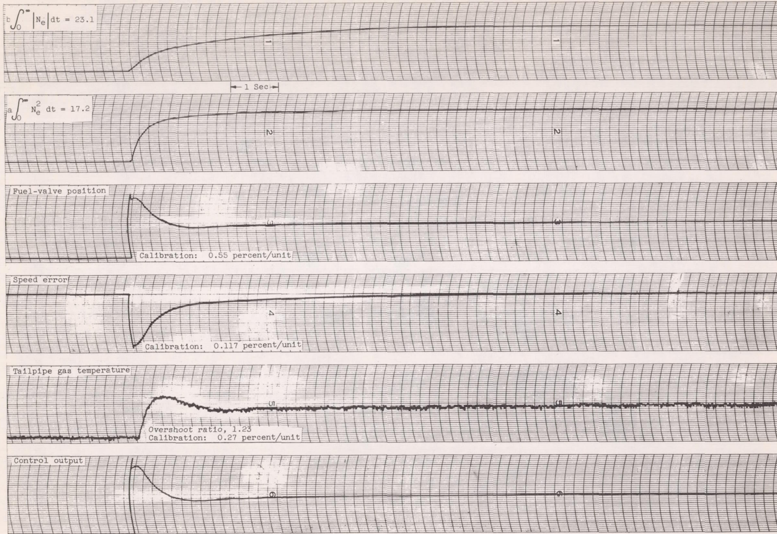
(a) Control integral time constant, 2.0 seconds; loop gain, 1.5.
