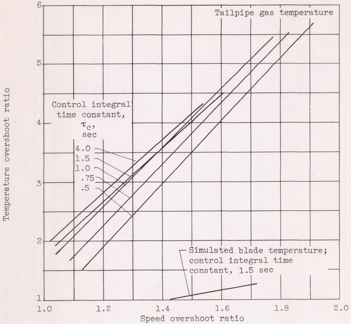
Figure 12. - Variation of tailpipe-gas-temperature overshoot ratio with speed overshoot ratio for speed - fuel-flow control.
