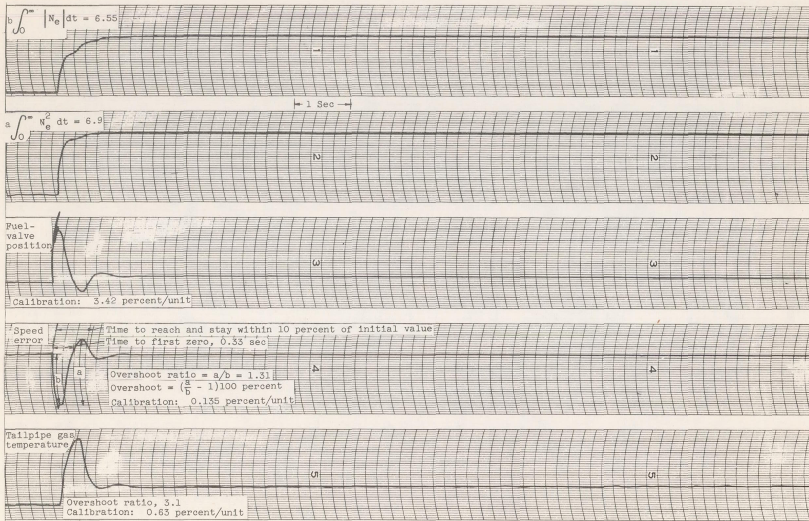
(b) Control integral time constant, 1.5 seconds; loop gain, 7.4.
