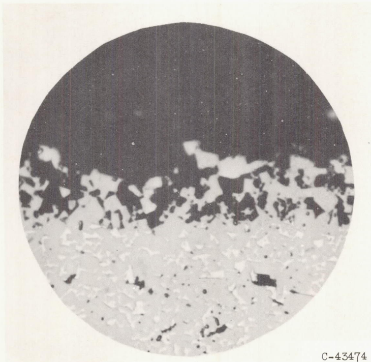
(h) Roughened with aqua regia.
