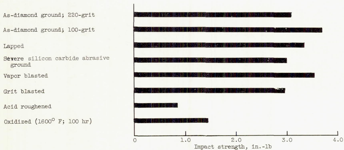
(b) Average impact strength.
