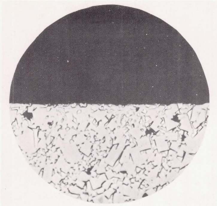
(a) 220-Grit diamond-abrasive ground.
