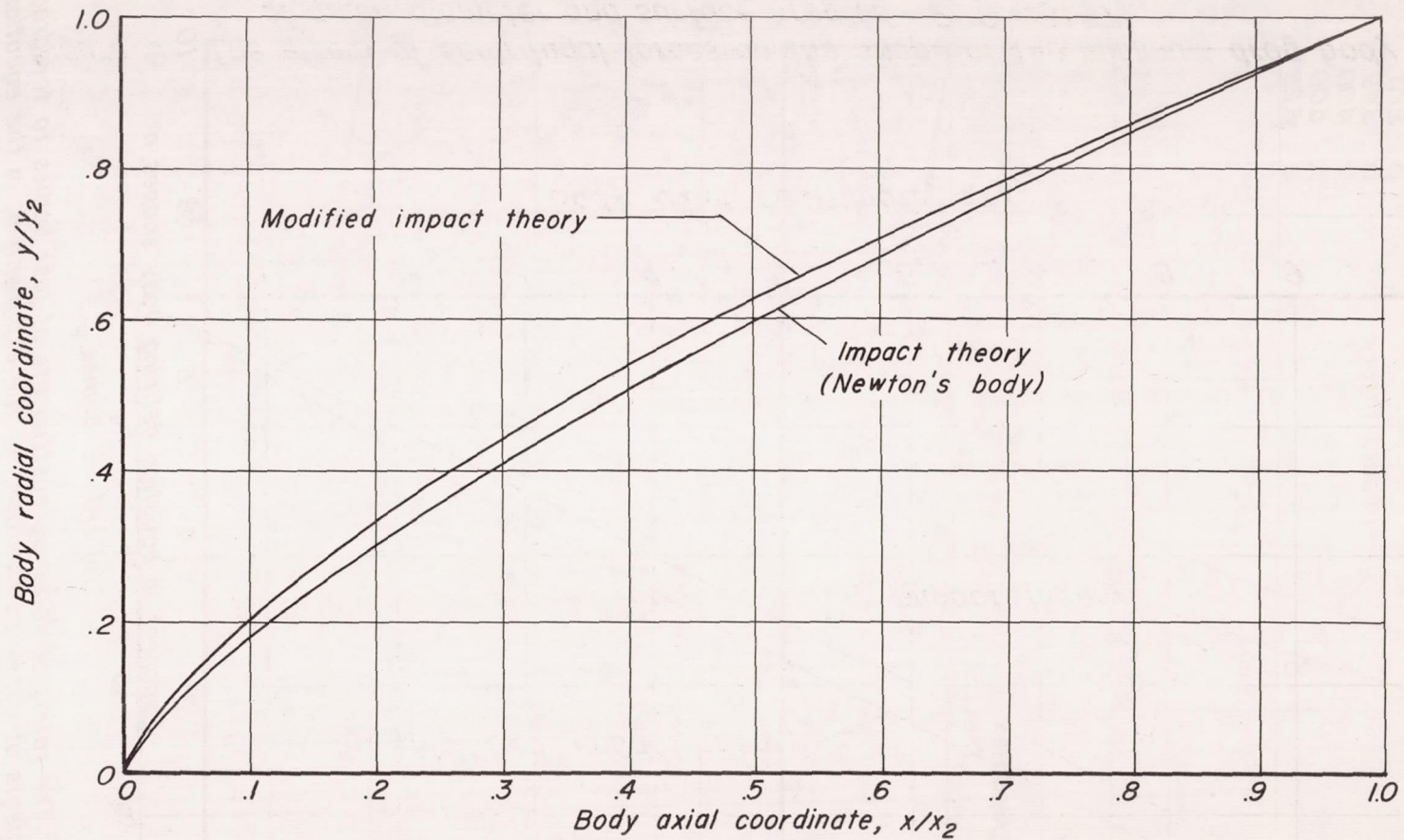
Figure 8.- The effect of centrifugal forces on the shape of the minimum drag body of given length and base diameter. ( 1/d=6.18 )
