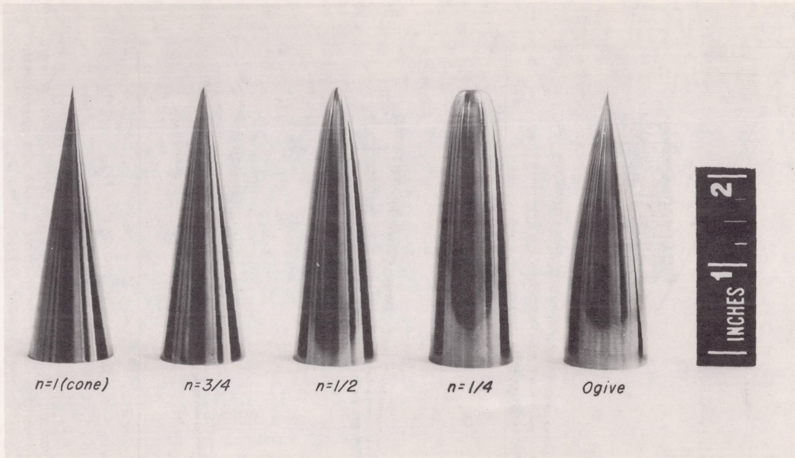
(a) Fineness ratio 3 bodies.
