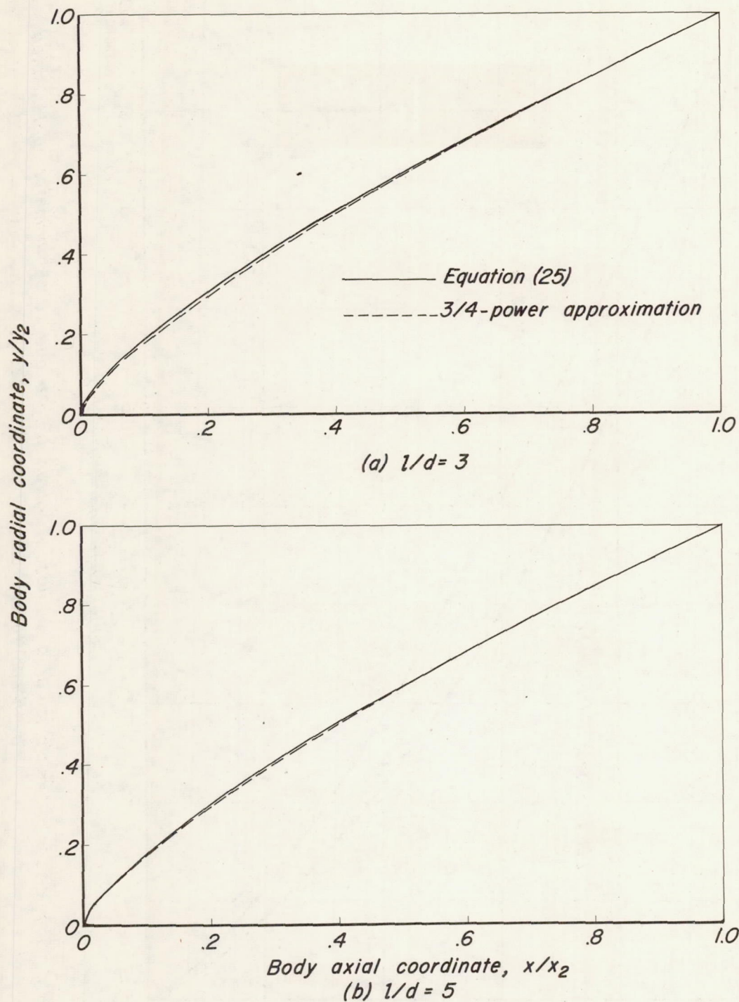
Figure 4.— Comparison of profiles of minimum drag bodies of revolution for given lengths and base diameters with the approximate profiles employed in the present tests.
