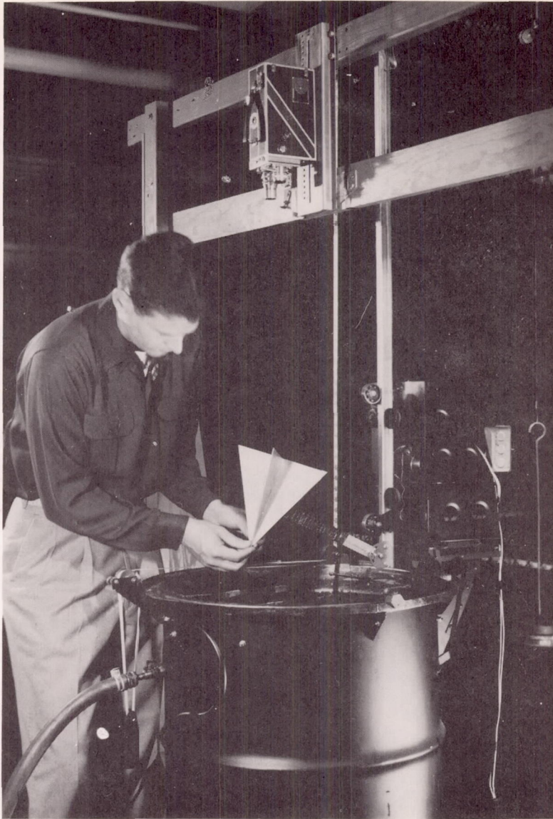
Figure 2.- Water tank with cruciform model.
