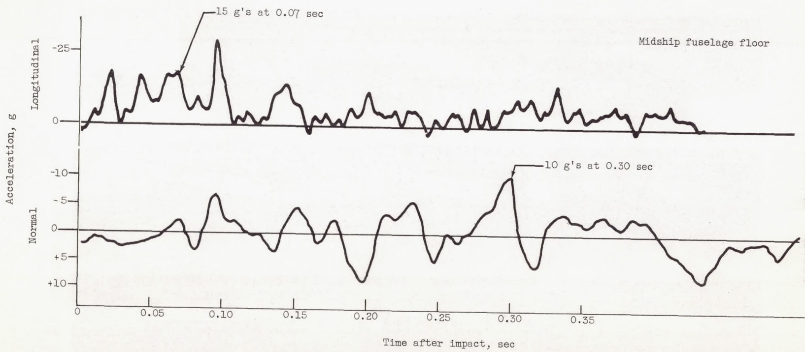
(a) Concluded. Sequence pictures and accelerations of 16° crash of high-wing airplane. Impact speed, 91 mph.
