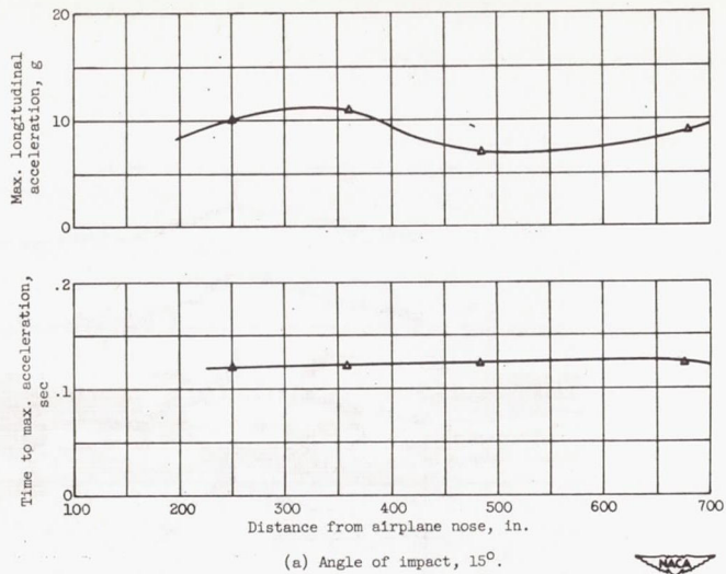
Figure 4. - Variation of maximum longitudinal acceleration and time to reach peak acceleration with position in airplane during crashes of pressurized transports.
