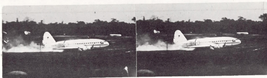
Figure 3. - Sequence pictures and accelerations of crashes of pressurized transports. (Zero time is fuselage nose impact with ground.)
