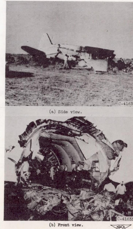
Figure 6. - Extent of fuselage crumpling resulting from Louisville crash of pressurized transport at 50° angle of impact and 150 mph. Photograph courtesy of Aviation Crash Injury Research of Cornell University.
