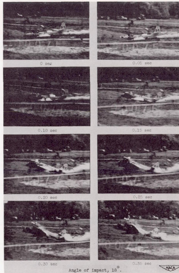
Figure 15. - Sequence pictures of crash of FH-1 fighter airplane.
