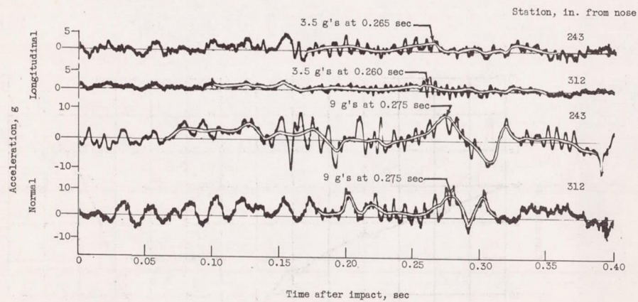
(b) Accelerations.
