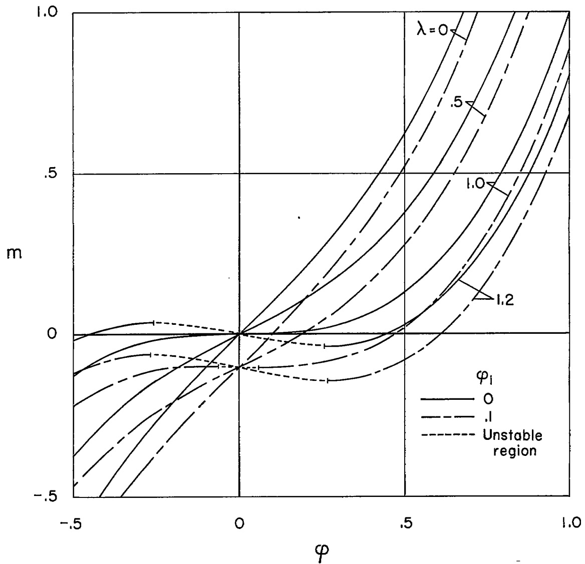
Figure 4.- Calculated twist as a function of applied moment for several combinations of temperature ratio and initial twist.
