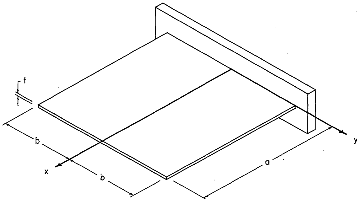
Figure 1.- Dimensions and coordinate system of cantilever plate.
