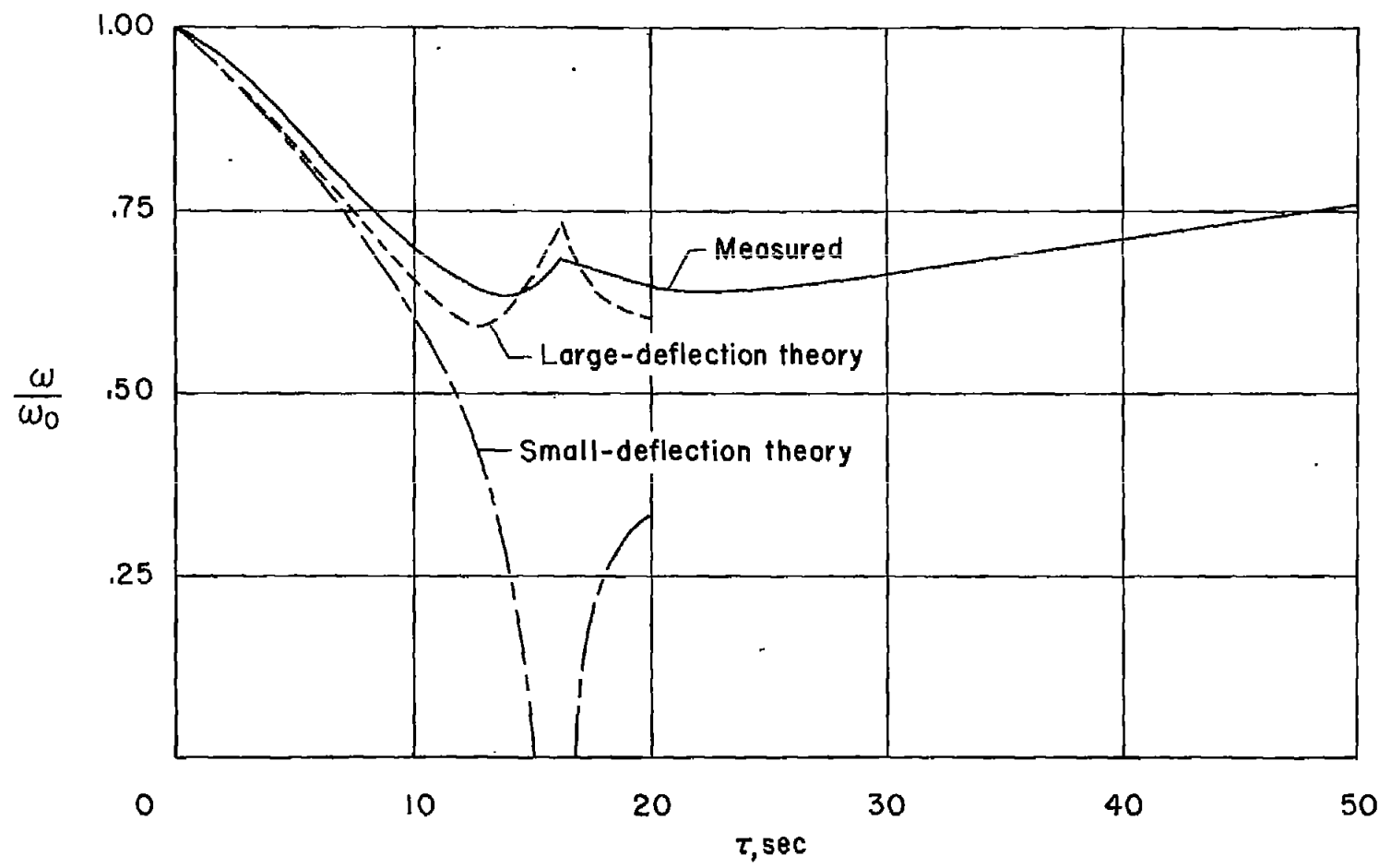
Figure 11.- Comparison of measured and calculated values of frequency ratio as a function of time for the rapidly heated plate.
