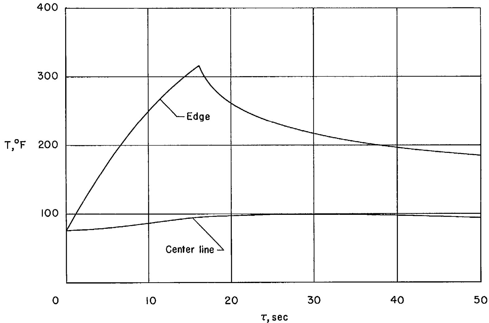
Figure 7.- Measured temperature histories for a heated edge and the center line of the plate test specimen.
