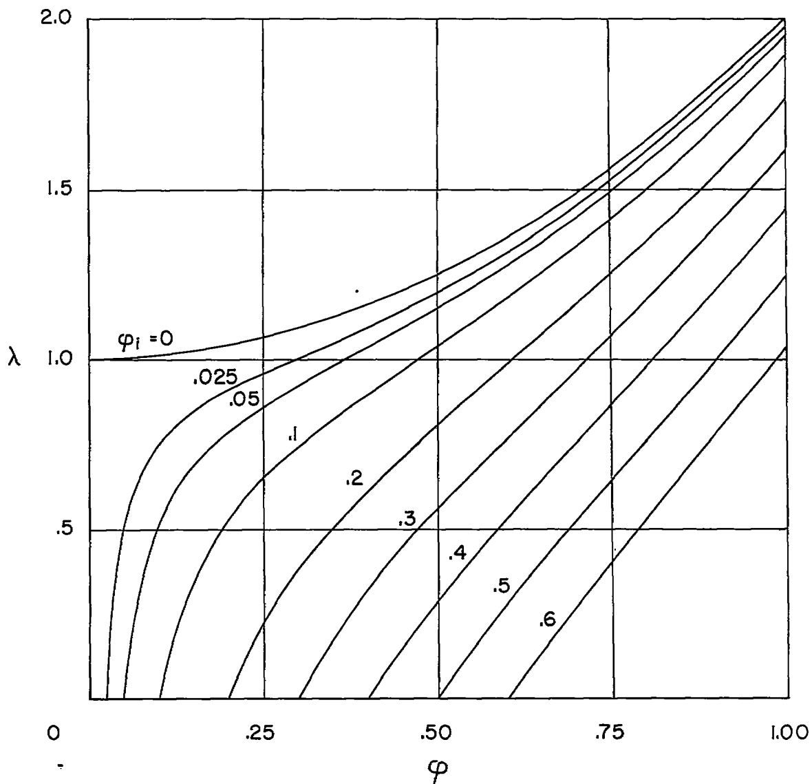
Figure 3.- Calculated twist as a function of temperature ratio for several values of initial twist.
