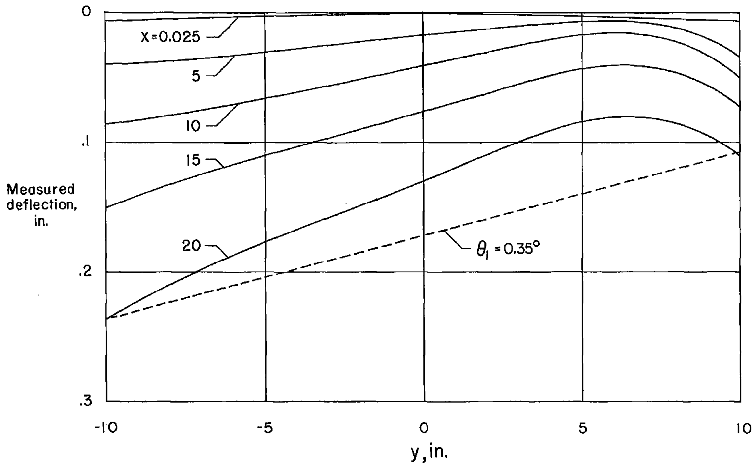
Figure 8.- Initial shape of plate test specimen.
