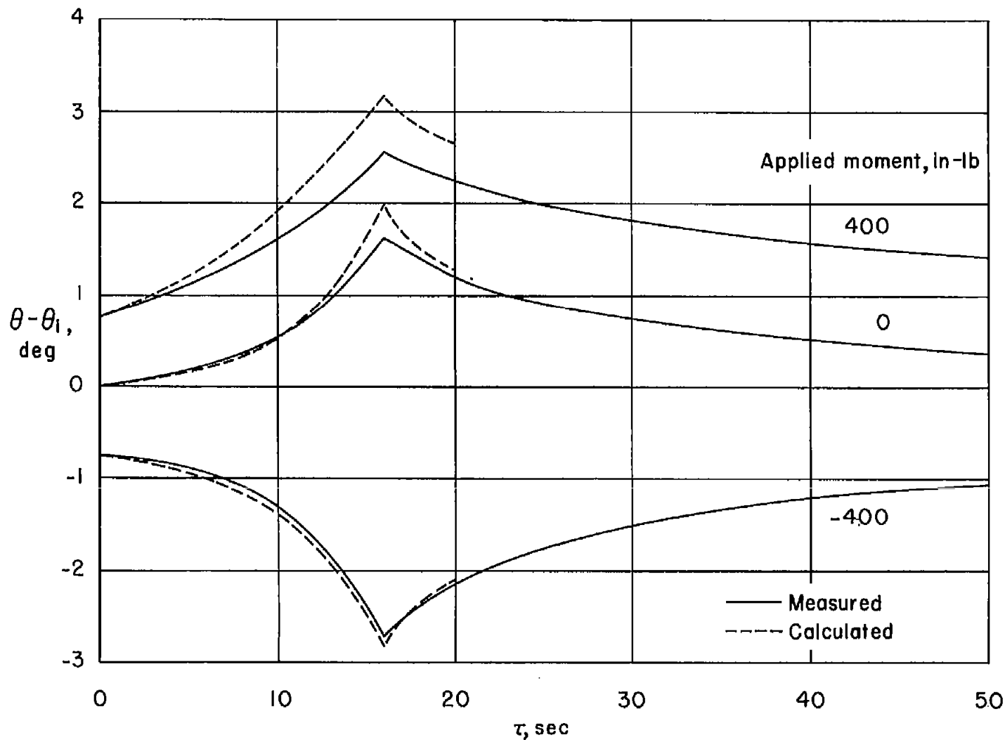
Figure 9.- Comparison of measured and calculated values of twist as a function of time for the rapidly heated plate for three values of applied moment.
