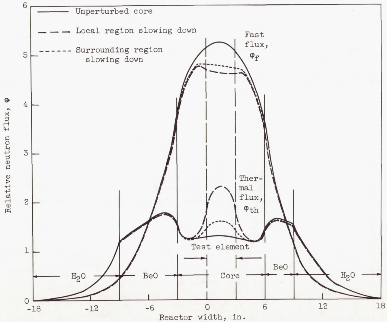
Figure 10. - Flux distributions along reactor width; slowing-down comparisons for cases with 10 plates removed.
