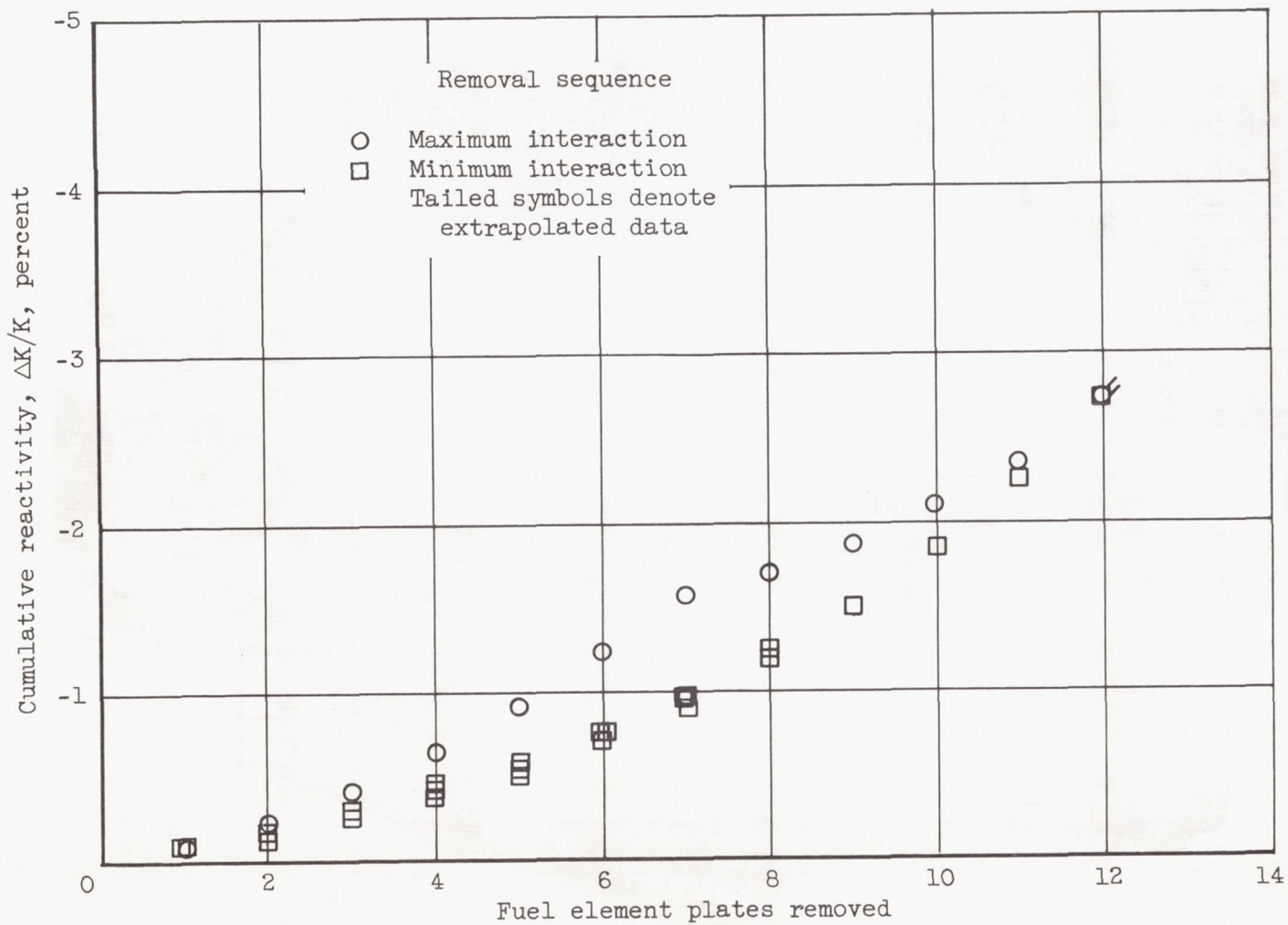
Figure 5. - Cumulative reactivity of fuel plates in element at grid position 25.
