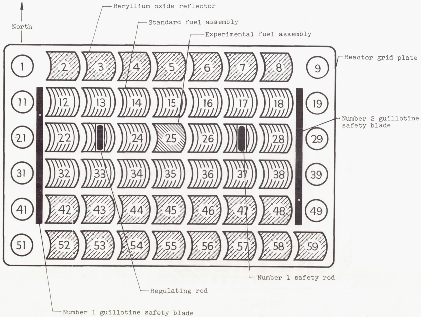
Figure 1. - Reactor loading for reactivity experiments at Bulk Shielding Reactor.
