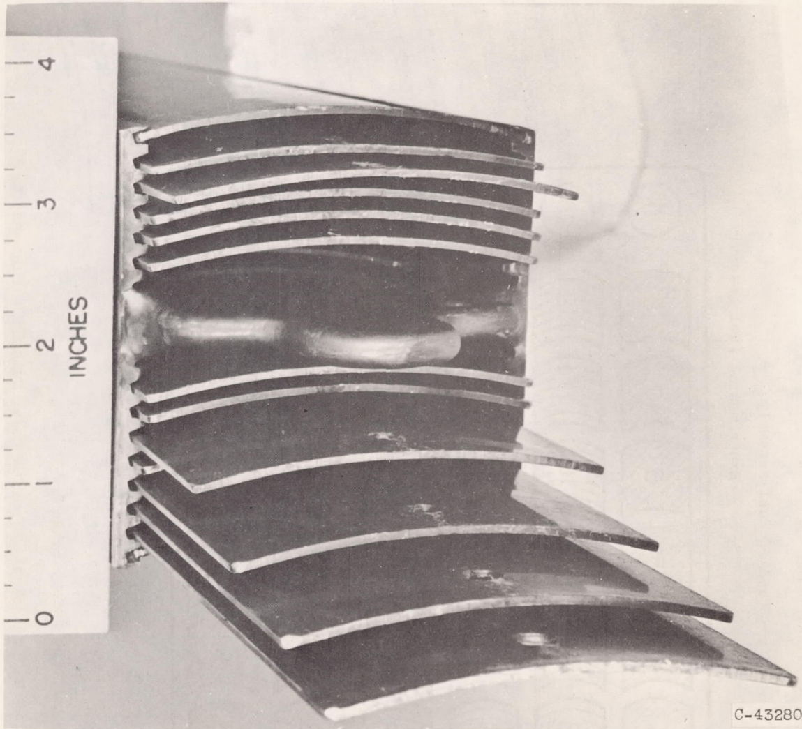
Figure 2. - Removable-fuel-plate element.
