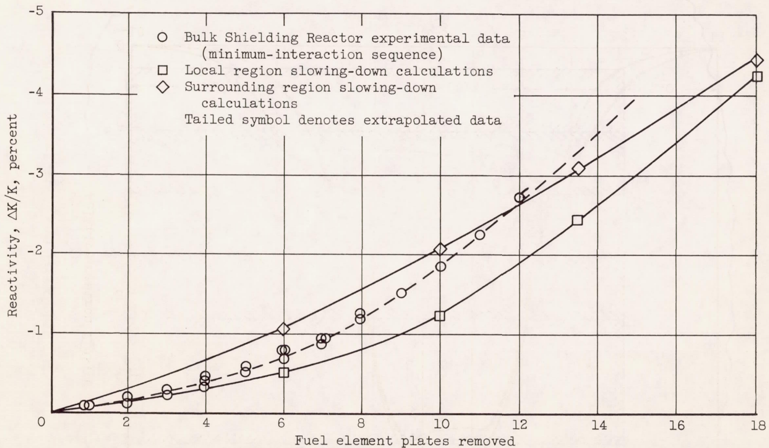
Figure 11. - Comparison of experimental and calculated reactivity effects of fuel-plate removal.
