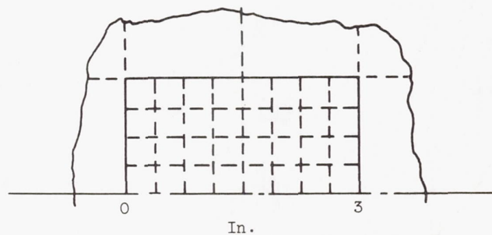
Removable-fuel-plate assembly at center of core
