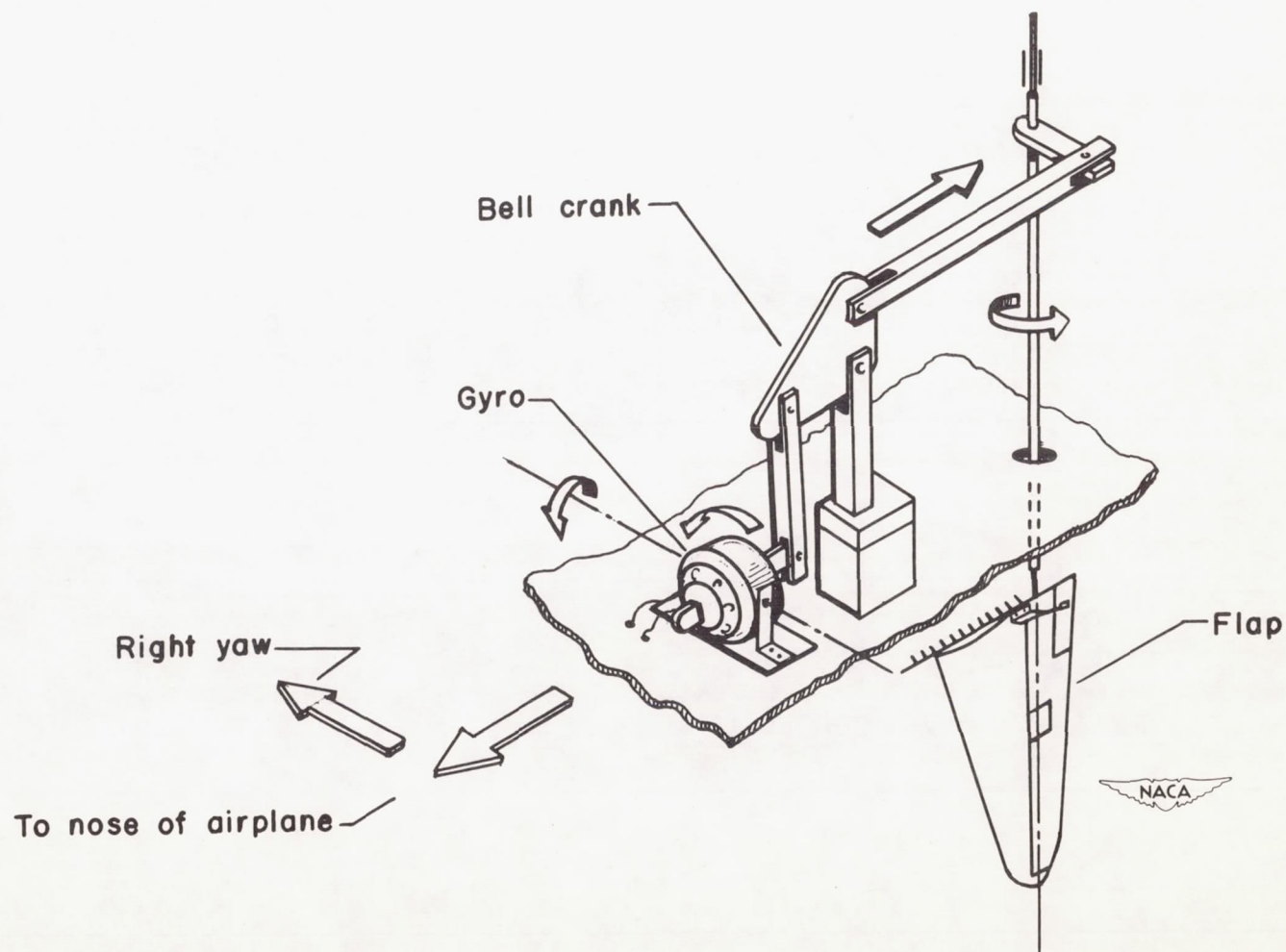
Figure 3.- Sketch of the variable-damping device used in this investigation. (Shaded arrows indicate response of system to right yawing velocity when acting as a yaw damper.)
