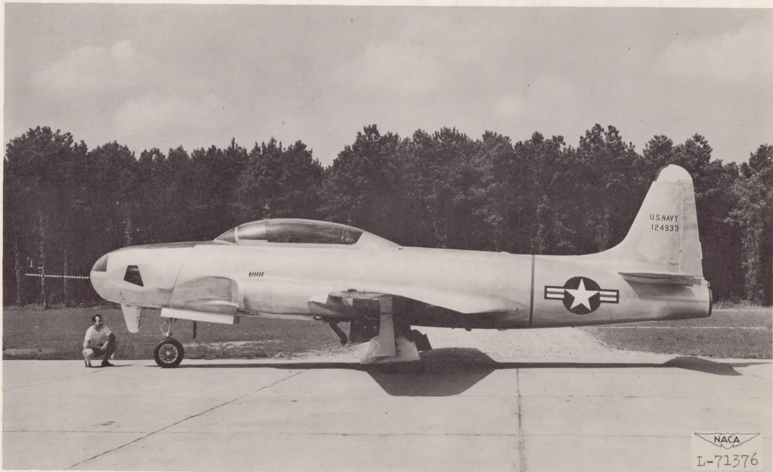
Figure 2.- Photograph of the test airplane.
