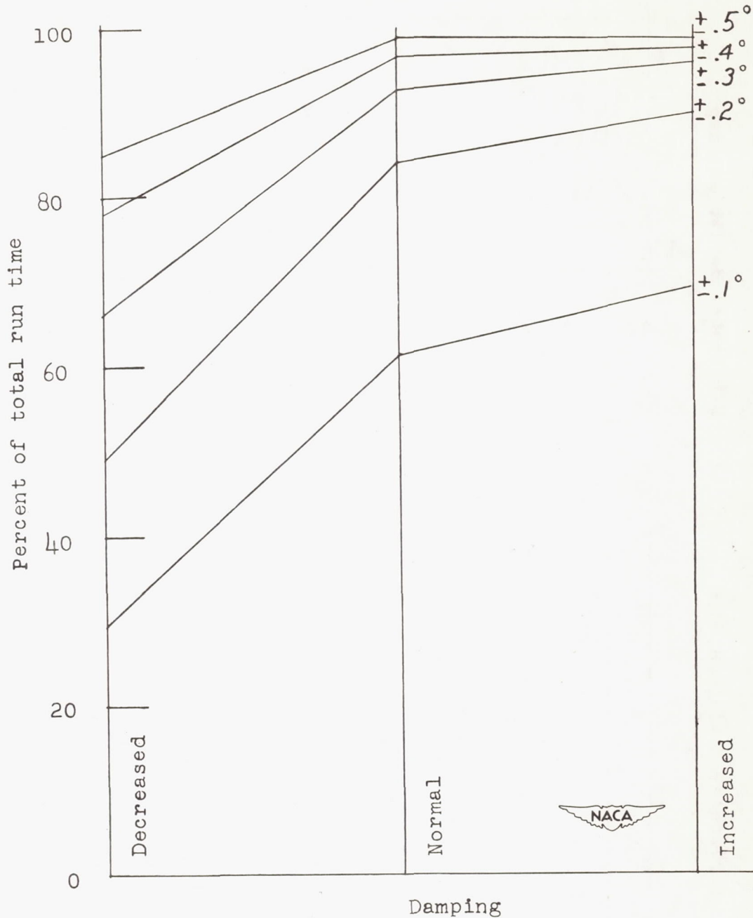
Figure 11.- Average variation of the percentage of total run time during which the sight line is within horizontal increments of \pm 0.1^\circ , \pm 0.2^\circ , \pm 0.3^\circ , \pm 0.4^\circ , and \pm 0.5^\circ of the target as the lateral damping is increased during strafing runs made with the fixed sight.
