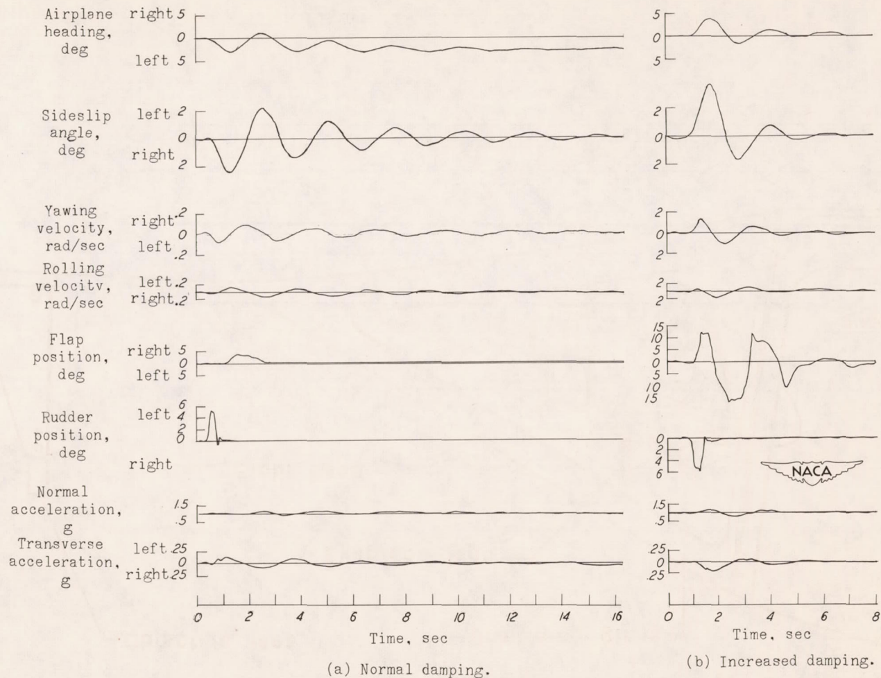
Figure 6.- Typical oscillation time histories of test airplane with normal, increased, and decreased damping following an abrupt rudder kick at an indicated airspeed of about 300 mph and an altitude of 30,000 feet.
