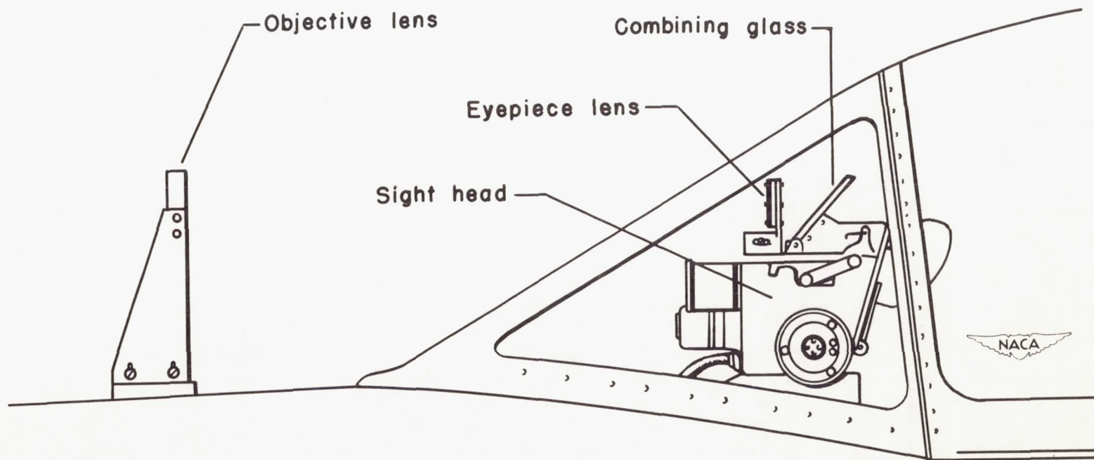
Figure 5.- Sketch of telescopic lens mounting in test airplane.
