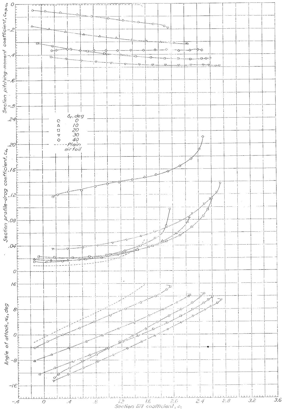
Figure 7.- Aerodynamic section characteristics of NACA 44012 airfoil with a 6.000 cotted flap 1-2. Slot gap = 0.03c.
