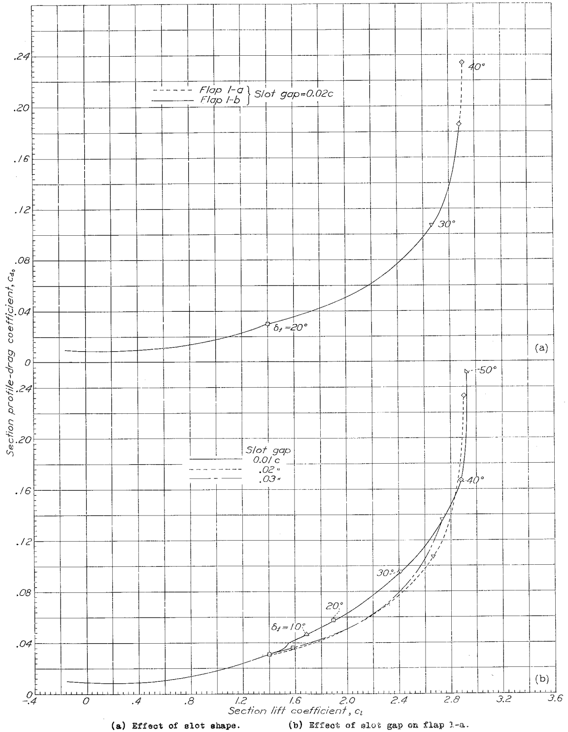
Figure 10.- Comparison of 0.30c slotted flaps on an NACA 23012 airfoil with extended slot lip.
