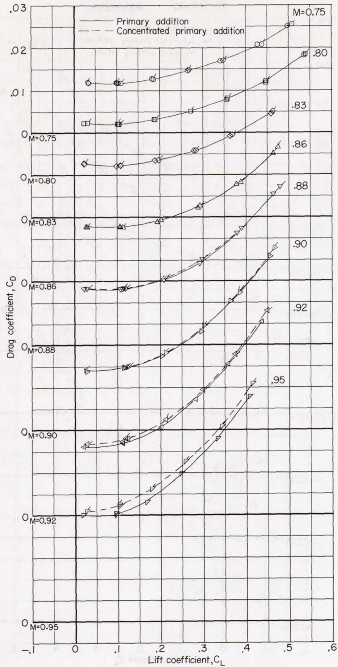
(f) Thick wing in low position; effects of concentrated primary addition.
