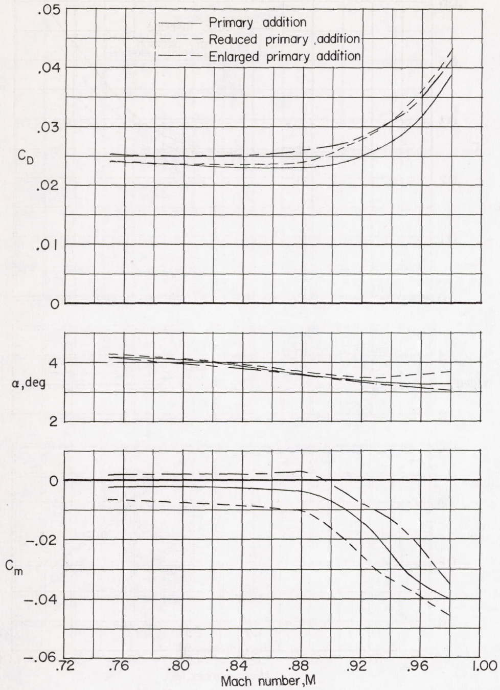
(d) Thin wing in low position; effects of addition size.
