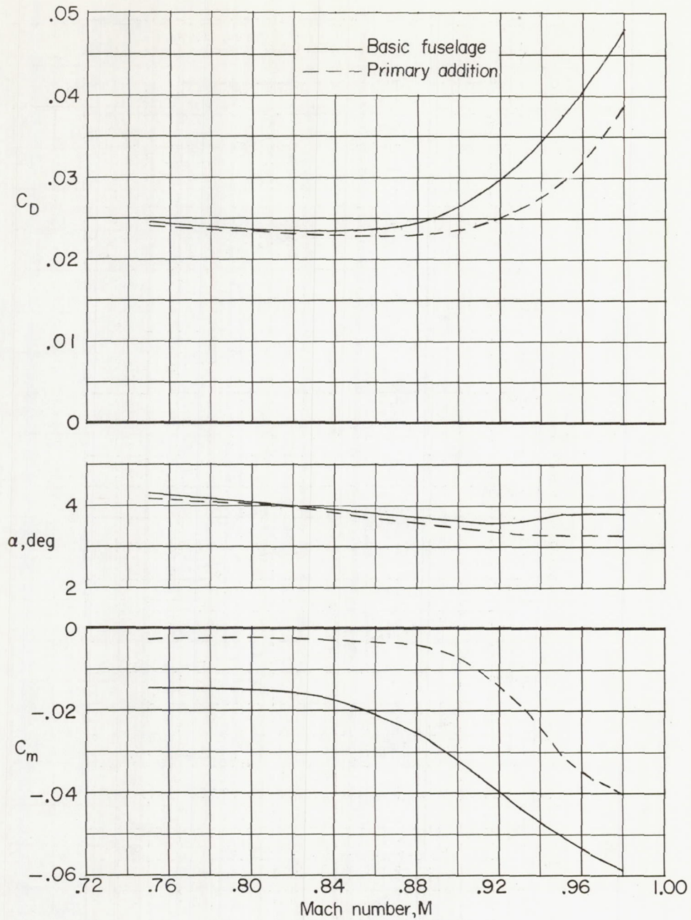
(a) Thin wing in low position; effects of primary addition.
