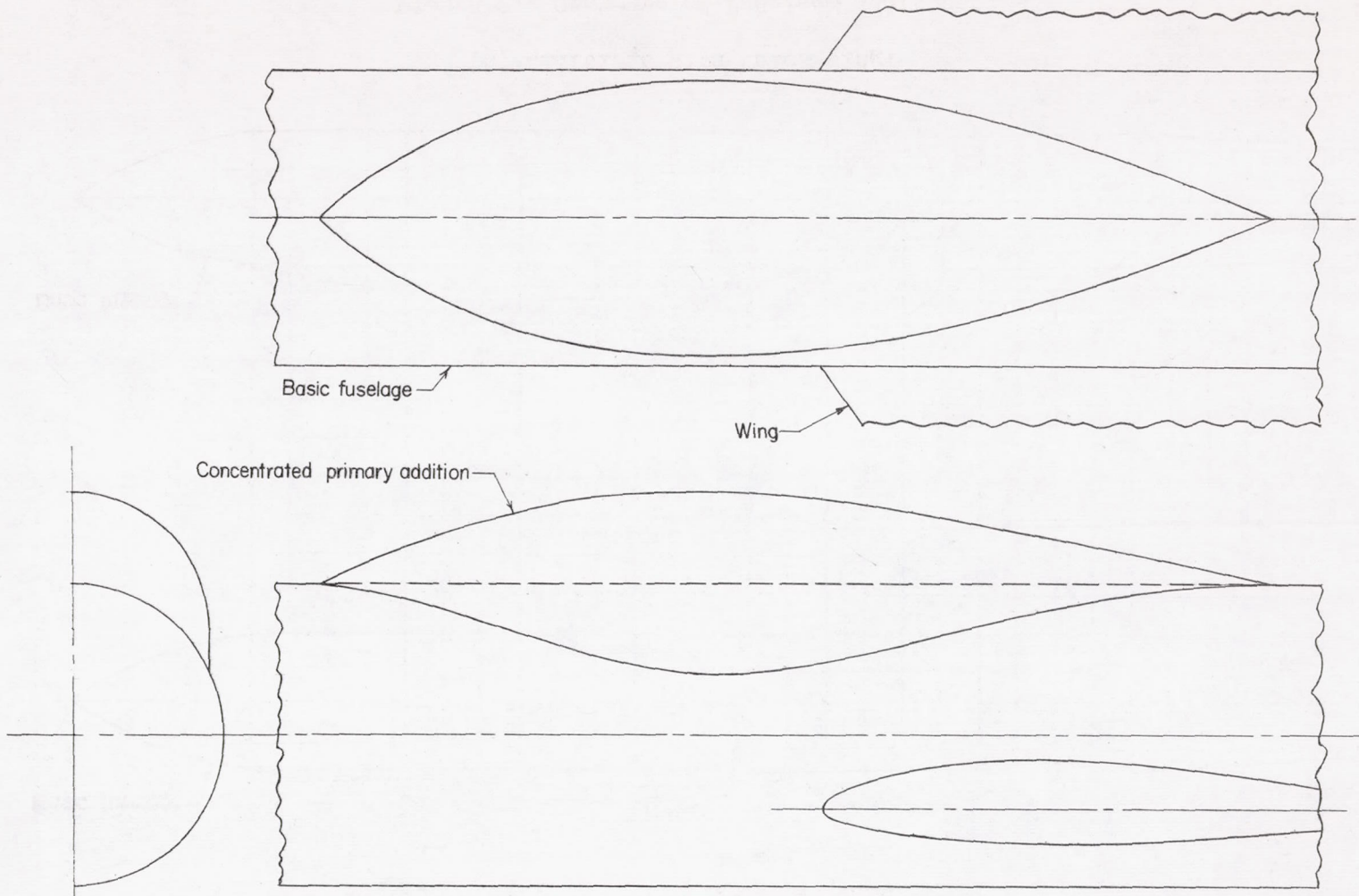
(c) Concentrated fuselage addition.
