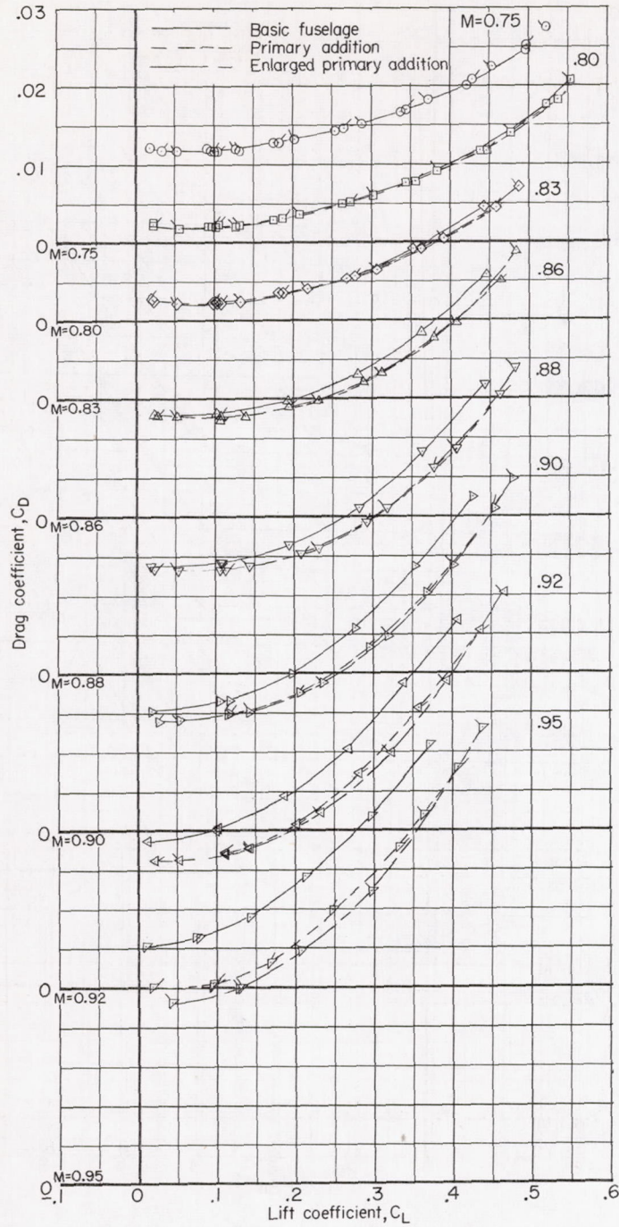
(b) Thick wing in low position; effects of primary addition.
