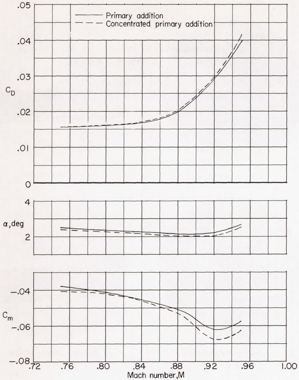
(f) Thick wing in low position; effect of concentrating primary addition.
