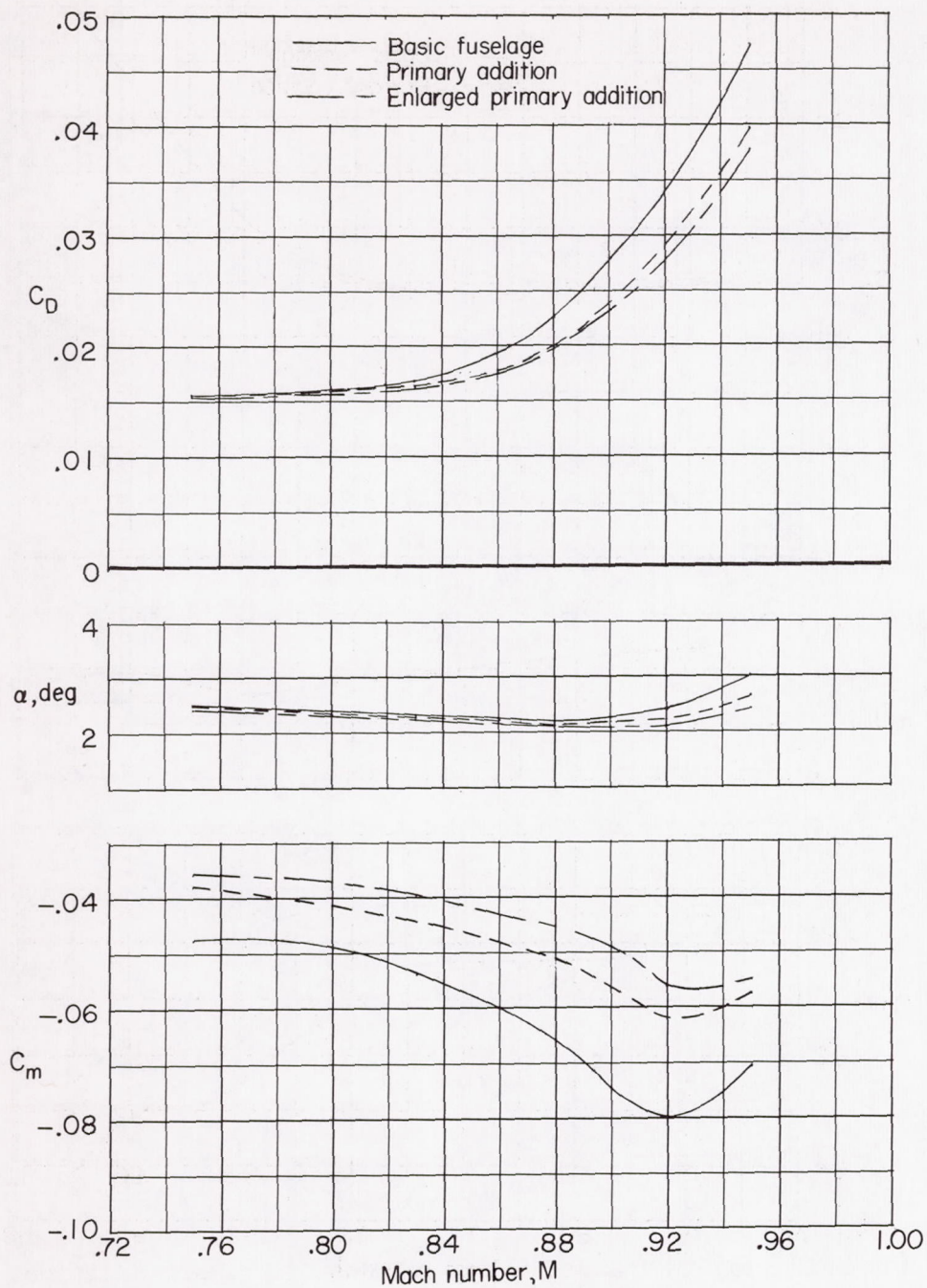
(b) Thick wing in low position; effects of primary addition.
