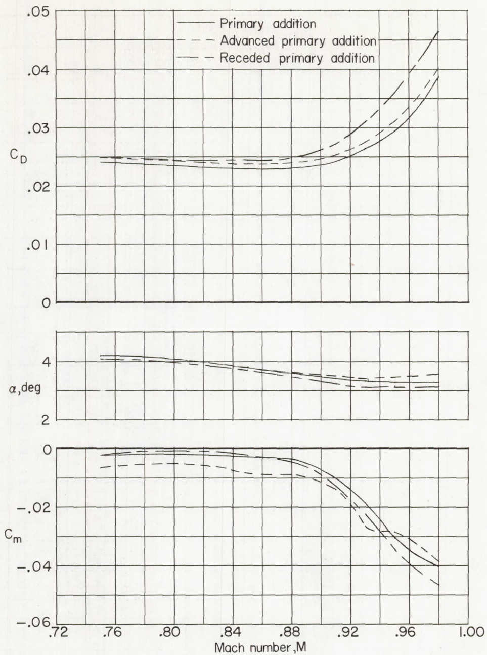
(e) Thin wing in low position; effects of longitudinal location of addition.
