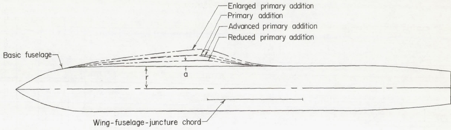
(a) Additions with thin wing.
