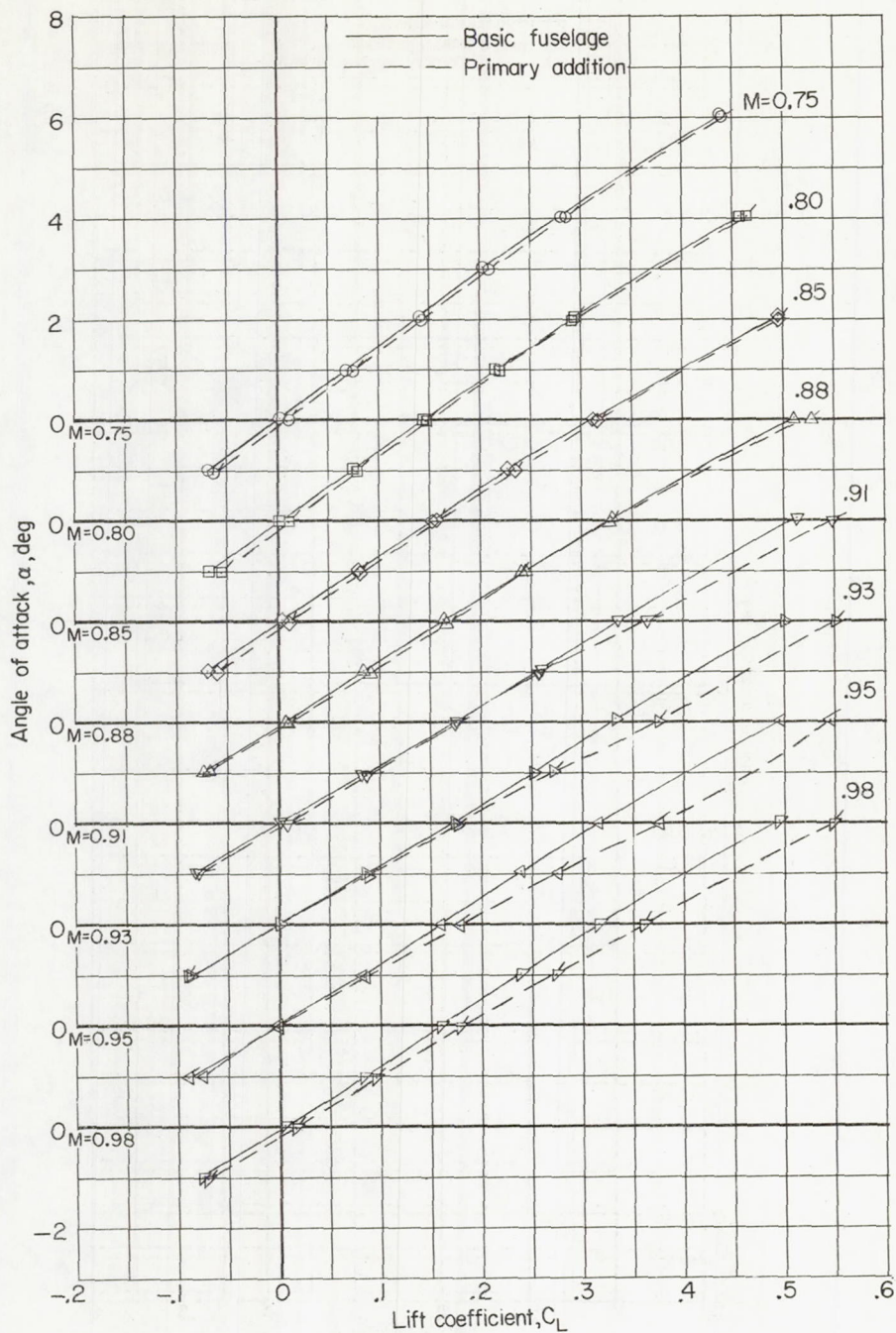
(a) Thin wing in low position; effects of primary addition.
