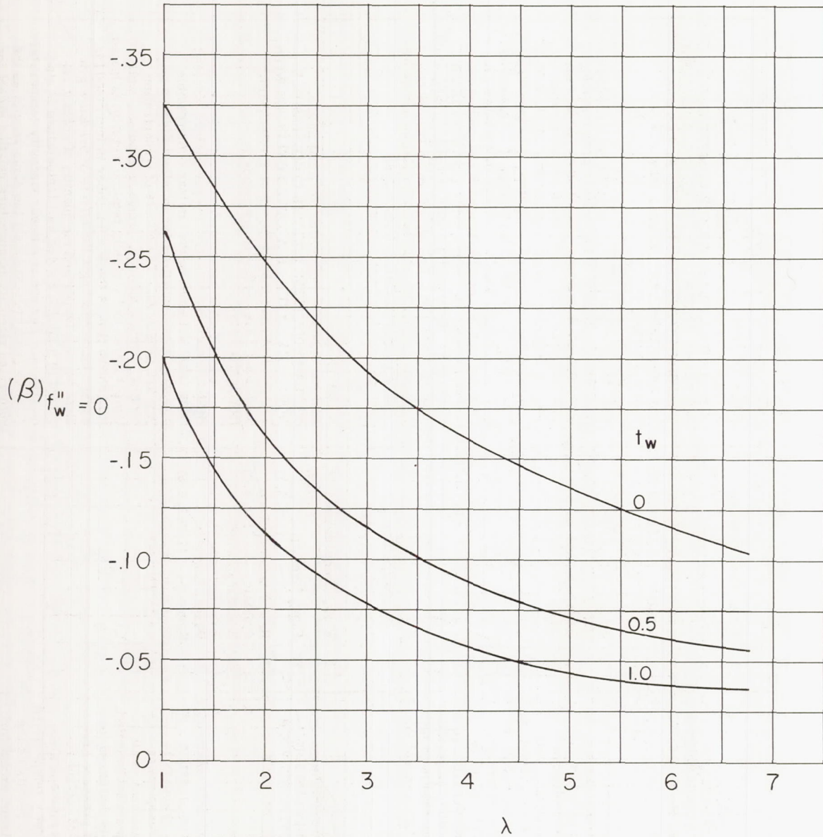
Figure 11.- Effect of yaw and wall temperature on pressure gradient required for chordwise separation. \phi = 1.0 ; N_{Pr} = 1.0 ; f_w = 0 .
