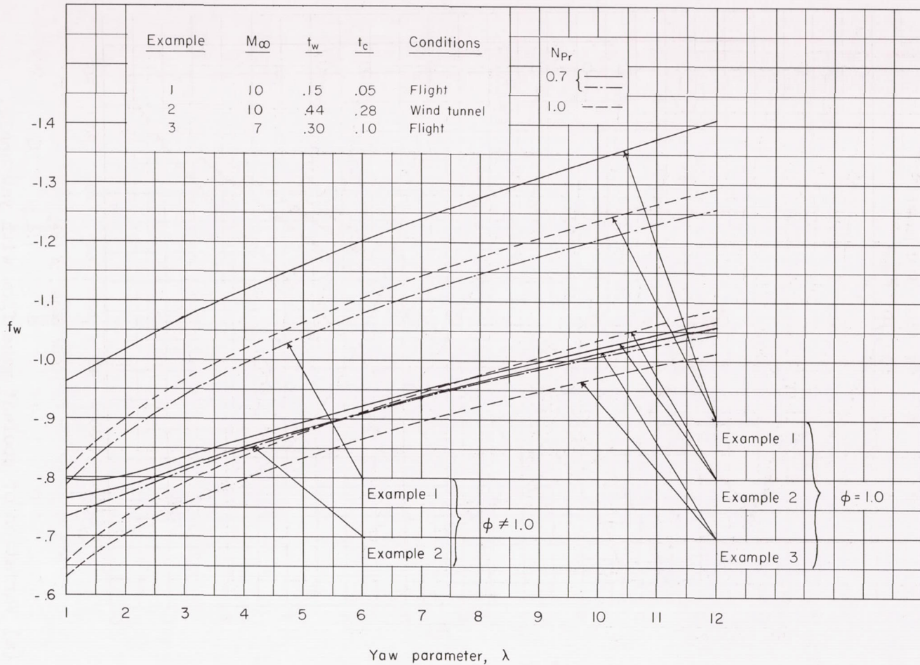
(b) Effect of compressibility on transpiration-cooling parameter. Curves for \phi = 1.0 have been arbitrarily extrapolated from \lambda = 6.5 to 11.0.
