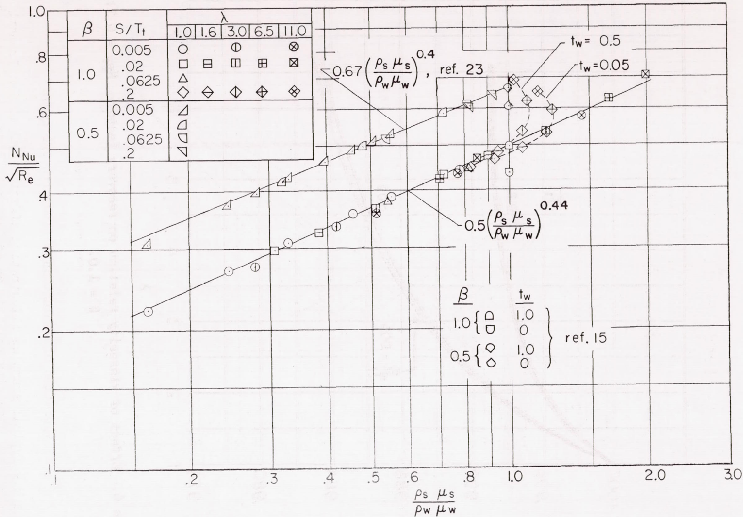
Figure 7.- Heat-transfer parameter at stagnation point on a body of revolution ( \beta = 0.5 ) and at the stagnation line of a yawed cylinder ( \beta = 1.0 ). N_{Pr} \approx 0.7 ; f_w = 0 .
