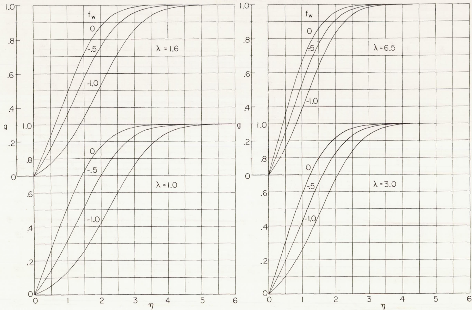
(b) Spanwise velocity ratios.
