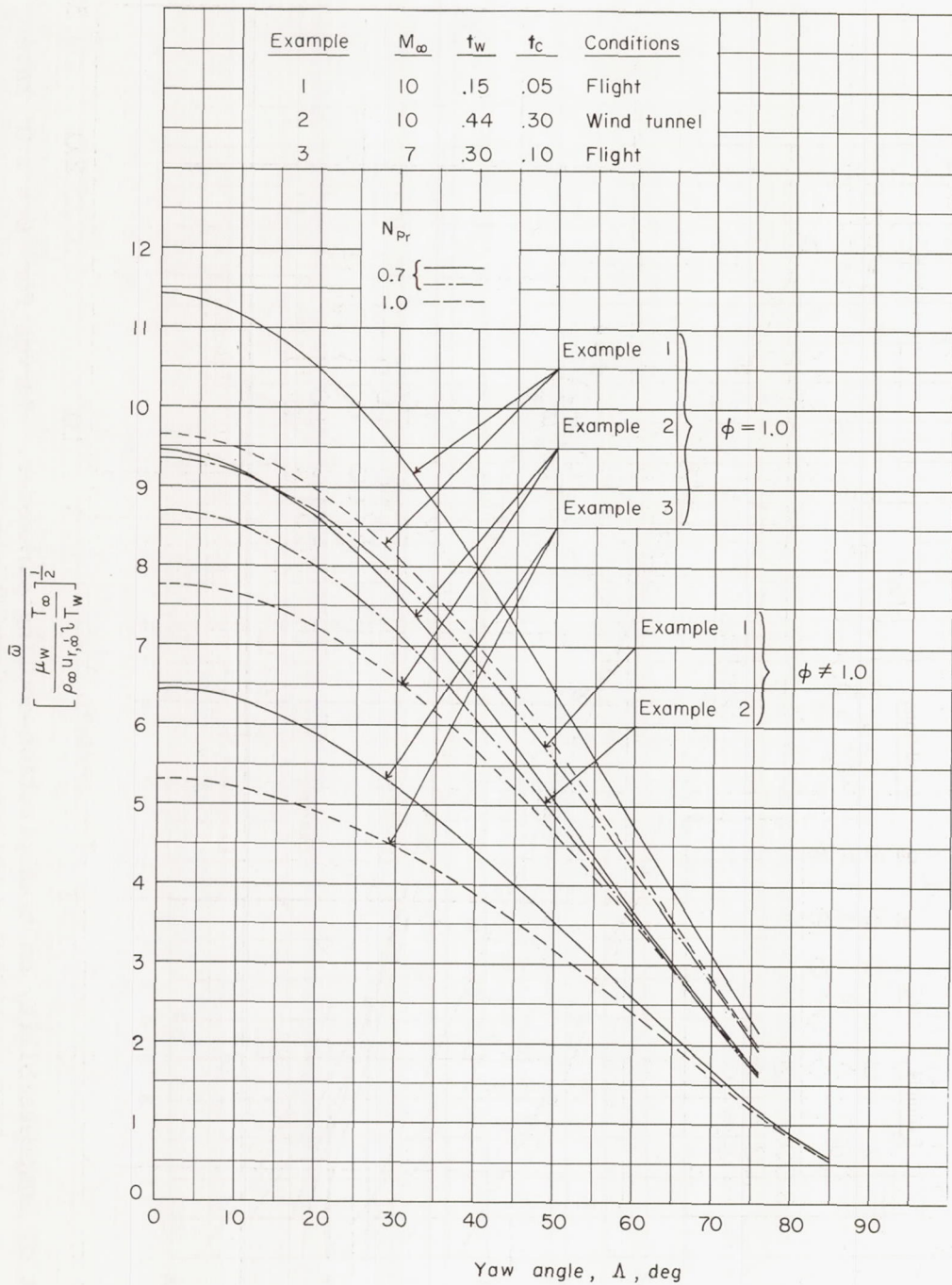
(a) Variation of coolant mass flow with yaw angle.
