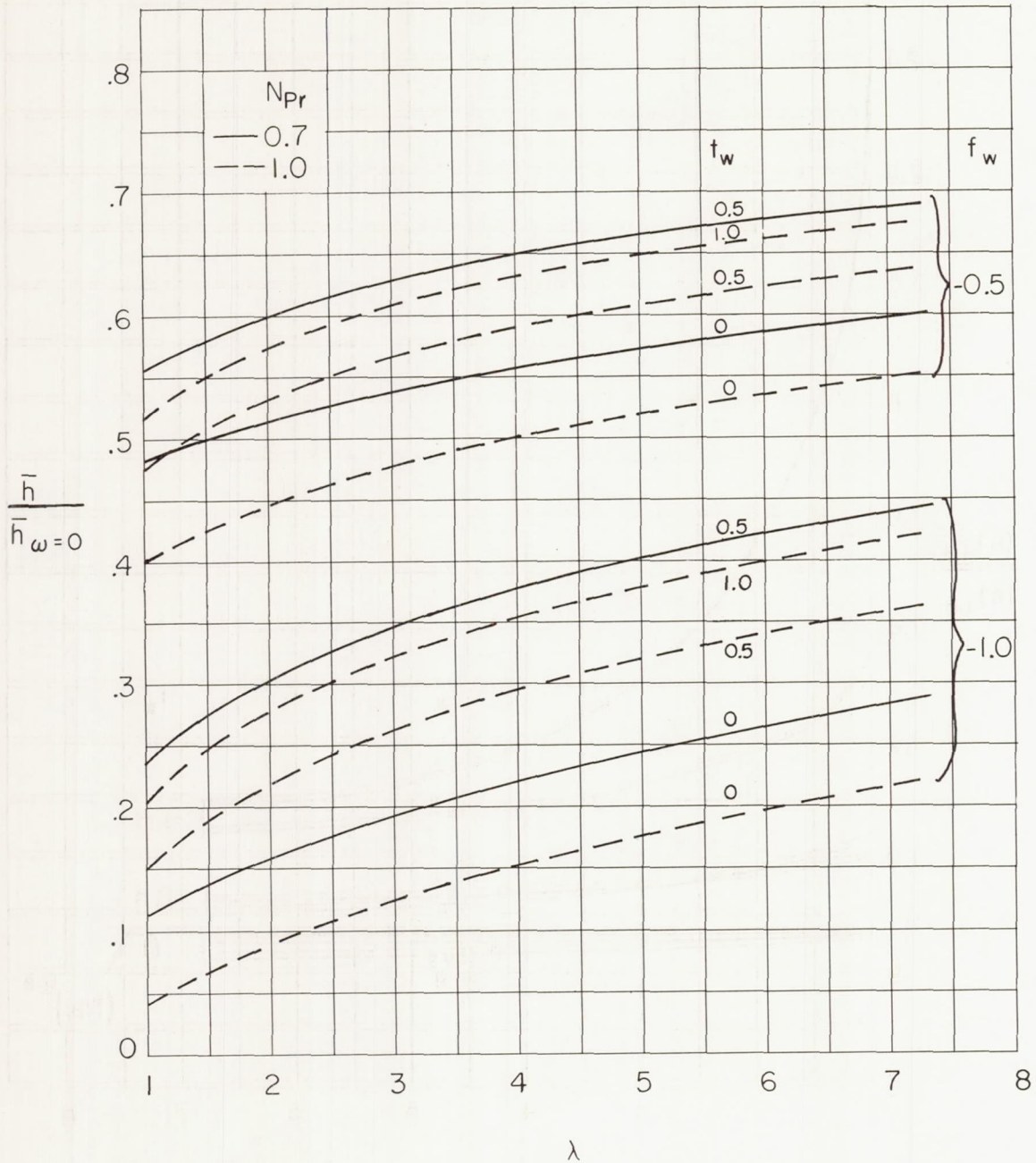
(b) Variation of ratio of \bar{h} for transpiration cooling to \bar{h} for non-porous wall with yaw-angle parameter.
