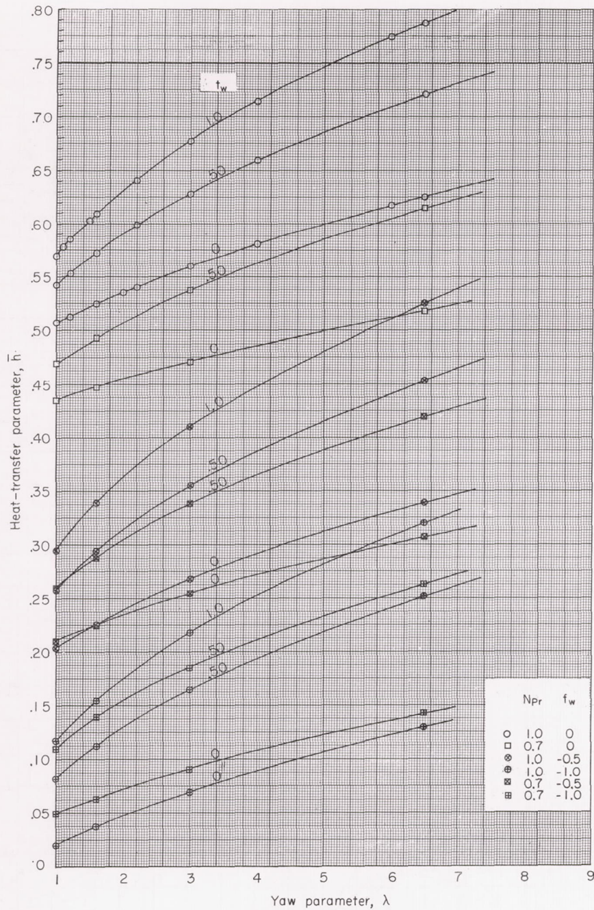
(a) Variation of heat-transfer parameter with yaw-angle parameter.
