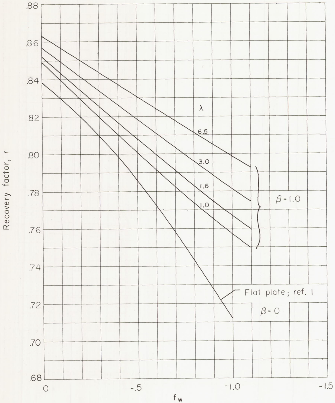
Figure 4.- Effect of transpiration cooling on recovery factor. \phi = 1.0 .
