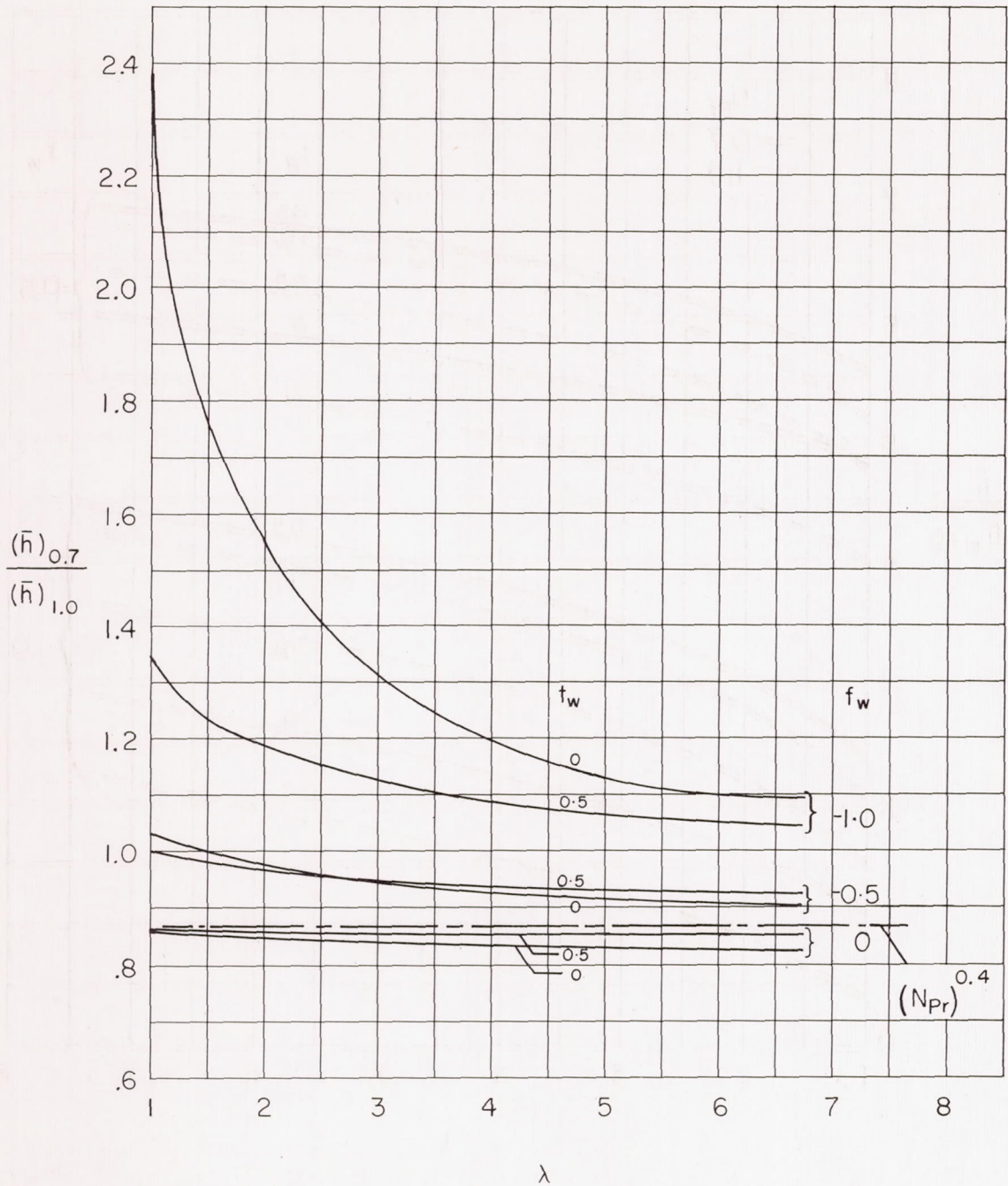
(c) Variation of ratio of \bar{h} for N_{Pr} = 0.7 to \bar{h} for N_{Pr} = 1.0 with yaw-angle parameter.
