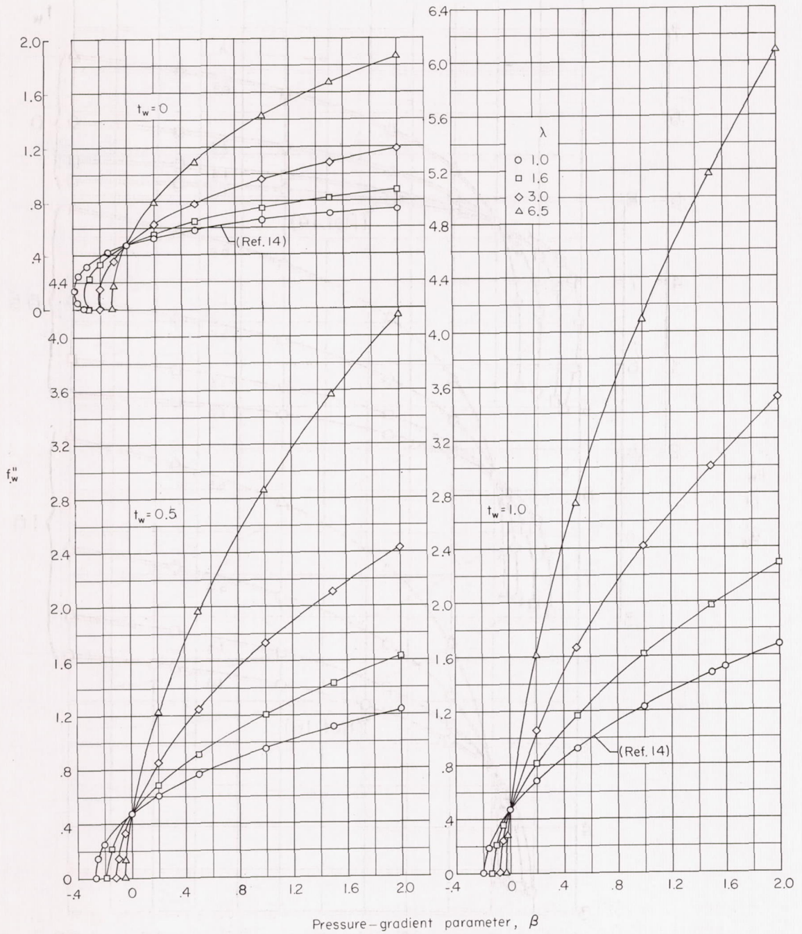
Figure 10.- Chordwise skin-friction parameter. \phi = 1.0 ; N_{Pr} = 1.0 ; f_w = 0 .
