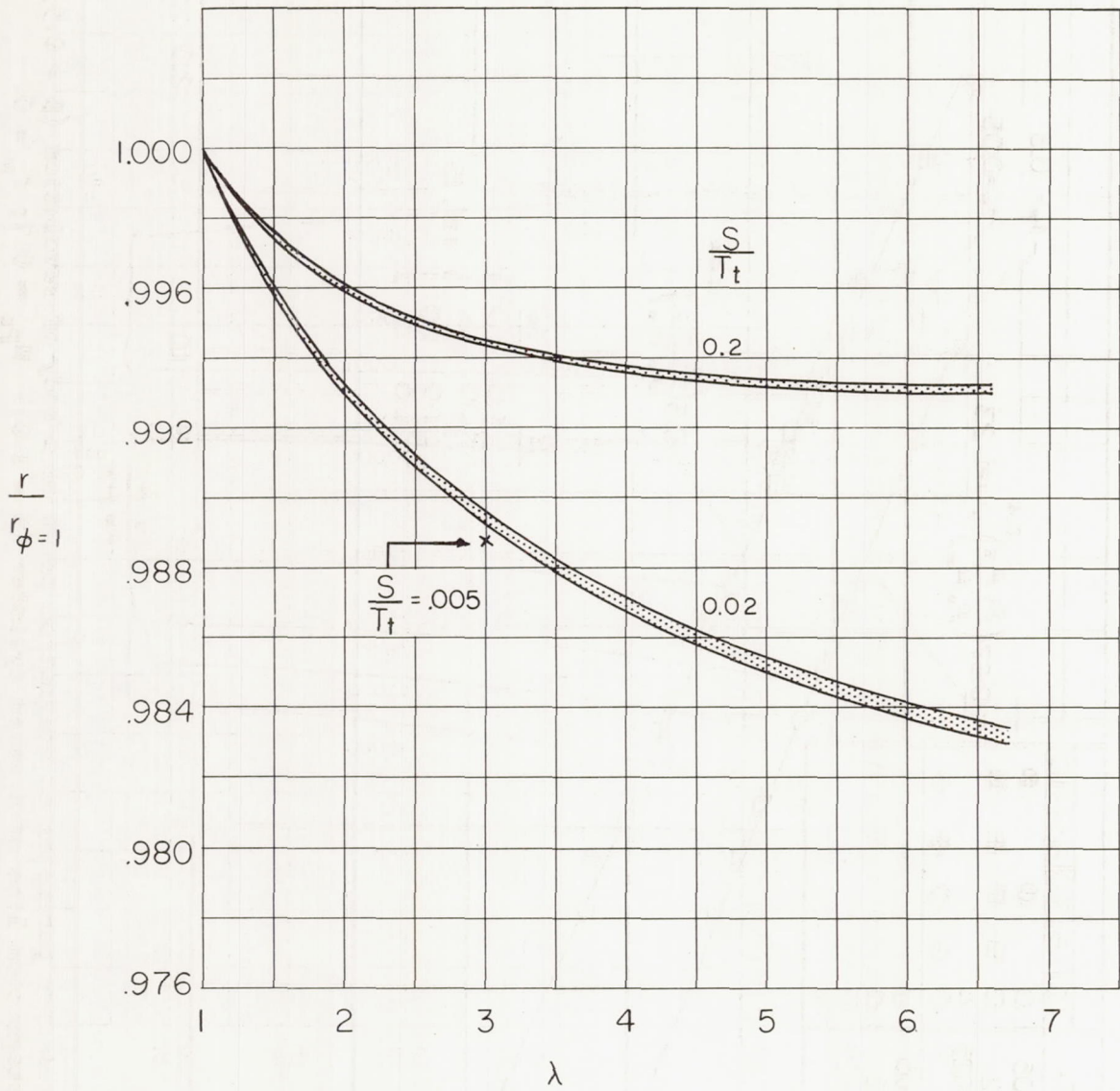
Figure 6.- Effect of viscosity relation on recovery factor. N_{Pr} = 0.7 ; \beta = 1.0 .
