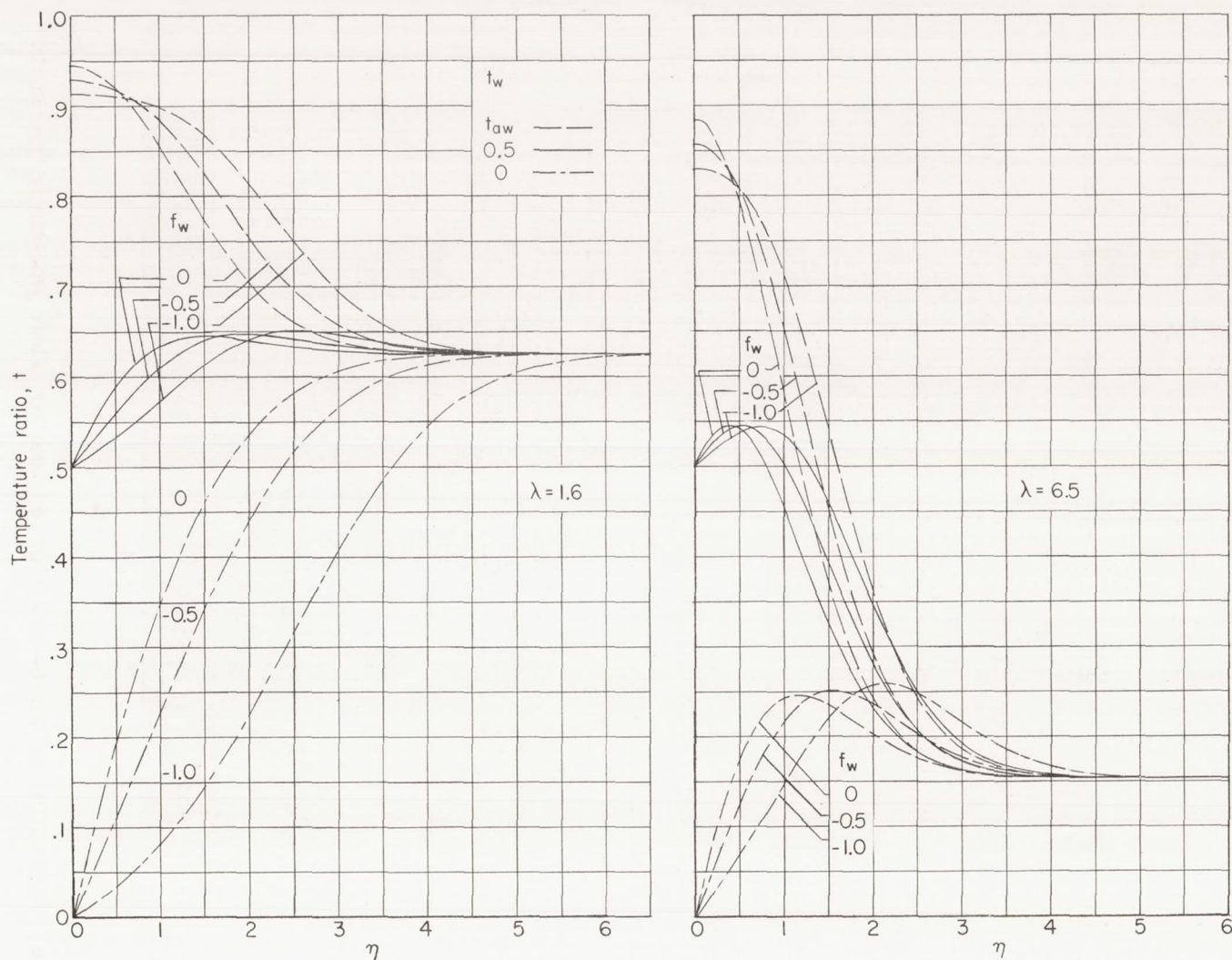
Figure 2.- Ratios of local static temperature to total stagnation temperature. \phi = 1.0 ; \beta = 1.0 ; N_{Pr} = 0.7 .
