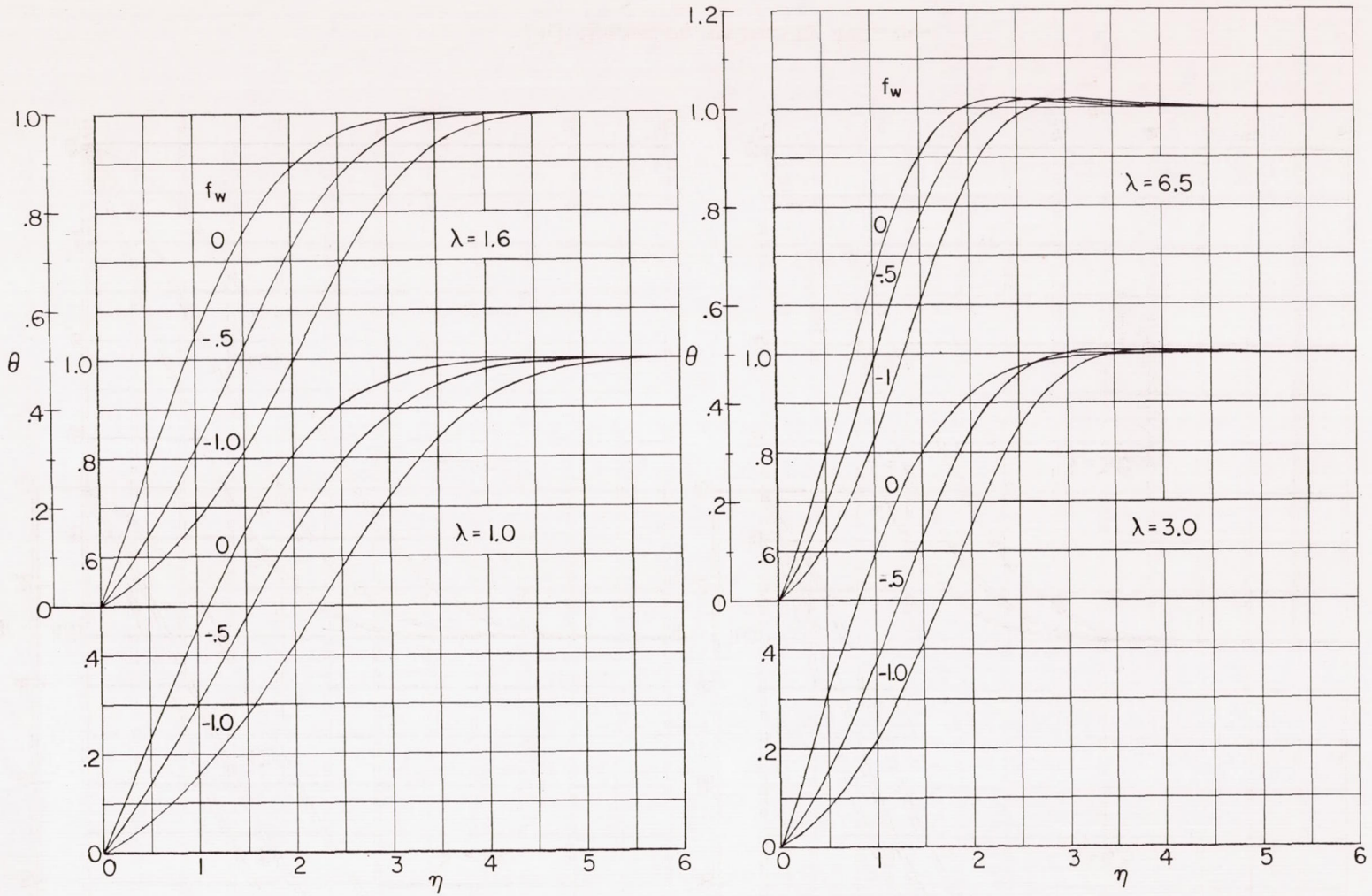
(c) Stagnation-enthalpy-difference ratios.
