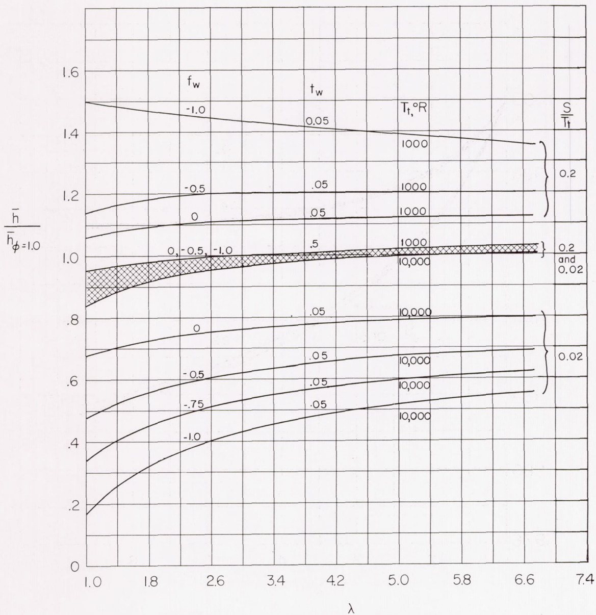
Figure 5.- Effect of viscosity relation on heat-transfer coefficient at stagnation line. N_{Pr} = 0.7 ; \beta = 1.0 .
