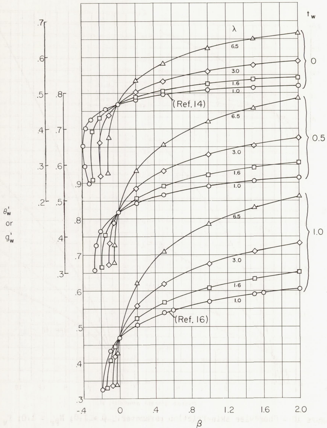
Figure 9.- Variation of heat-transfer and spanwise skin-friction parameters with pressure-gradient parameter. \phi = 1.0 ; N_{Pr} = 1.0 ; f_w = 0 .
