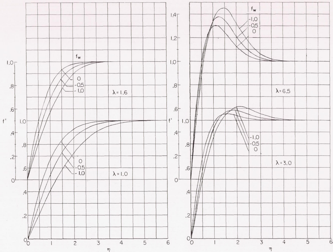
(a) Chordwise velocity ratios.
