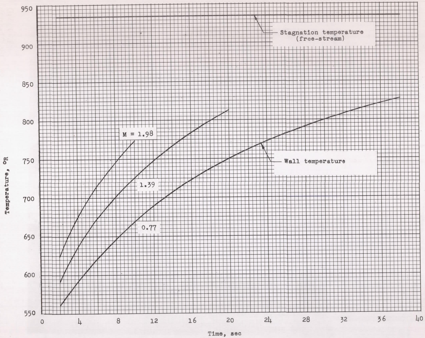
Figure 3.- Typical temperature time histories for three Mach numbers.
