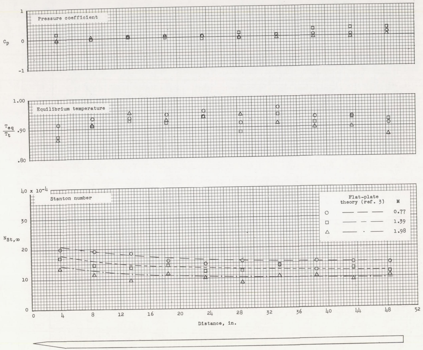
Figure 4.- Distribution of heat-transfer parameters and pressures for plate I at M = 0.77, 1.39, and 1.98.
