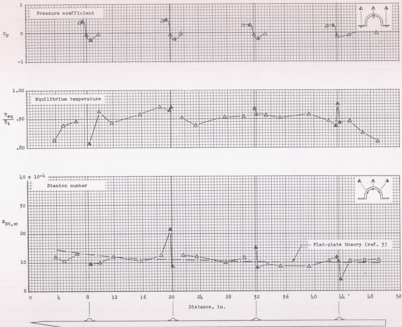
Figure 7.- Distribution of heat-transfer parameters and pressures for plate II at M = 1.98 .
