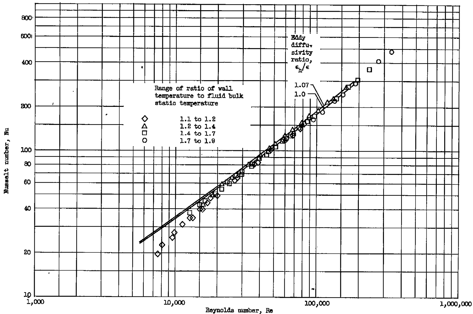
Figure 9. - Variation of Nusselt number with Reynolds number at various ratios of wall temperature to fluid bulk static temperature and several values of \epsilon_w/\epsilon . (Properties evaluated at film temperature.)
