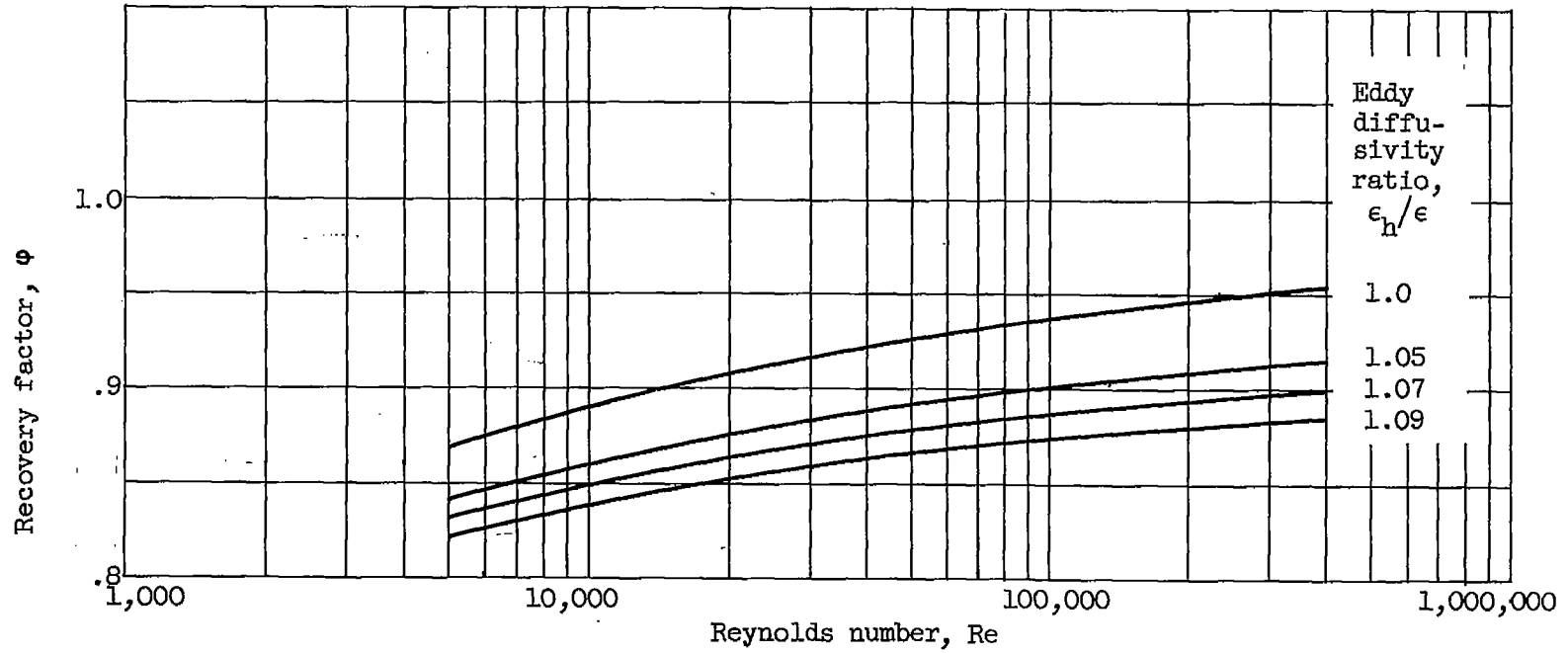
Figure 6. - Variation of recovery factor with Reynolds number for various eddy diffusivity ratios.
