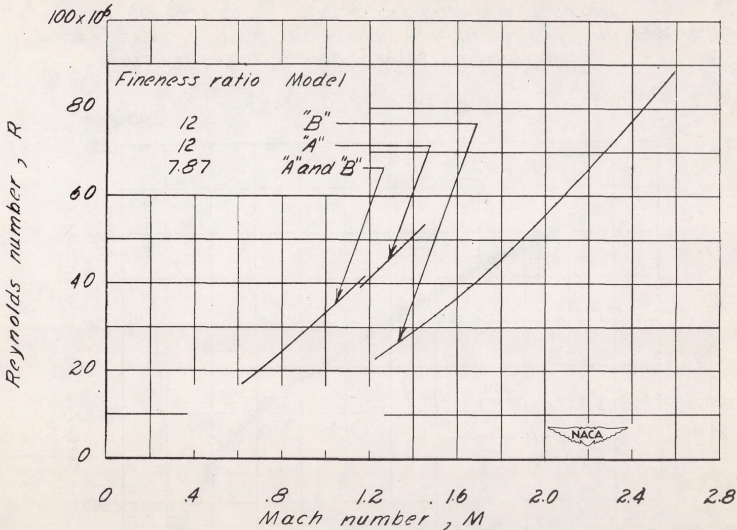
Figure 6.- Variation of Reynolds number with Mach number for both fineness-ratio configurations.
