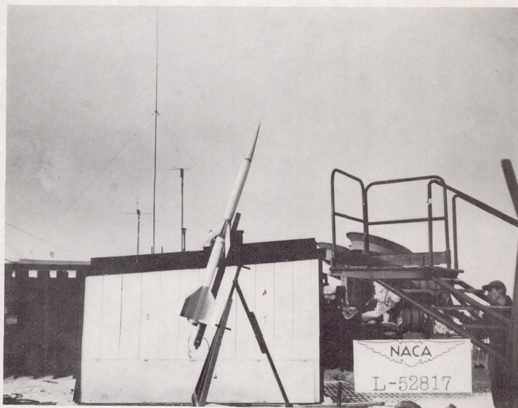
Figure 5.- View of fineness-ratio 12 "B" model in launcher.
