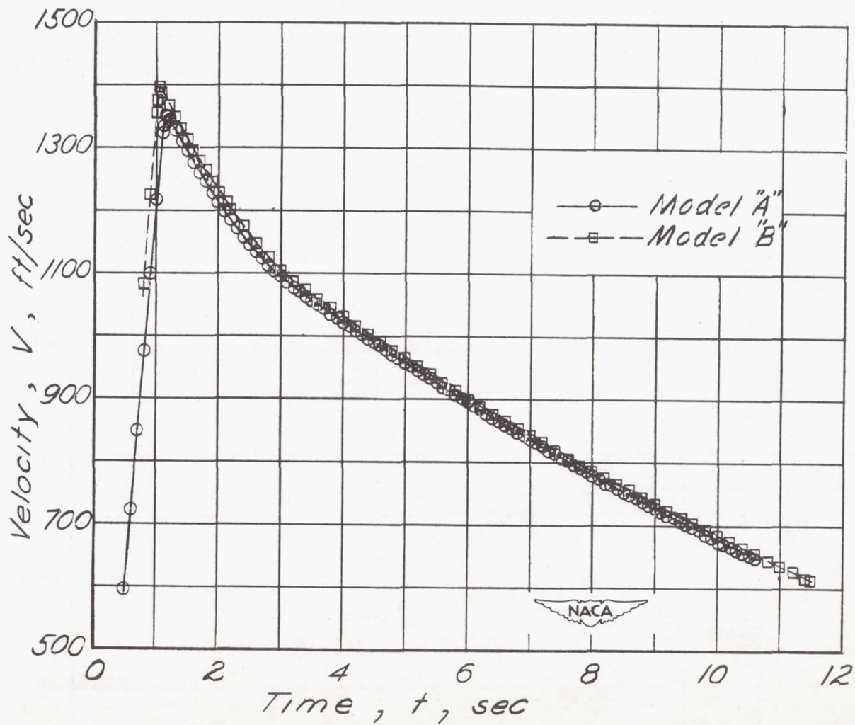
(a) Fineness-ratio 7.87 configuration. Figure 7. - Velocity-time relations for the two body fineness-ratio configurations investigated.
