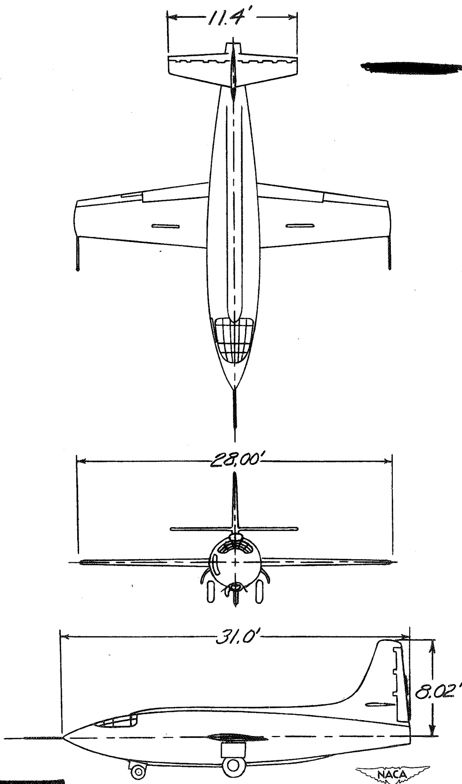
Figure 1.- Three-view drawing, X8-1 airplane.
