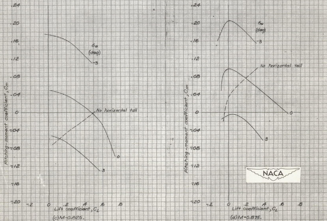
Figure 12.—Static longitudinal stability characteristics of the complete model with various elevator deflections, and the model without horizontal tail, I_x = 0^\circ .
