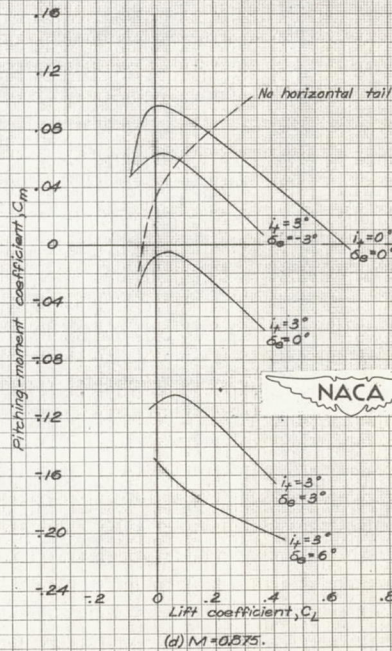
Figure 13.—Static longitudinal stability characteristics of the complete model with various stabilizer settings and elevator deflections, and the model without horizontal tail.
