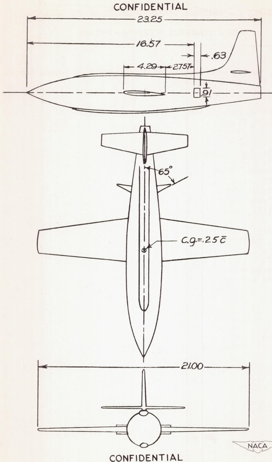
Figure 1.— Three-view drawing of a 1/16-scale model of the Bell XS-1 airplane with speed-reduction brakes as tested in the Langley 8-foot high-speed tunnel. All dimensions in inches.
