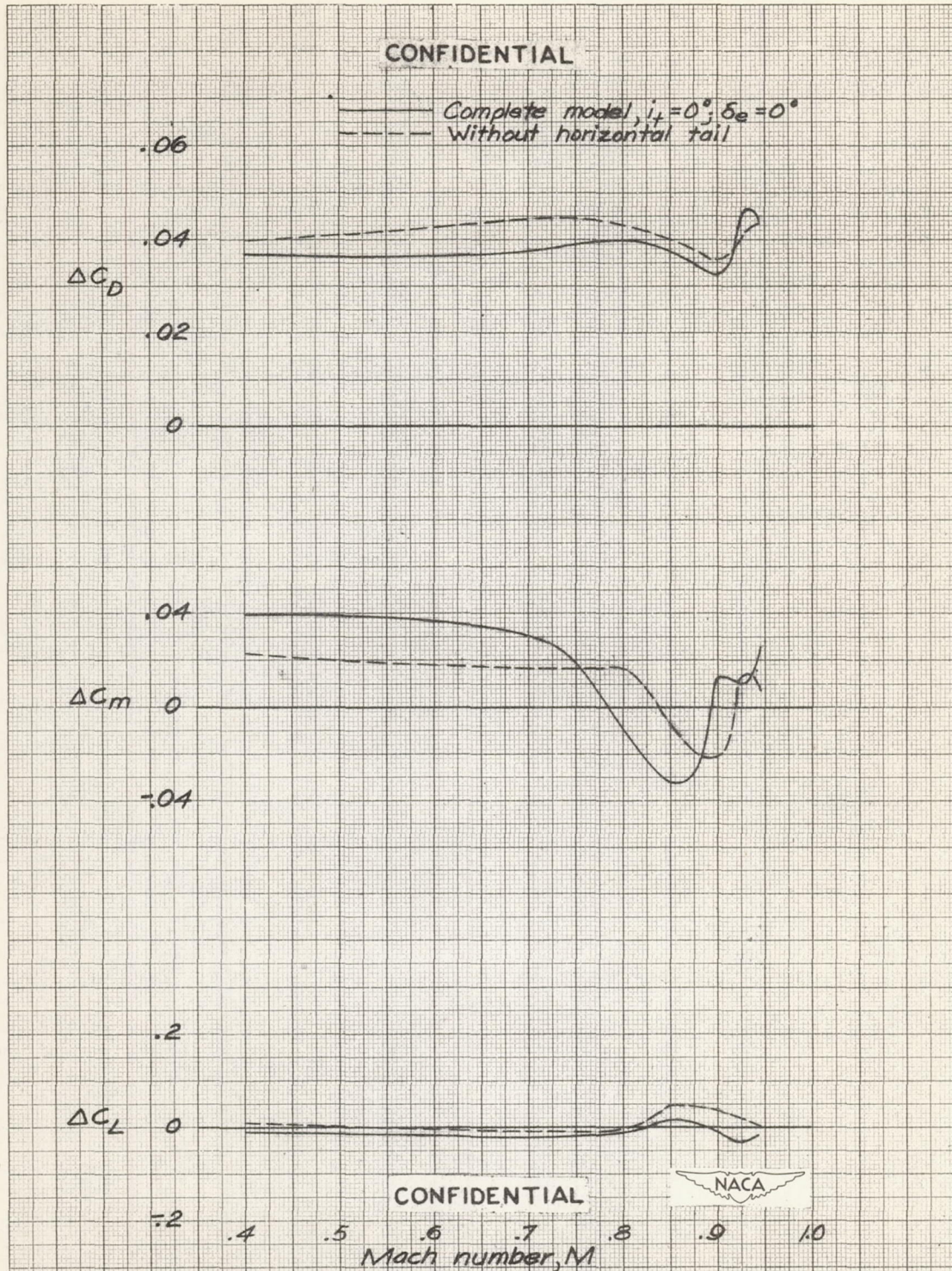
Figure 9.-Variation of incremental lift, drag, and pitching-moment coefficients with Mach number for the speed-reduction brakes on the model with and without horizontal tail. \alpha = -2^\circ
