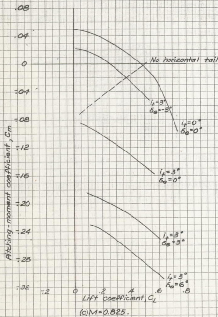
Figure 13.—Static longitudinal stability characteristics of the complete model with various stabilizer settings and elevator deflections, and the model without horizontal tail.
