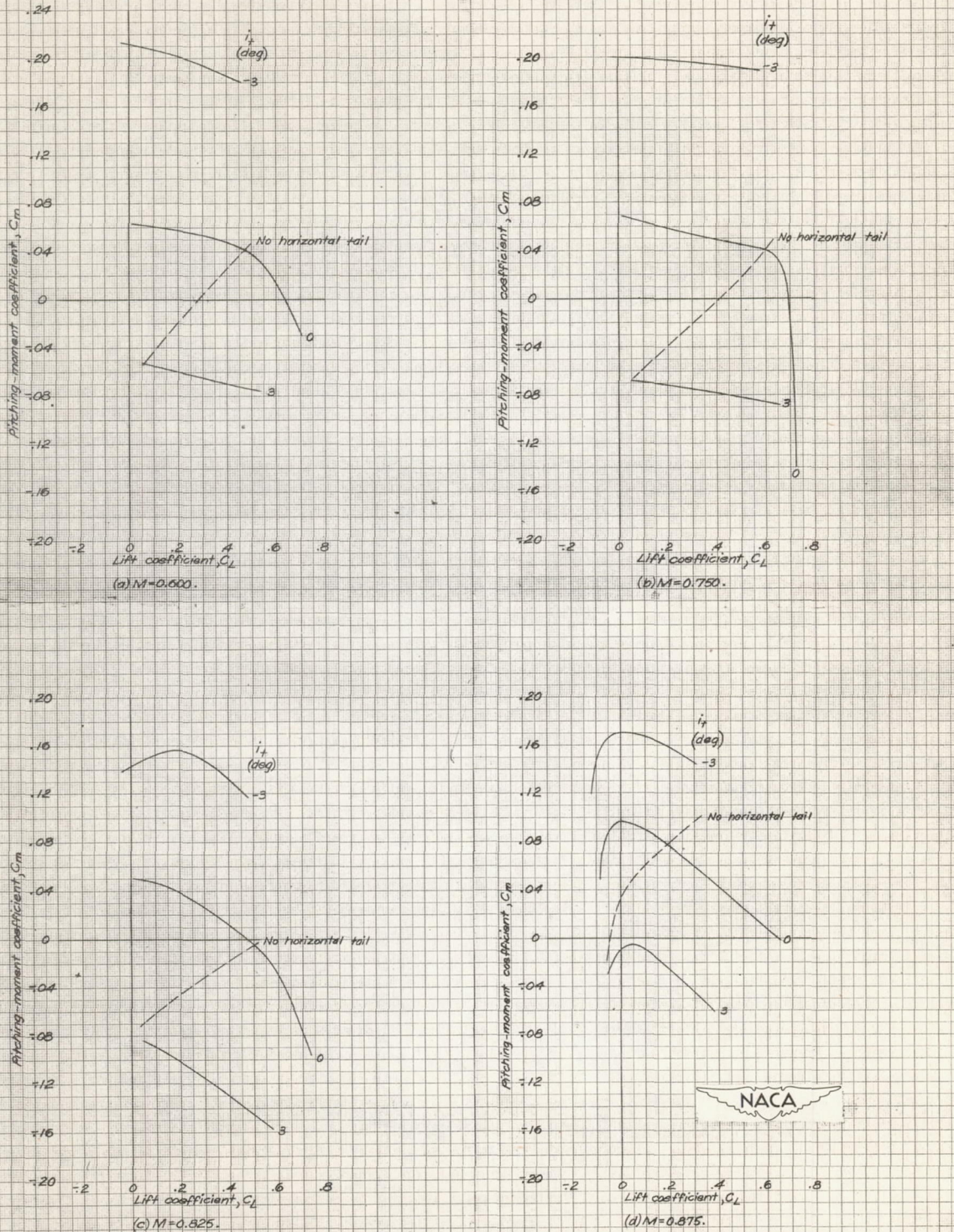
Figure 11.-Static longitudinal stability characteristics of the complete model with various stabilizer settings, and the model without horizontal tail. \zeta_{\theta} = 0^\circ .
