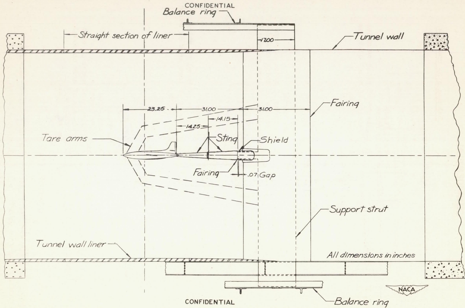
Figure 2.— X5-1 model on sting support in the Langley 8-foot high-speed tunnel.
