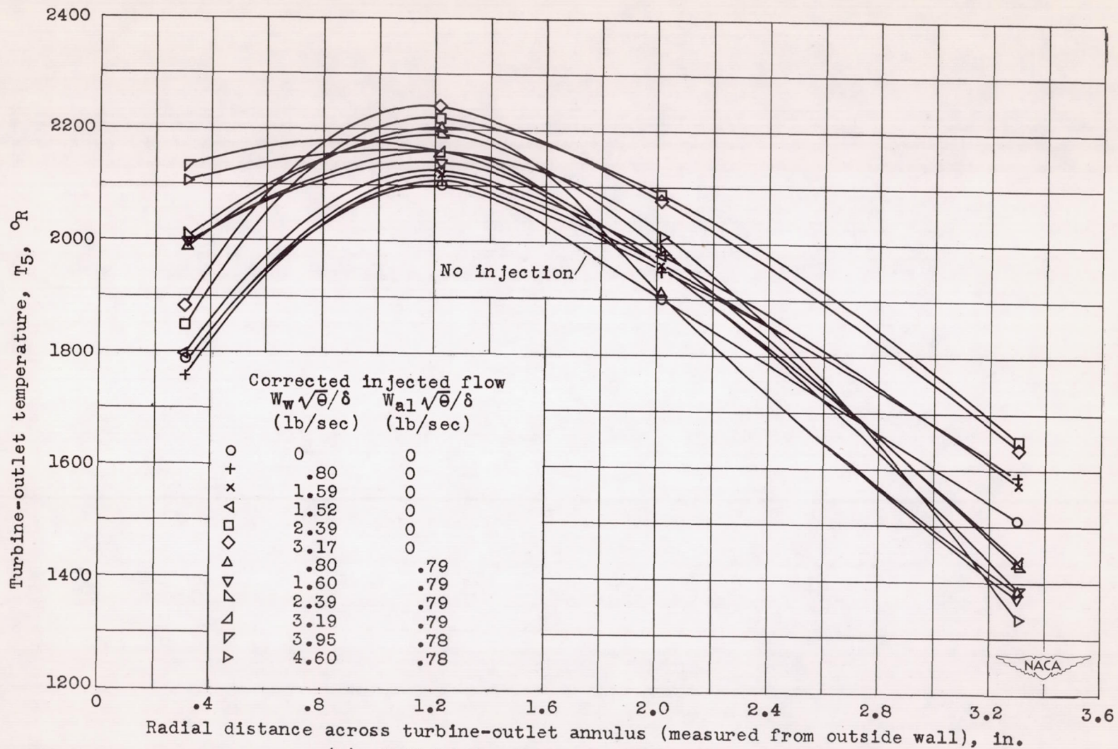
(b) Radial distribution downstream of burner.
