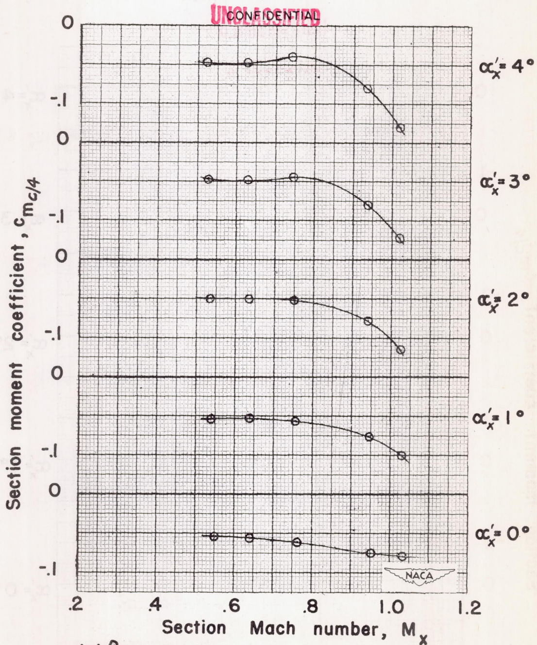
Figure 21. — Variation of section moment coefficient with section Mach number for several angles of attack. Radial station = 0.90.
