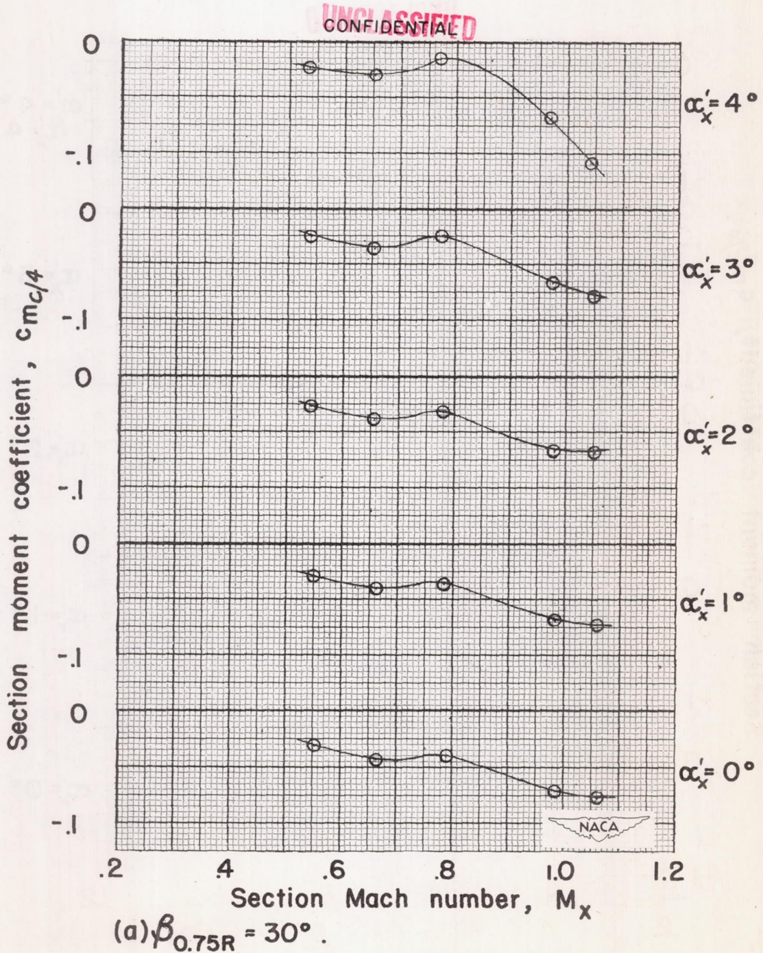
Figure 22.— Variation of section moment coefficient with section Mach number for several angles of attack. Radial station = 0.95.
