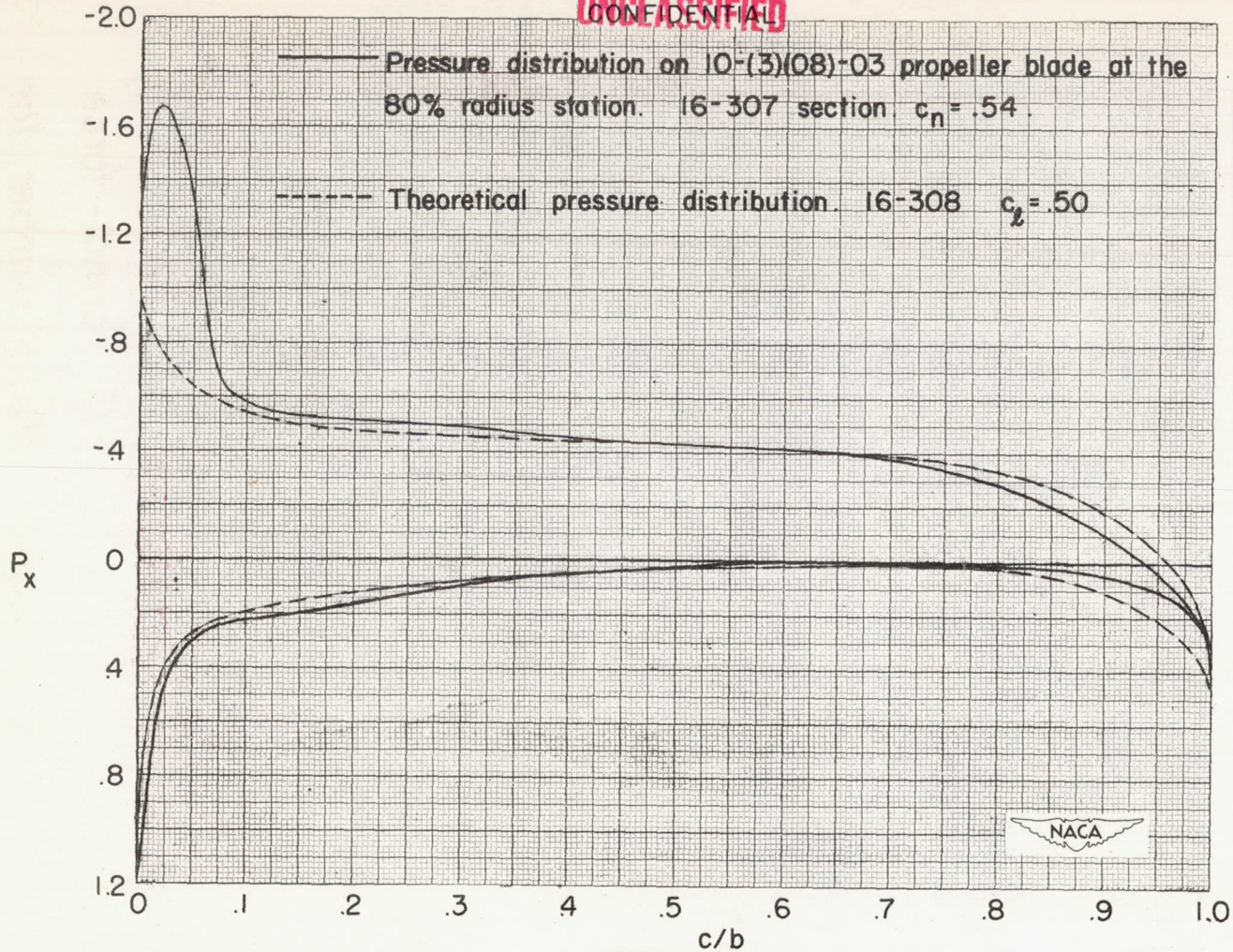
Figure 4. — Comparison of experimental pressure distribution on rotating propeller blade section with theoretical pressure distribution.
