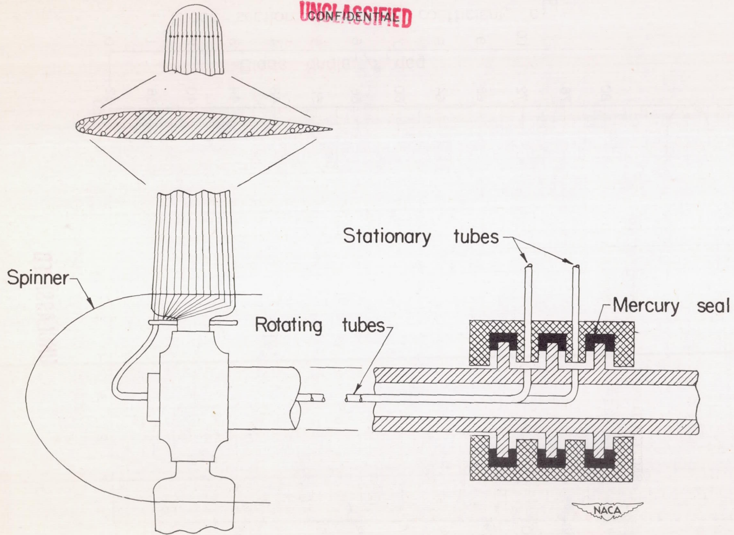
Figure 1. — Schematic diagram showing method of measuring pressures.
