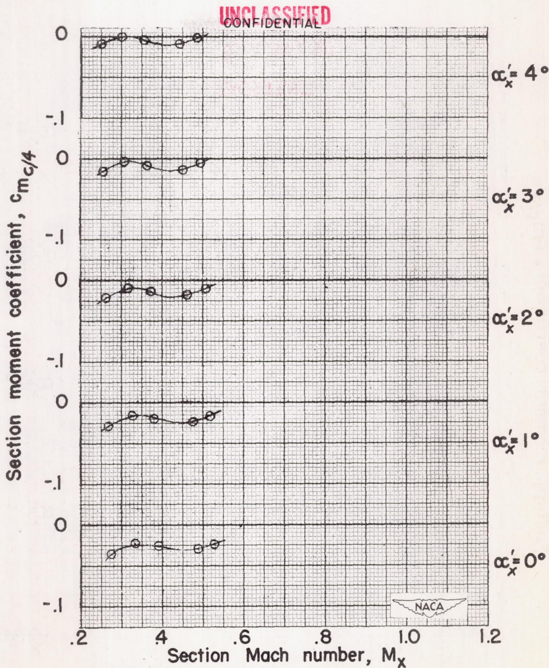
Figure 14.— Variation of section moment coefficient with section Mach number for several angles of attack. Radial station = 0.30.
