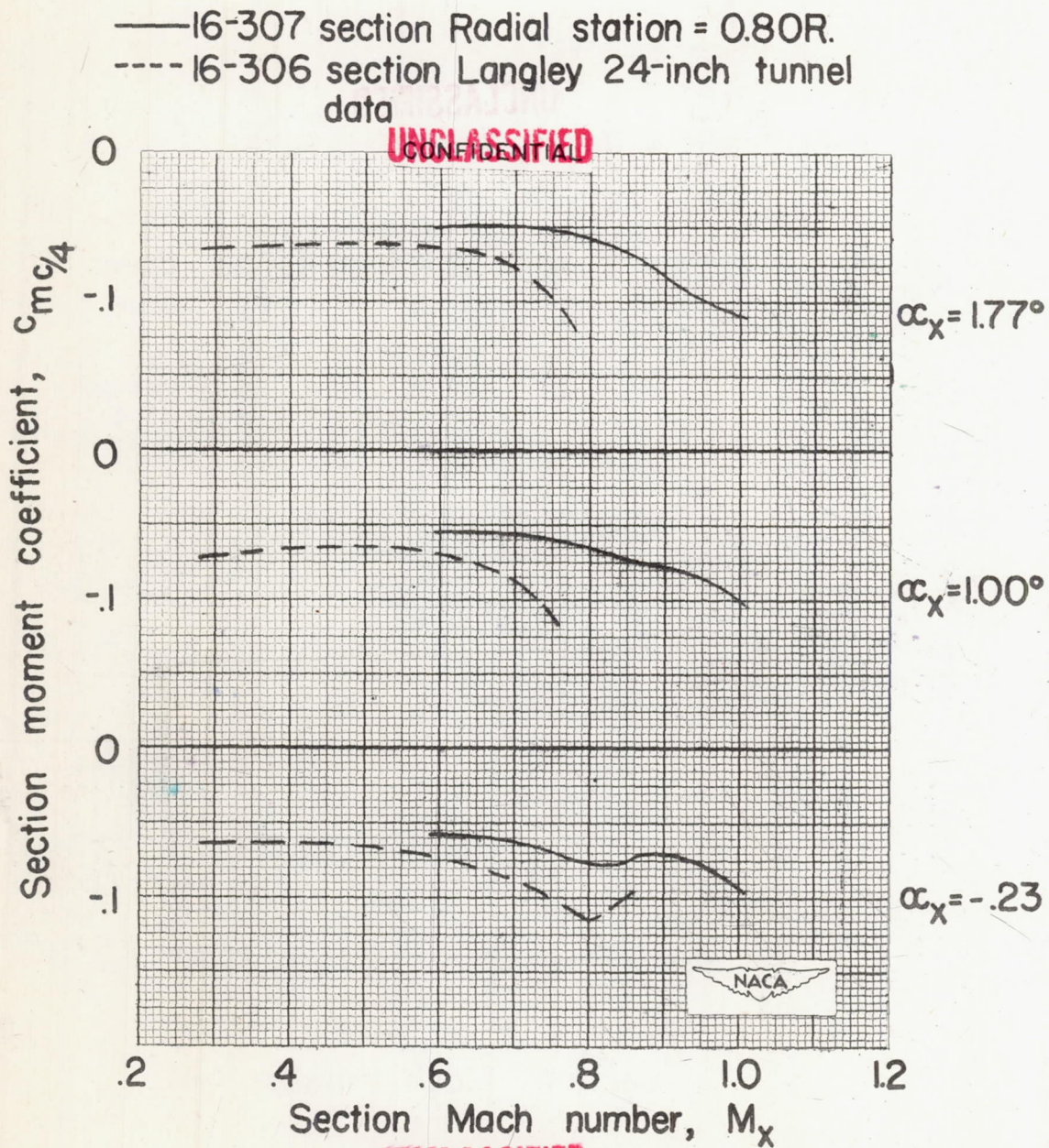
Figure 24.— Comparison of section moment coefficient obtained in propeller tests with the moment coefficient obtained in tunnel tests of an infinite-aspect-ratio model.
