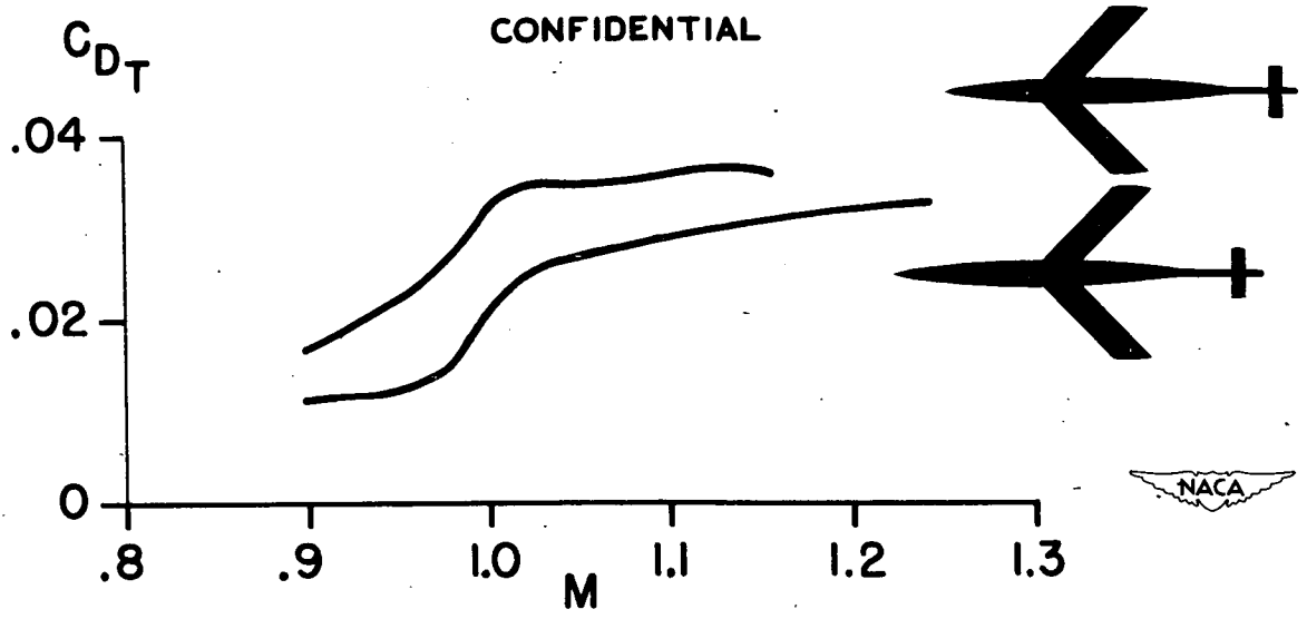
Figure 13.- Effect on drag of wing-body-tail combination through transonic range due to fore-and-aft position of 45° swept wing.
