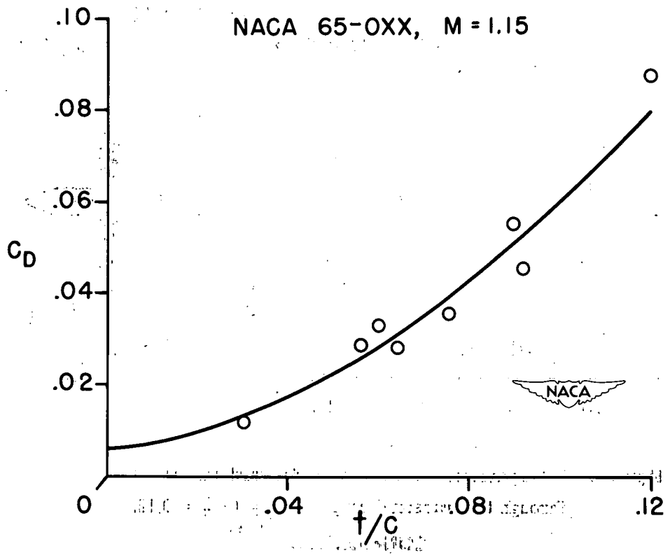
Figure 4.- Variation of drag coefficient of unswept wings with thickness ratio. M = 1.15 ; C_L = 0 .
