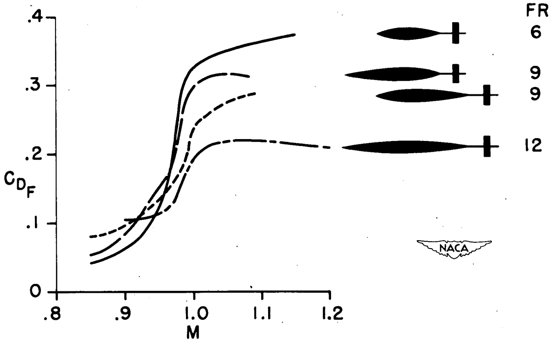
Figure 9.- Effects of fineness ratio and thickness distribution on the drag of bodies of revolution at transonic speeds.
