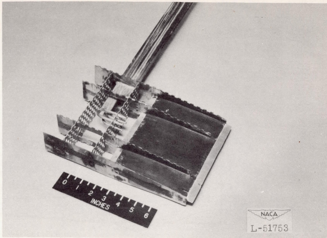
Figure 2.- Construction details of two-dimensional diffuser.
