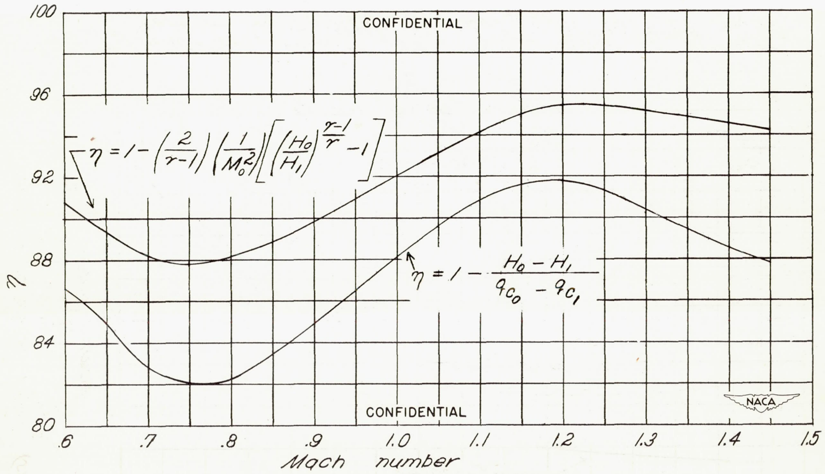
Figure 9. - Diffuser efficiency against flight Mach number from test of two-dimensional diffuser.
