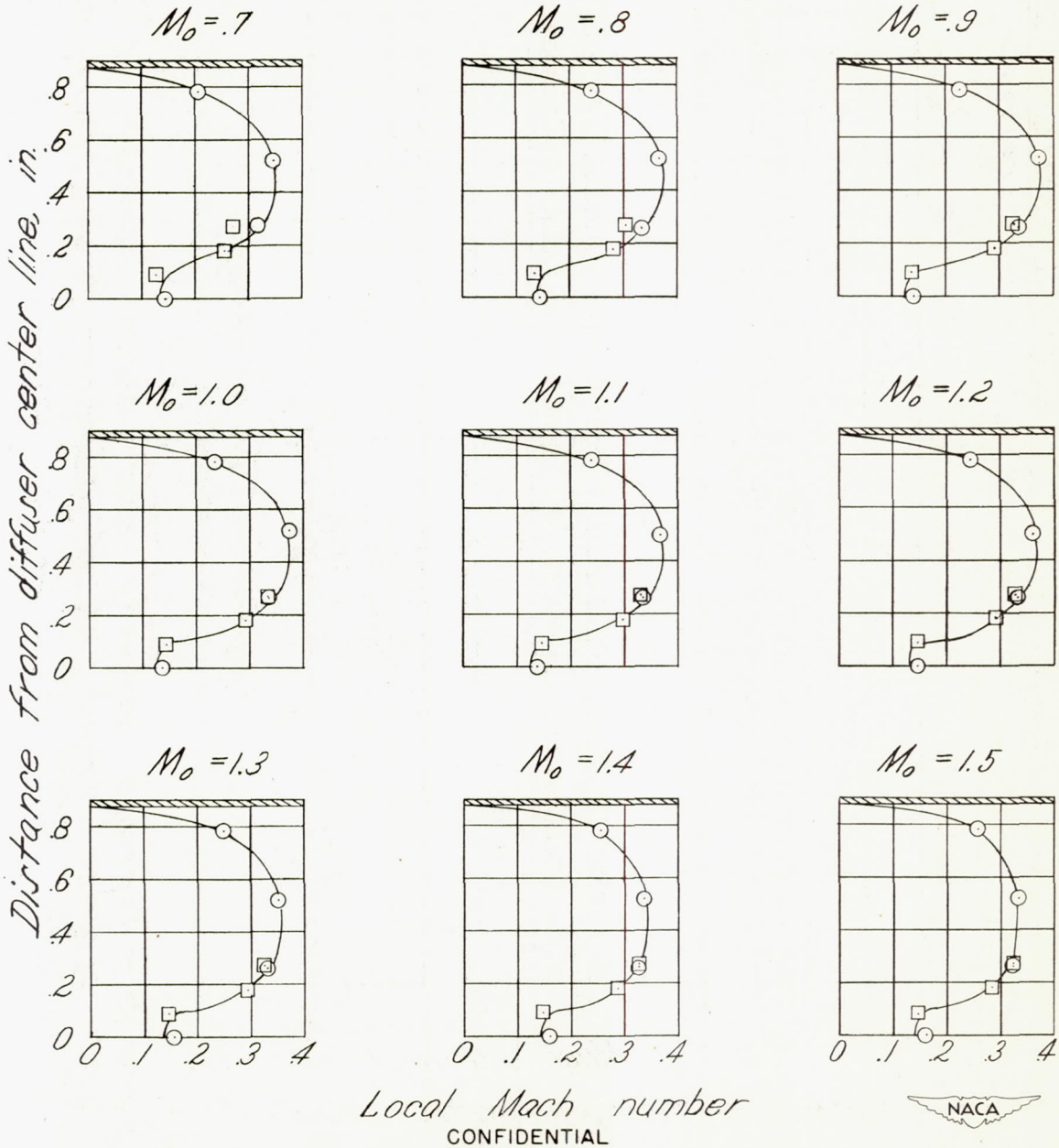
Figure 7. - Velocity distribution at diffuser exit from test of two-dimensional diffuser.
