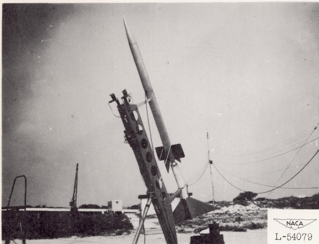
Figure 4.- Diffuser test vehicle assembled on launching rack. CONFIDENTIAL
