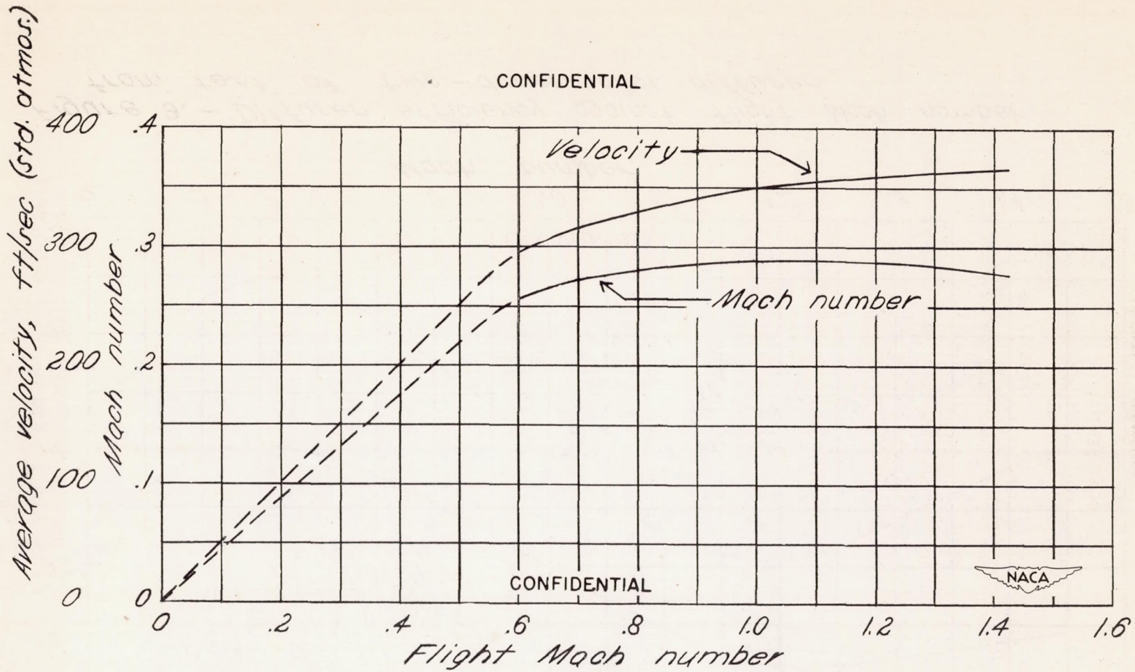
Figure 8. - Average velocity and Mach number at diffuser exit against flight Mach number from test of two-dimensional diffuser.
