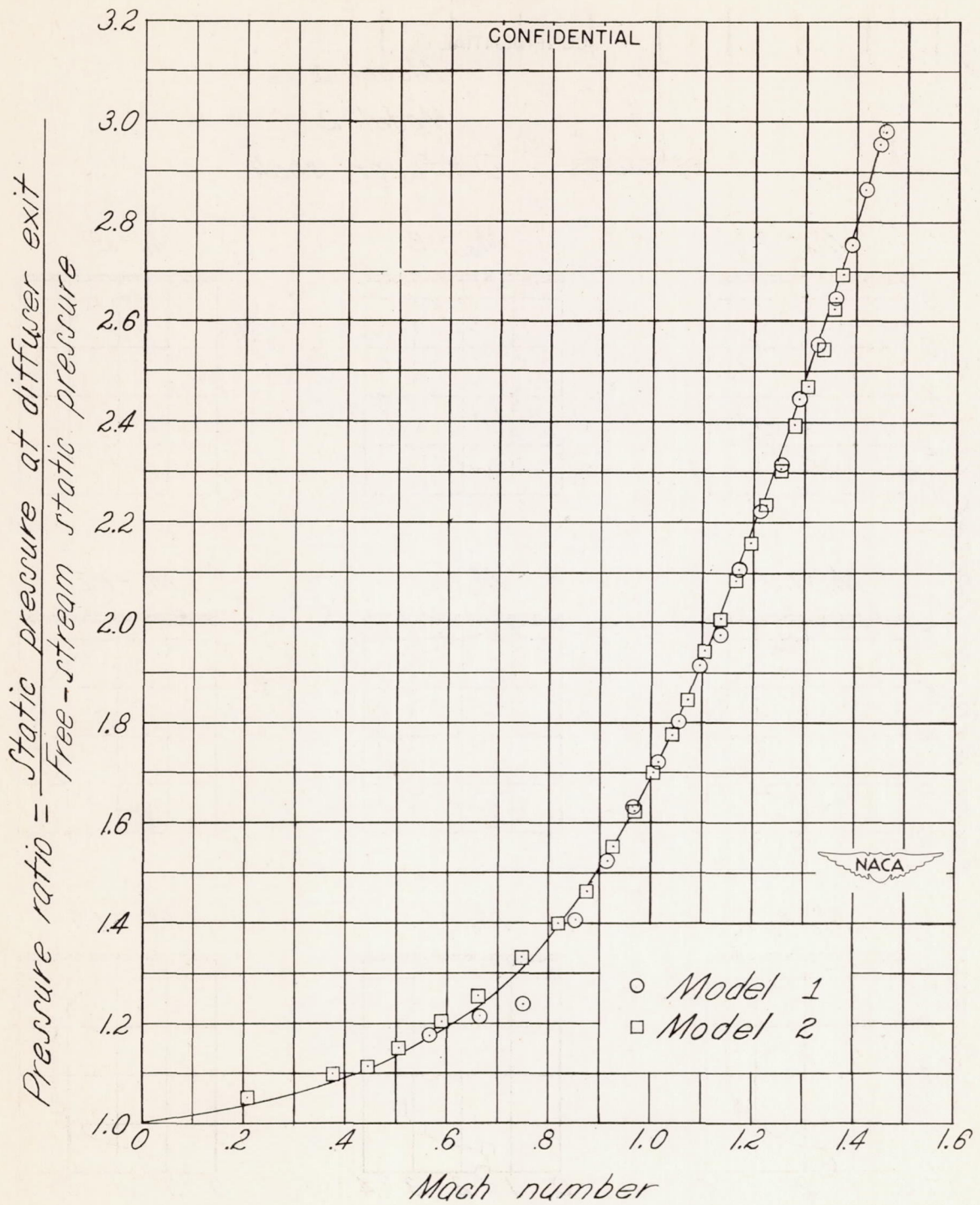
Figure 6. - Pressure ratio against flight Mach number from test of two-dimensional diffuser.
