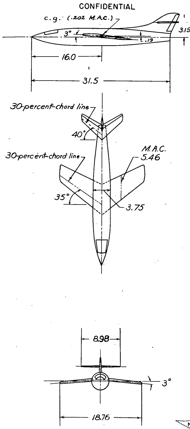
Figure 3.- Drawing of the \frac{1}{16} - scale model of the D-558-2 as tested in the Langley 8-foot high-speed tunnel. (All dimensions in inches)
