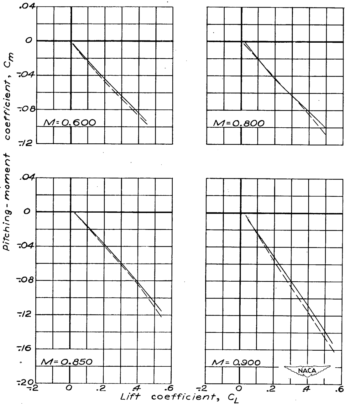
Figure 6. — Variation of pitching-moment coefficient with lift coefficient for various Mach numbers, for complete model and complete model with hydrofoil. i_f = 1.9^\circ ; \delta_e = 0^\circ .
