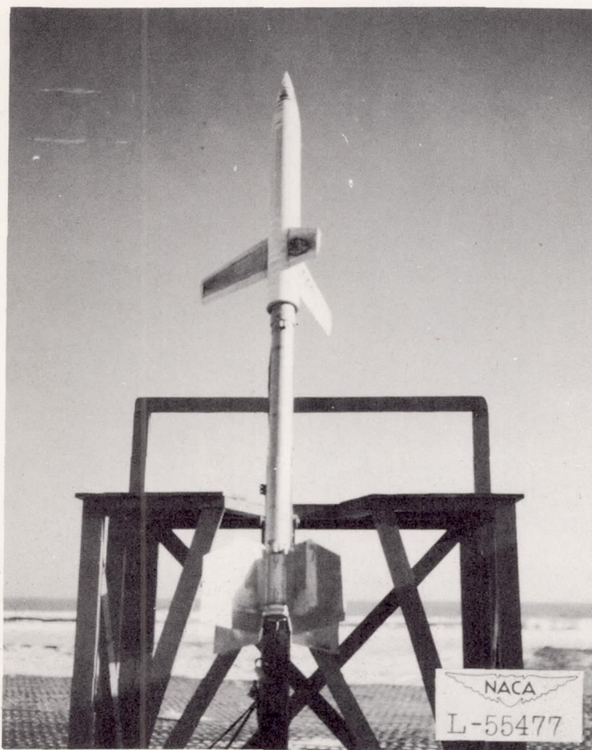
Figure 2.- Typical RM-5 test vehicle prior to launching.
