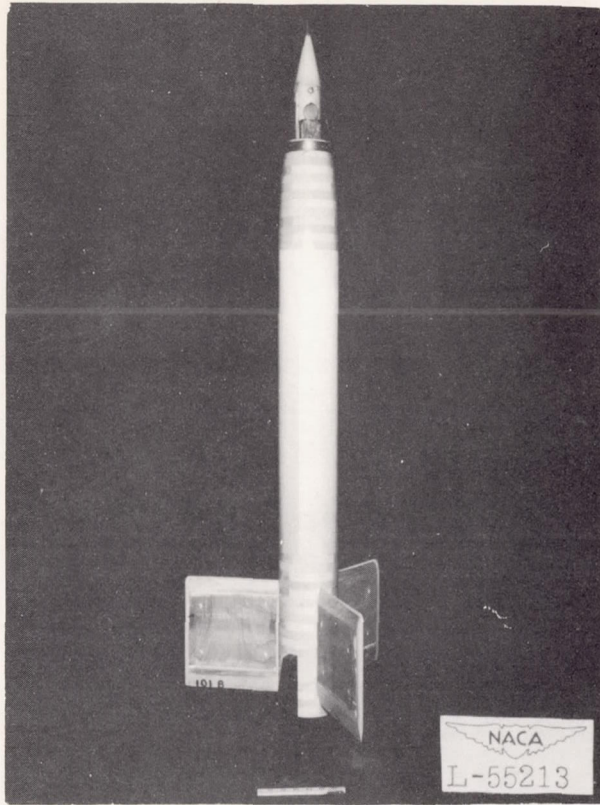
(a) Untapered.
