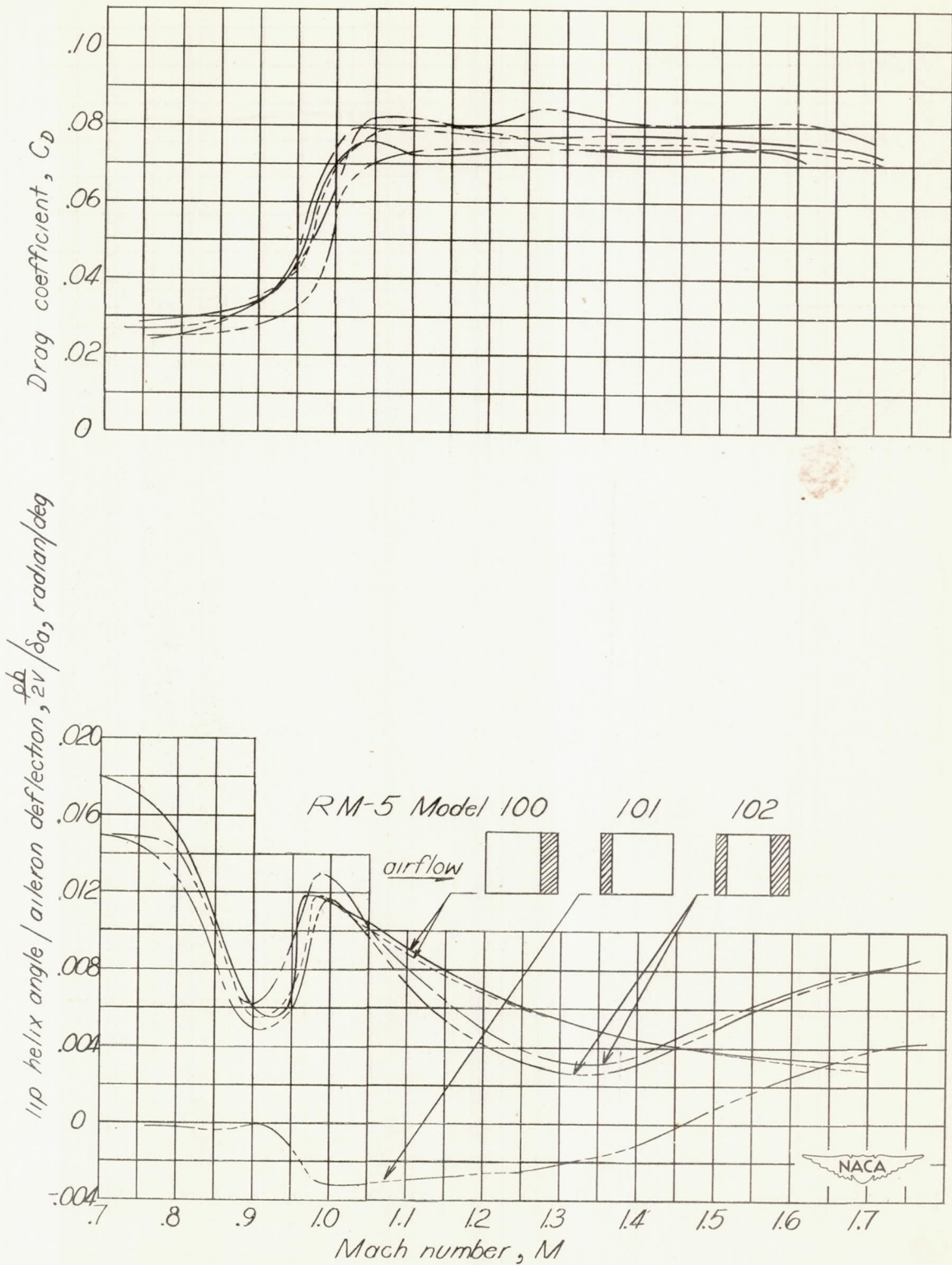
Figure 6.- Variation of tip helix angle and drag coefficient with Mach number.
