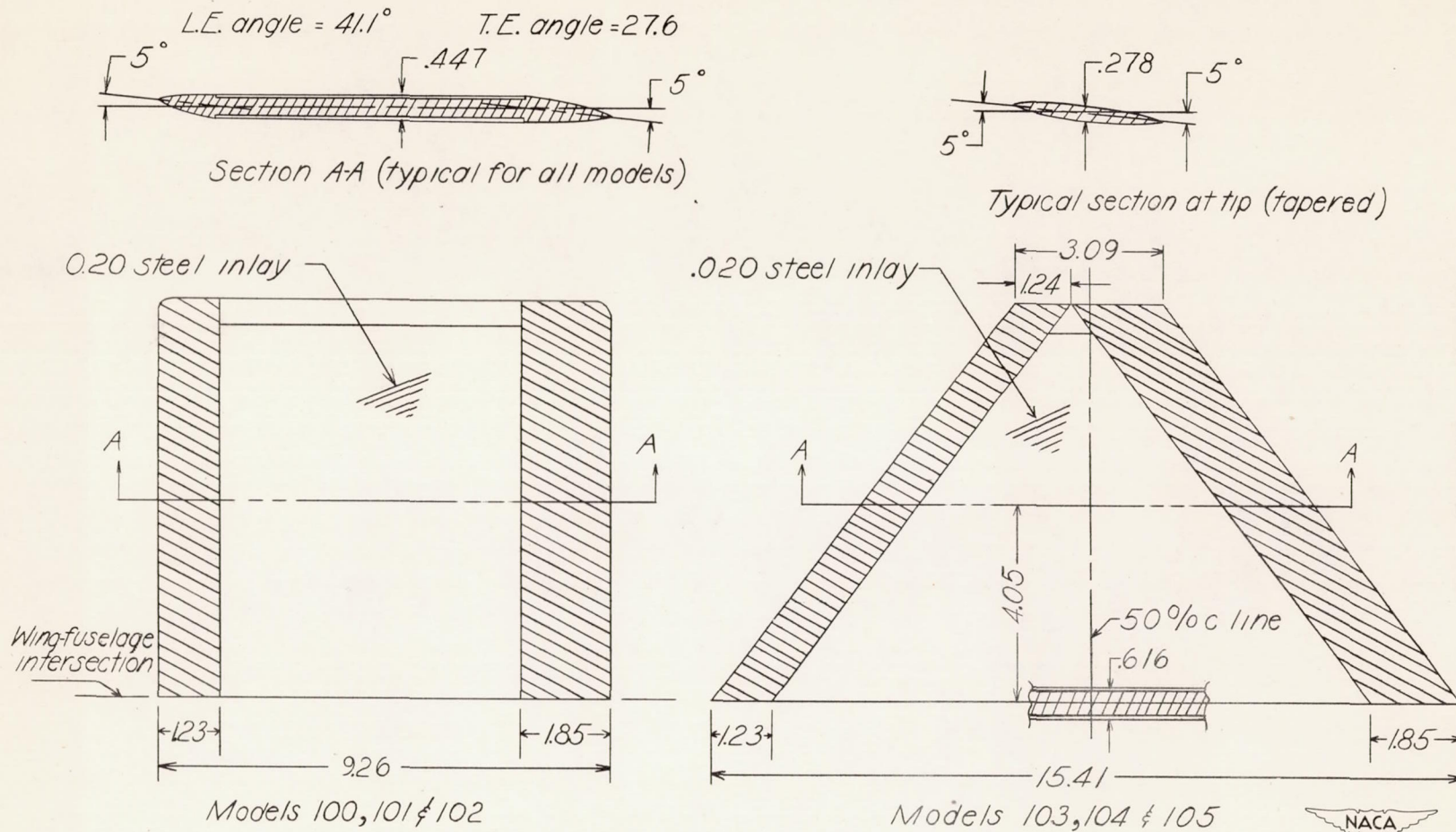
Figure 3.- Plan forms of RM-5 models tested.
