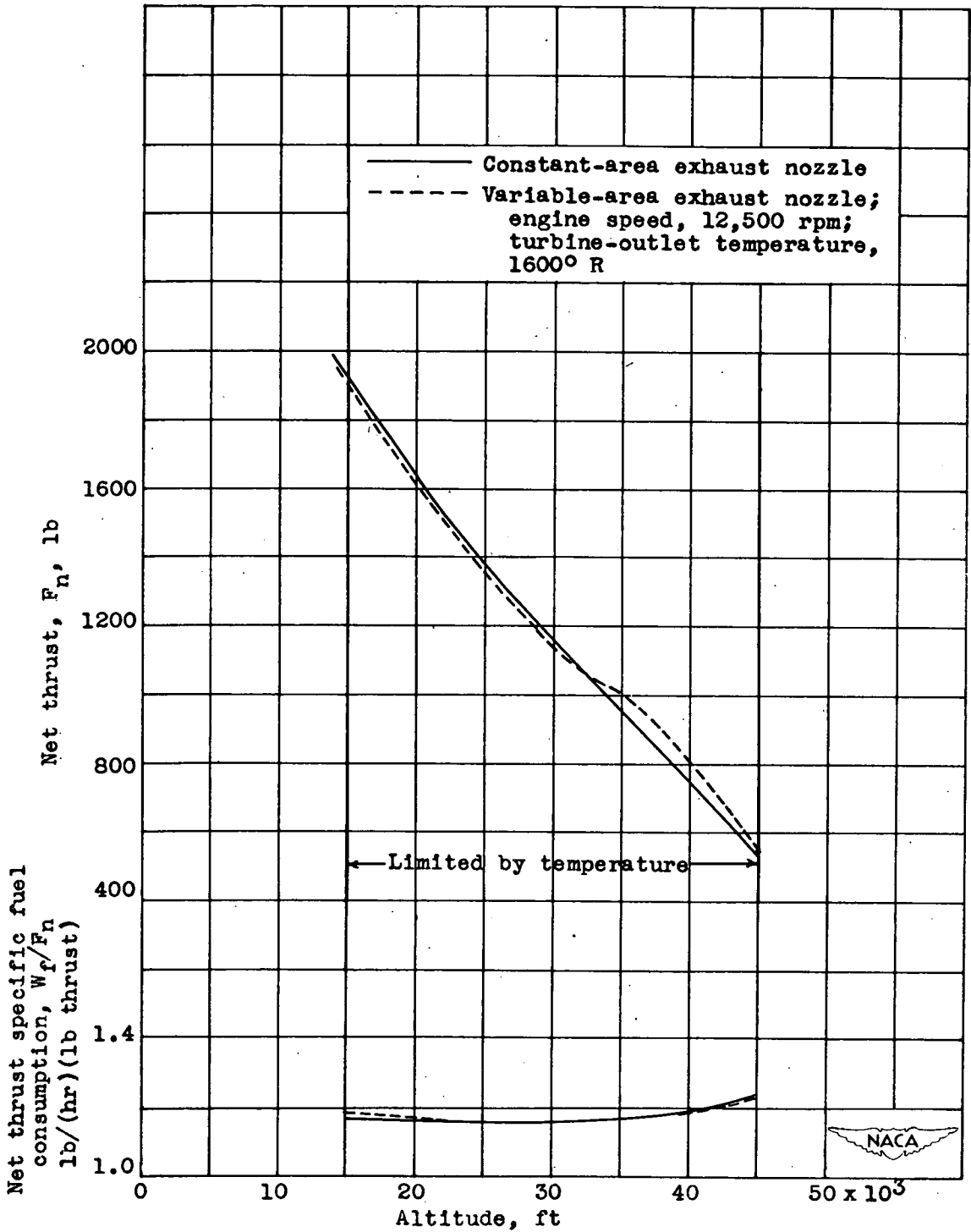
Figure 9. - Variation of net thrust and specific fuel consumption with altitude for assumed exhaust-nozzle efficiency of 100 percent. Approximate flight Mach number, 0.53.
