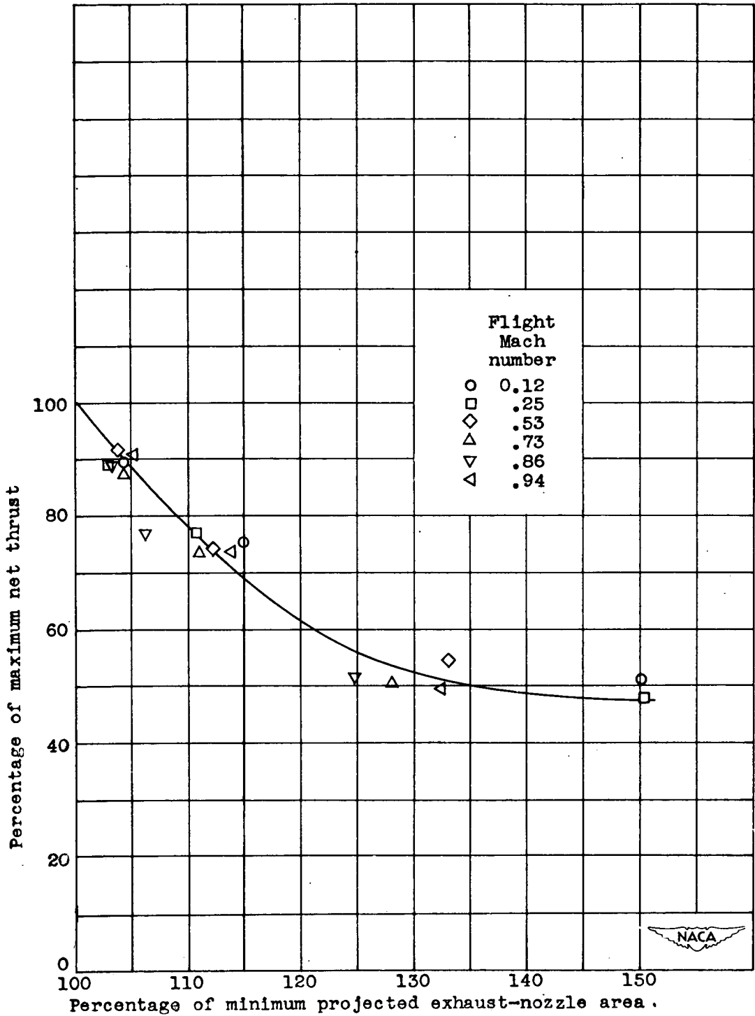
Figure 14. - Variation of net thrust with projected exhaust-nozzle area. Engine speed, 12,500 rpm; altitude, 25,000 feet.
