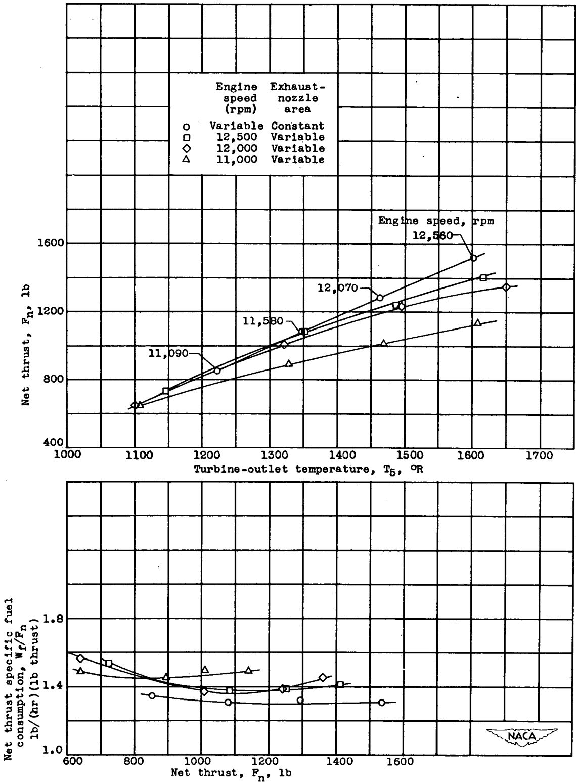
(b) Altitude, 25,000 feet; flight Mach number, 0.86.
