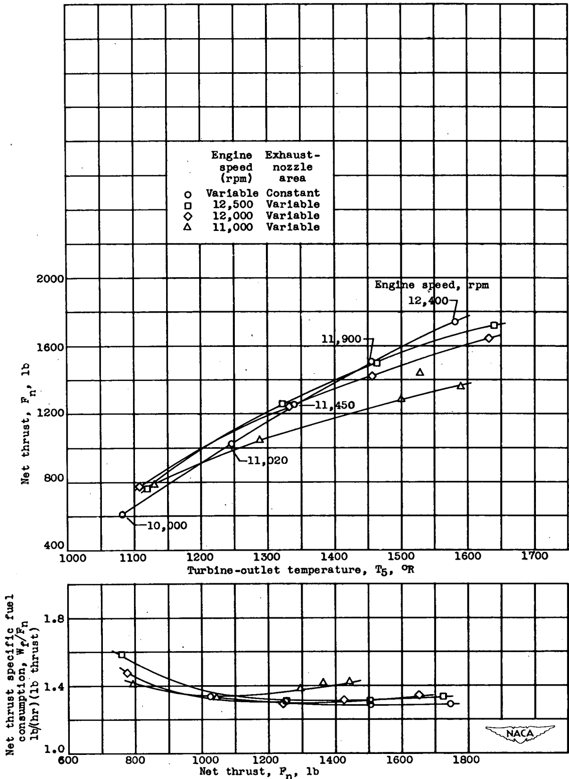
(c) Altitude, 15,000 feet; flight Mach number, 0.53.
