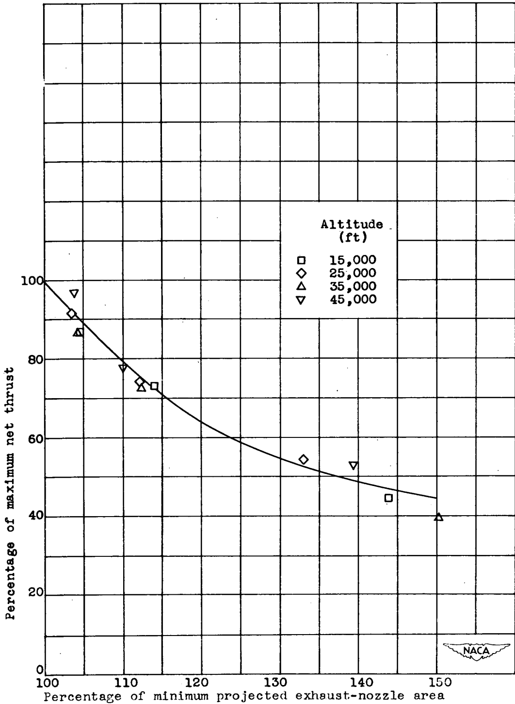
Figure 16. - Variation of net thrust with projected exhaust-nozzle area. Engine speed, 12,500 rpm; approximate flight Mach number, 0.53.
