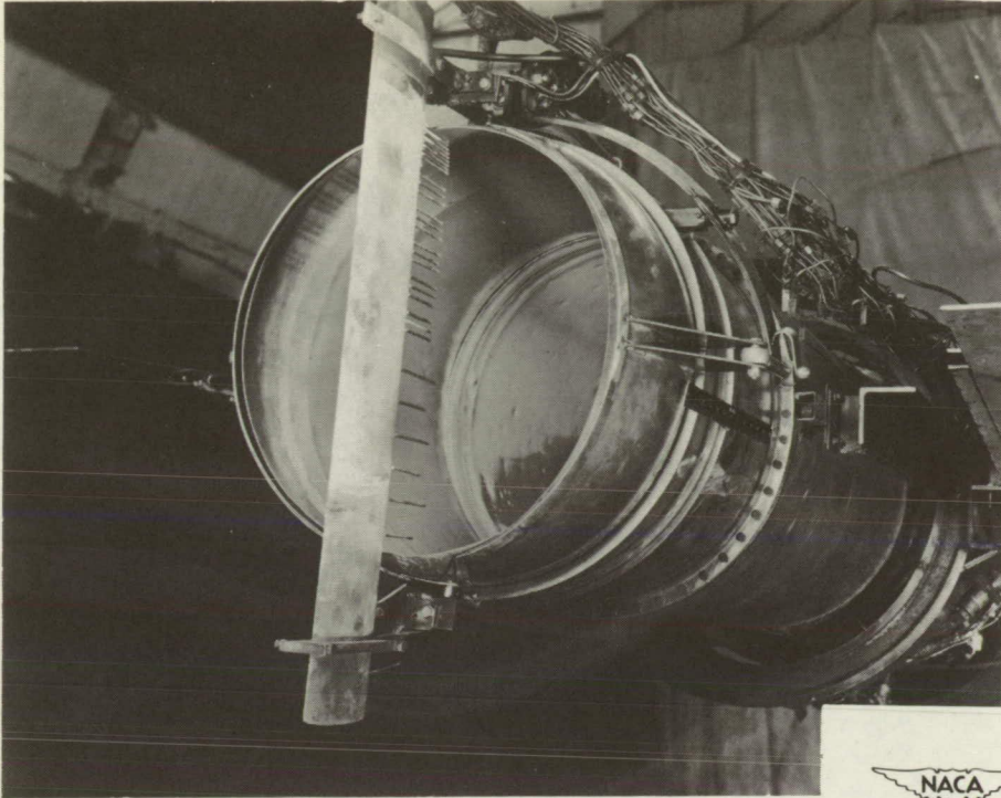
(a) Nozzle in open position.
