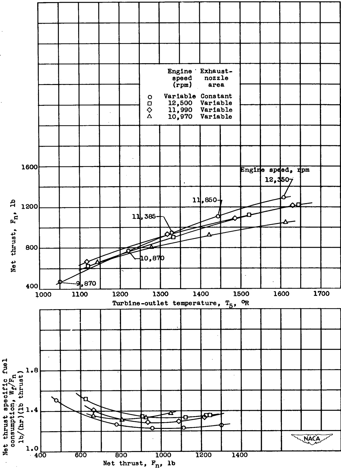
(a) Altitude, 25,000 feet; flight Mach number, 0.53.
