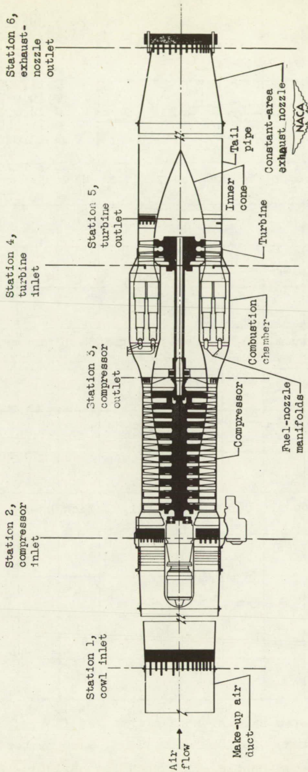
Figure 4. - Cross section of turbojet installation showing relation of component parts and measuring stations in engine.
