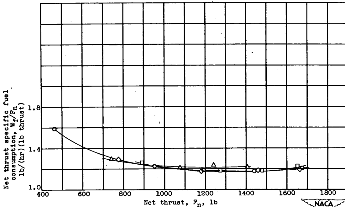
(b) Altitude, 25,000 feet; flight Mach number, 0.86.
