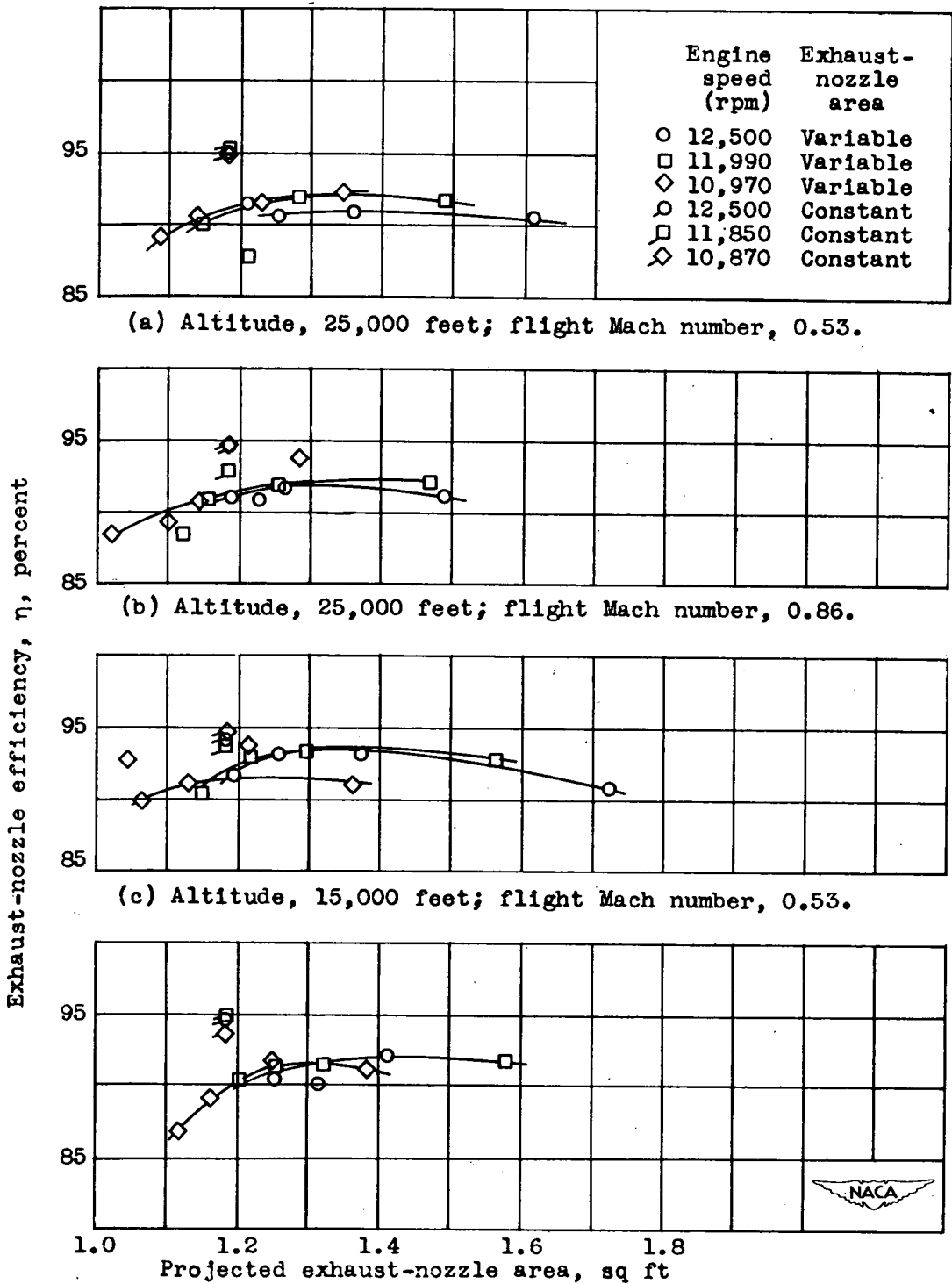
Figure 5. - Exhaust-nozzle efficiency for variable- and constant-area nozzles.
