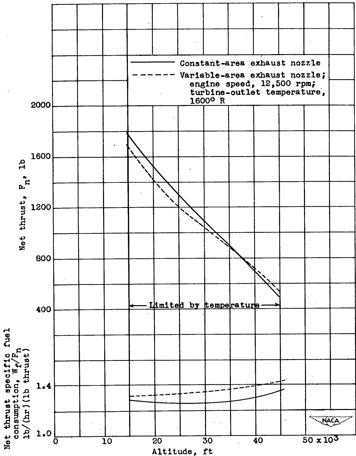
Figure 15. - Variation of net thrust and specific fuel consumption with altitude for actual exhaust-nozzle efficiencies. Approximate flight Mach number, 0.53.
