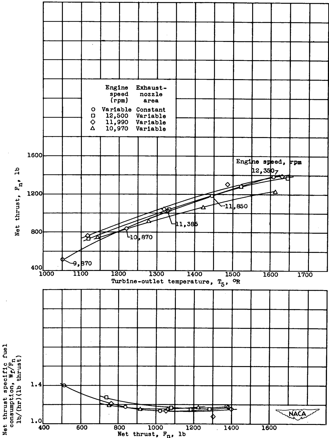
(a) Altitude, 25,000 feet; flight Mach number, 0.53.
