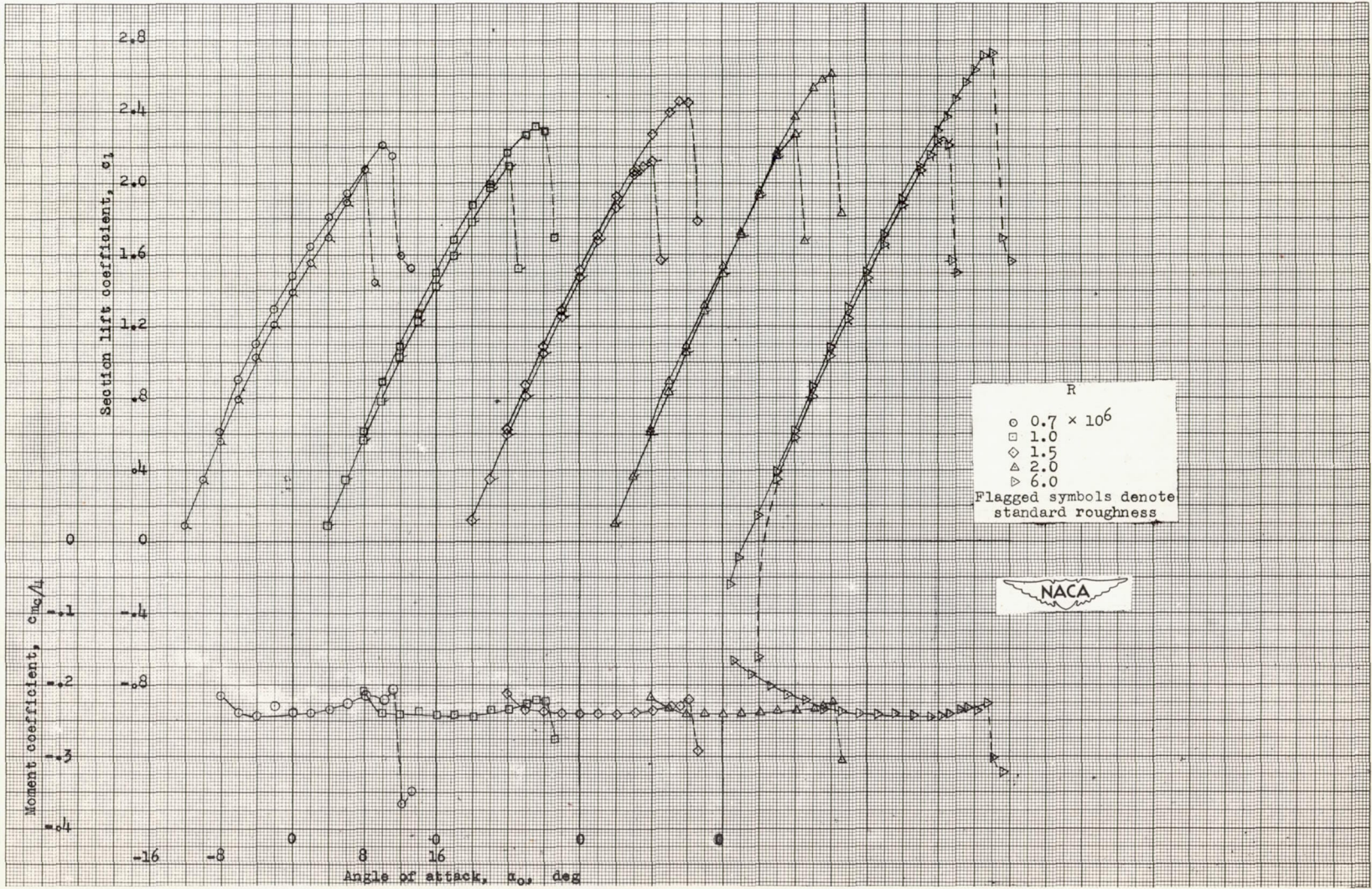
(b) Section lift and pitching-moment characteristics of the NACA 23012 airfoil section with a 0.20c simulated split flap deflected 60°.
