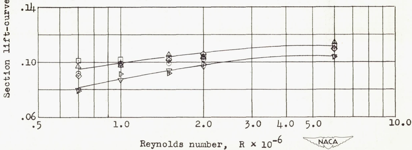
(b) Airfoils with standard leading-edge roughness .
