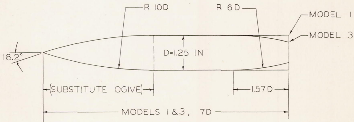
FIGURE 2.-MODEL DIMENSIONS
