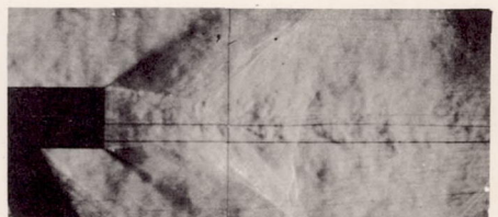
l/D = 5.2 \quad d/D = 0.3
