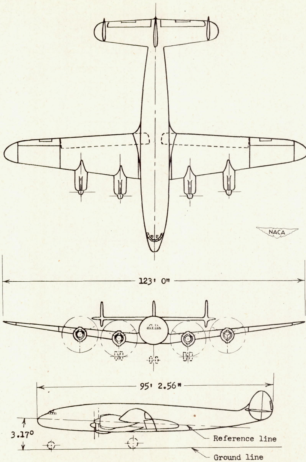
Figure 1.- Three-view drawing of the Lockheed Constellation airplane.
