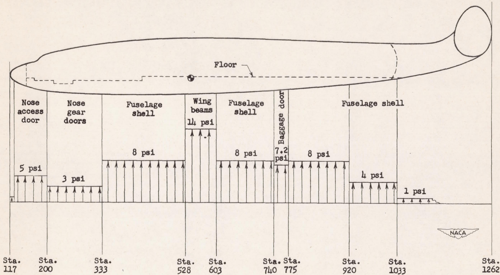
Figure 3.- Estimated strength of fuselage below floor.
