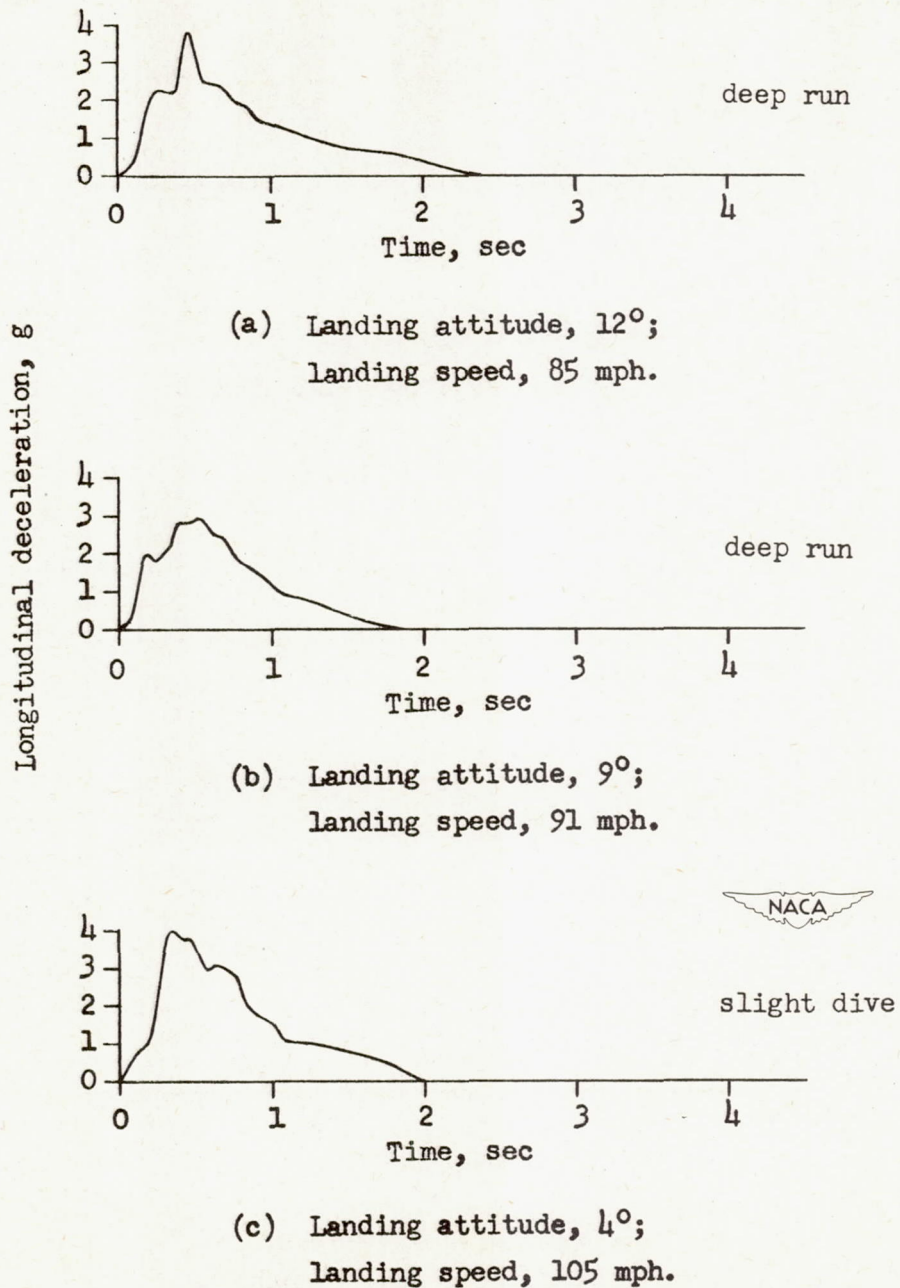
Figure 9.- Longitudinal decelerations with scale-strength bottom installed and flaps full down. All values are full scale.
