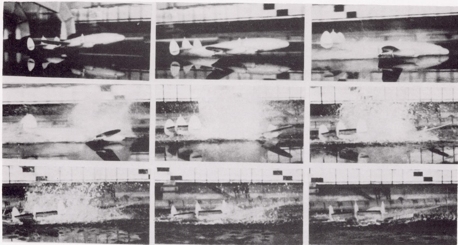
(b) Landing attitude, 9^\circ ; deep run.
