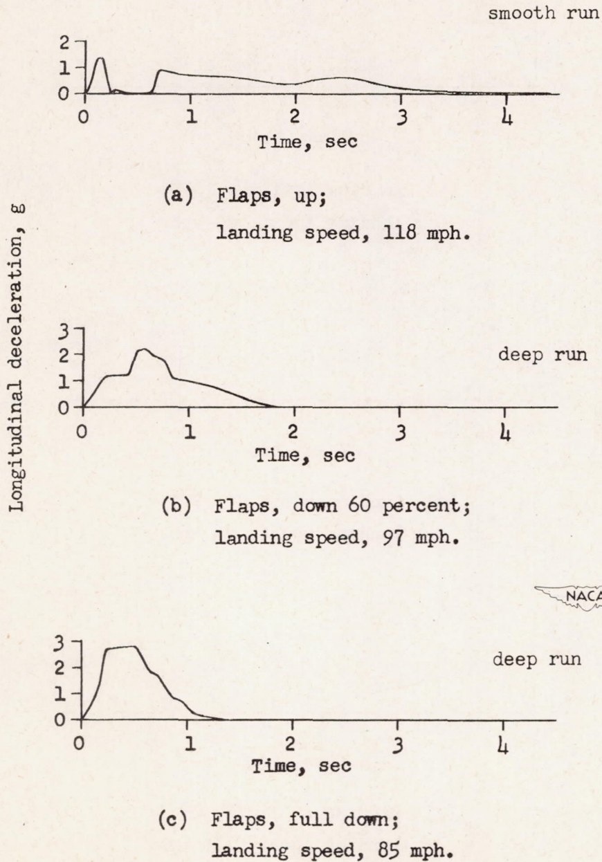
Figure 8.- Longitudinal decelerations at 12° landing attitude with no damage simulated. All values are full scale.
