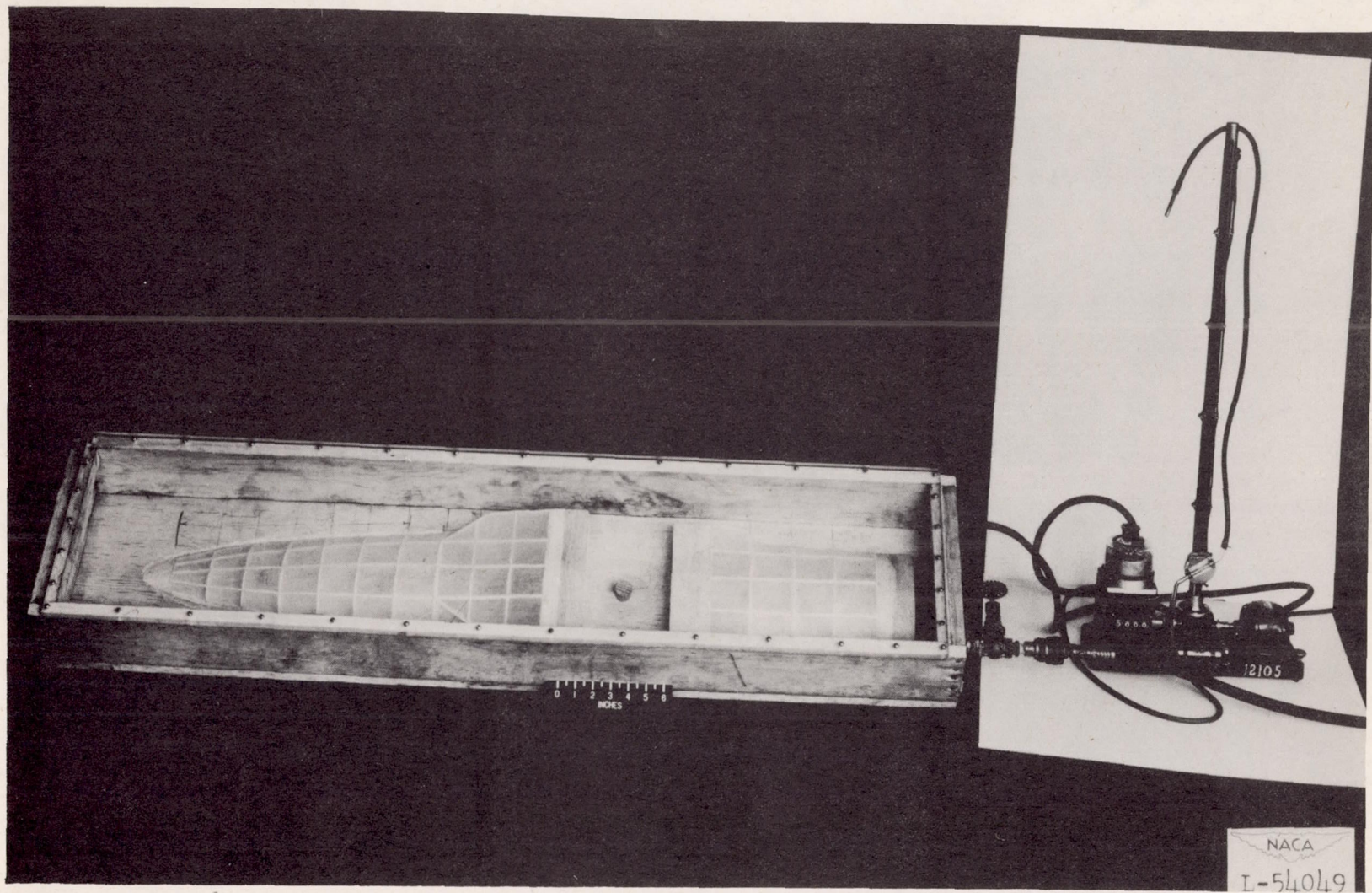
Figure 5.- Scale-strength bottom in testing apparatus.
