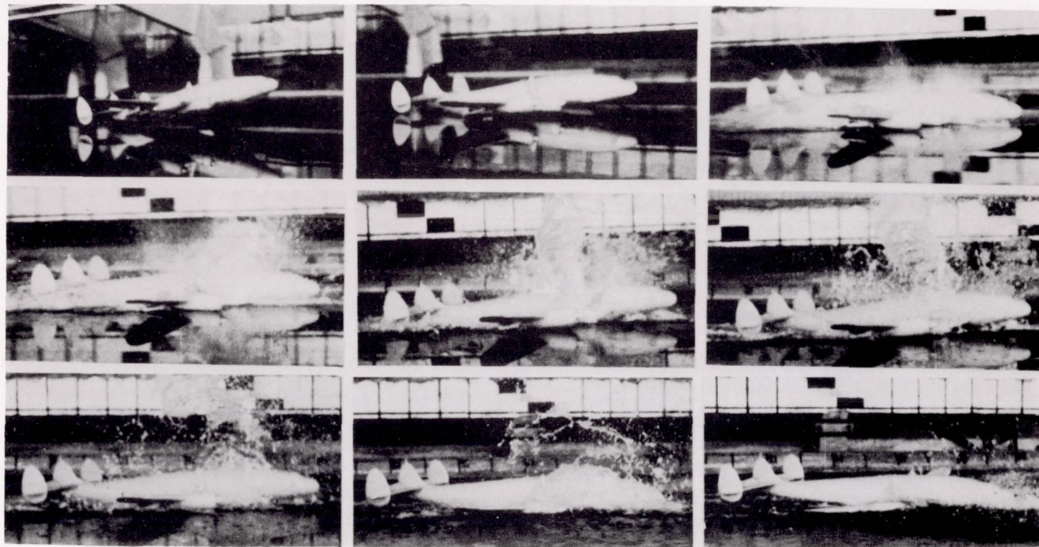
(a) Landing attitude, 12^\circ ; smooth run.
