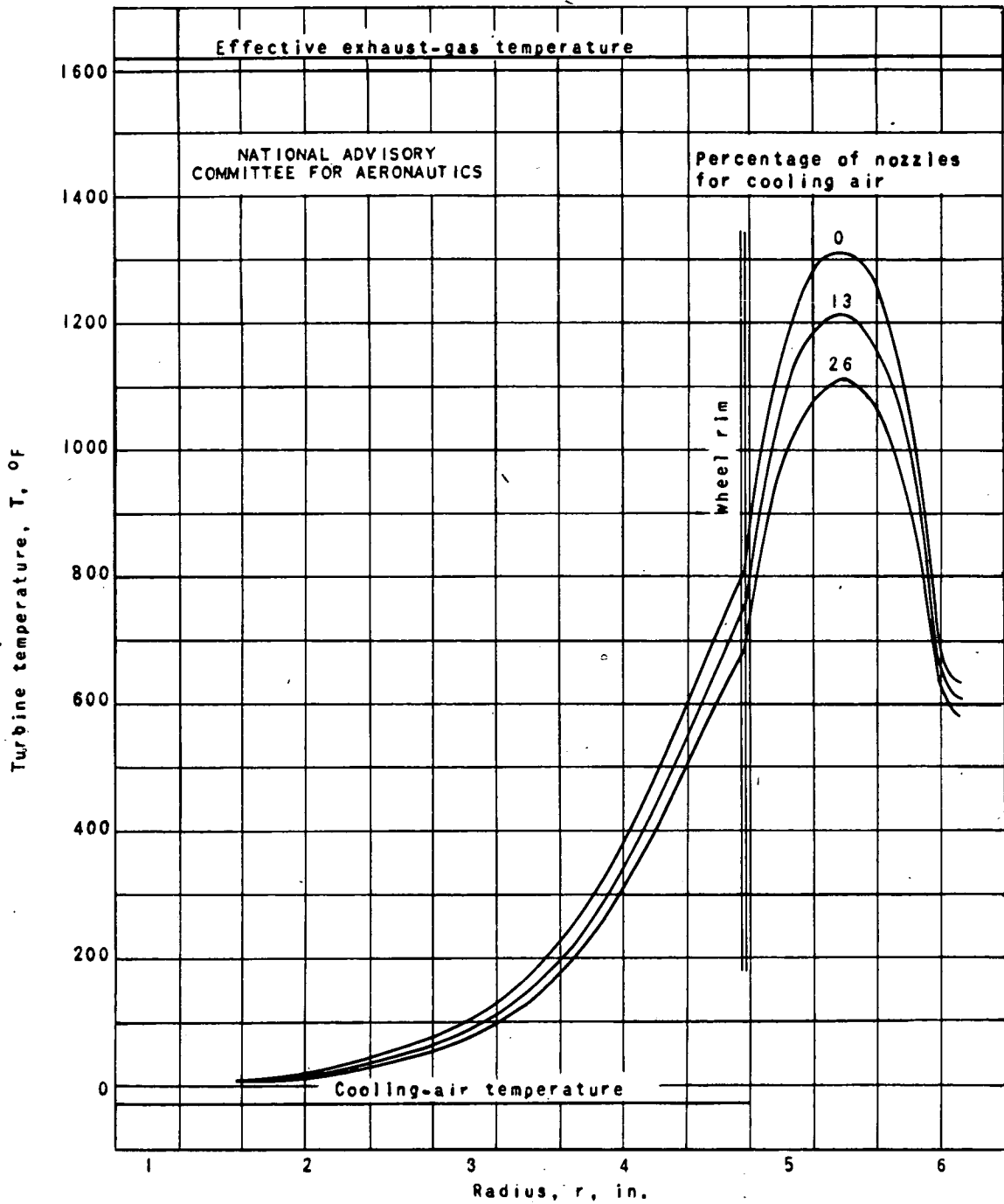
Figure 5. - Temperature distribution through turbine with partial admission of cooling air and with fins. Exhaust-gas temperature, 2000° F.
