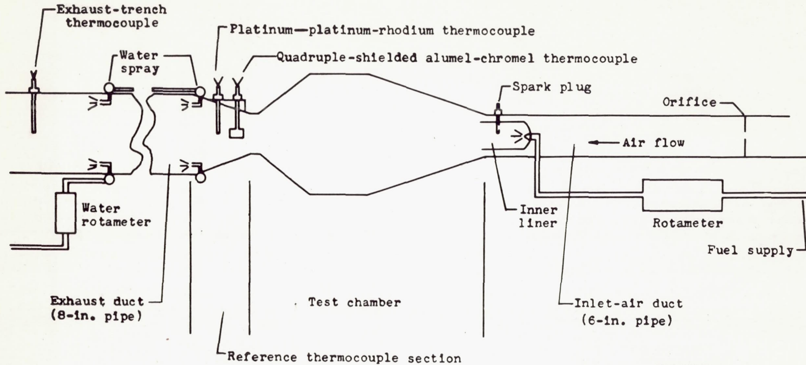
Figure 3. - Schematic diagram of ceramic-lined combustion-chamber test unit.
