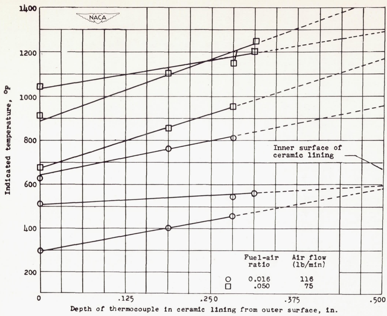
Figure 5. - Temperature gradient through ceramic lining for two fuel-air ratios and air flows.
