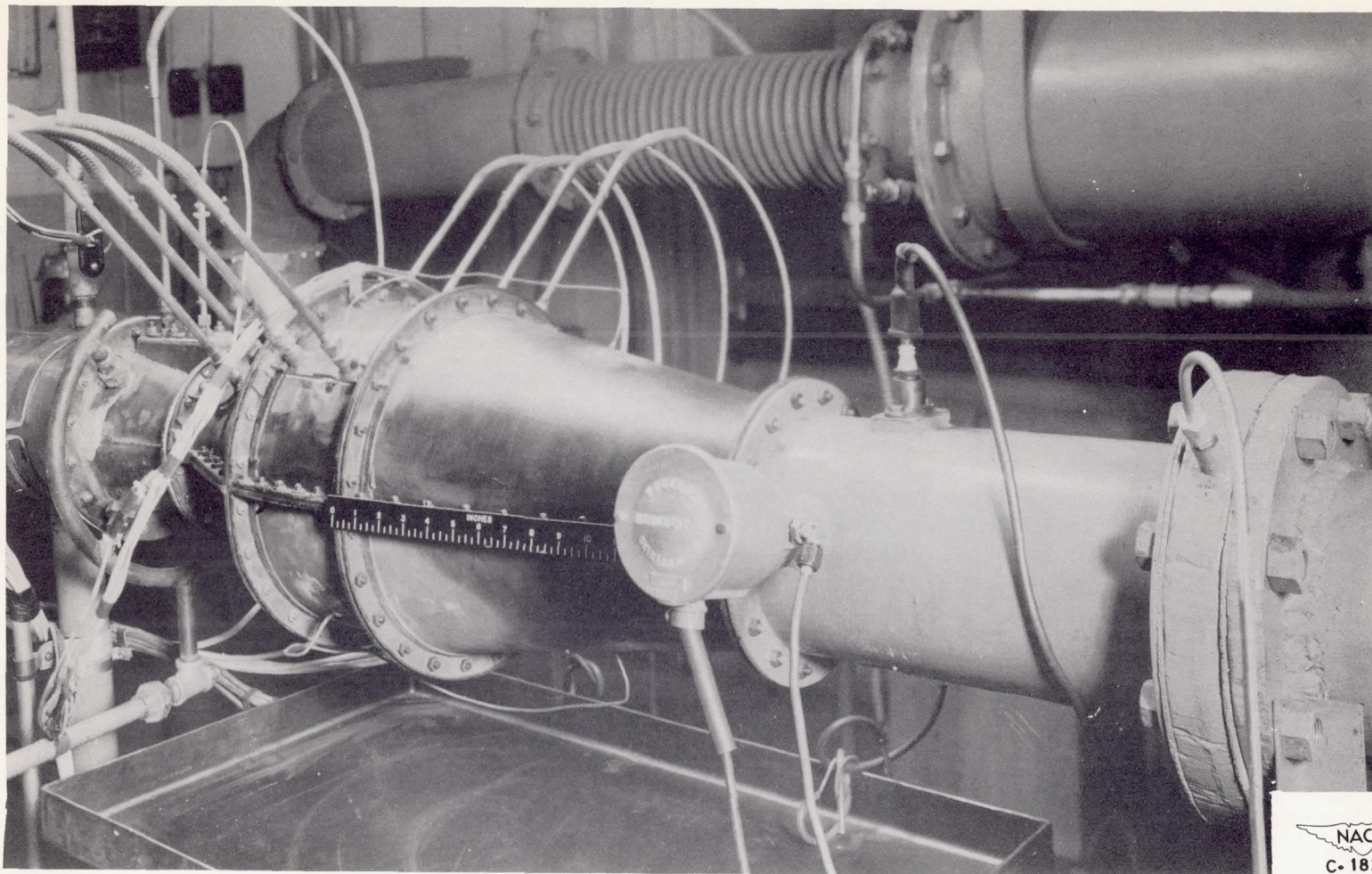
Figure 2. - Photograph of test unit. Air-flow direction from right to left.
