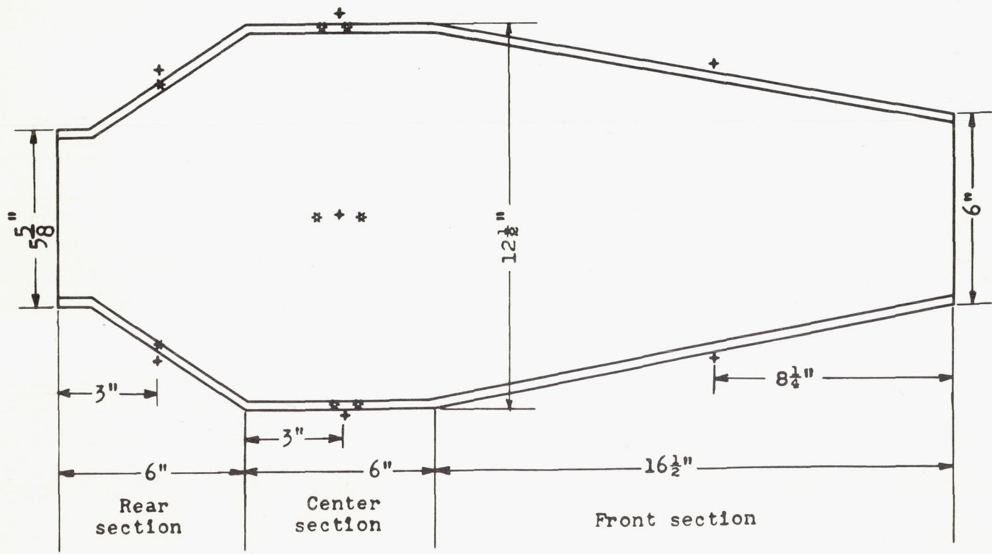
Figure 1. - Sketch showing location of thermocouples installed on outside surface of metal housing and embedded in ceramic lining and dimensions of test chamber.
