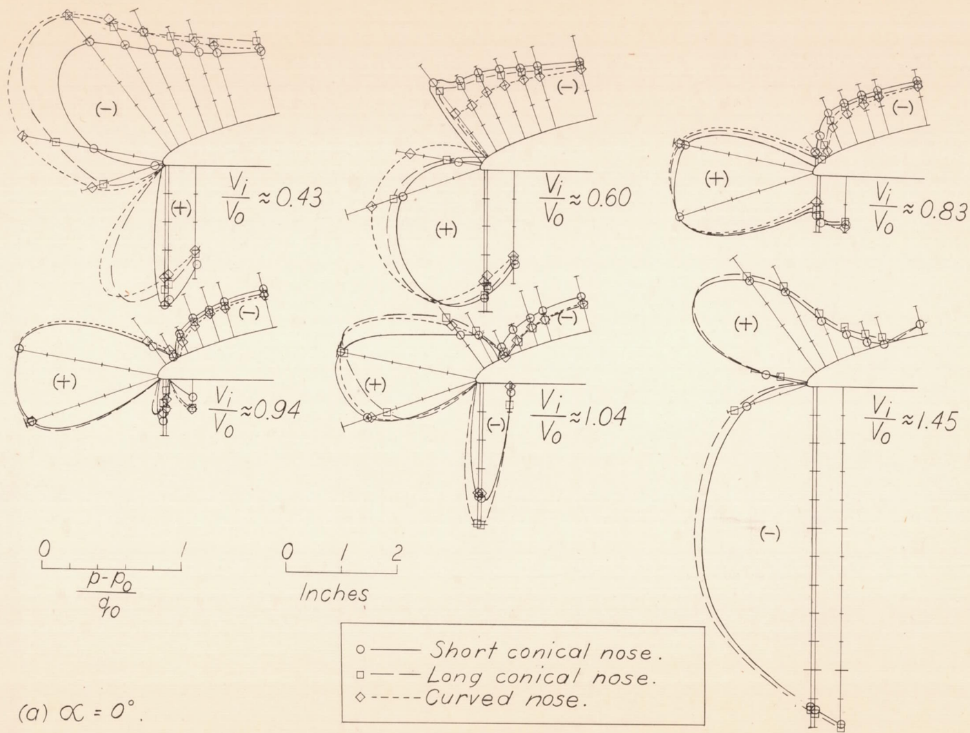
Figure 10. -Static-pressure distributions around top section of lip of NACA 1-85-050 cowling with the three noses installed.
