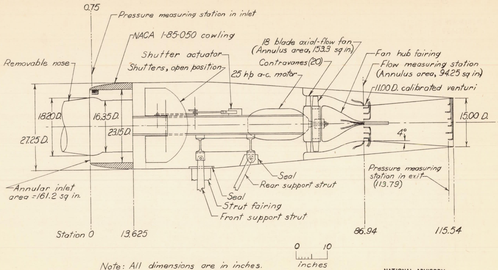
Figure 3.—Schematic drawing of body of model showing the arrangement, instrumentation, and principal dimensions.
