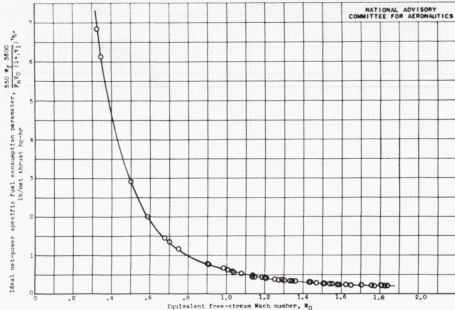
Figure 11.- Effect of equivalent free-stream Mach number M_0 on ideal net-power specific fuel consumption parameter \frac{550 W_f 3600}{F_n V_0 (1 + \sqrt{\tau_1})} \eta_b . 20-inch ram jet with 5-foot combustion chamber and 16.8-inch-diameter exhaust nozzle.
