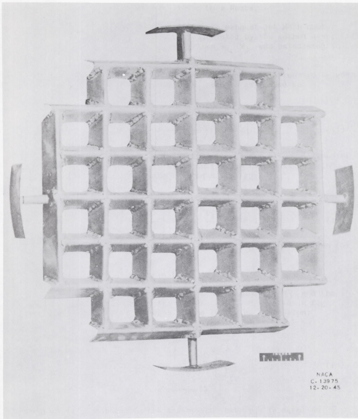
Figure 3. - Flame holder used in wind-tunnel investigation of 20-inch ram jet.
