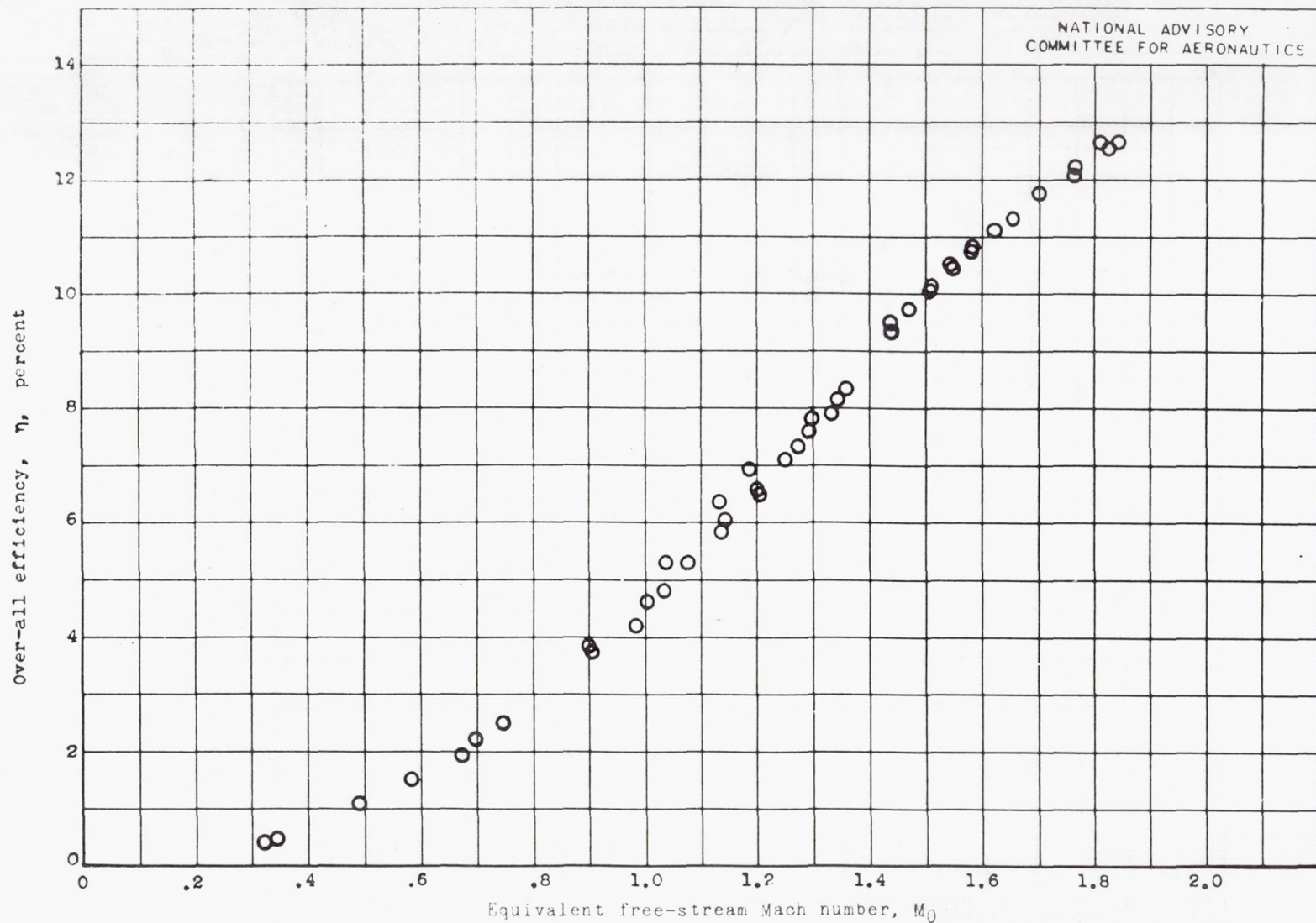
Figure 14.- Effect of equivalent free-stream Mach number M_0 on over-all efficiency \eta . 20-inch ram jet with 5-foot combustion chamber and 13.8-inch-diameter exhaust nozzle.
