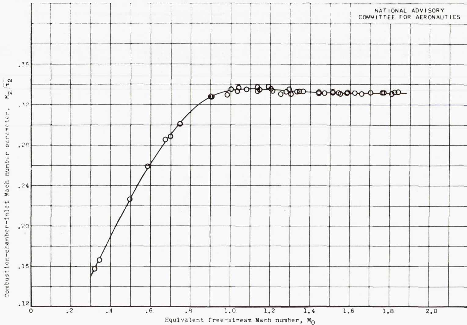
Figure 17.- Effect of equivalent free-stream Mach number M_0 on combustion-chamber-inlet Mach number parameter M_2\sqrt{T_2} . 20-inch ram jet with 5-foot combustion chamber and 16.8-inch-diameter exhaust nozzle.
