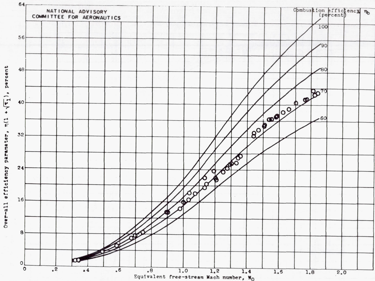
Figure 12.- Effect of equivalent free-stream Mach number M_0 and combustion efficiency \eta_b on over-all efficiency parameter \eta(1 + \sqrt{\tau_1}) . 20-inch ram jet with 5-foot combustion chamber and 16.8-inch-diameter exhaust nozzle.
