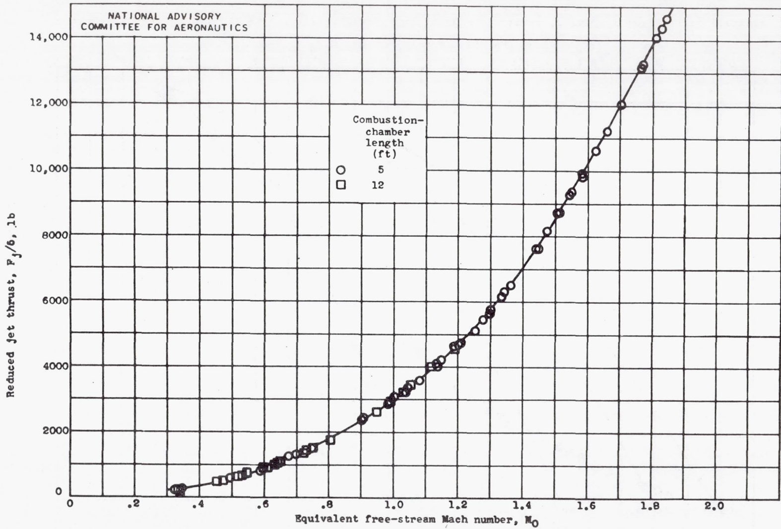
Figure 6.- Effect of equivalent free-stream Mach number M_0 and combustion-chamber length on reduced jet thrust F_j/6 . 20-inch ram jet with 16.8-inch-diameter exhaust nozzle; jet thrust reduced to NACA standard atmospheric conditions at sea level.
