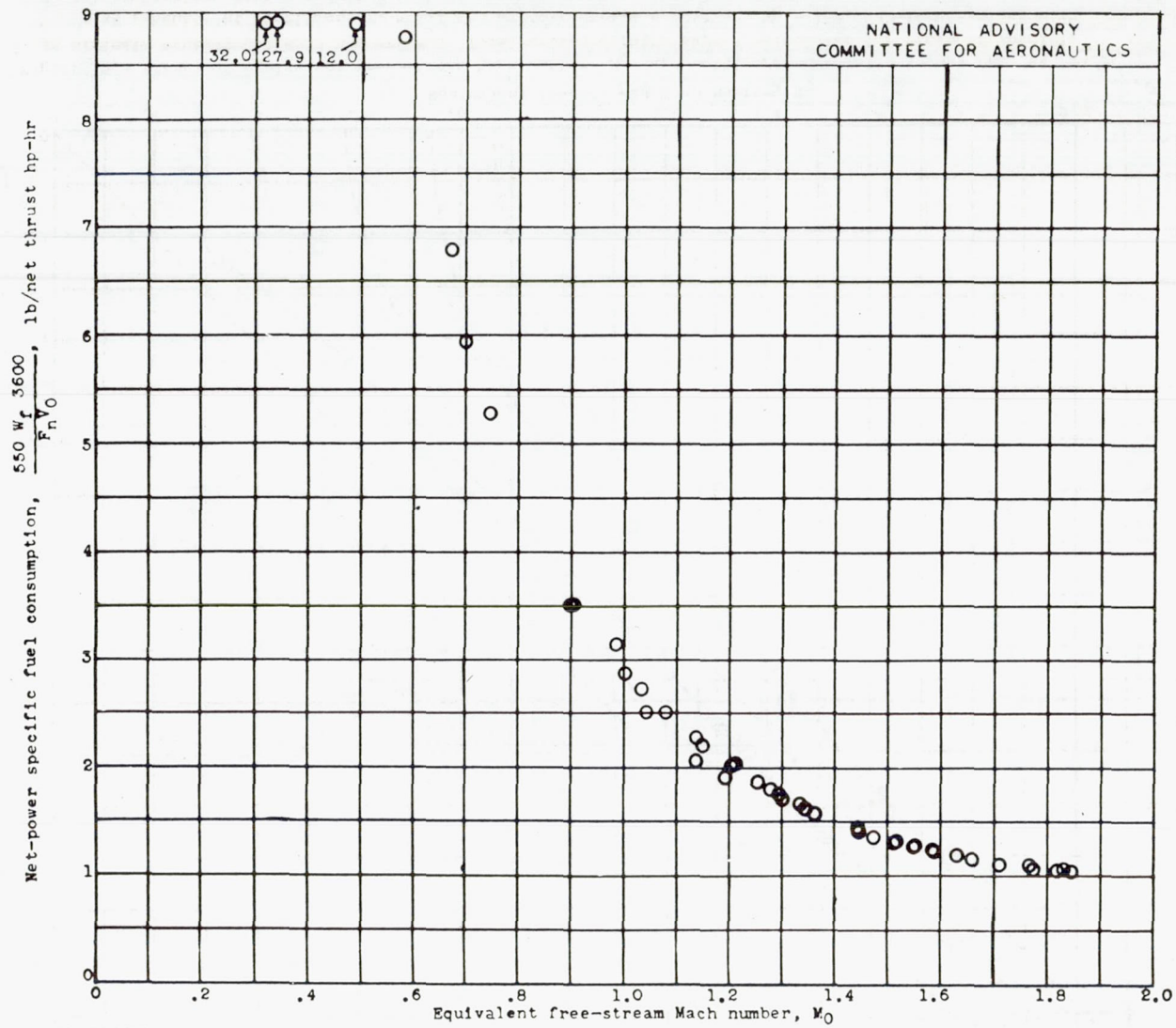
Figure 15.- Effect of equivalent free-stream Mach number M_0 on net-power specific fuel consumption \frac{550 W_f 3600}{F_n V} . 20-inch ram jet with 5-foot combustion chamber and 16.8-inch-diameter exhaust nozzle.
