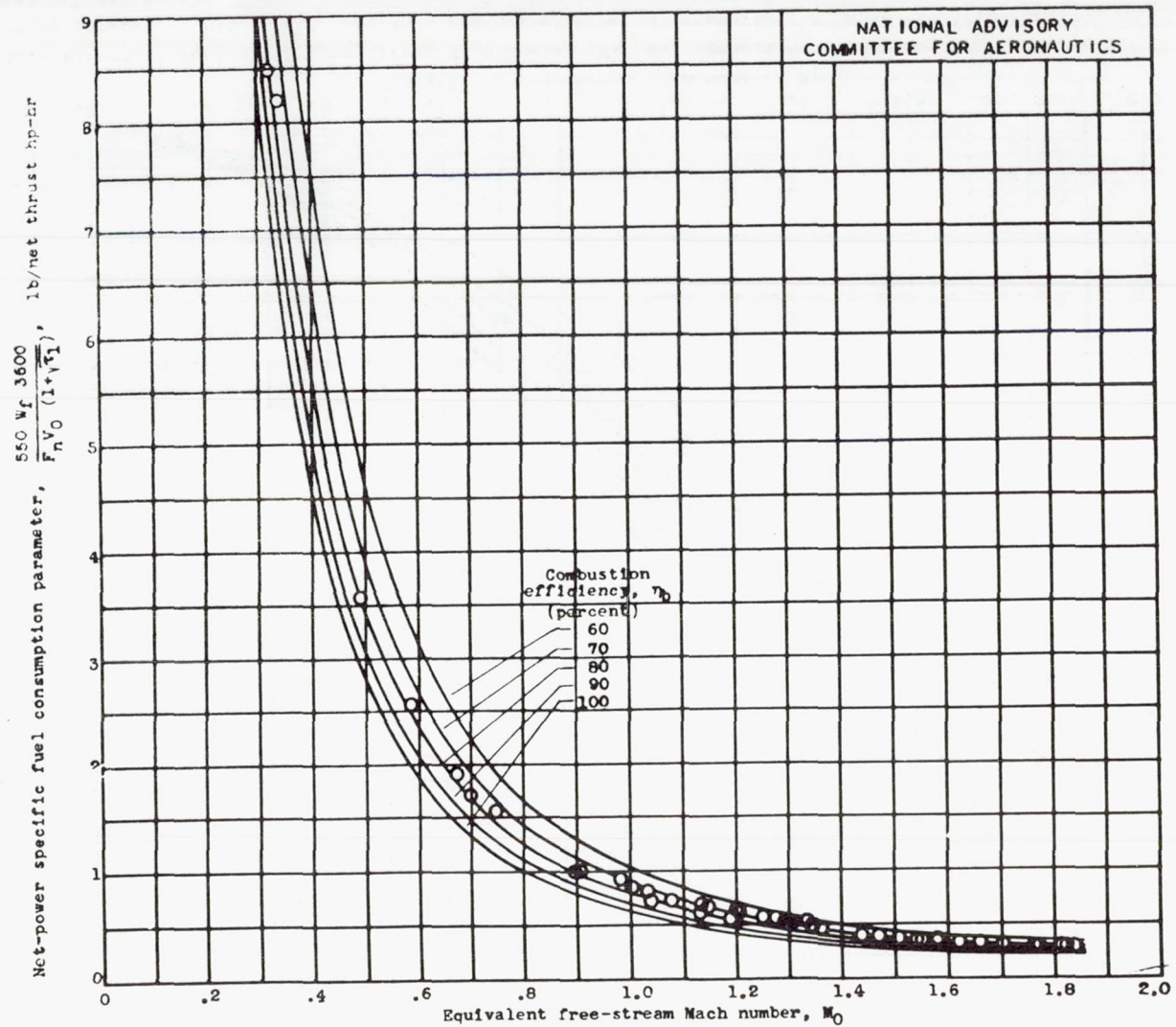
Figure 13.- Effect of equivalent free-stream Mach number M_0 and combustion efficiency \eta_b on net-power specific fuel consumption parameter \frac{550 W_f 3600}{F_n V_0 (1 + \sqrt{\tau_1})} . 20-inch ram jet with 5-foot combustion chamber and 16.8-inch-diameter exhaust nozzle.
