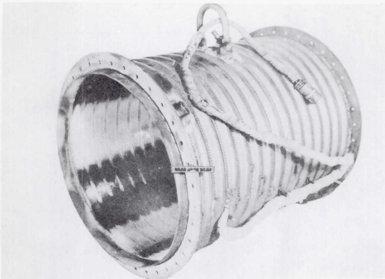
Figure 4. - Modified combustion-chamber section used in wind-tunnel investigation of 20-inch ram jet.
