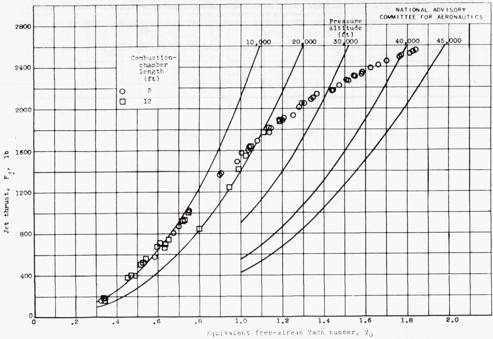
Figure 7.- Effect of equivalent free-stream Mach number M_0 , combustion-chamber length, and pressure altitude on jet thrust F_j . 20-inch ram jet with 12.8-inch-diameter exhaust nozzle.
