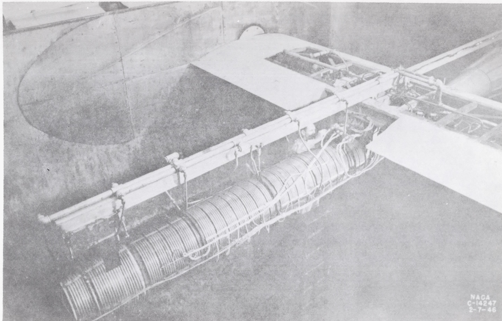
Figure 1.-Installation of 20-inch ram jet with 12-foot combustion chamber and 16.8-inch-diameter exhaust nozzle in altitude wind tunnel.
