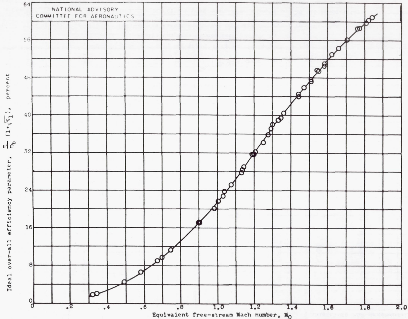
Figure 10.- Effect of equivalent free-stream Mach number M_0 on ideal over-all efficiency parameter \frac{\eta}{\eta_0} (1 + \sqrt{\tau_1}) . 20-inch ram jet with 5-foot combustion chamber and 16.8-inch-diameter exhaust nozzle.
