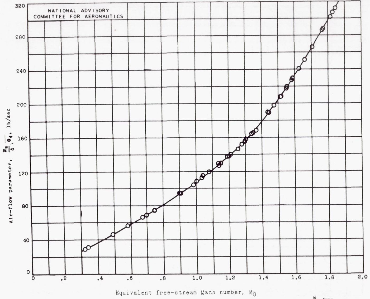
Figure 18.—Effect of equivalent free-stream Mach number M_0 on air-flow parameter \frac{W_a}{s} \sqrt{\theta_4} . 20-inch ram jet with 5-foot combustion chamber and 16.8-inch-diameter exhaust nozzle.
