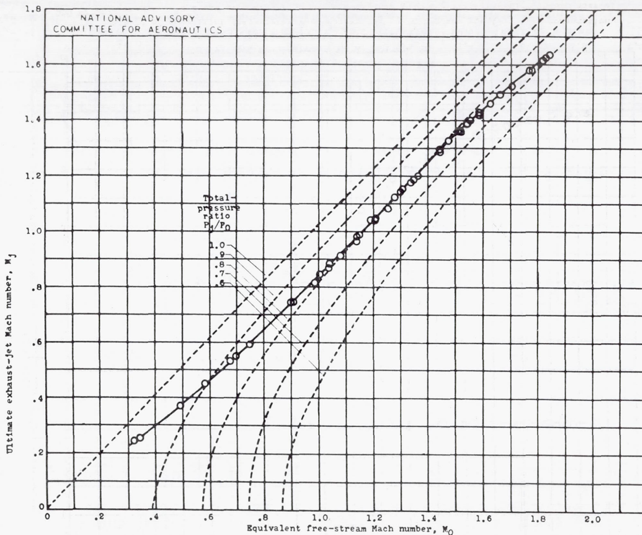
Figure 16.- Effect of equivalent free-stream Mach number M_0 and total-pressure ratio across ram jet P_j/P_0 on ultimate exhaust-jet Mach number M_j . Total-pressure ratio curves calculated for ratio of specific heats at exhaust-jet condition \gamma_j = 1.3 and at free-stream condition \gamma_0 = 1.4 . 20-inch ram jet with 5-foot combustion chamber and 16.8-inch-diameter exhaust nozzle.
