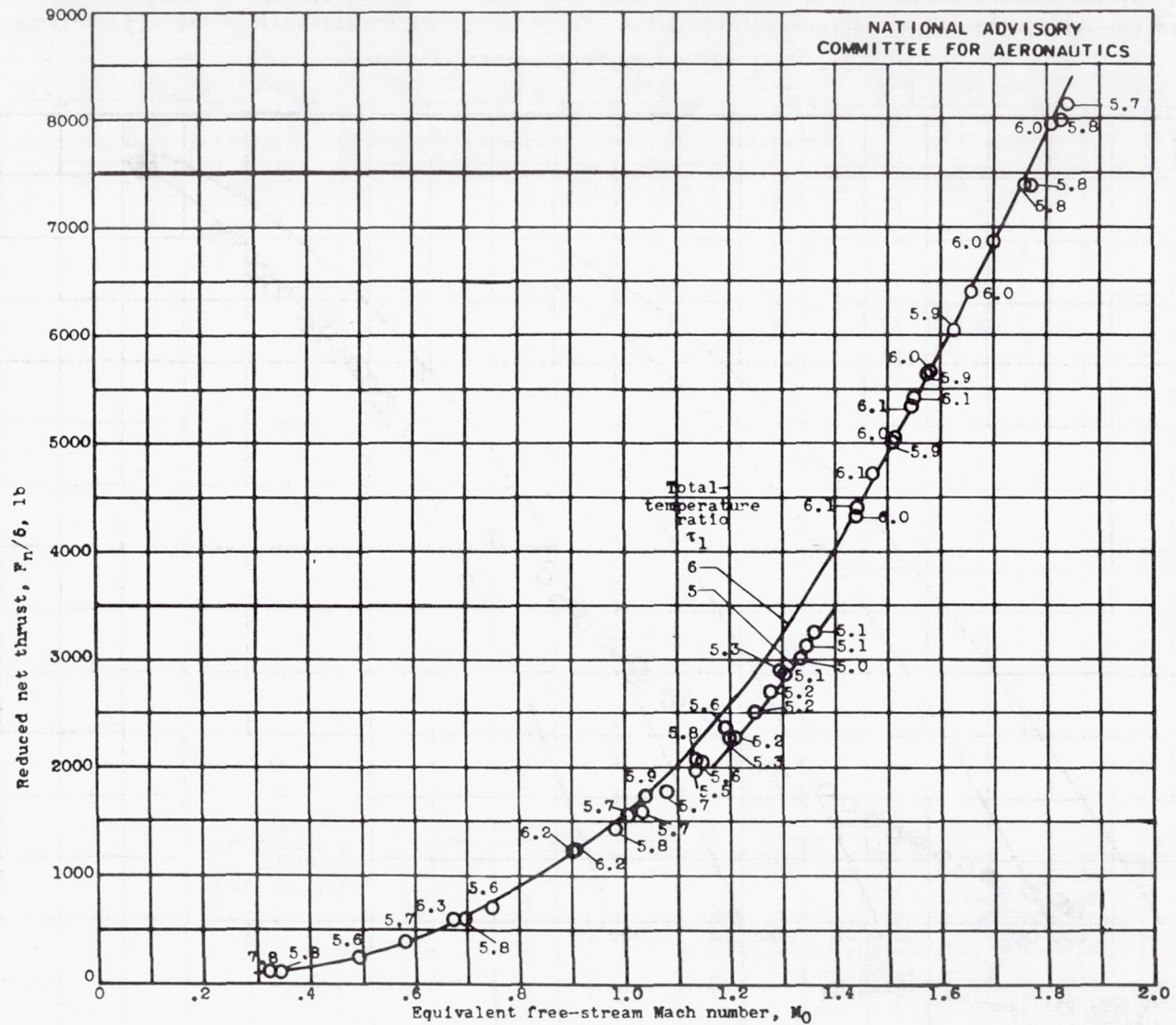
Figure 8.- Effect of equivalent free-stream Mach number M_0 and total-temperature ratio \tau_1 on reduced net thrust F_n/b . 20-inch ram jet with 5-foot combustion chamber and 16.8-inch-diameter exhaust nozzle; net thrust reduced to NACA standard atmospheric conditions at sea level.
