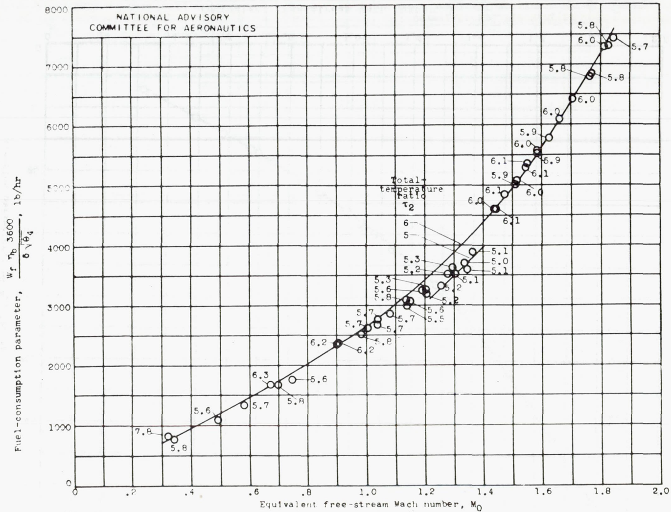
Figure 19.- Effect of equivalent free-stream Mach number M_0 and total-temperature ratio \tau_2 on fuel-consumption parameter \frac{W_f \eta_b 3600}{\delta \sqrt{\theta_4}} . 20-inch ram jet with 5-foot combustion chamber and 16.8-inch-diameter exhaust nozzle.
