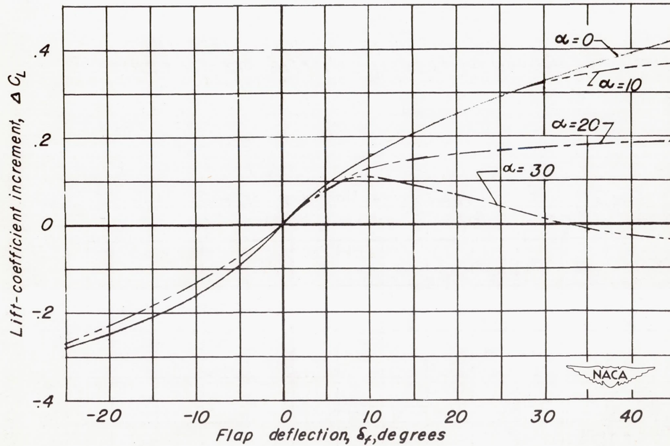
Figure 12.— The effect of flap deflection on the lift coefficient of the wing.
