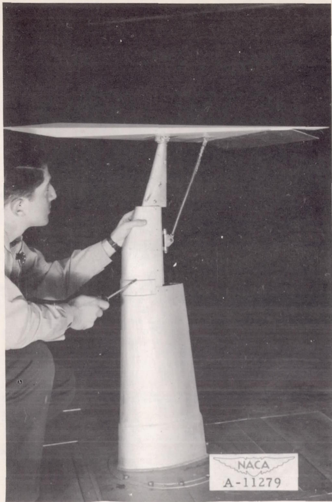
(a) Wing with split flaps.
