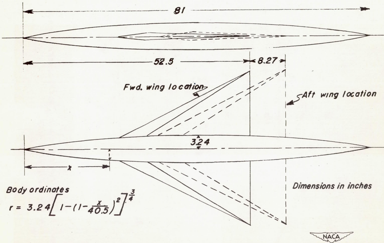
Figure 2.—The body of fineness ratio 12.5 with the two wing locations.
