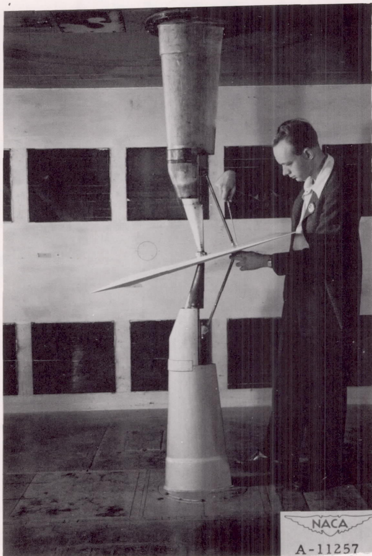
Figure 6.— The image-strut system used to evaluate strut tares.
