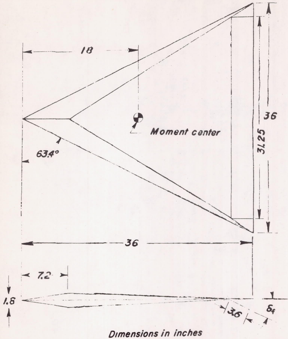
Figure 1.- The triangular wing with constant-chord, trailing-edge, split flap.
