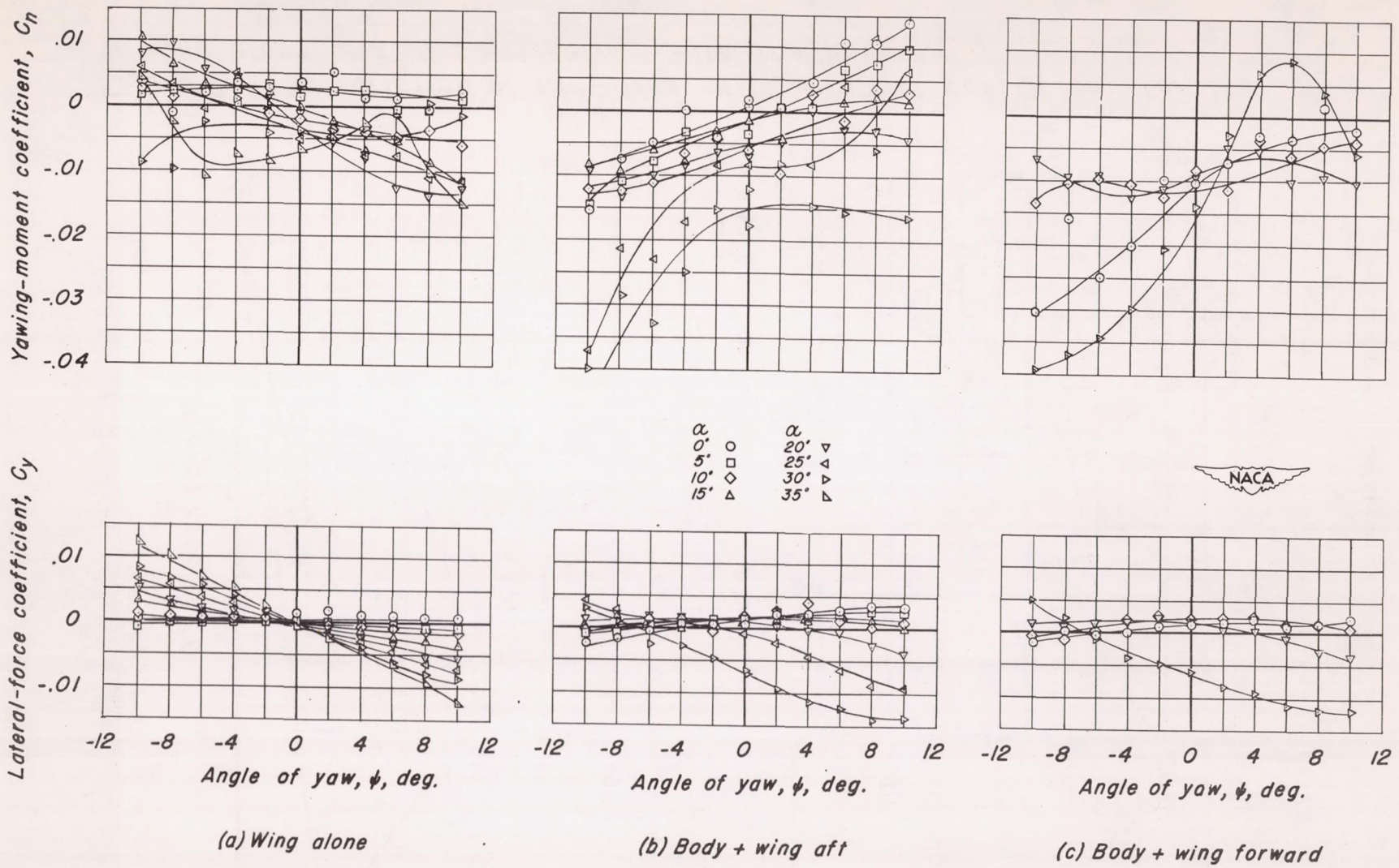
Figure 9.- The effect of angle of attack on the lateral characteristics of the model
