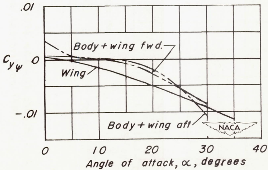
Figure 10.— The variation of the parameters C_{n\psi} and C_{y\psi} with angle of attack.
