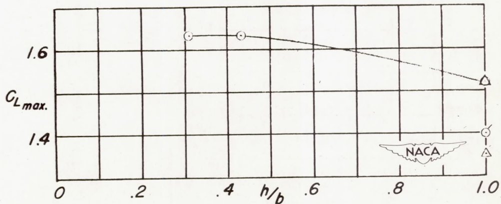
Figure 14.- The effect of height above the ground plane on the longitudinal characteristics of the model.
