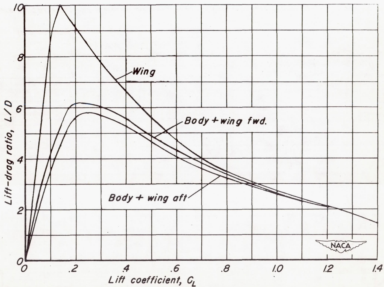
Figure 8.—The variation of lift-drag ratio with lift coefficient for the wing alone and in combination with the body.
