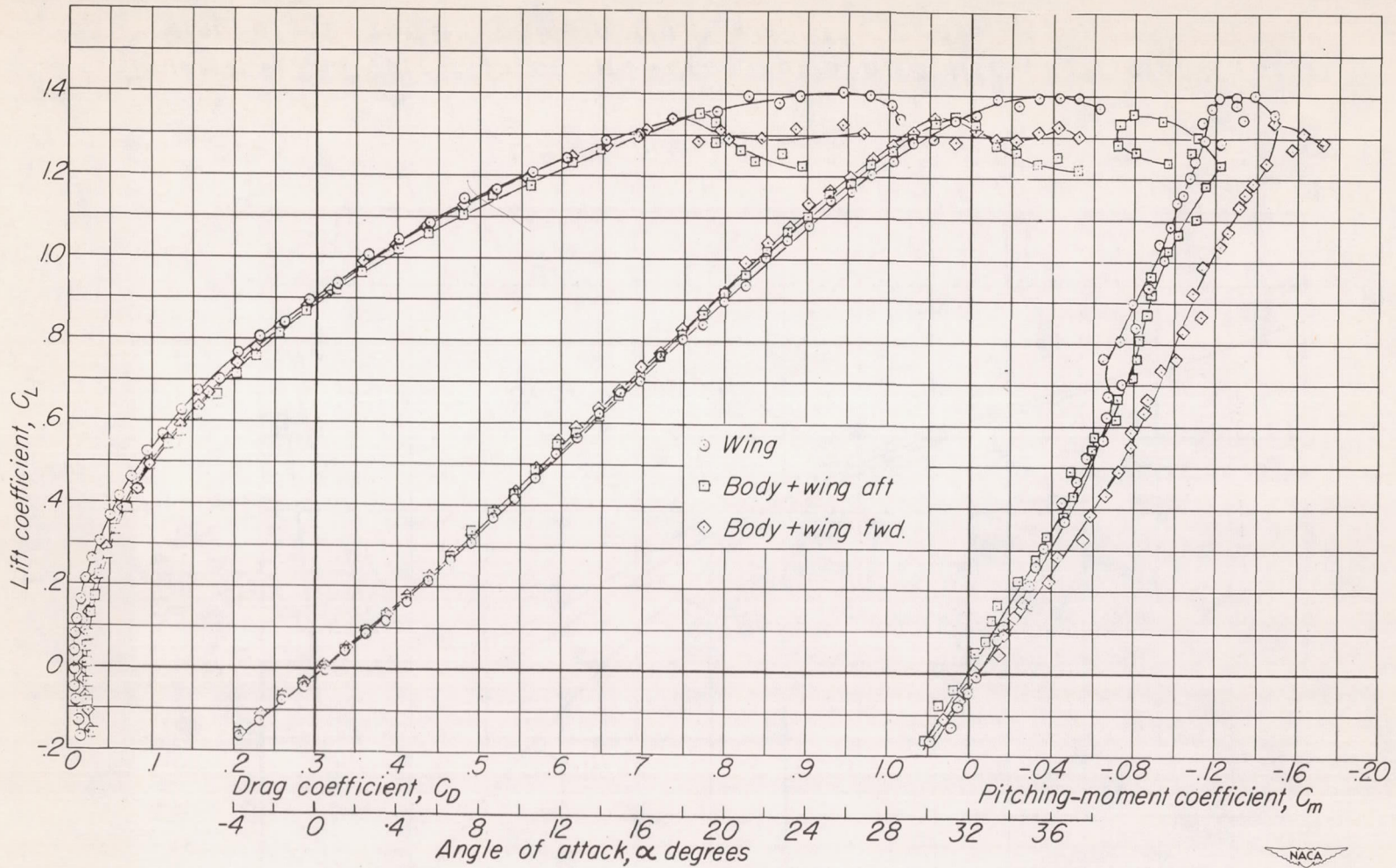
Figure 7.- Lift, drag and pitching-moment coefficients for wing and wing-body combinations.
