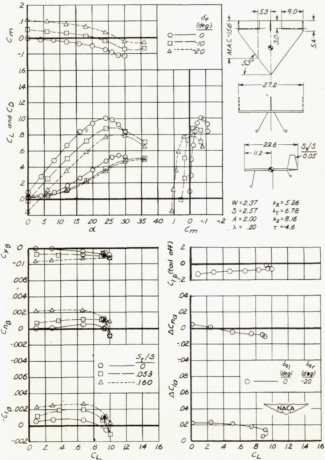
Figure 2.- Aerodynamic characteristics of model 2.
