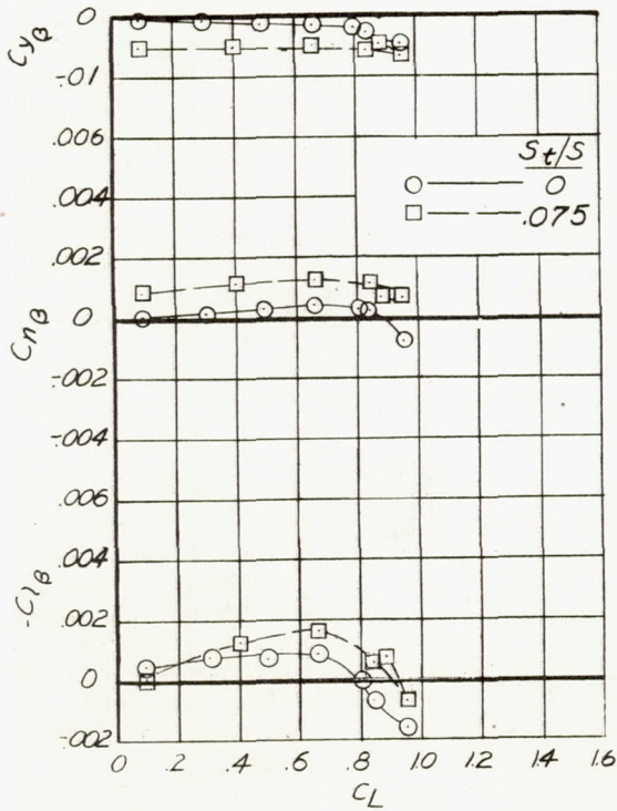
Figure 1.- Aerodynamic characteristics of model 1.
