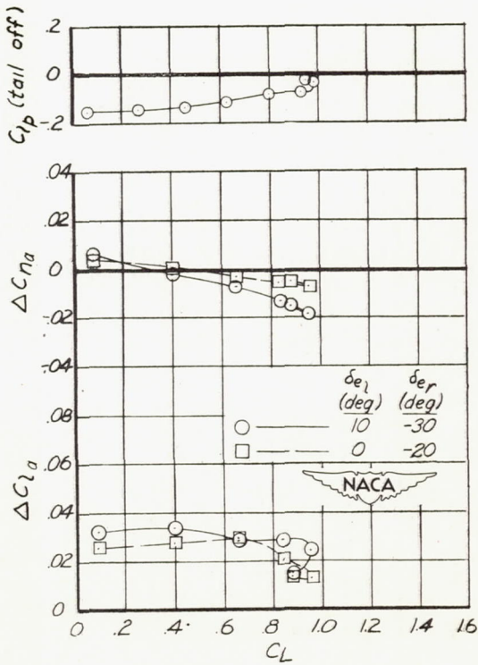
Figure 1.- Aerodynamic characteristics of model 1.
