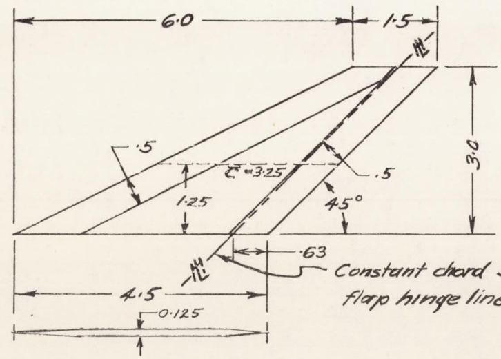
Figure 2. — Detail dimensions of the low aspect ratio wing control model series. CONFIDENTIAL
