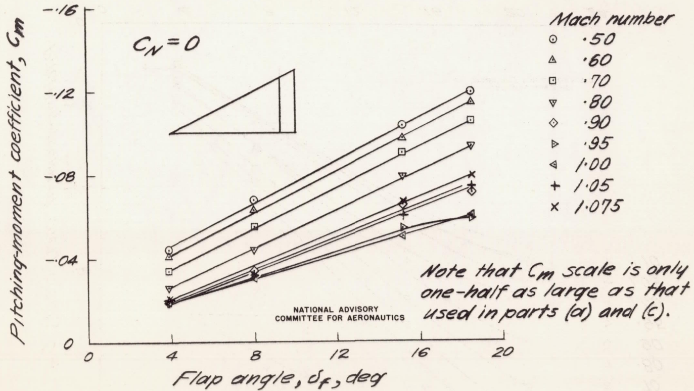
(b) Constant-chord flap
