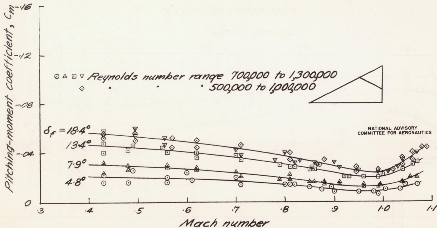
(a) Triangular drooped-tip flap
