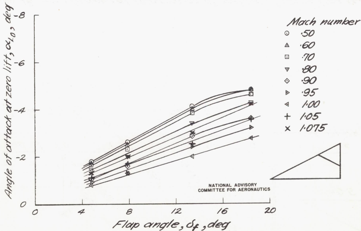
(a) Triangular drooped-tip flap
