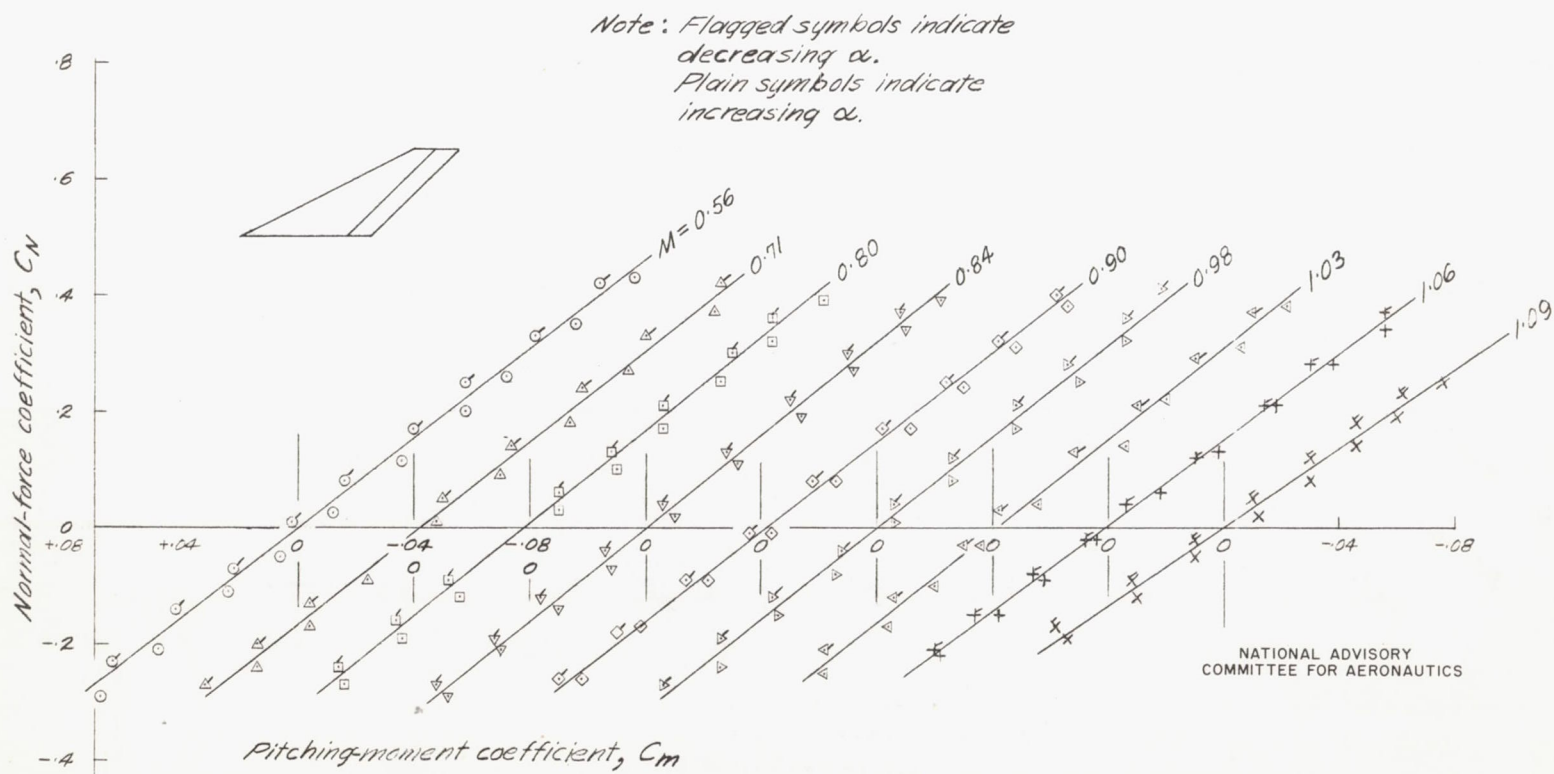
Figure 13. — Variation of pitching-moment coefficient with normal-force coefficient at various Mach numbers for swept-back planform, \delta_f=0^\circ .
