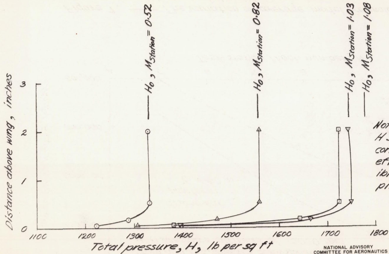
(c) Typical boundary layer profiles as measured at the test station for several test station Mach numbers
