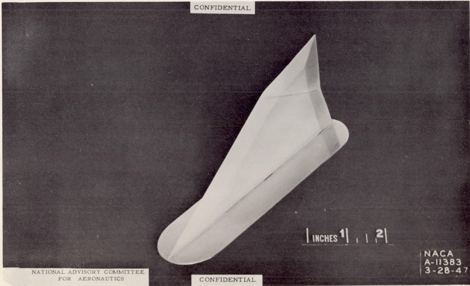
Figure 3.- Low-aspect-ratio wing-control model with end plate attached.
