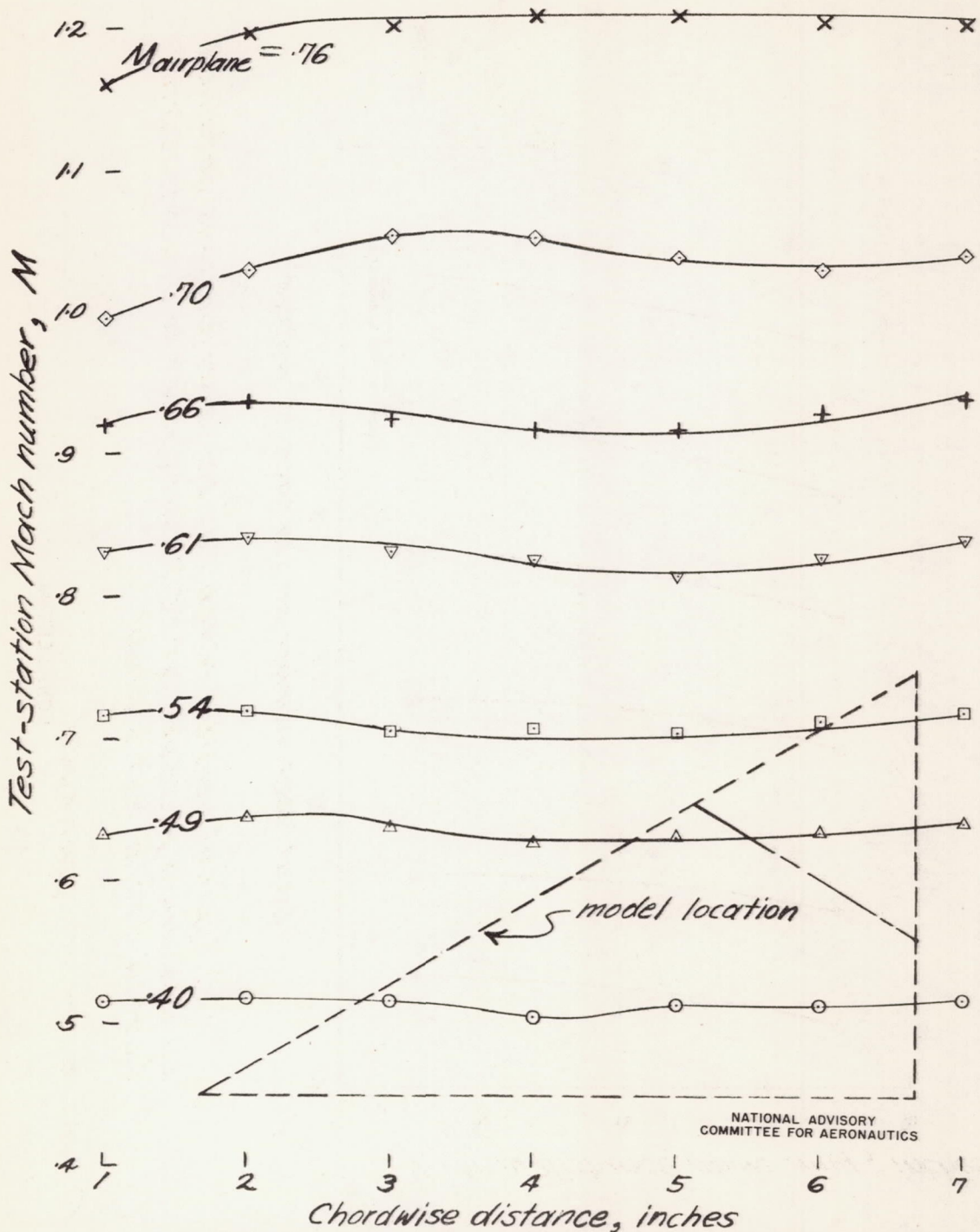
(a) Typical chordwise Mach number distributions Figure 6. — Test station characteristics.
