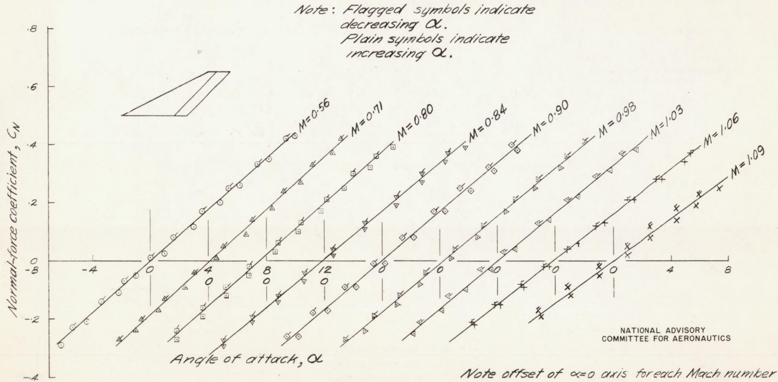
Figure 12. — Variation of normal-force coefficient with angle of attack at various Mach numbers for swept-back platform, \delta_f = 0^\circ .
