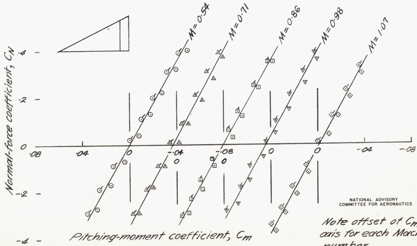
(b) \delta_f = 0^\circ Figure 11. — concluded.
