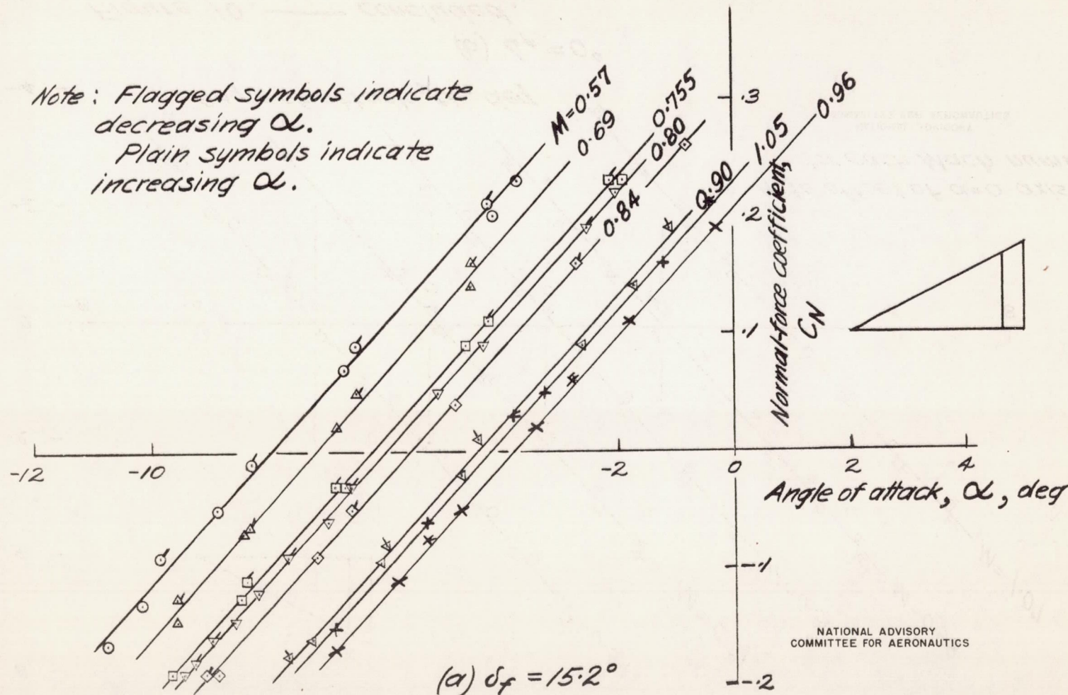
Figure 10. — Variation of normal-force coefficient with angle of attack at various Mach numbers for triangular wing with constant-chord flap.
