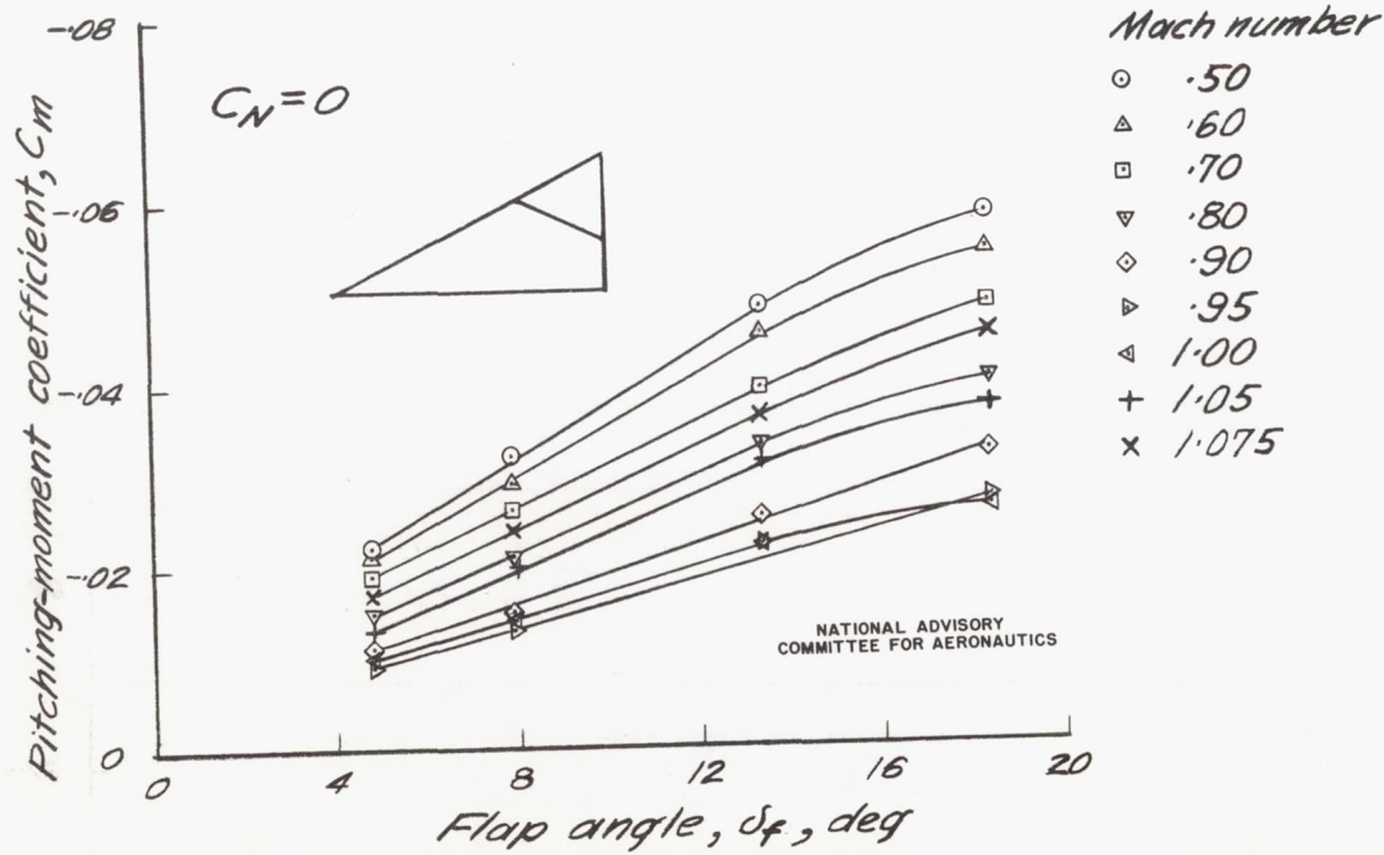
(a) Triangular drooped-tip flap
