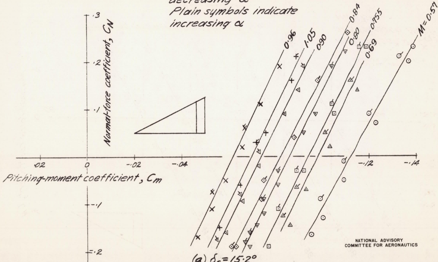
Figure 11. ——— Variation of pitching-moment coefficient with normal-force coefficient at various Mach numbers for triangular wing with constant-chord flap.
