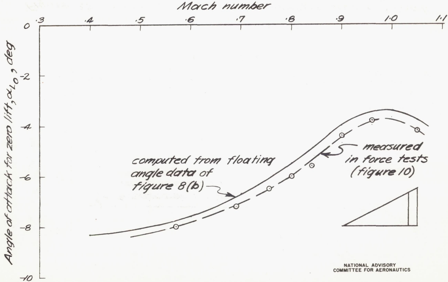
Figure 24. — Variation of angle of attack for zero lift with Mach number for constant-chord flap, \delta_f = 15.2^\circ , comparing results from both test methods.
