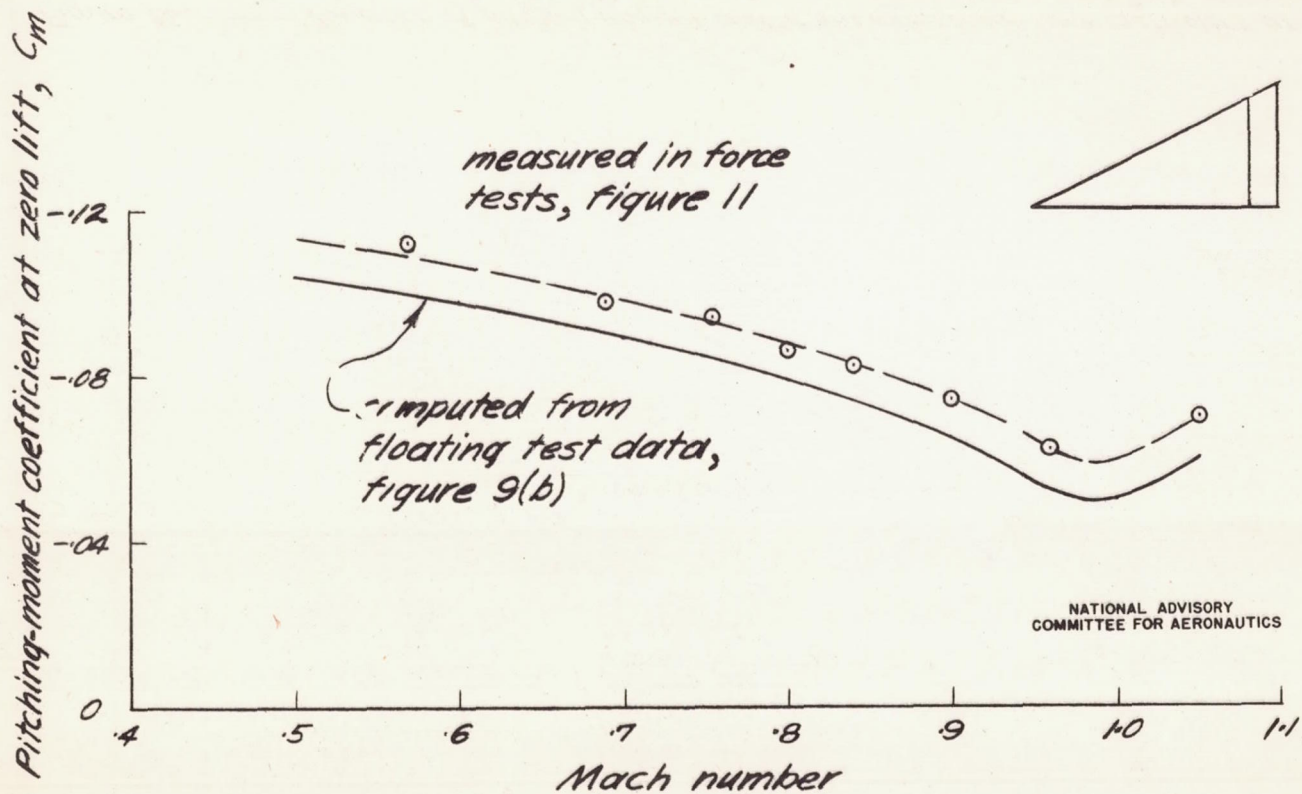
Figure 25. — Variation of pitching-moment coefficient at zero lift with Mach number for constant-chord flap, \delta_f = 15.2^\circ , comparing results from both test methods.
