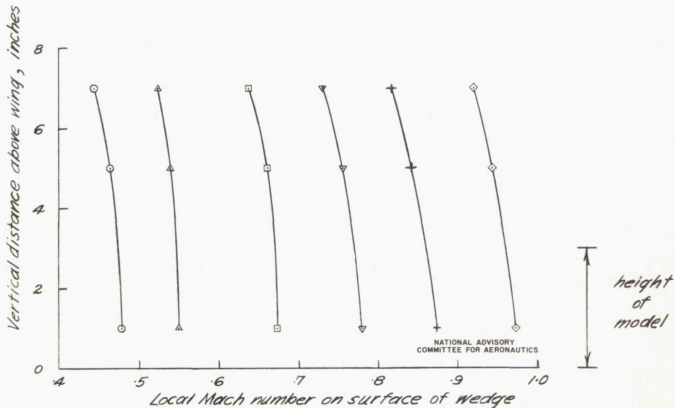
(b) Typical vertical Mach number distributions obtained by measuring pressure at 60% chord point on a wedge airfoil located at the test station
