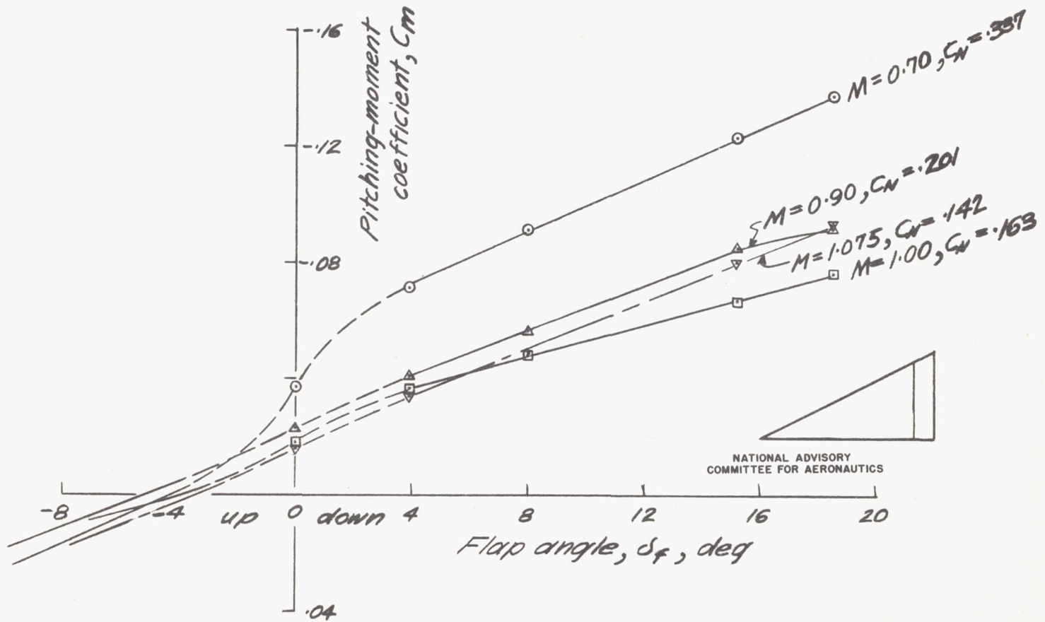
Figure 27. — Variation of pitching-moment coefficient with flap angle at specified Mach numbers and normal-force coefficients.
