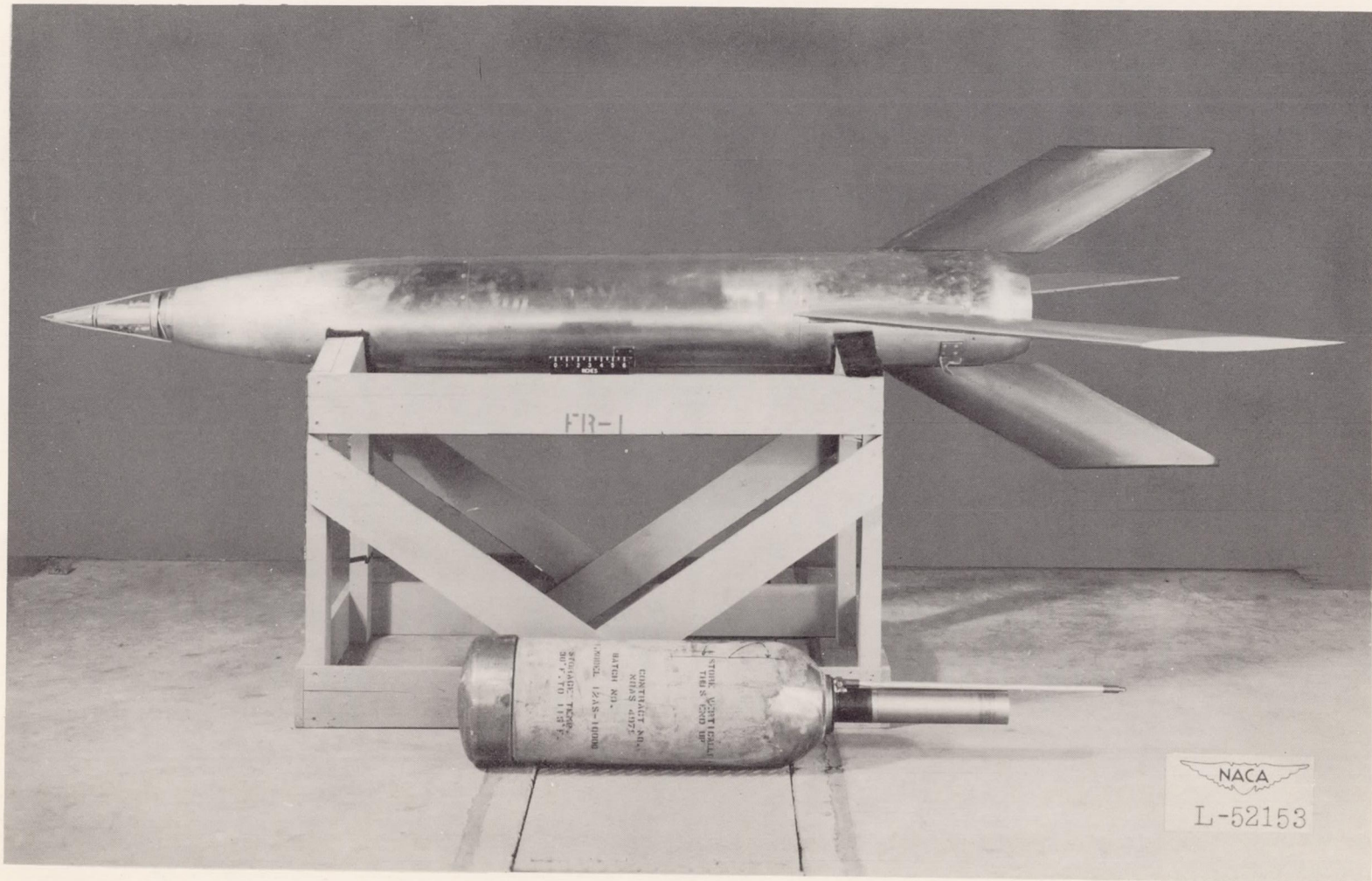
Figure 2.- Side view of the FR-1-A with power plant.
