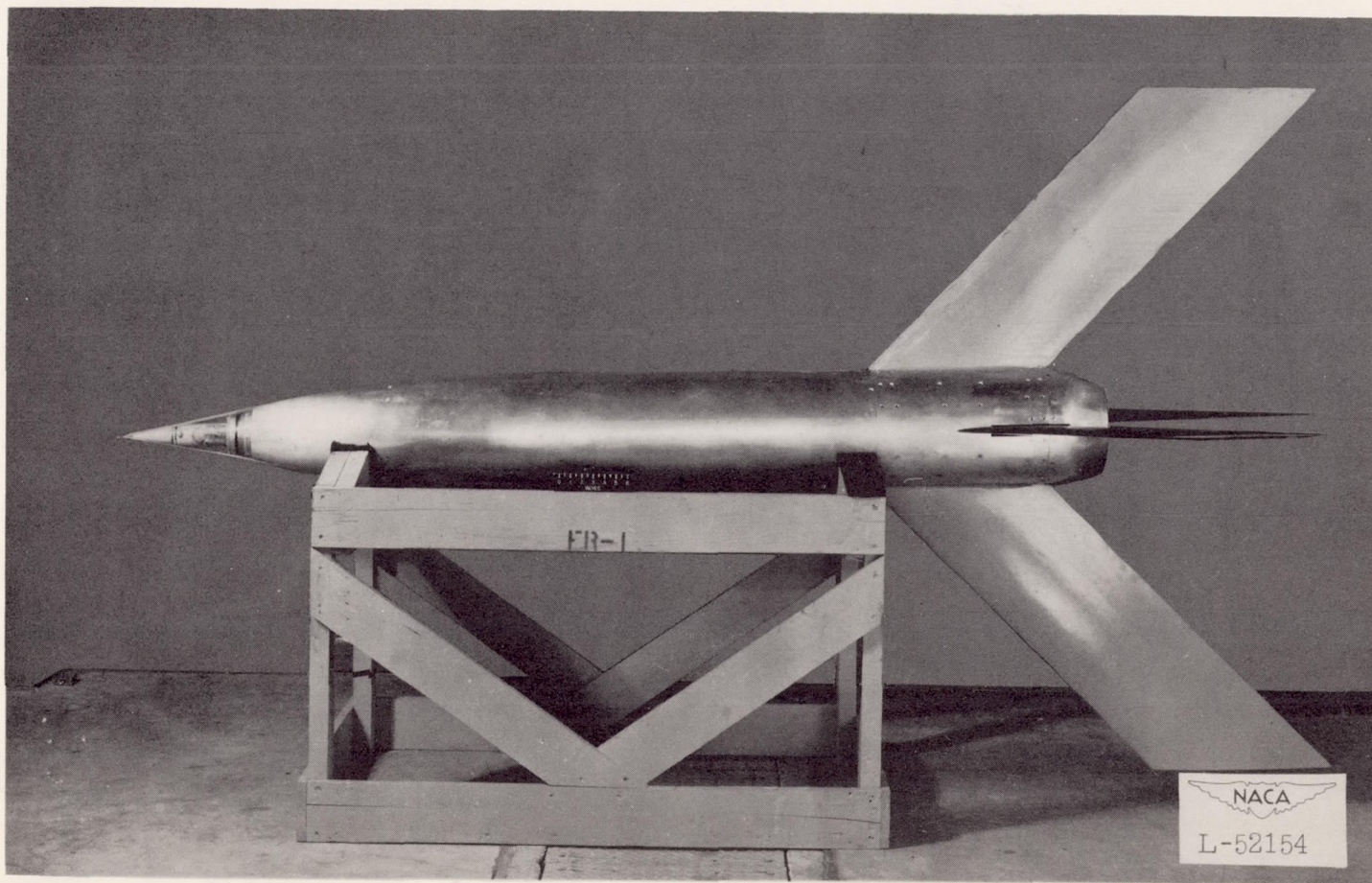
Figure 3.- Top view of the FR-1-A showing the flutter test wings.
