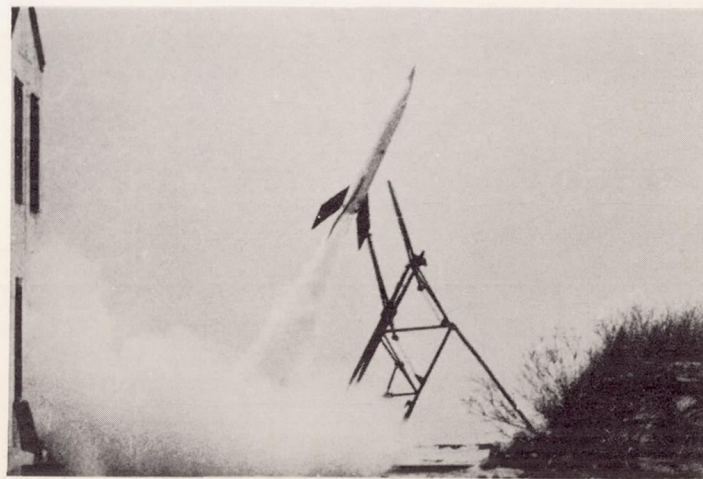
Figure 7.- Sequence of pictures of the launching of the FR-1-A at approximately \frac{1}{4} -second time intervals.
