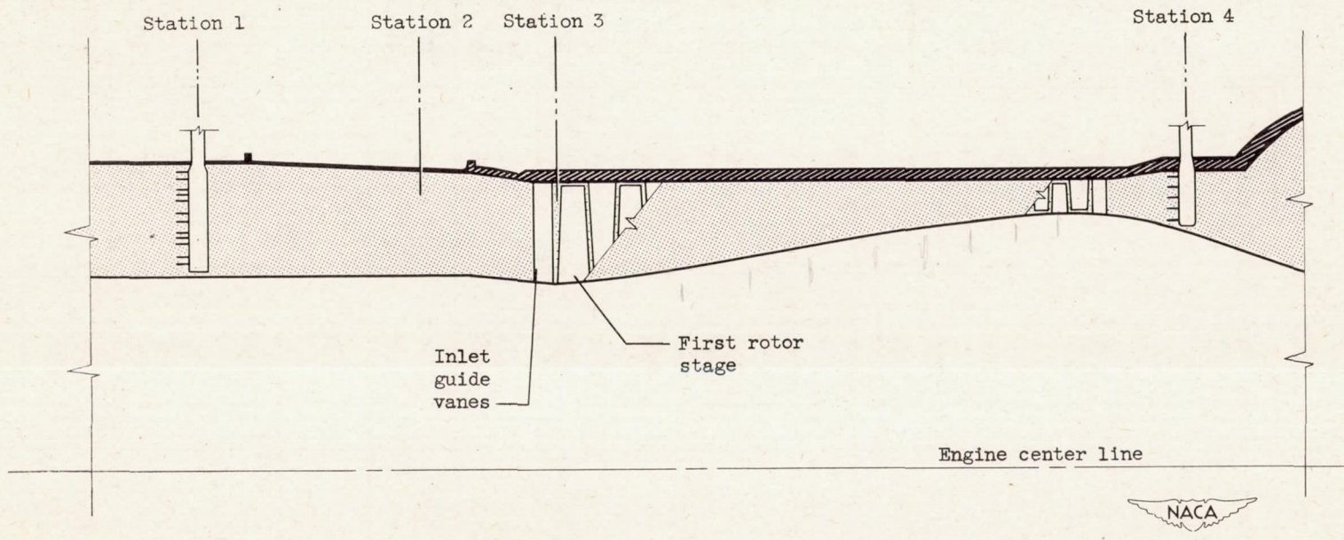
Figure 1. - Schematic view of compressor showing measuring stations.
