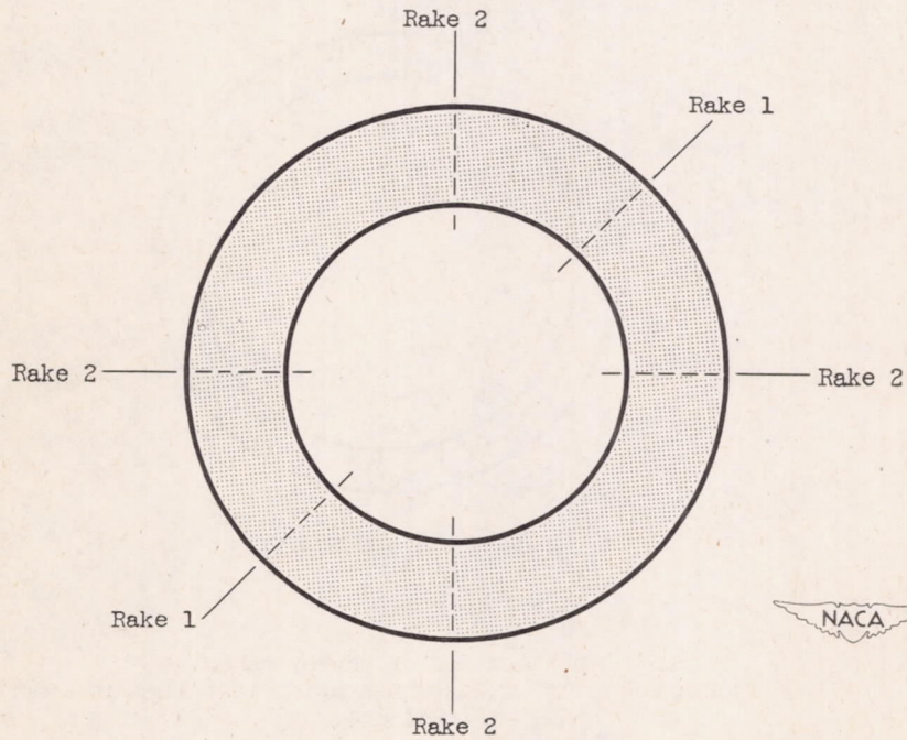
(b) Location of survey rakes. Figure 2. - Location and details of instrumentation installed at engine inlet, station 1.
