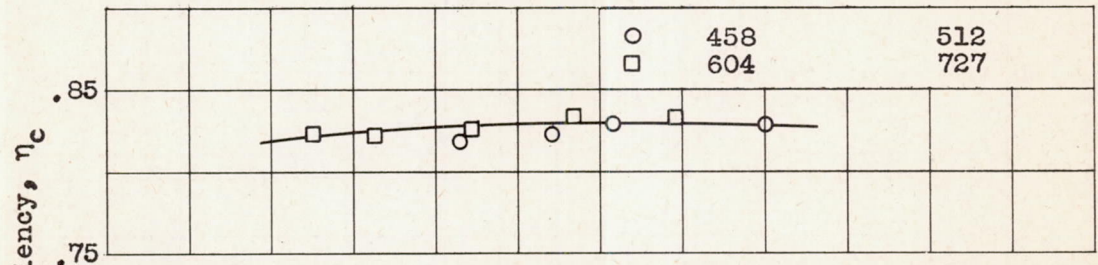
(b) Average compressor-inlet Reynolds number, 132,500.
