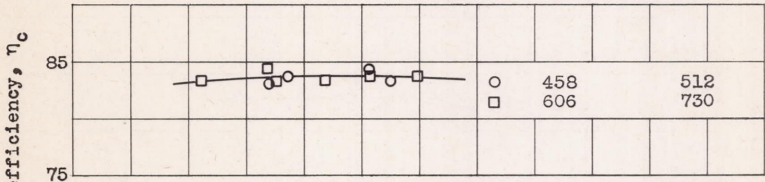
(b) Average compressor-inlet Reynolds number, 124,800.
