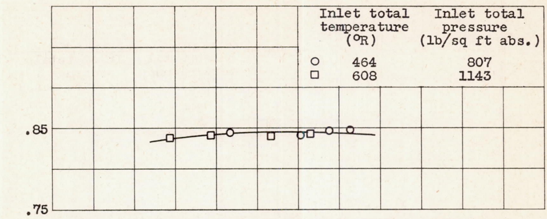
(a) Average compressor-inlet Reynolds number, 207,900.
