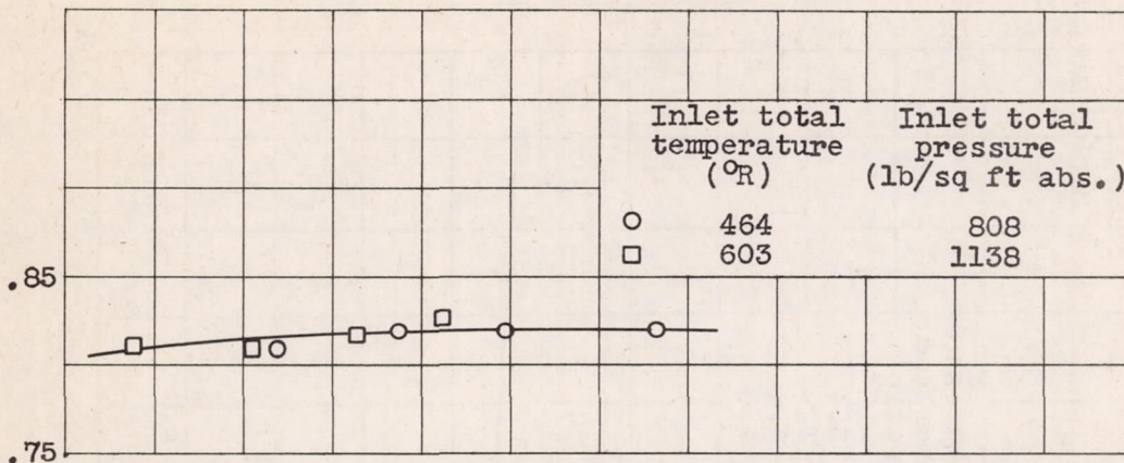
(a) Average compressor-inlet Reynolds number, 218,900.
