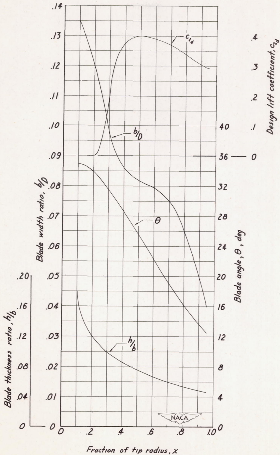
Figure 3.- Blade-form curves for the model propeller.
