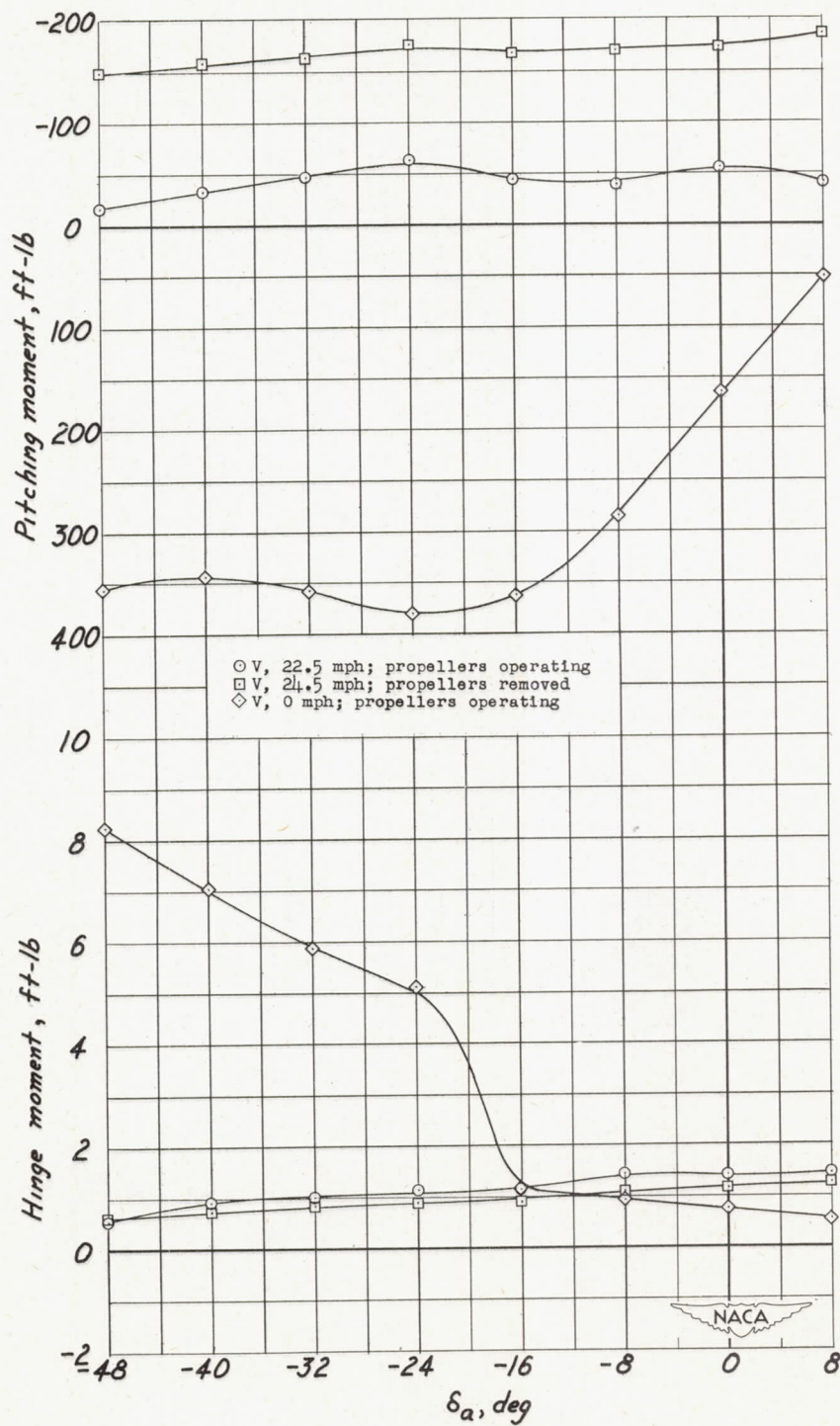
(a) Variation of M and H with \delta_a .
