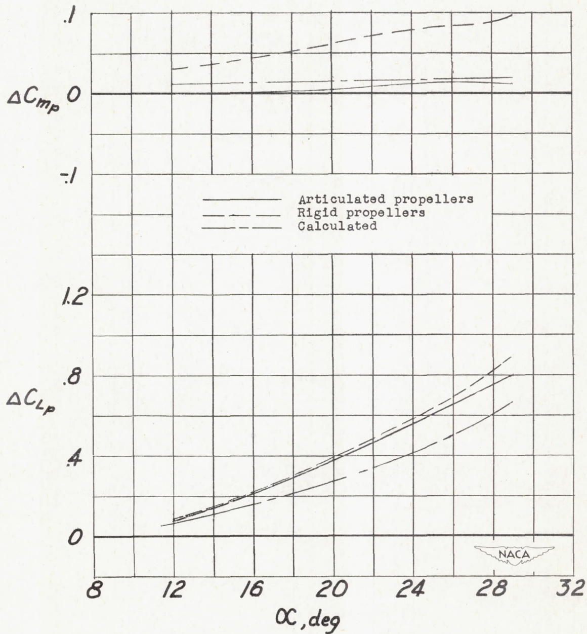
Figure 10.— Increments of pitching moment and lift coefficients due to propeller operation for model with all-movable horizontal tail removed. Full-power operation; \delta_F = 0^\circ .
