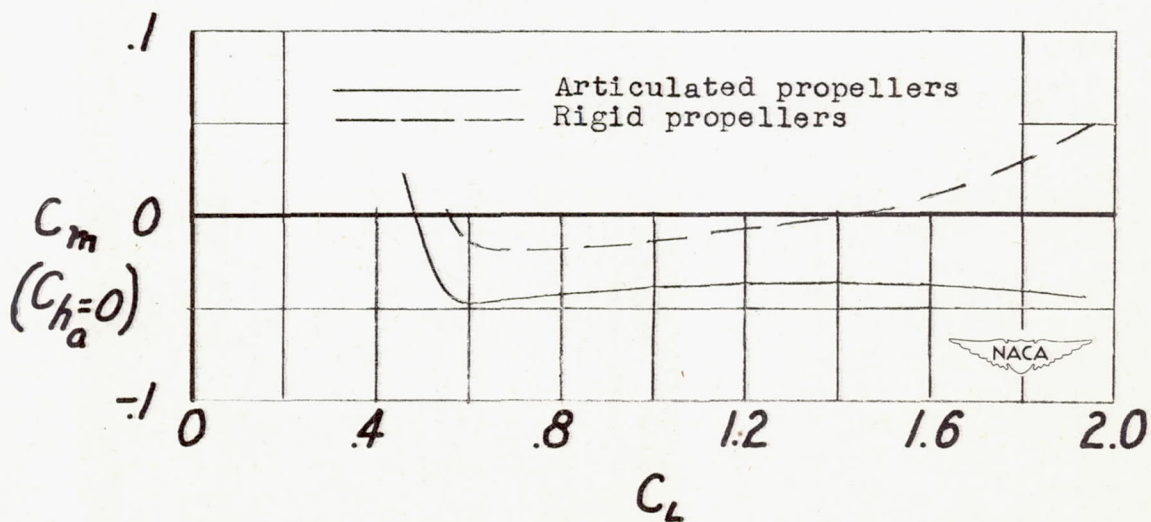
Figure 7.- Effect of propeller articulation on the variation of C_m with C_L stick free for simulated full-power operation.
