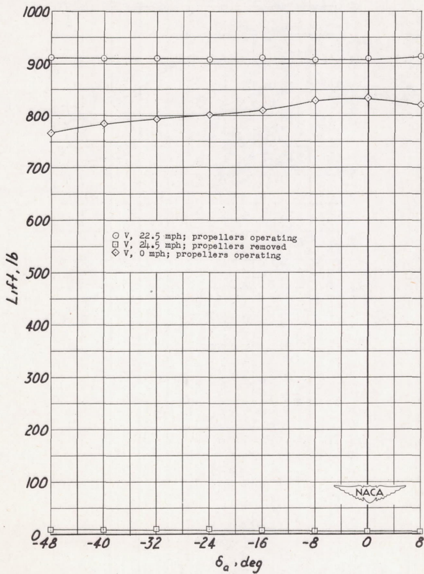
(b) Variation of lift with \delta_a .
