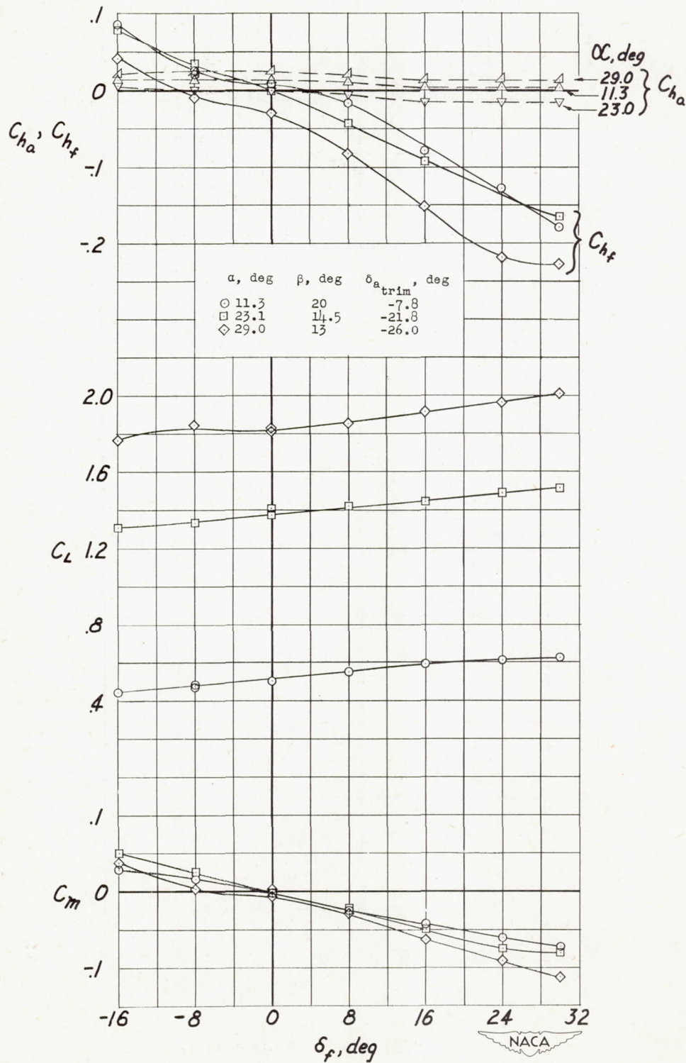
Figure 16.- Variation of C_m , C_L , C_{H_F} , and C_{H_B} with \delta_f for simulated full-power operation with articulated propellers.
