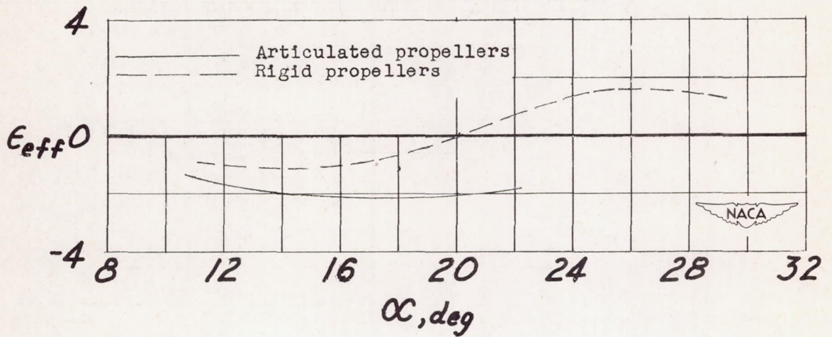
Figure 13.- Effect of propeller articulation of the variation of \epsilon_{eff} with \alpha for simulated full-power operation. \delta_f = 0^\circ .
