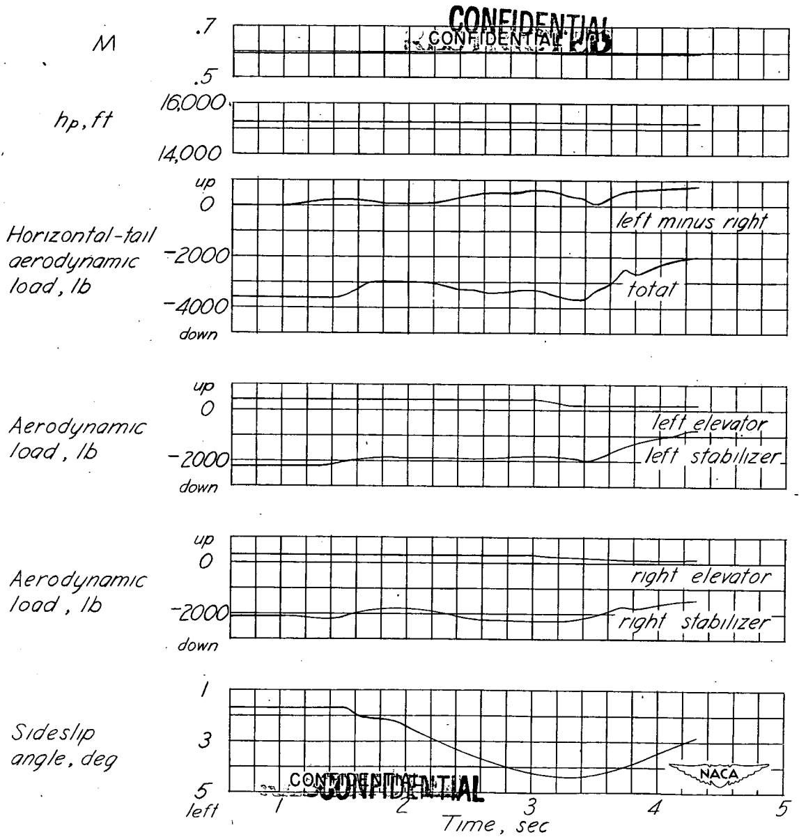
Figure 3.- Time histories of measured quantities during a left roll. Airplane weight, 61,000 pounds; center of gravity at 28.30 percent mean aerodynamic chord.
